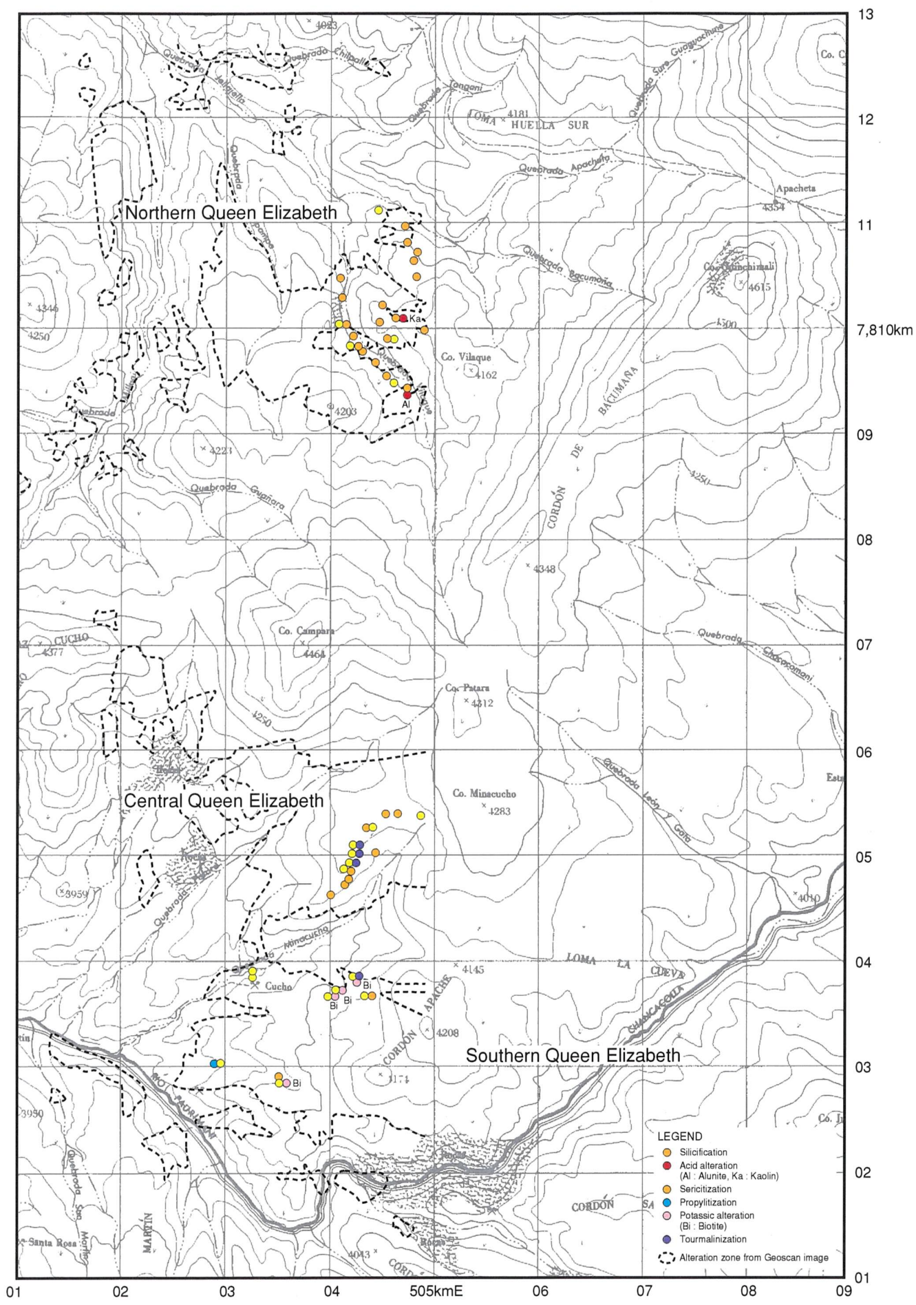
Fig. 2-2-9 Distribution Map of Alteration Minerals at the Queen Elizabeth Area
