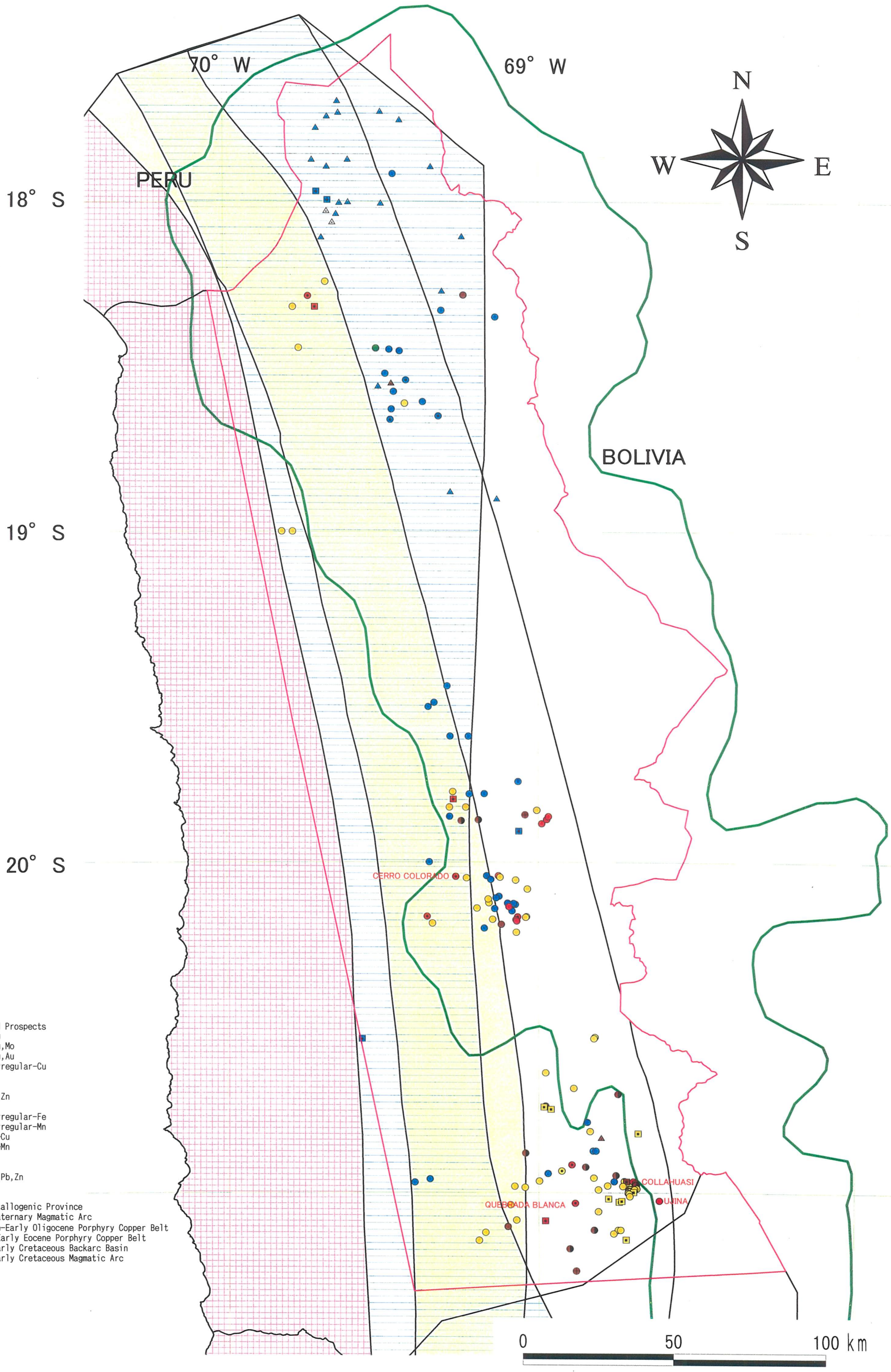
Fig. 2-1-2 Magmatic and Metallogenic Province in the Region I Area
