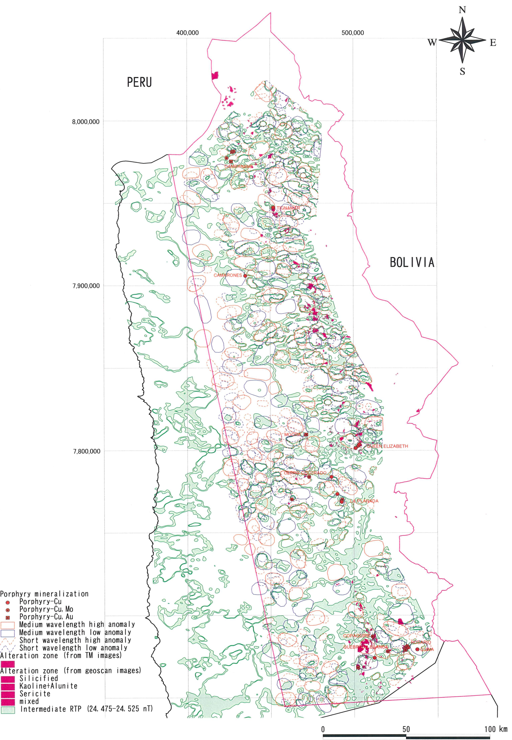
Fig. 1-13 Relationship Between Airborne Magnetic Anomalies and Alteration Zone
