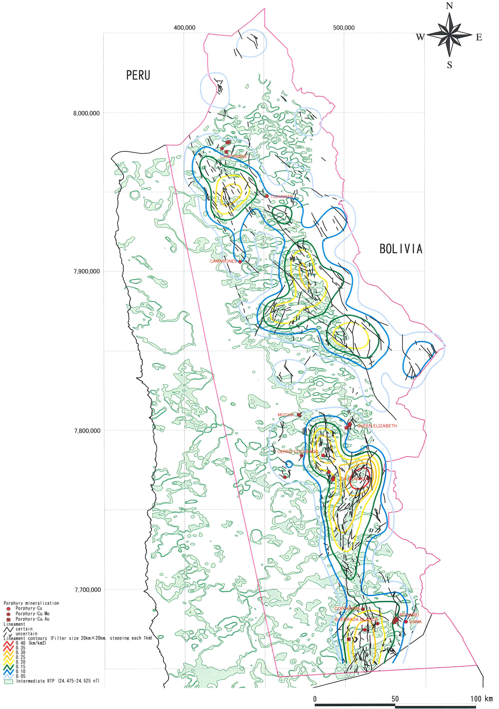
Fig. 1-12 Relationship Between Intermediate Magnetic Intensity Zones and Lineaments
