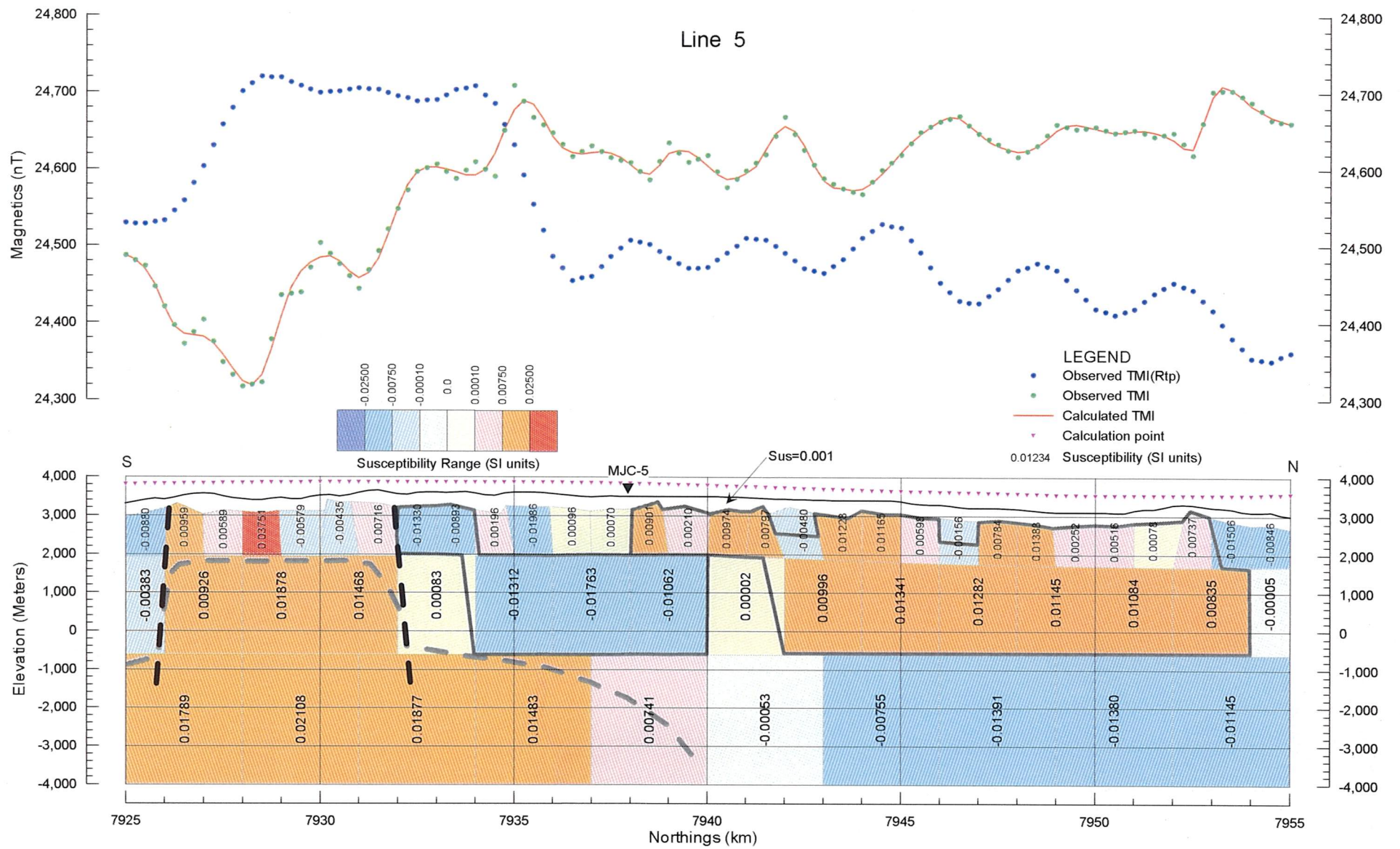
Fig. 2-3-37 Line 5 - 2D Model Profile
