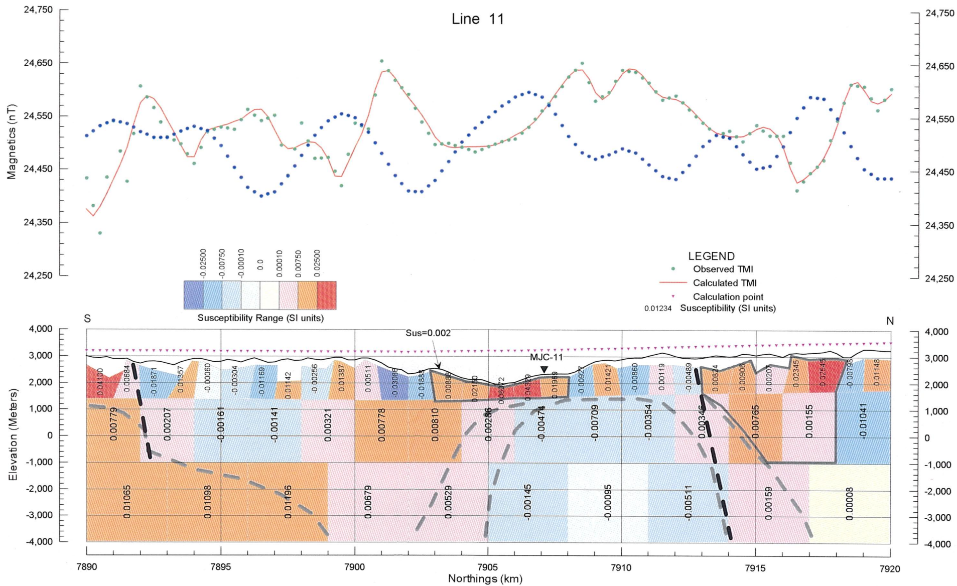
Fig. 2-3-43 Line 11 - 2D Model Profile
