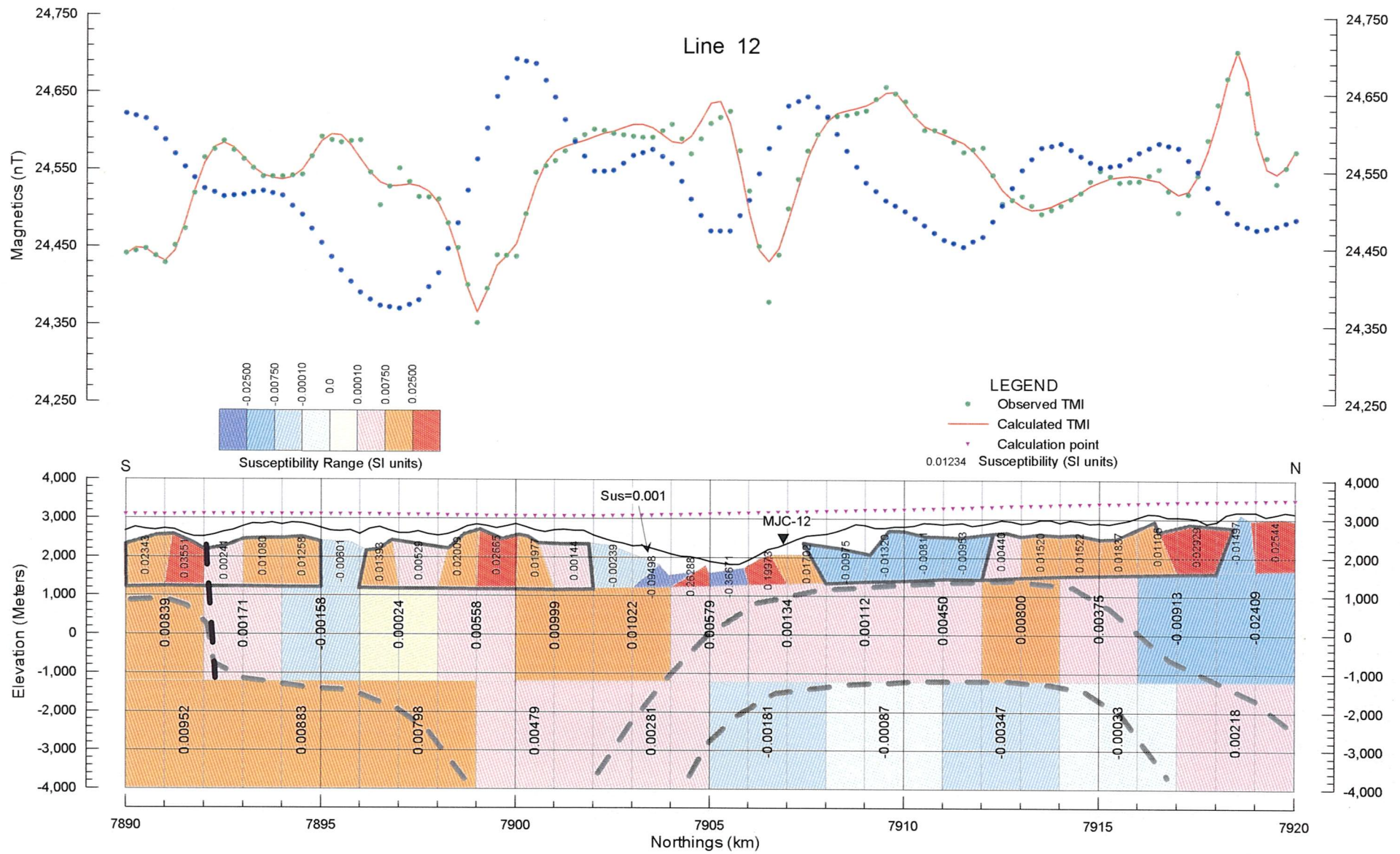
Fig. 2-3-44 Line 12 - 2D Model Profile
