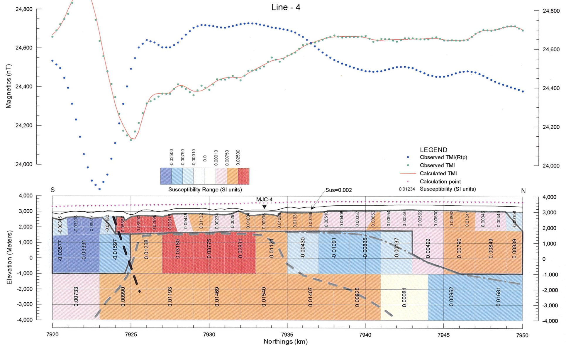
Fig. 2-3-36 Line 4 - 2D Model Profile
