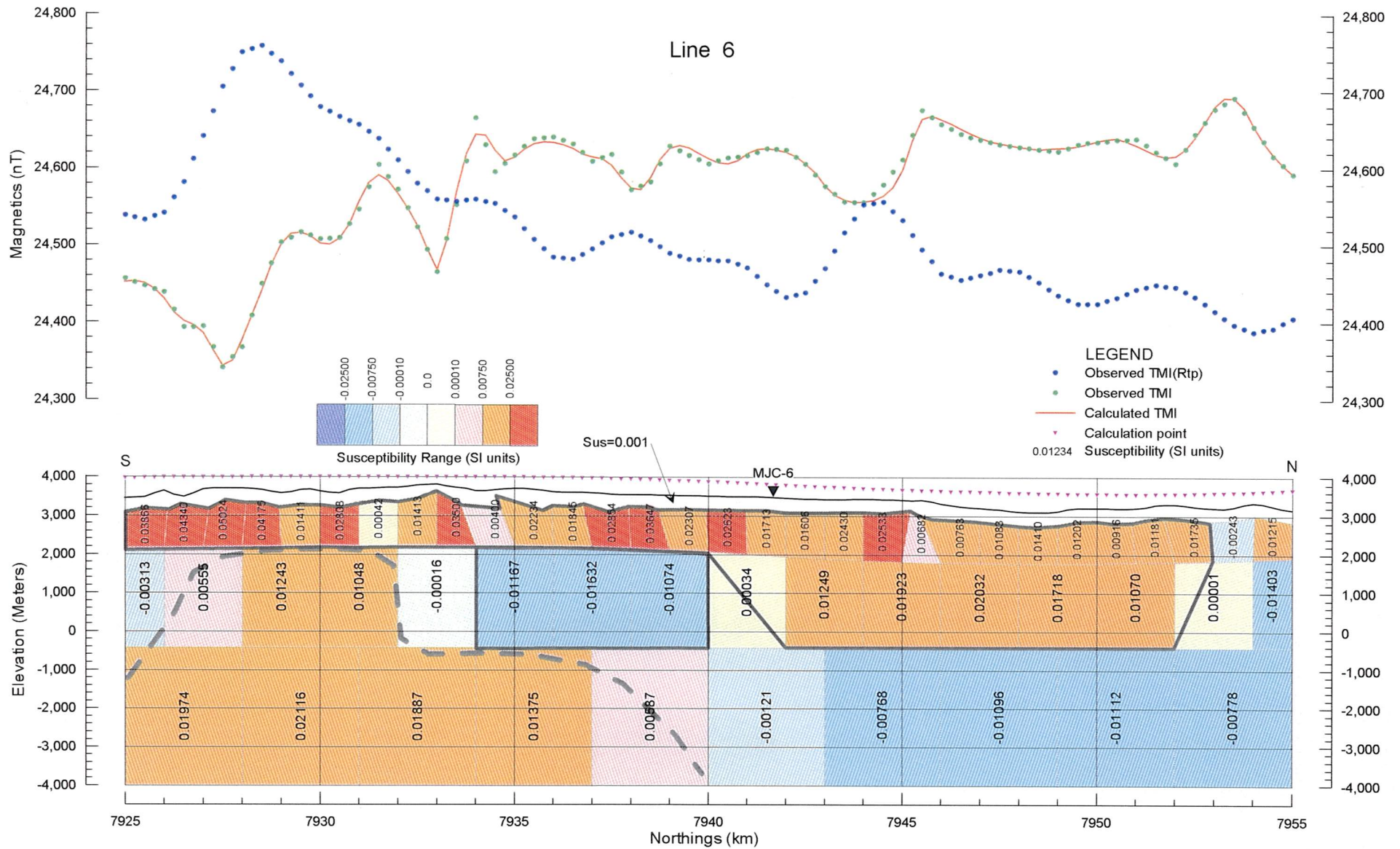
Fig. 2-3-38 Line 6 - 2D Model Profile
