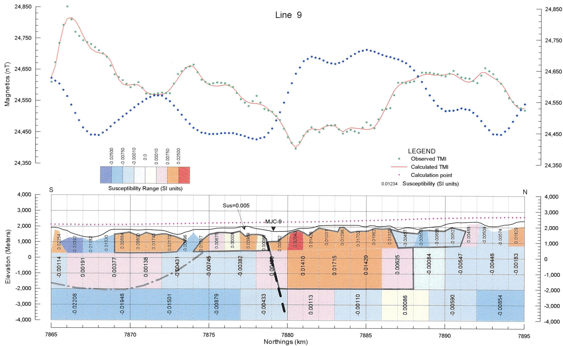
Fig. 2-3-41 Line 9 - 2D Model Profile
