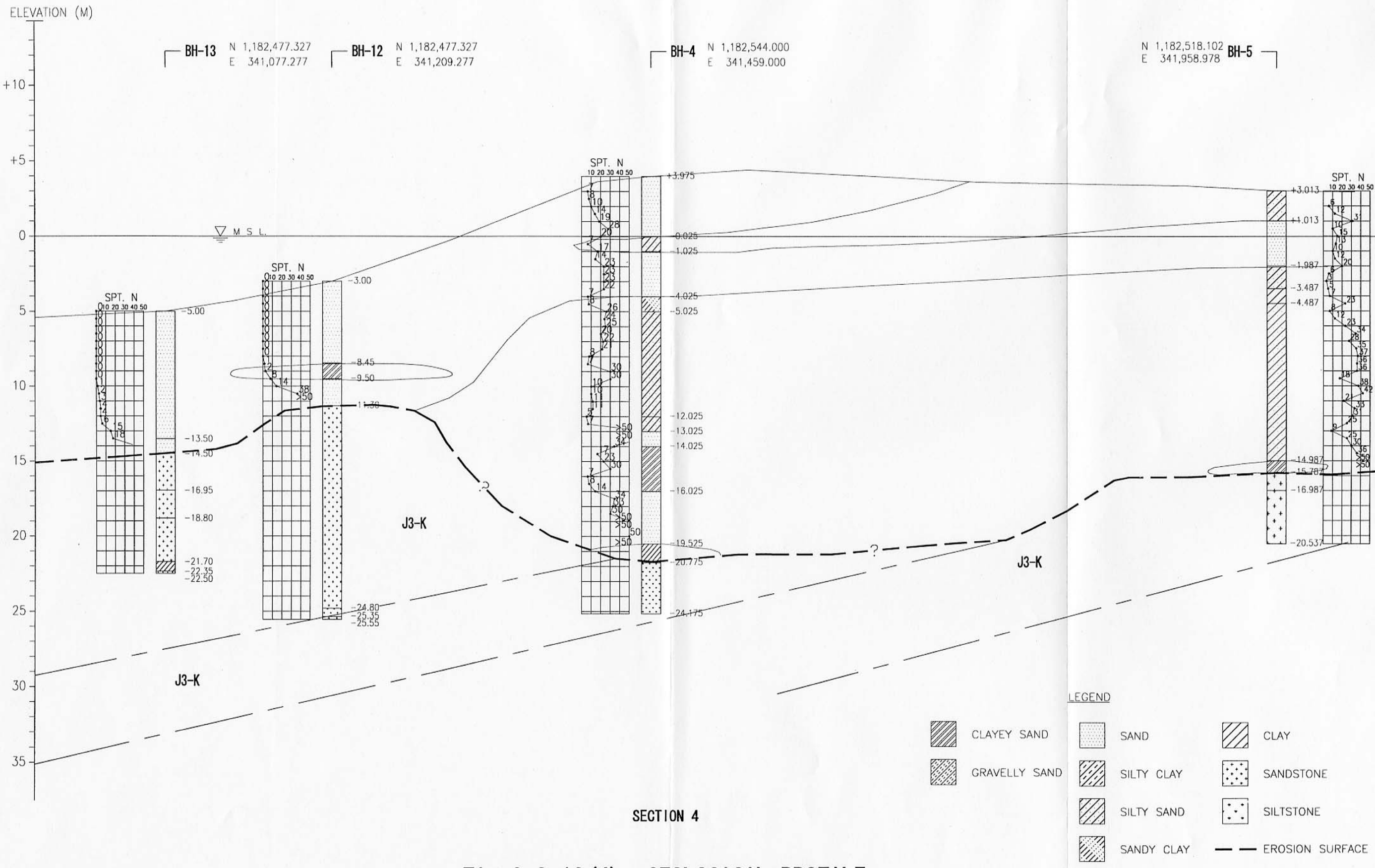
Fig. 2. 2-12(4) GEOLOGICAL PROFILE
