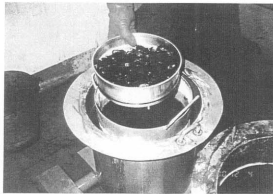
Ph-10 Upgrading Test by Drying Method
