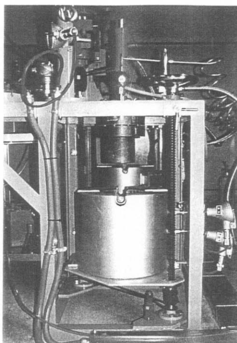
Ph-12 Upgrading Test by Low-Temperature Liquid Phase Cracking Process
