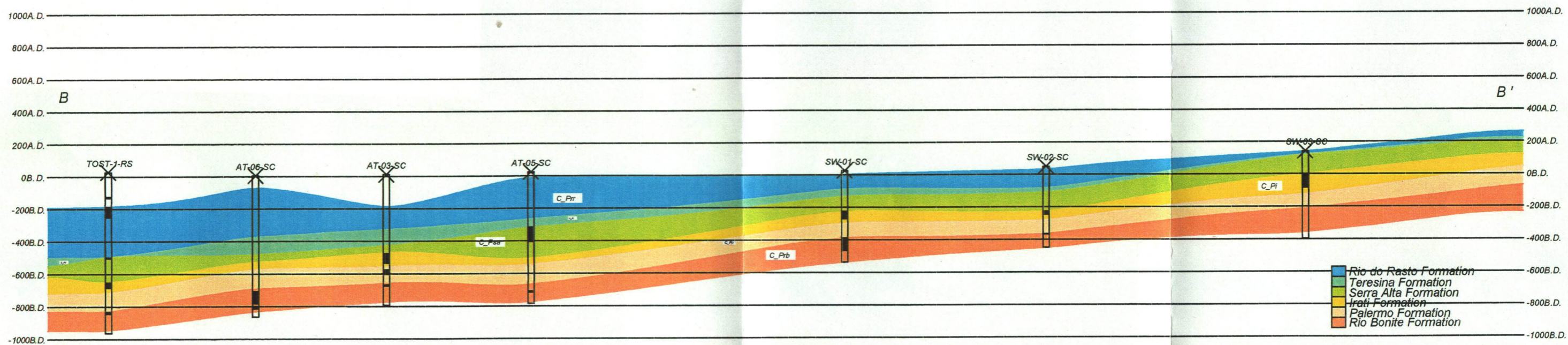
Fig. II-3-8-12 Southeast block B-B' section (scale; 1:250,000, H/V; 1:10)
