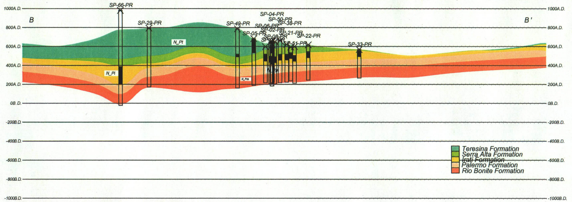
Fig. II-3-8-19 North block B-B' section (scale; 1:150,000, H/V; 1:6)
