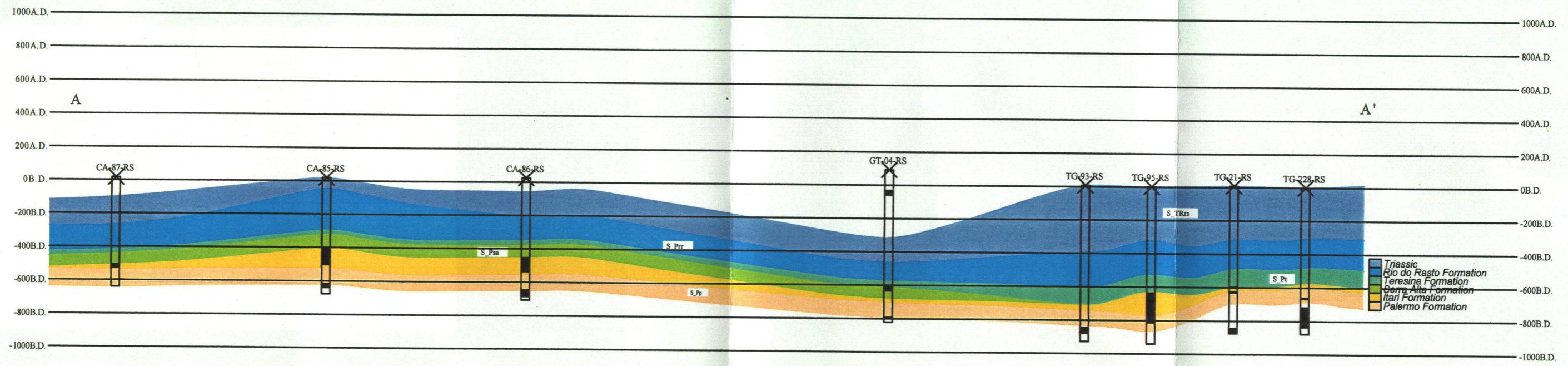
Fig. II-3-8-15 South Block A-A' Section (Scale; 1:250,000, H/V:1:10)
