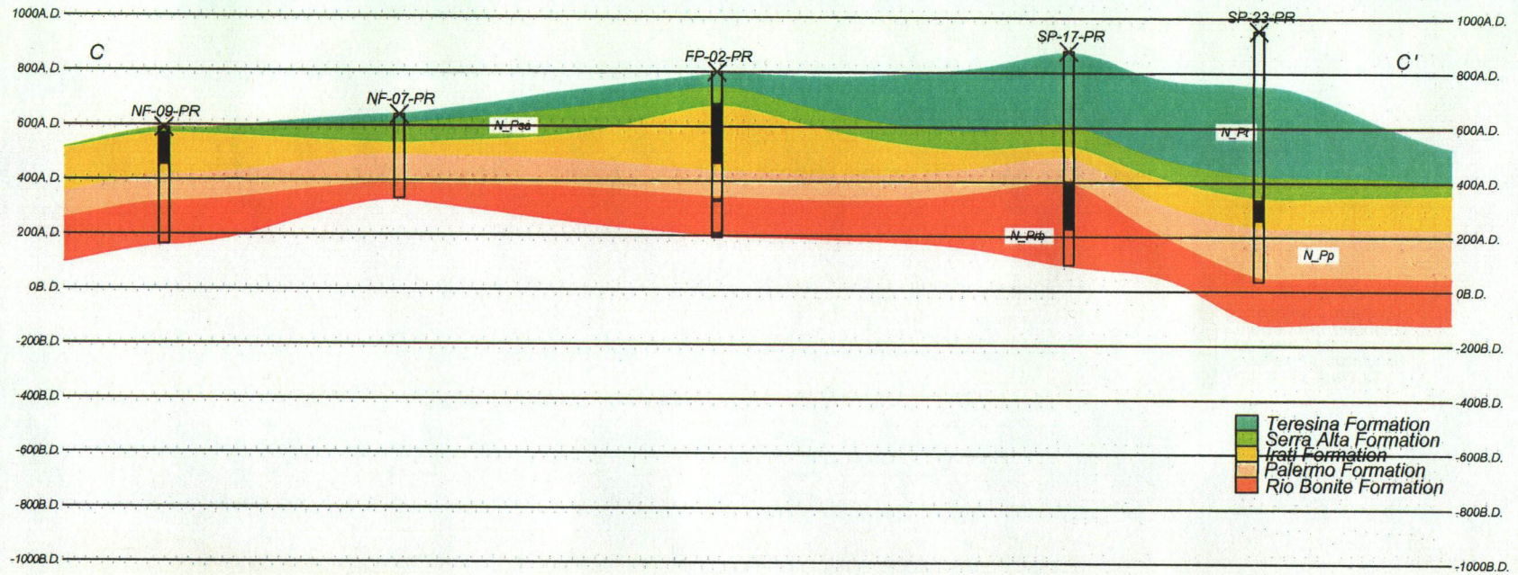
Fig. II-3-8-20 North block C-C' section (scale; 1:150,000, H/V; 1:6)
