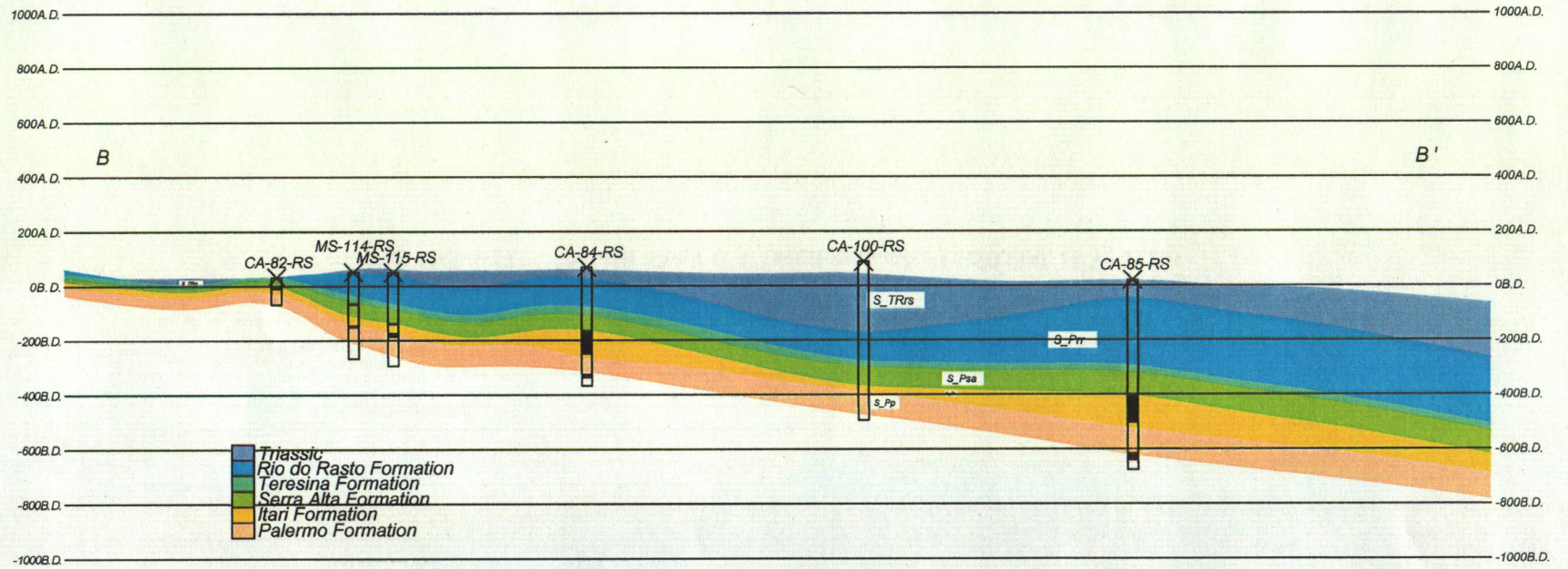
Fig. II-3-8-16 South block B-B' section (scale; 1:250,000, H/V; 1:10)
