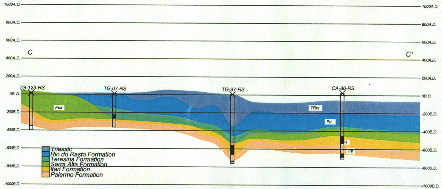
Fig. II-3-8-17 South block C-C' section (scale; 1:250,000, H/V; 1:10)
