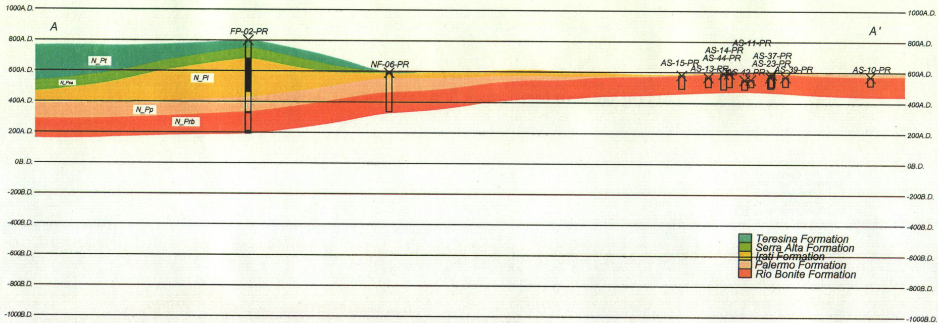
Fig. II-3-8-18 North block A-A' section (scale; 1:150,000, H/V; 1:6)
