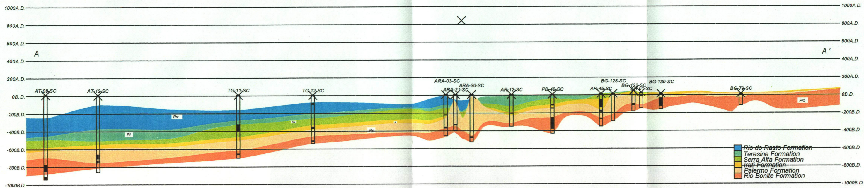
Fig. II-3-8-11 Southeast block A-A' section (scale; 1:250,000, H/V; 1:10)
