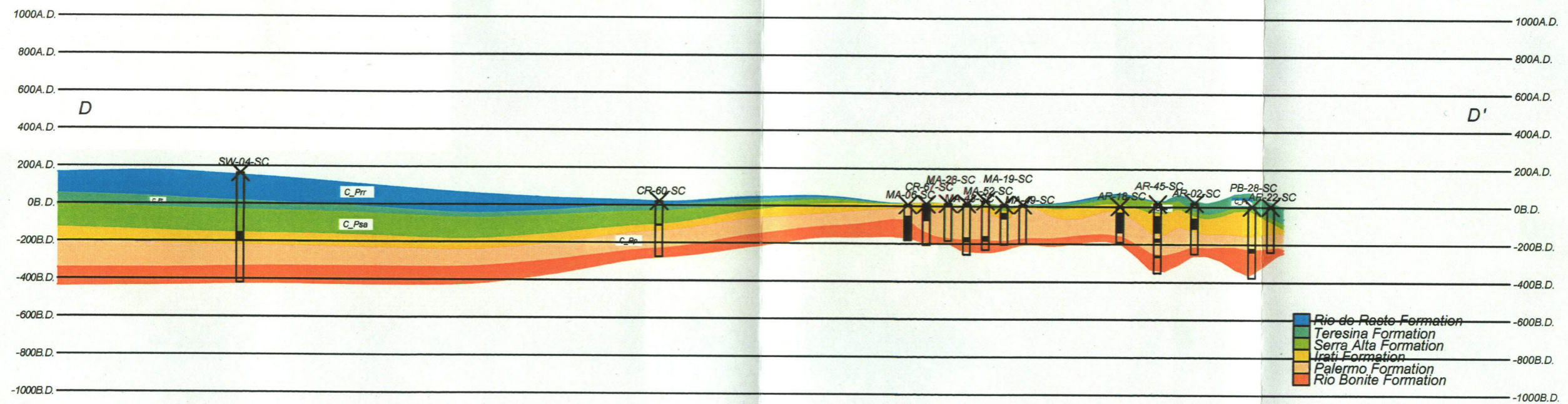
Fig. II-3-8-14 Southeast Block D-D' Section (Scale; 1:250,000, H/V;1:10)
