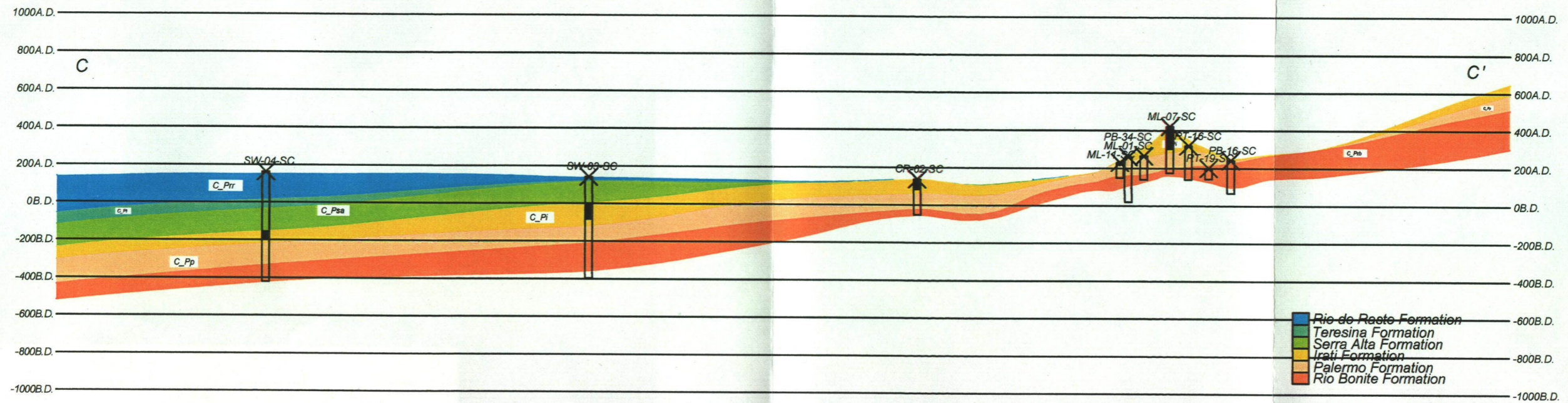
Fig. II-3-8-13 Southeast Block C-C' Section (Scale; 1:250,000, H/V;1:10)
