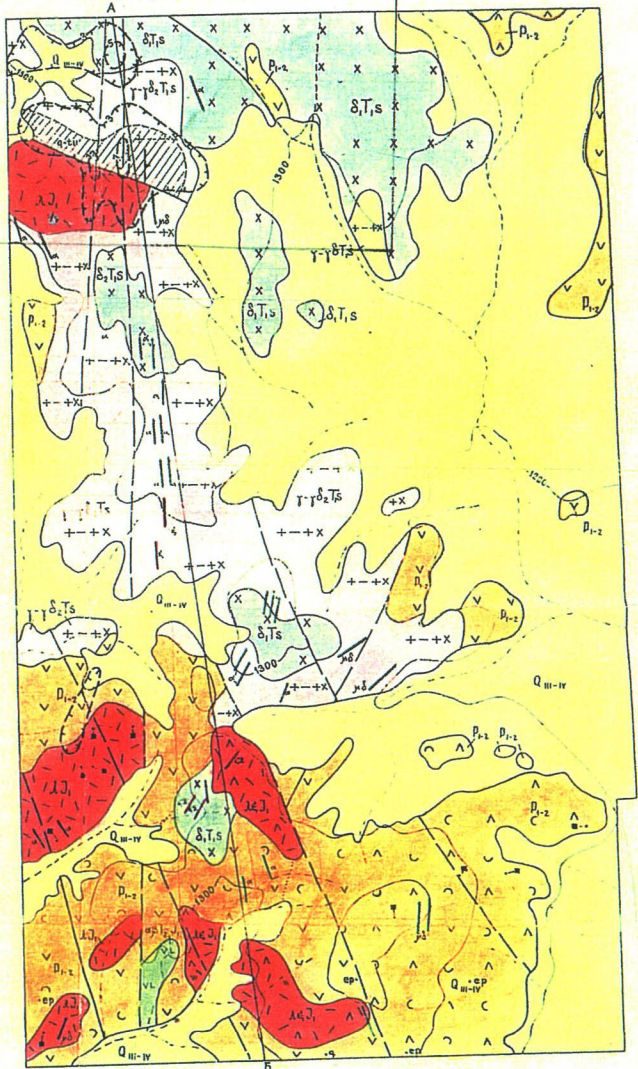
Geological Map
