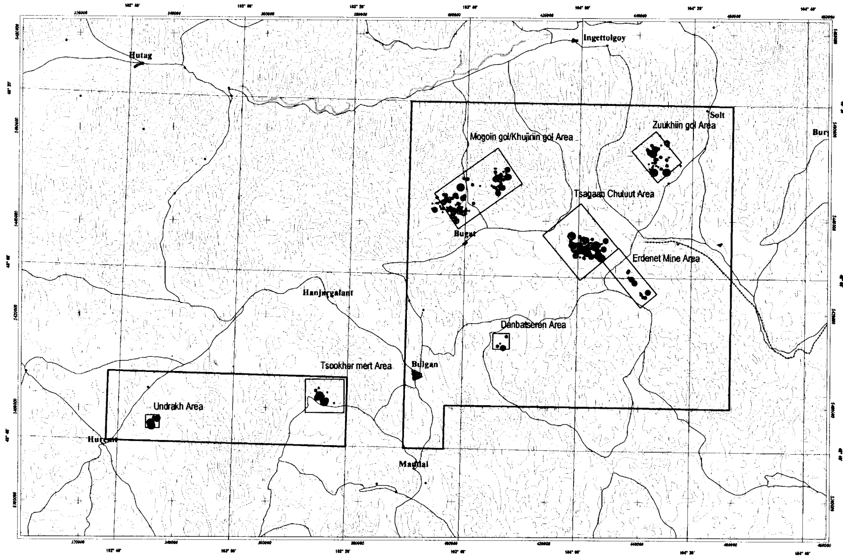
Factor score 4 distribution map
