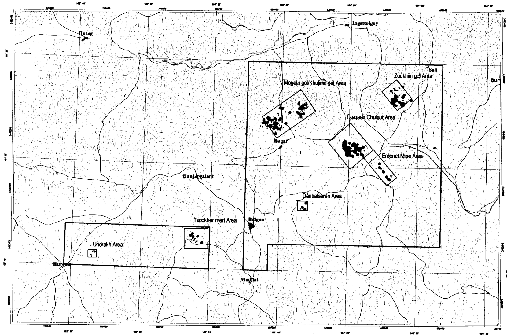
Sr distribution map
