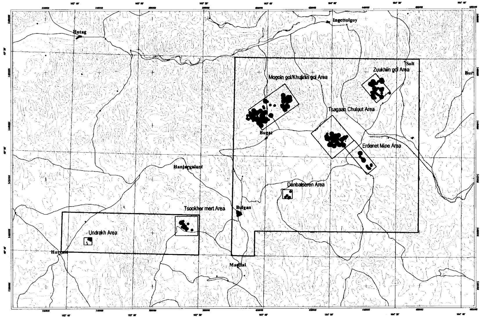
Fe distribution map
