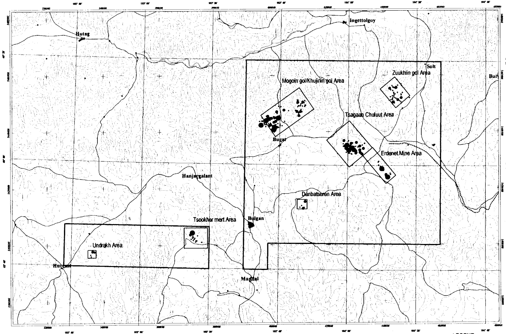
As distribution map
