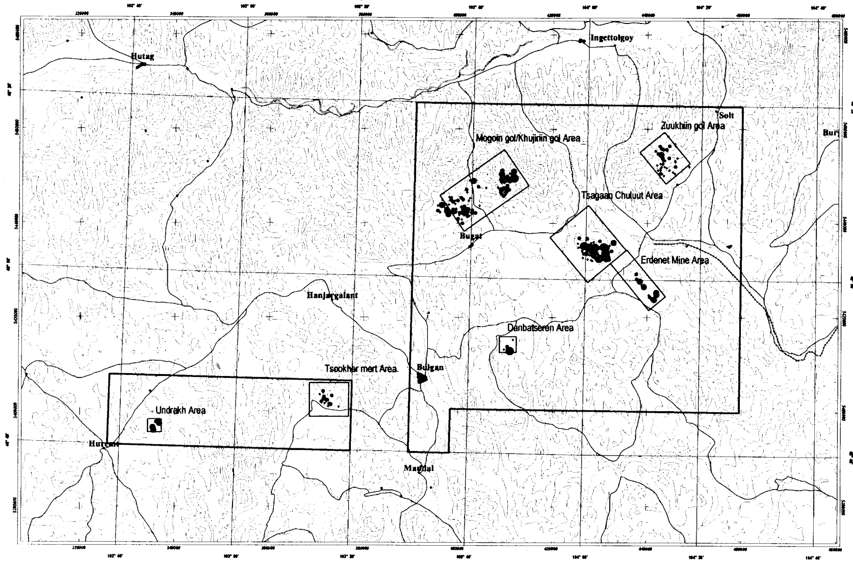
Factor score 3 distribution map
