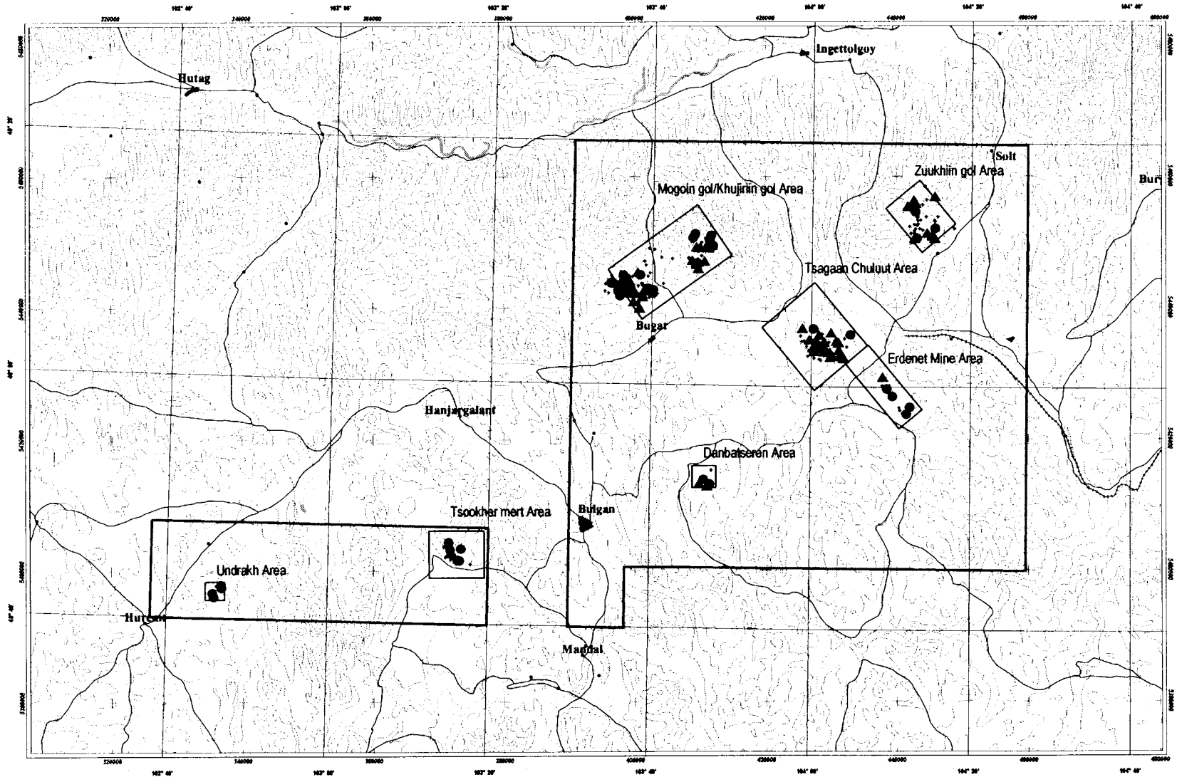
K distribution map
