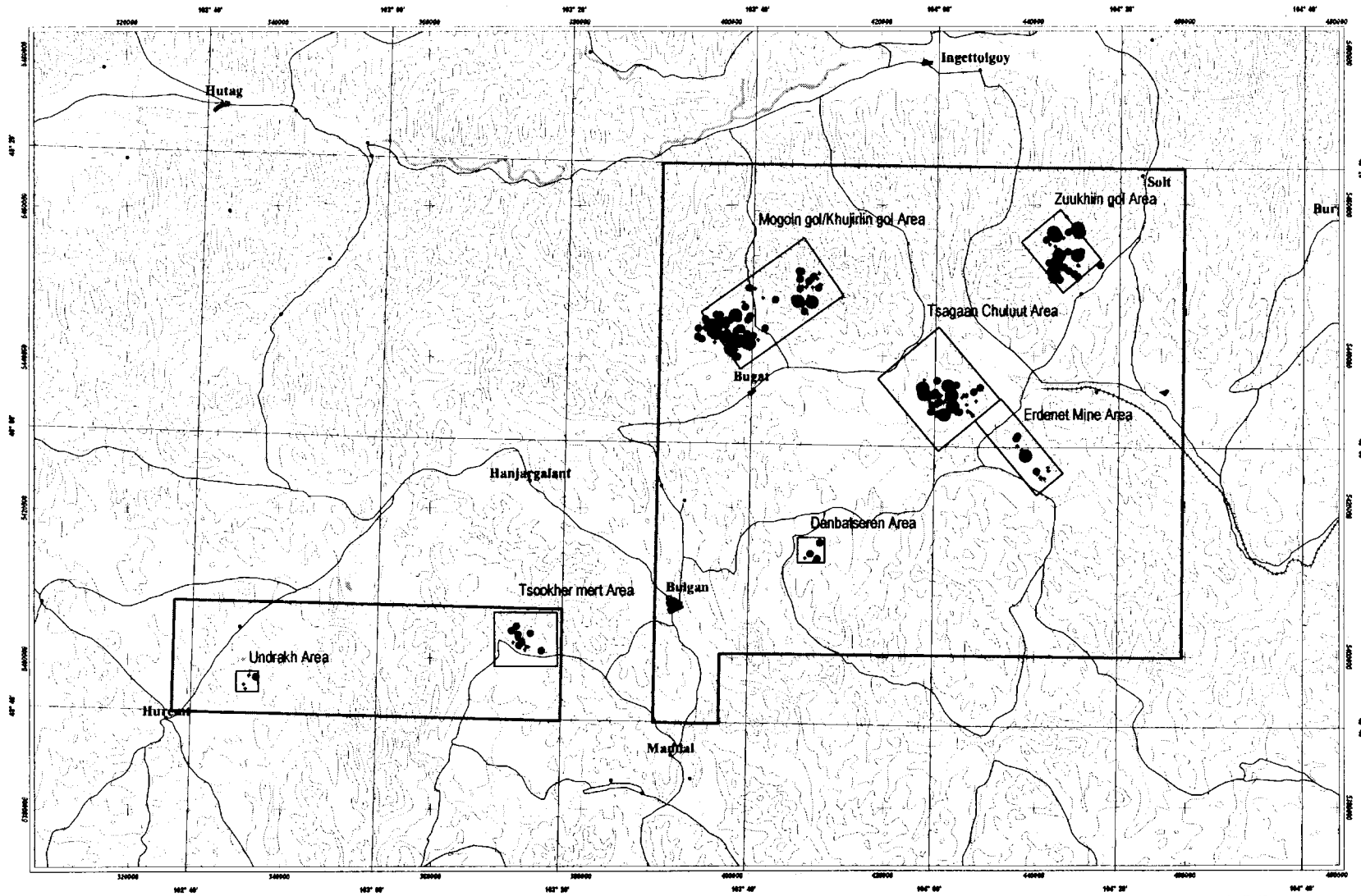
Co distribution map
