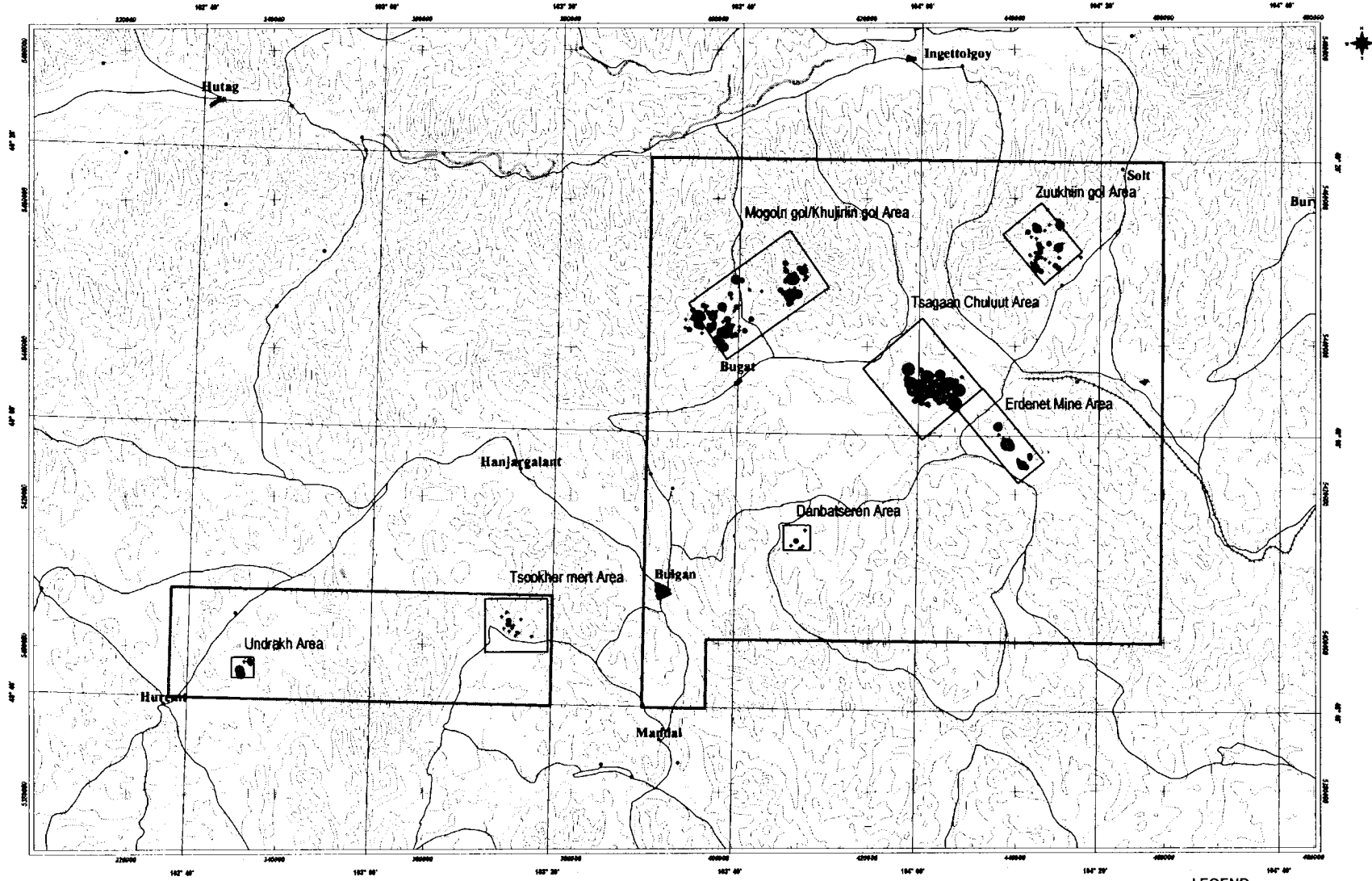
Factor score 1 distribution map
