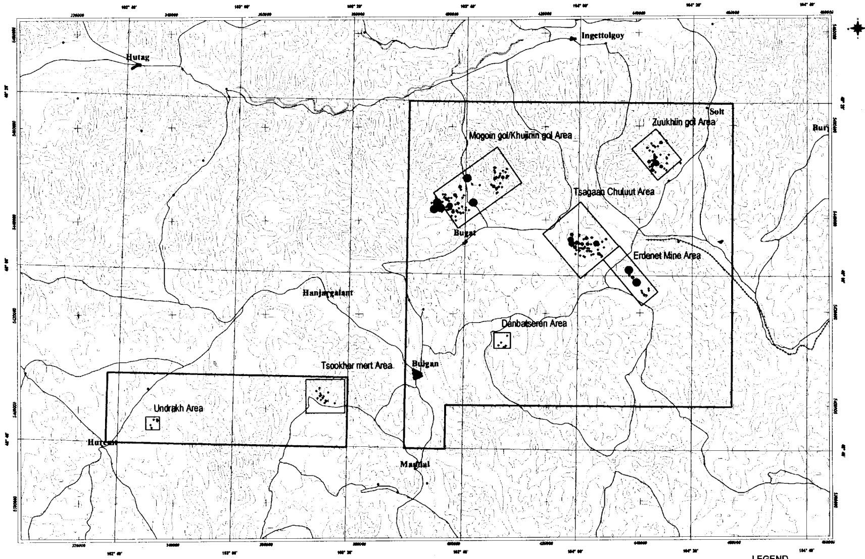
Factor score 5 distribution map
