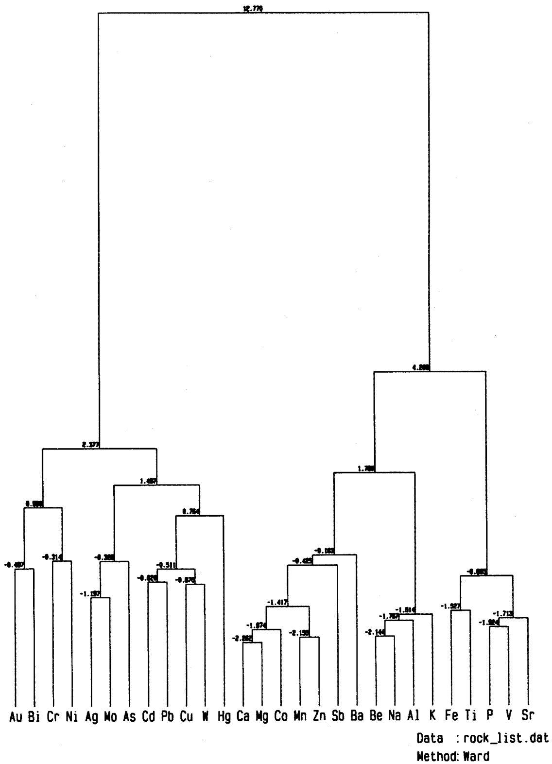
Cluster Dendrogram
