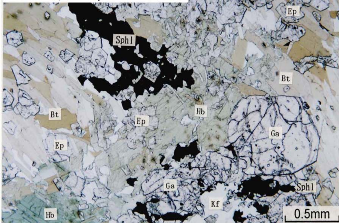
36:M1-35, Ga-Ms-Bt schist
