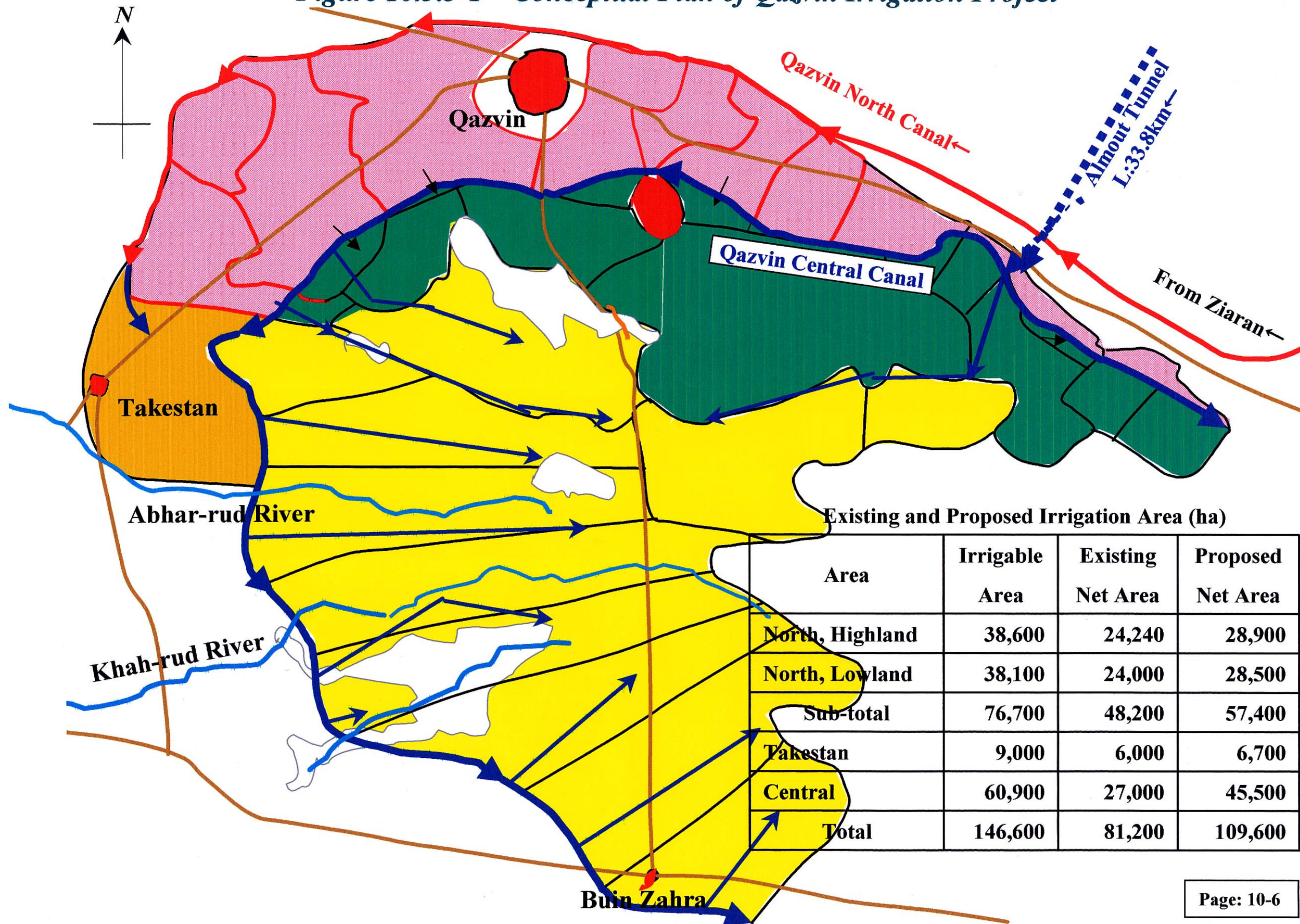
Figure 10.3.3-1 Conceptual Plan of Qazvin Irrigation Project
