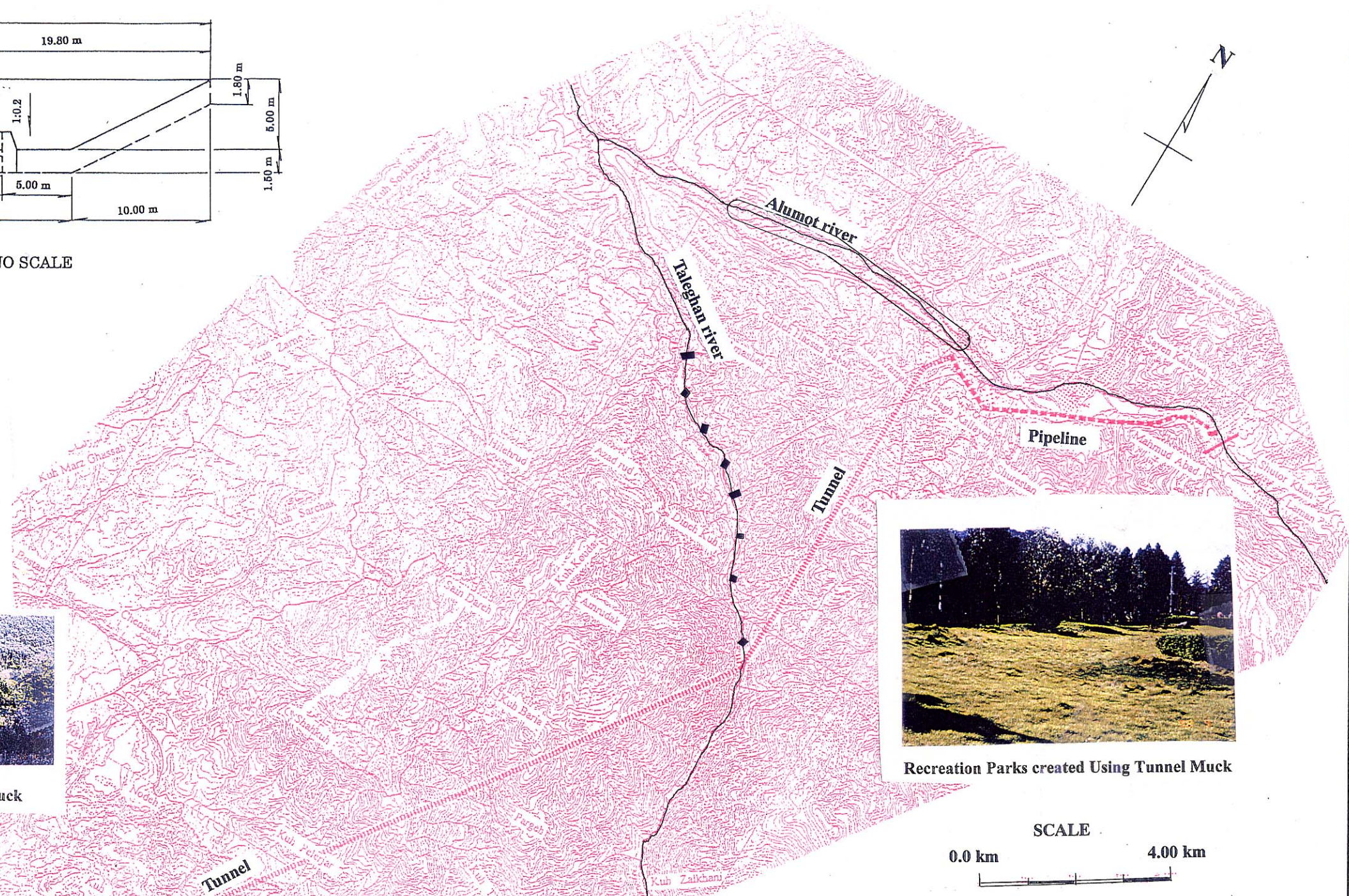
LOCATIN OF TUNNEL MUCK STOCK YARD
