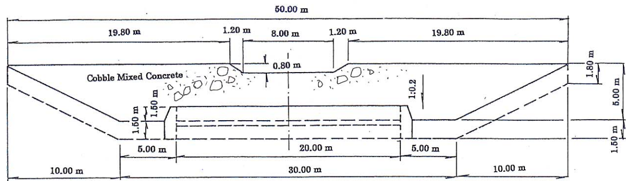
ELEVATION (A-A) NO SCALE
