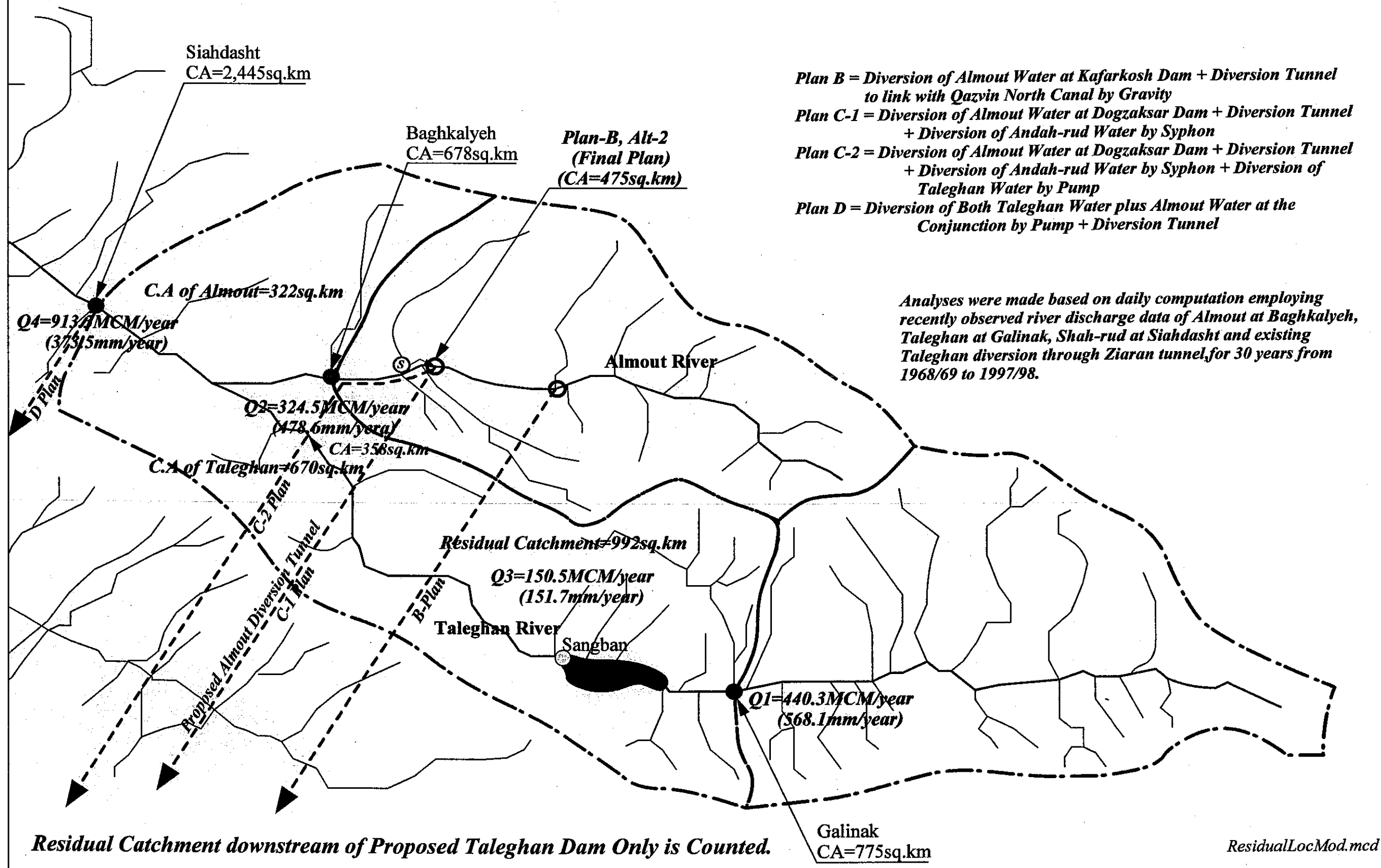
Figure 5.1.5.1 Outline Location of Almout Water Diversion Plan (Final Plan)
