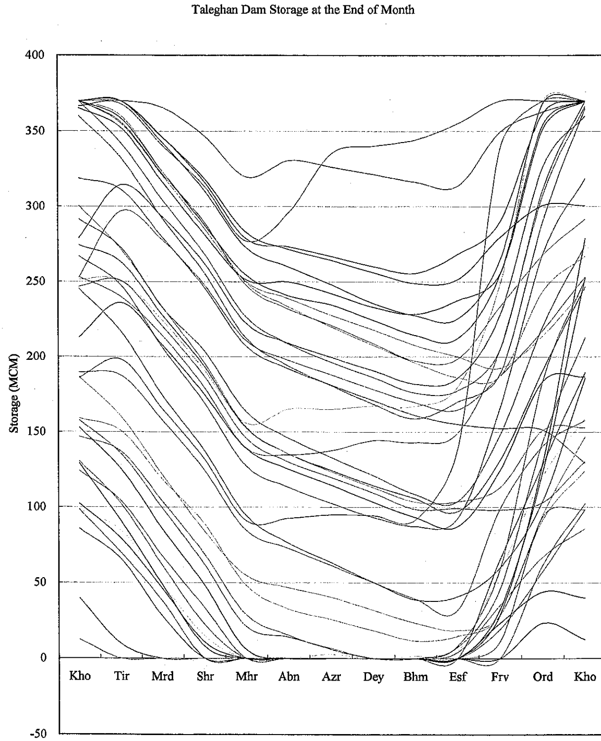
Figure 5.1.4.1 Operation of Taleghan Storage Dam (Future Operation without and with Rule)
