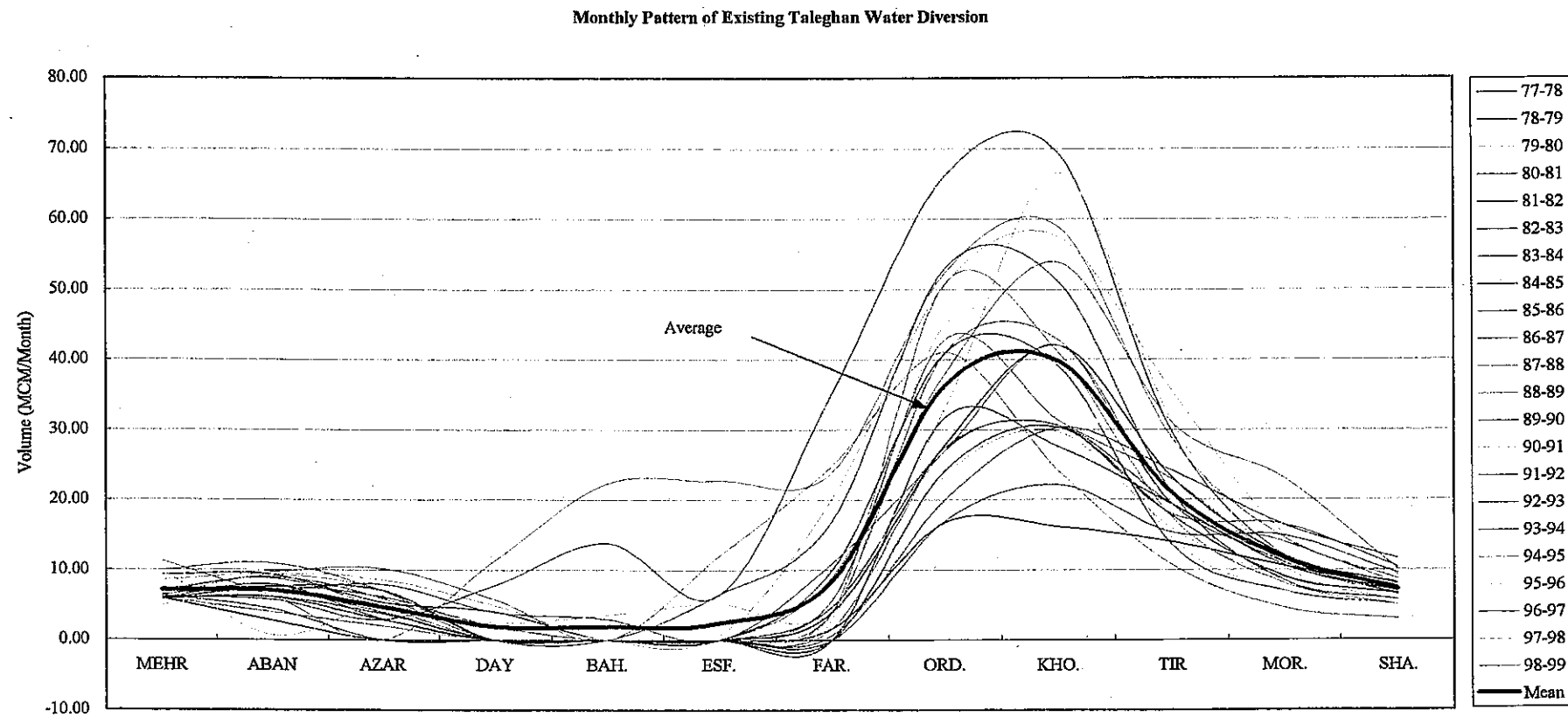
Figure 5.1.3.1 Existing Operation of Taleghan Diversion Dam
