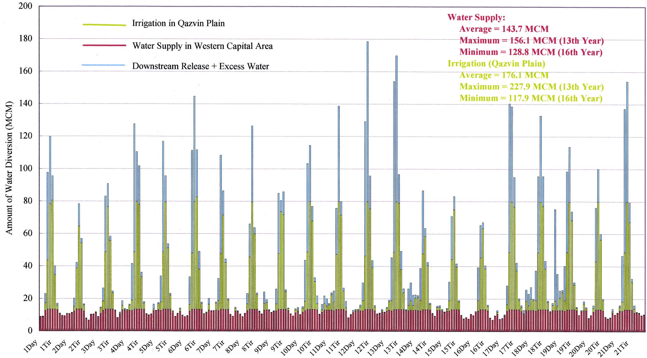
Figure 5.1.3.2 Water Balance at the Existing Sangban Diversion Dam (Priority: Water Supply)
