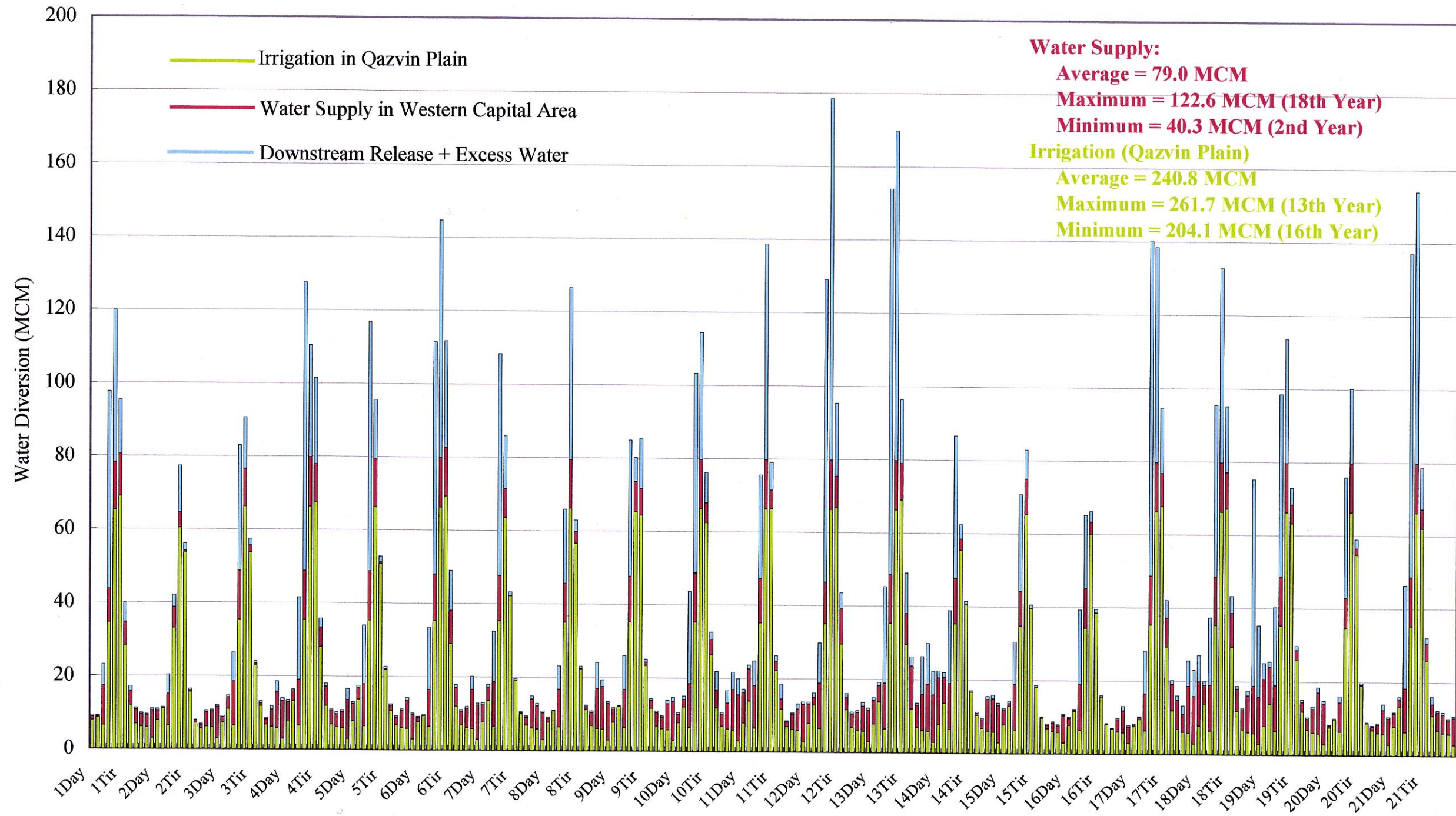
Figure 5.1.3.3 Water Balance at the Existing Sangban Diversion Dam (Priority : Irrigation)
