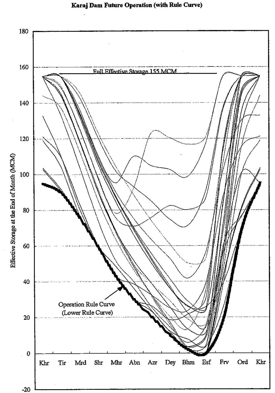
Figure 5.1.1 Karaj Dam Operation (Past Operation, Future Operation without Rule and Future Operation with Rule)
