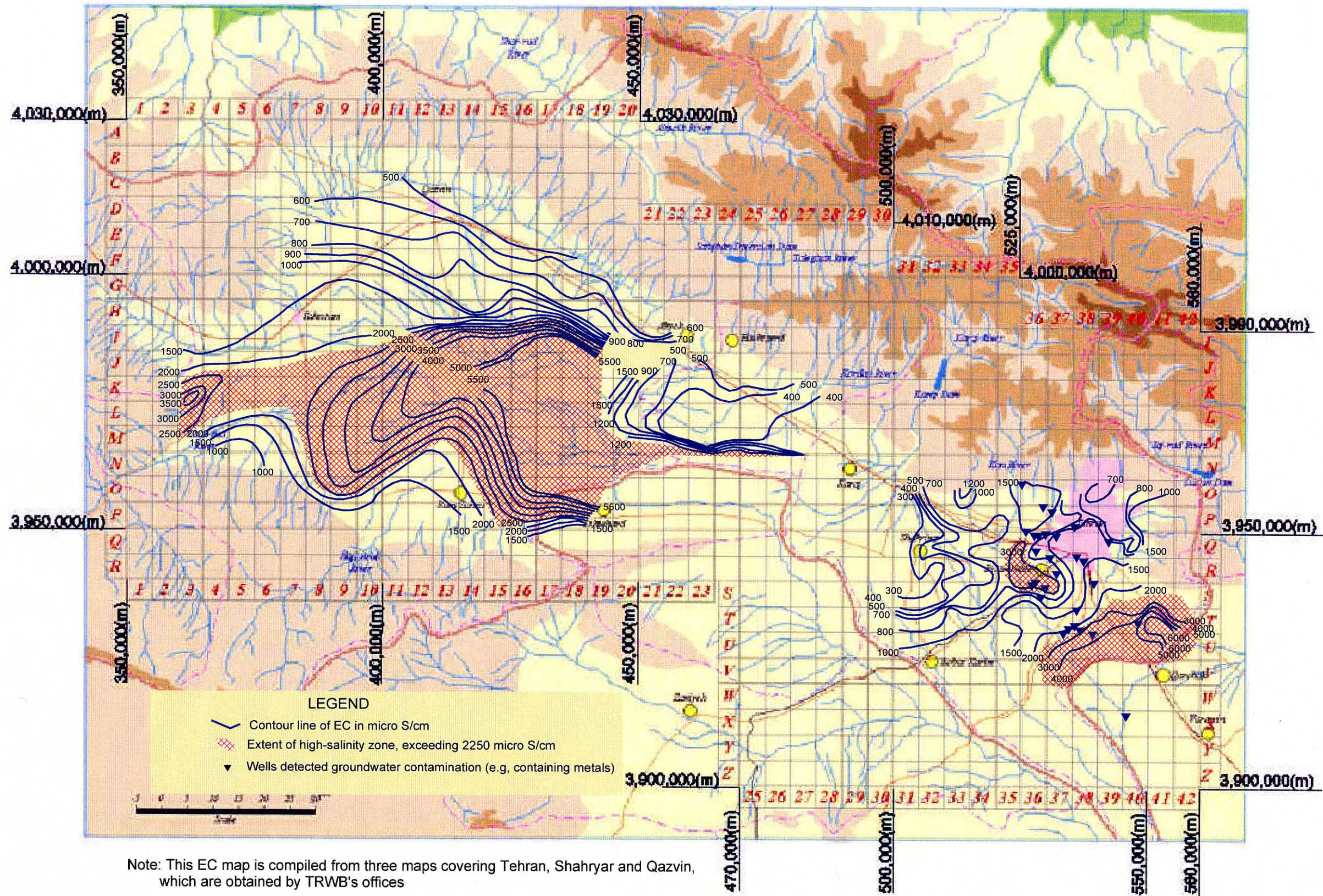
Figure 3.4.6.1 Contour Map of Electric Conductivity (EC) Observed in 1995
