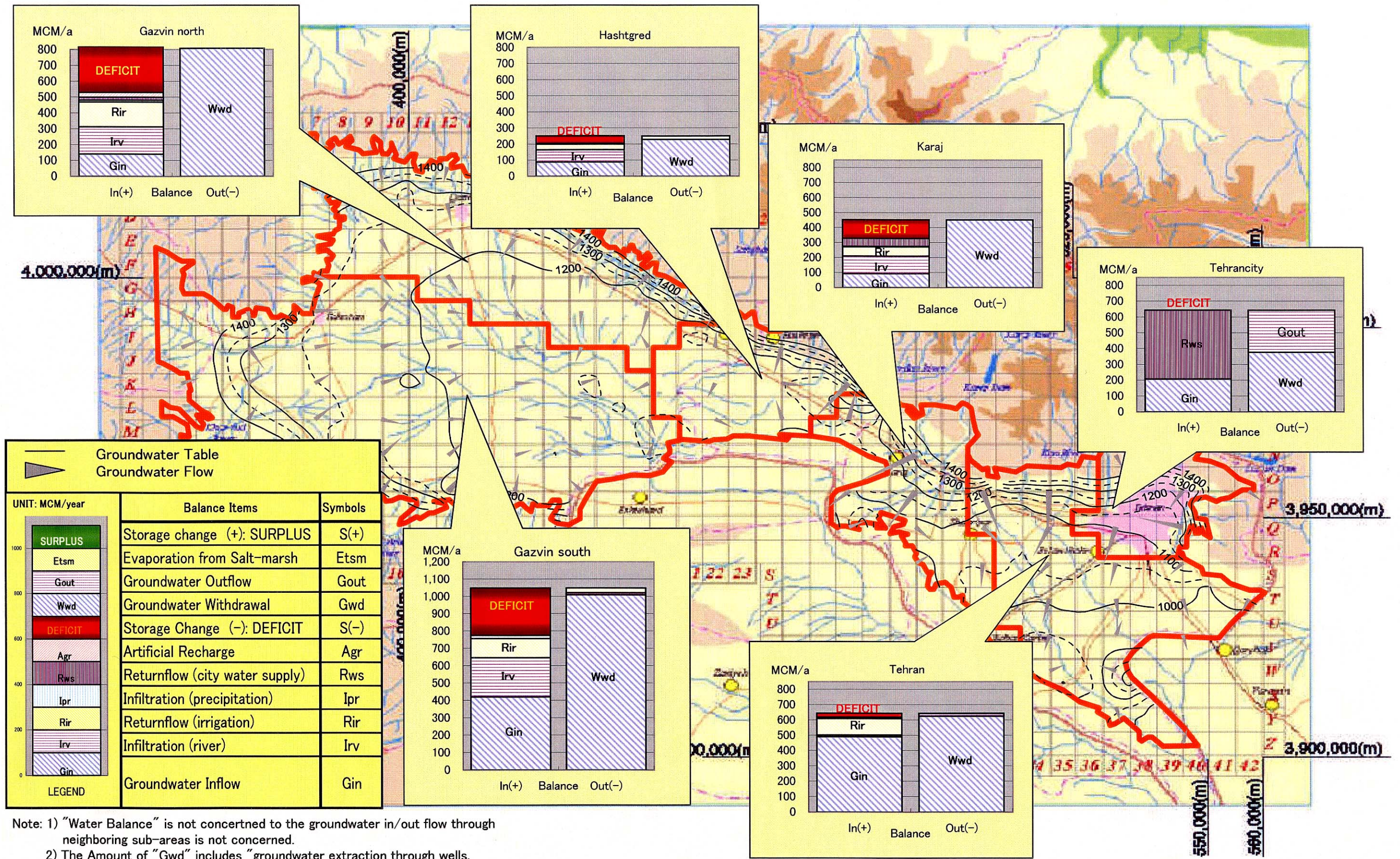
Figure 3.4.5.4 Groundwater Balance (1999/2000 Current Condition)
