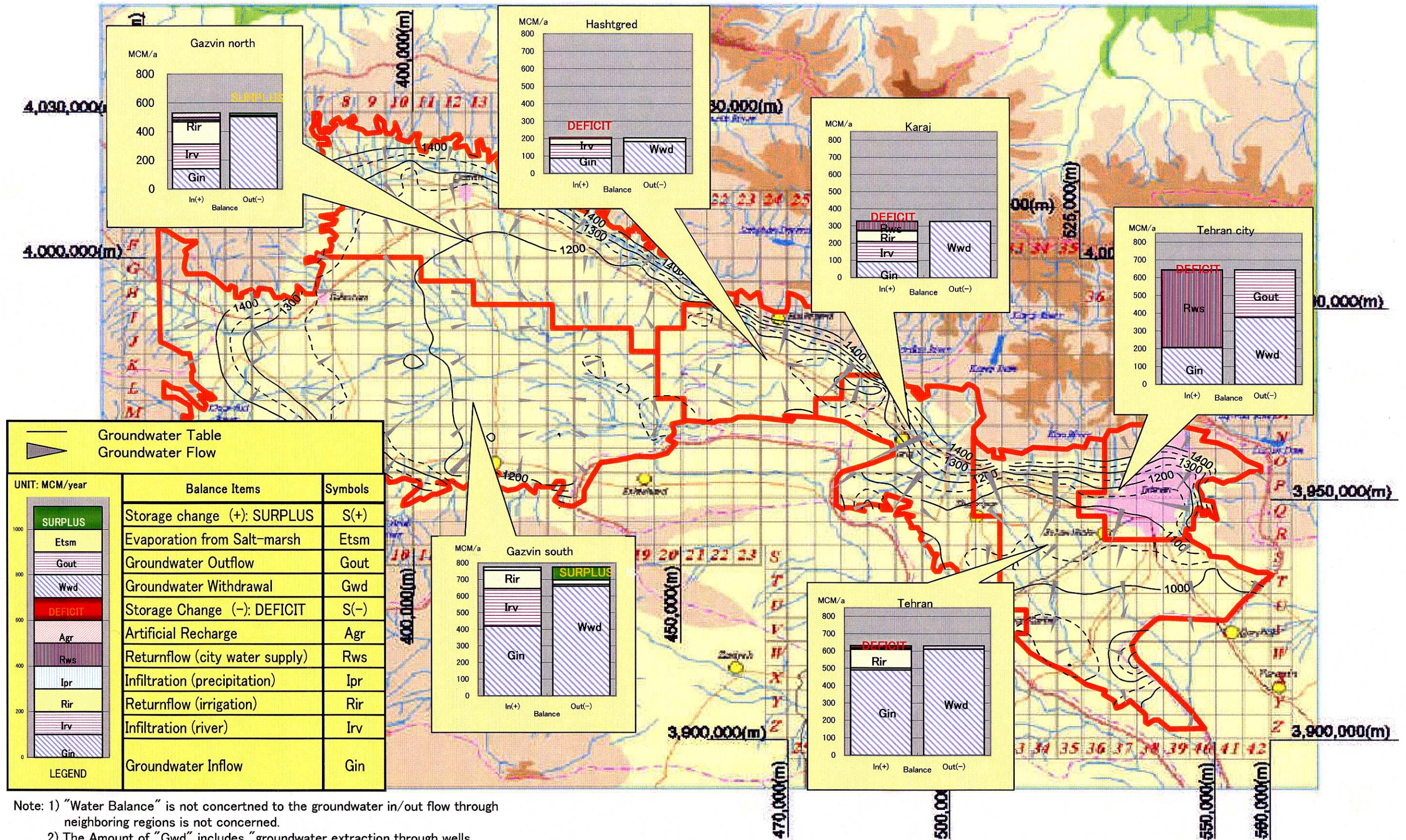
Figure 3.4.5.3 Groundwater Balance (1996/1997 Current Condition)
