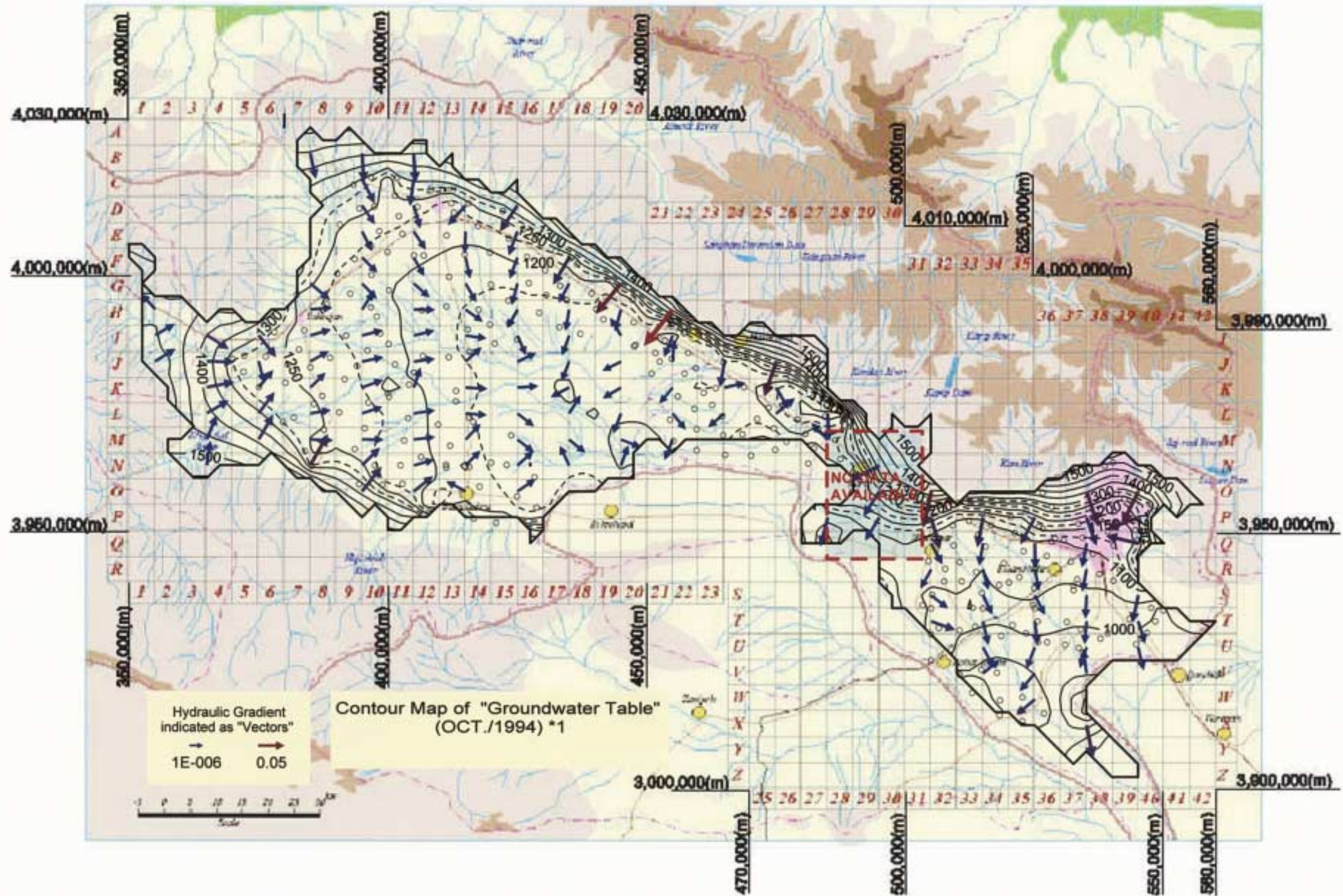
Figure 3.4.1.6 Contour of Groundwater Level (October 1994)
