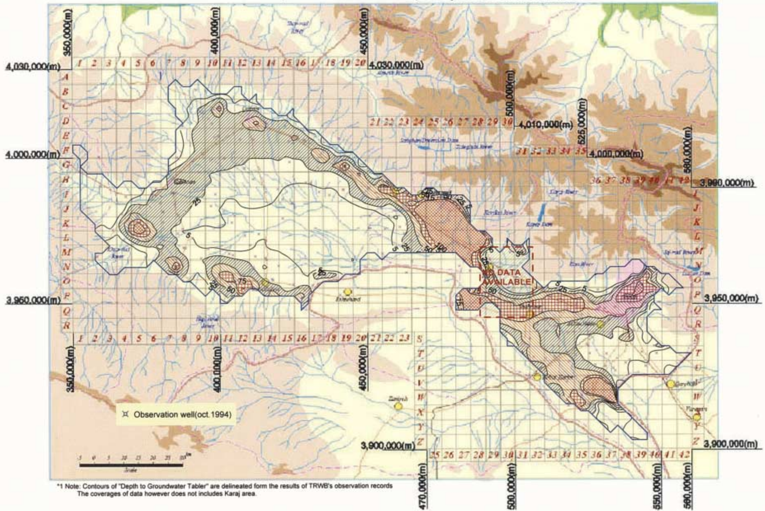
Figure 3.4.1.7 Contour Map of Depth to Groundwater Table
