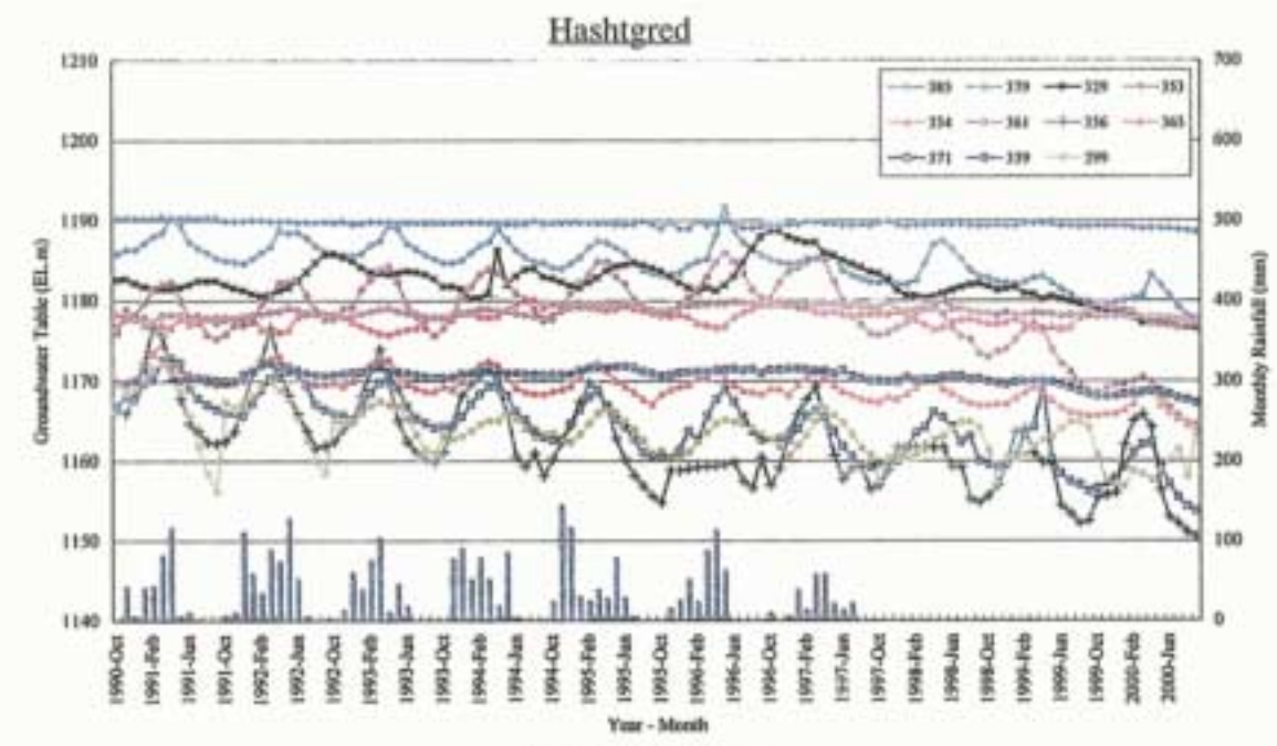
Figure 3.4.1.8 Groundwater Table in TRWB's Observation Wells(Selected wells, Oct.1990 – Sep.2000)
