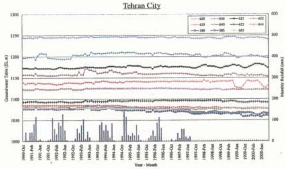
Figure 3.4.1.8 Groundwater Table in TRWB's Observation Wells(Selected wells, Oct.1990 – Sep.2000)
