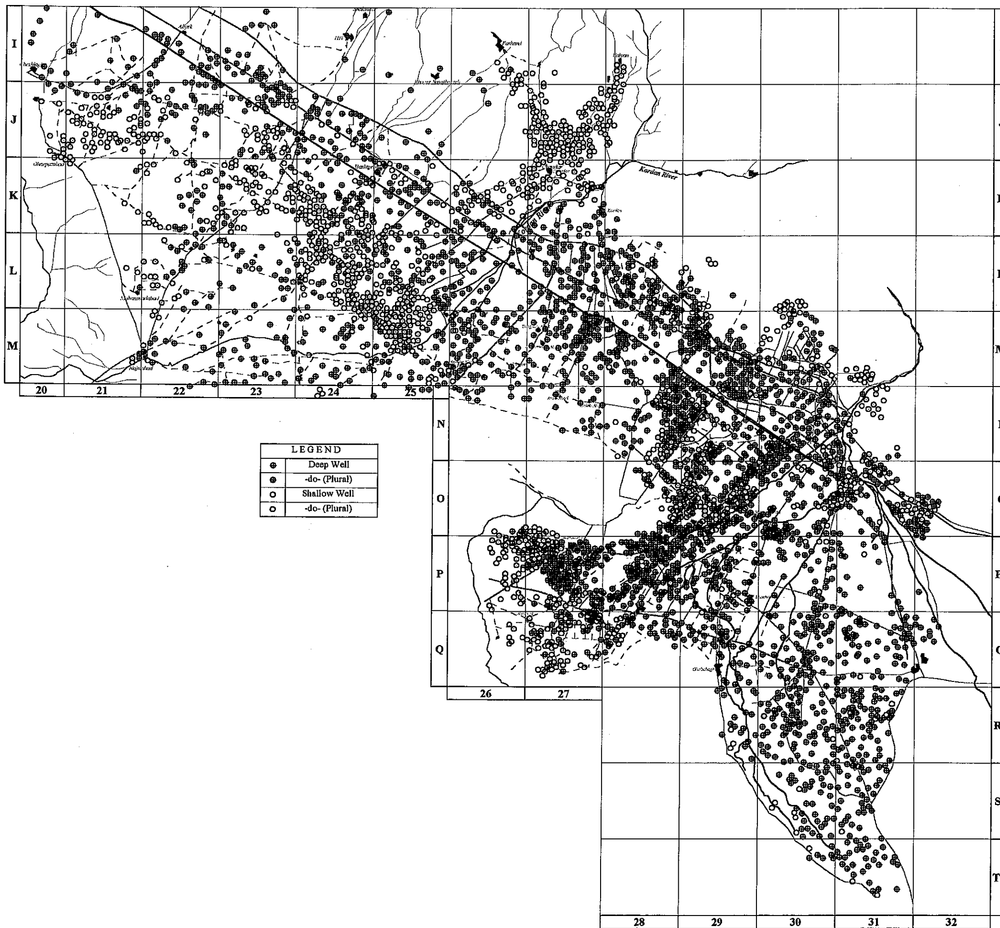
Figure 3.4.3.3 Distribution of Existing Production Wells at Karaj and Hashtgerd
