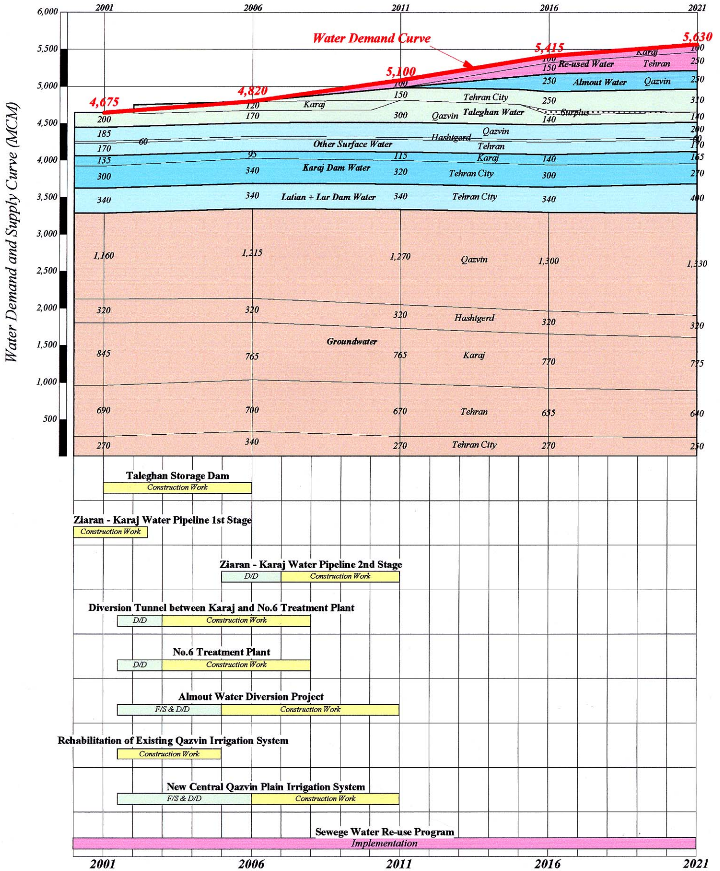
Figure 31 Implementation Schedule of Water Resources Development Sub-Projects
