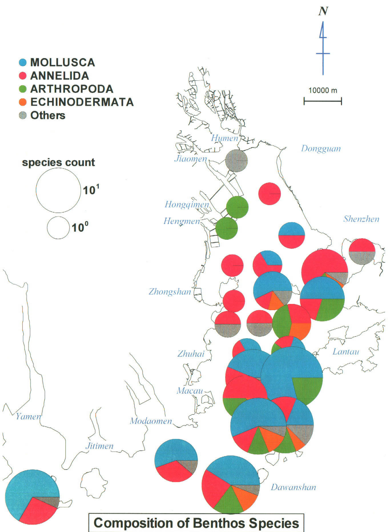
Figure 3.4.6(2) Result of the Survey on Benthos (Rainy Season) July 31 - August 10, 2000
