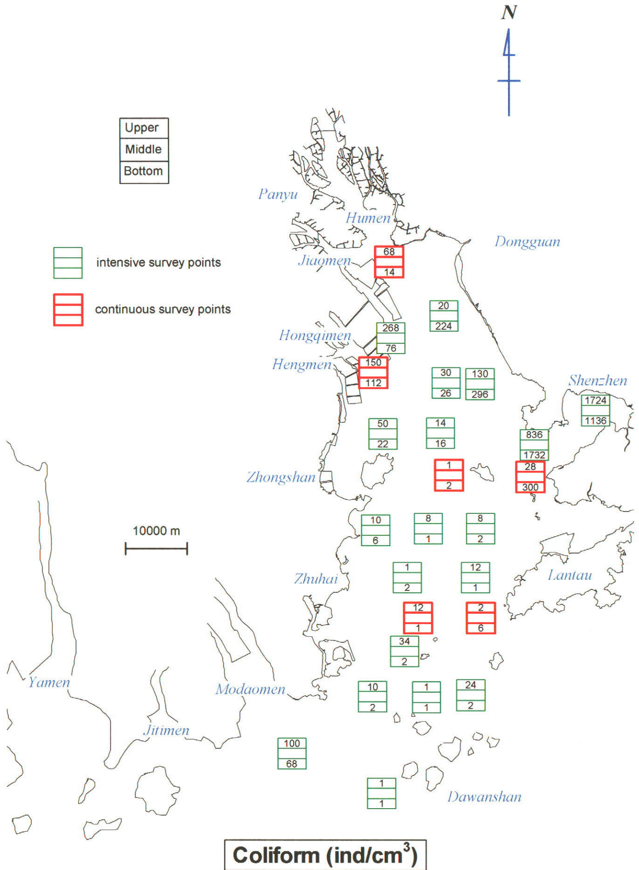
Figure 3.4.11 Distribution of Coliforms (Dry Season)
