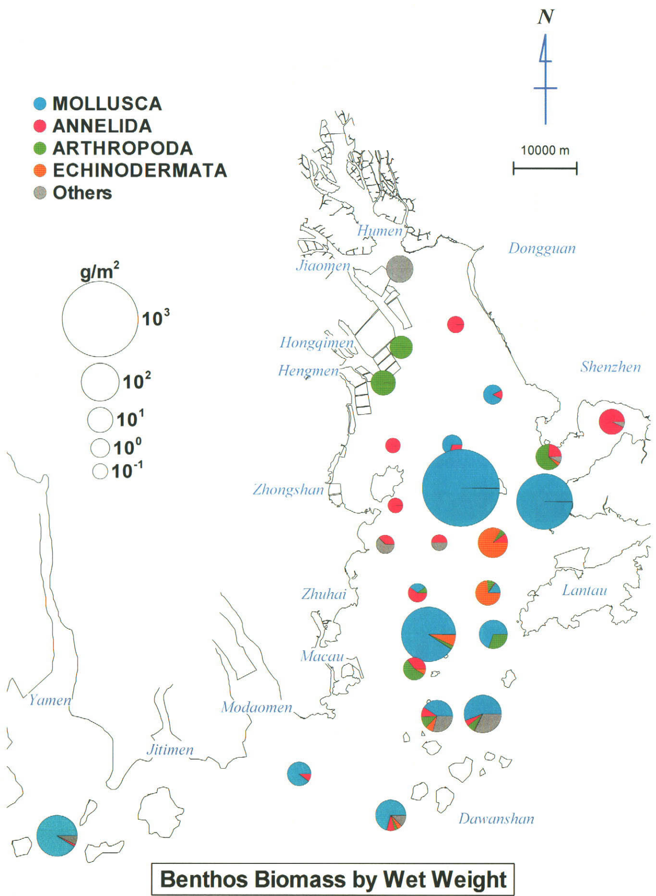
Figure 3.4.8 Result of the Survey on Benthos Biomass by Wet Weight (Rainy Season)
