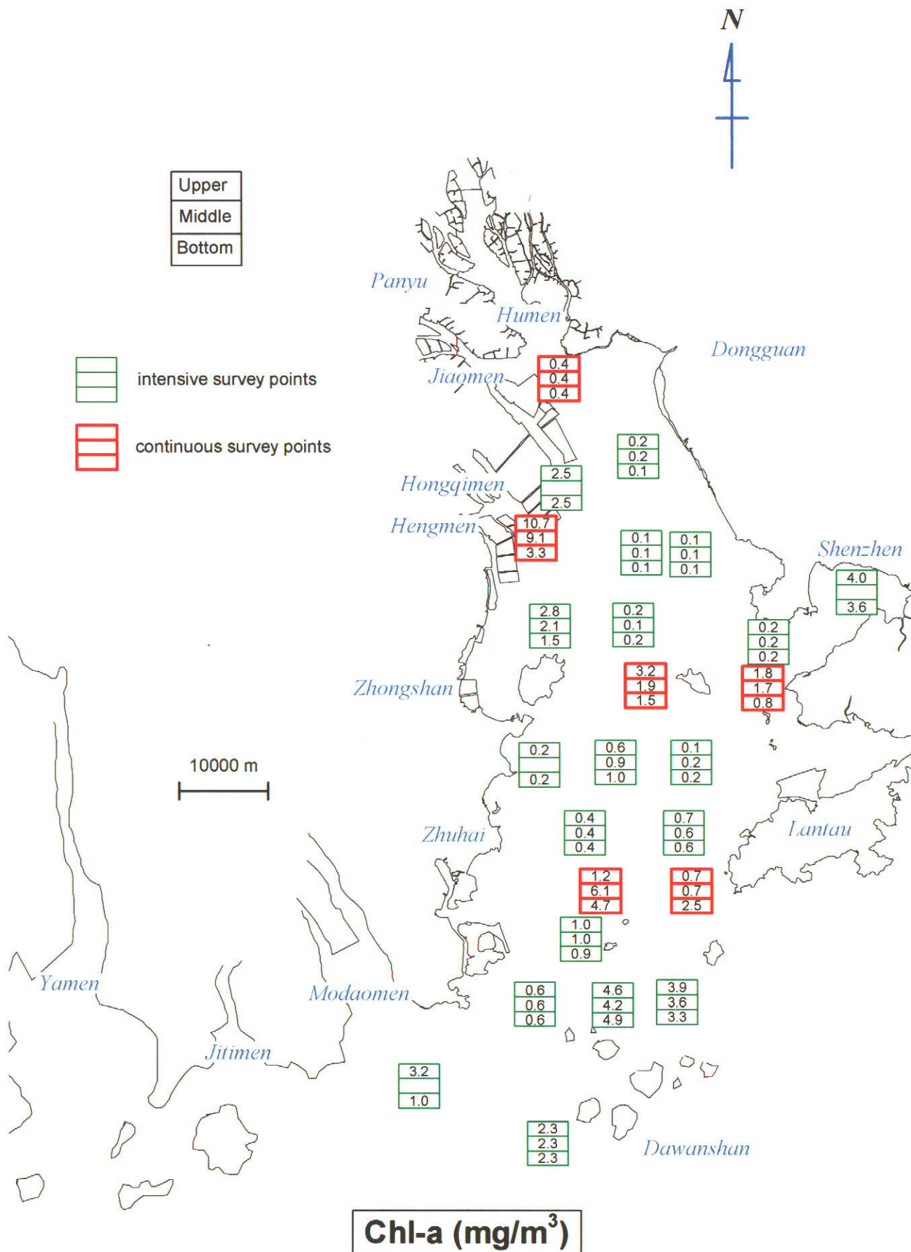
Figure 3.4.10(2) Distribution of Chlorophyll-a (Neap Tide, Dry Season)
