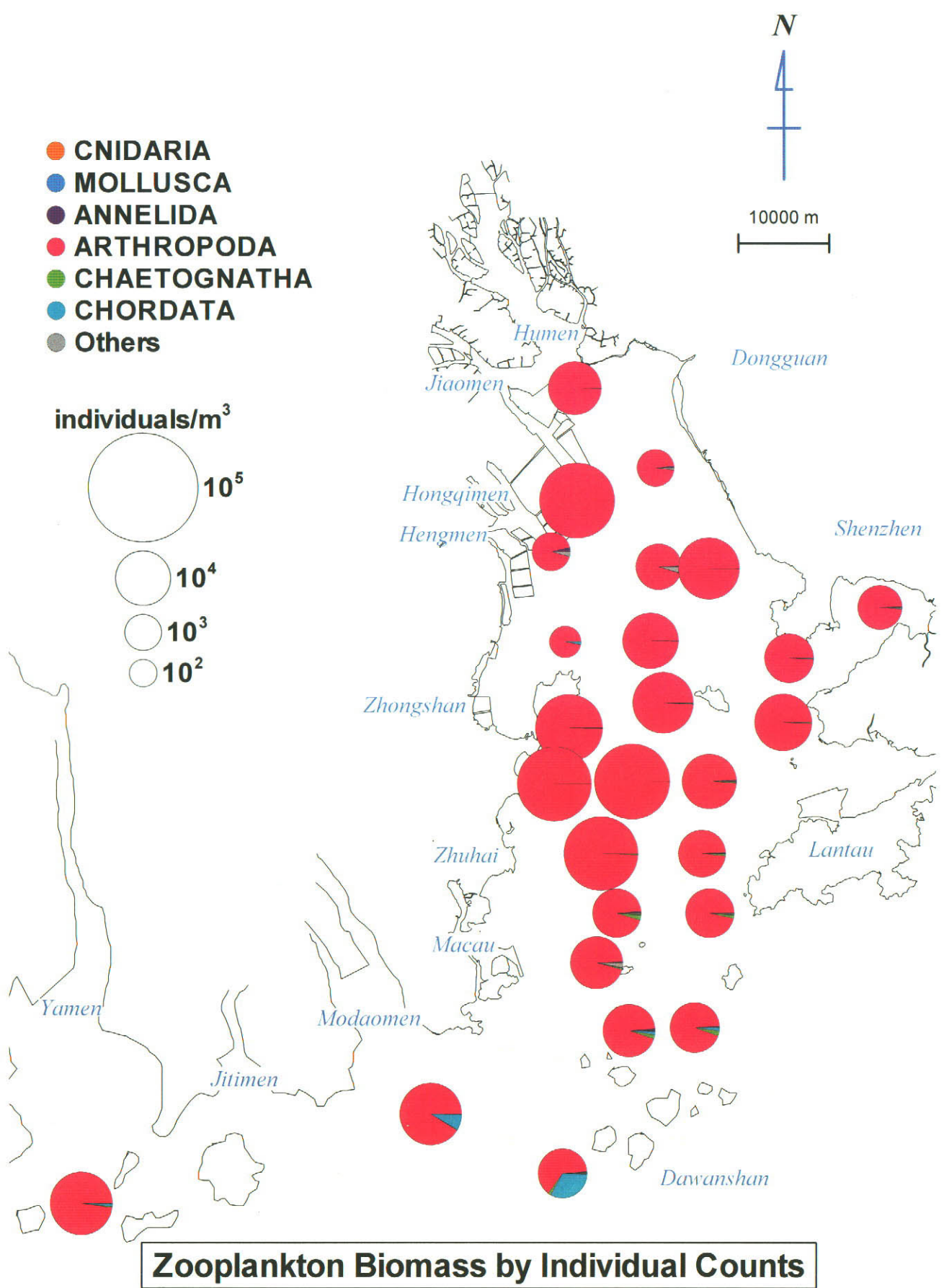
Figure 3.4.7 Result of the Survey on Zooplankton Biomass by Individual Counts (Rainy Season)
