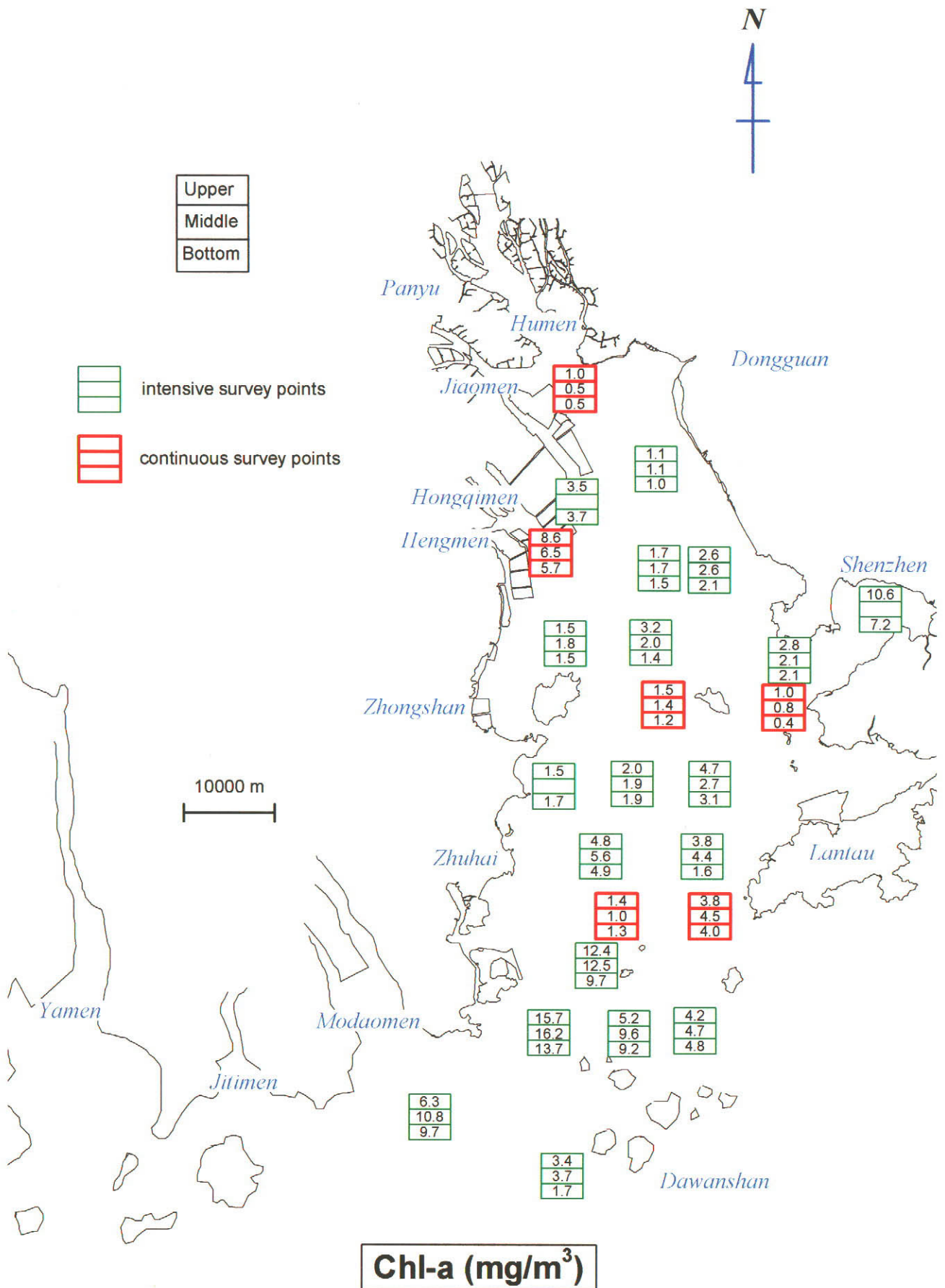
Figure 3.4.10(1) Distribution of Chlorophyll-a (Spring Tide, Dry Season)
