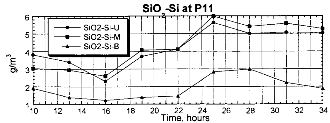
Figure 3.2.114(1) Result of the Survey on Water Quality (P11, Neap Tide, Rainy Season)
