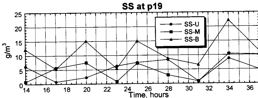
Figure 3.2.116(2) Result of the Survey on Water Quality (P19, Neap Tide, Rainy Season)
