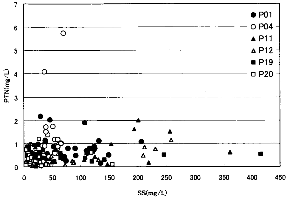
Figure 3.2.129 Scatter Chart of SS - PTN (Continuous Survey, Spring Tide, Rainy Season)
