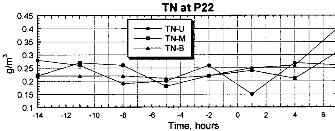
Figure 3.2.138(3) Result of the Survey on Water Quality (P22, Spring Tide, Dry Season)
