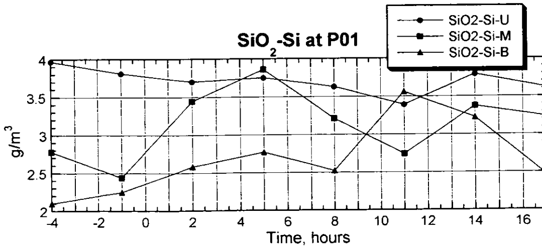
Figure 3.2.139(1) Result of the Survey on Water Quality (P01, Neap Tide, Dry Season)
