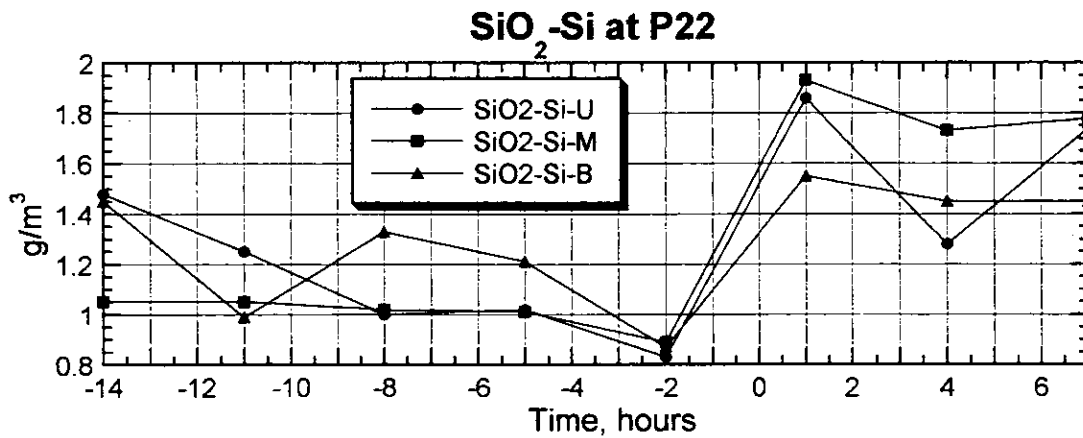
Figure 3.2.144(1) Result of the Survey on Water Quality (P22, Neap Tide, Dry Season)
