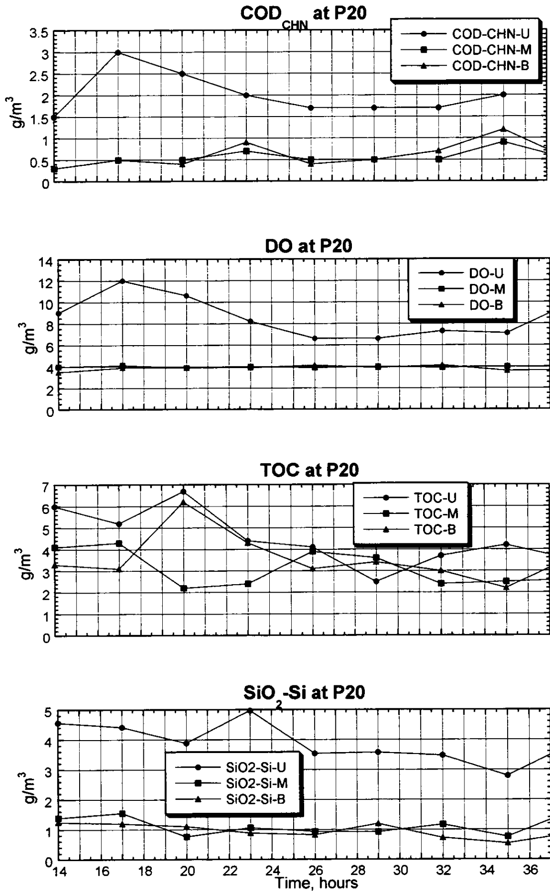
Figure 3.2.117(1) Result of the Survey on Water Quality (P20, Spring Tide, Rainy Season)
