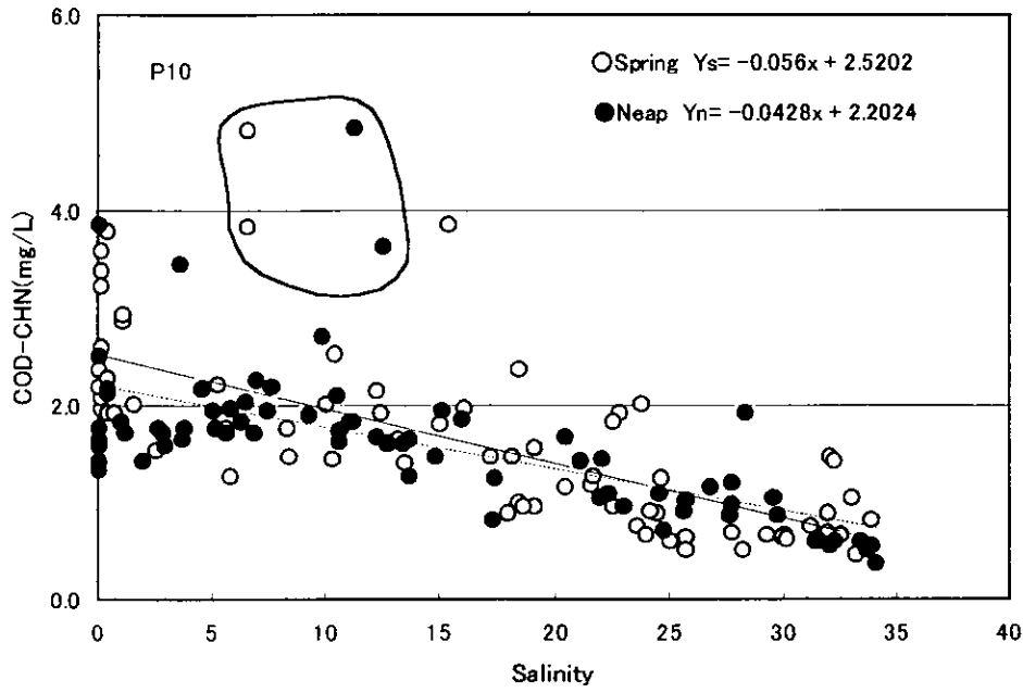
Figure 3.2.96 Scatter Chart of Salinity - COD CHN (Intensive Survey, Rainy Season)
