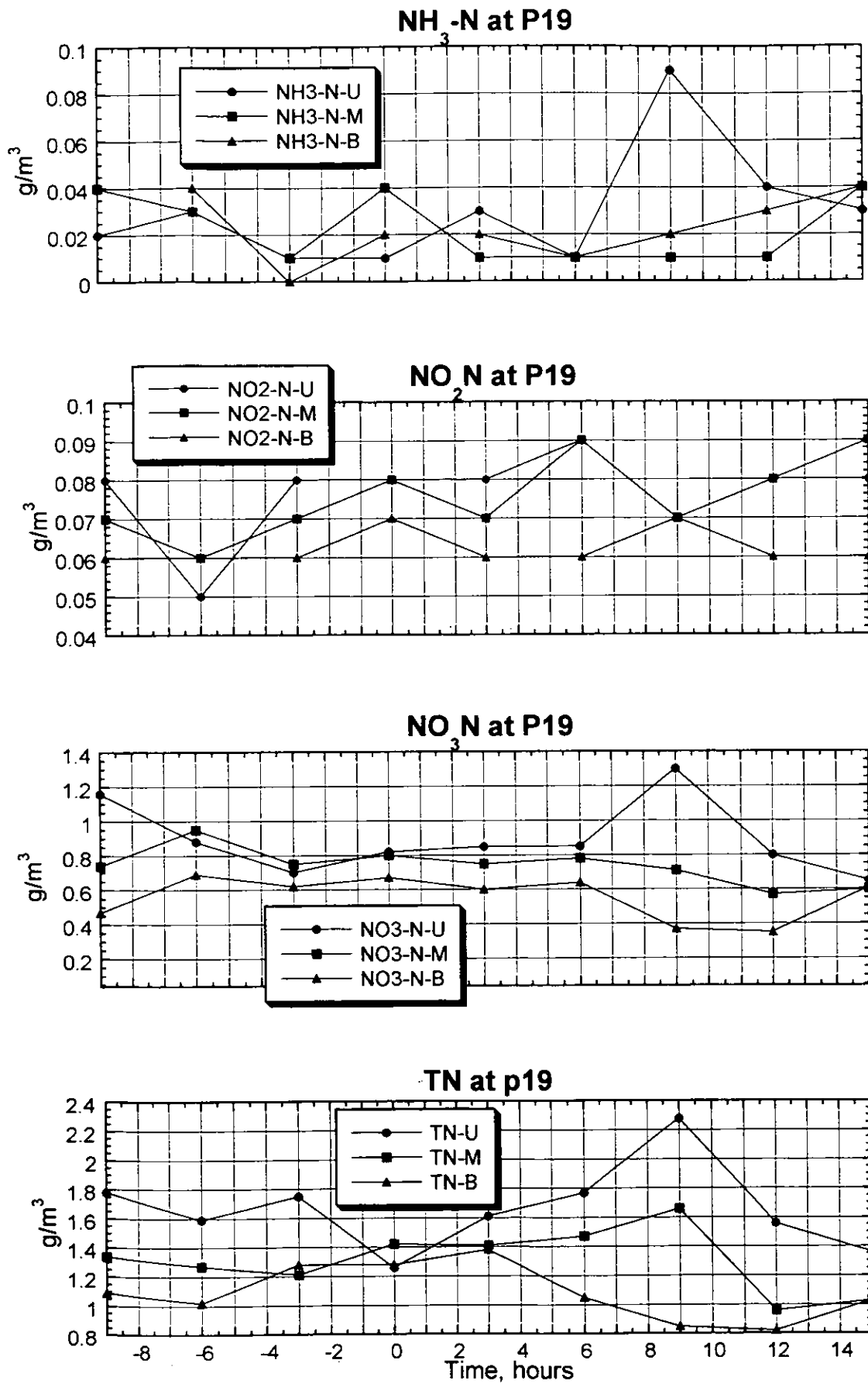
Figure 3.2.110(3) Result of the Survey on Water Quality (P19, Spring Tide, Rainy Season)
