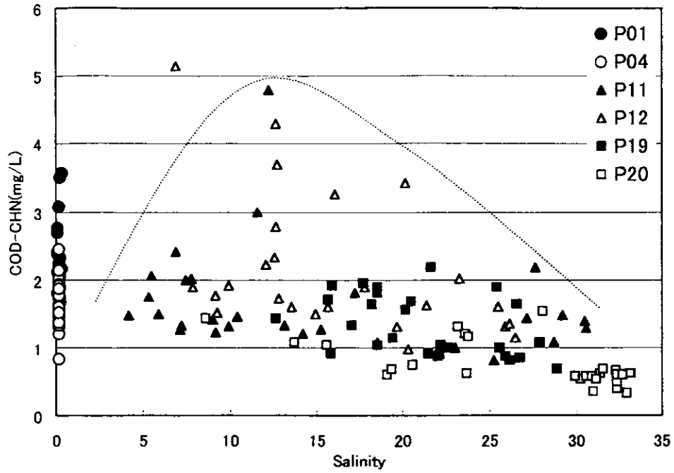
Figure 3.2.118 Scatter Chart of Salinity - COD_{CHN} (Continuous Survey, Spring Tide, Rainy Season)
