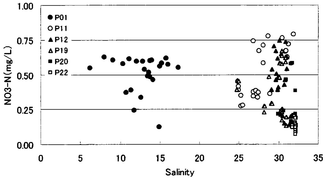
Figure 3.2.147 Scatter Chart of Salinity - NO 3 -N (Continuous Survey, Spring Tide, Dry Season)
