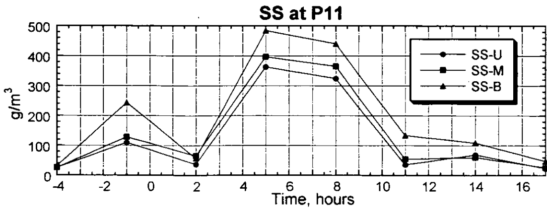
Figure 3.2.134(2) Result of the Survey on Water Quality (P11, Spring Tide, Dry Season)
