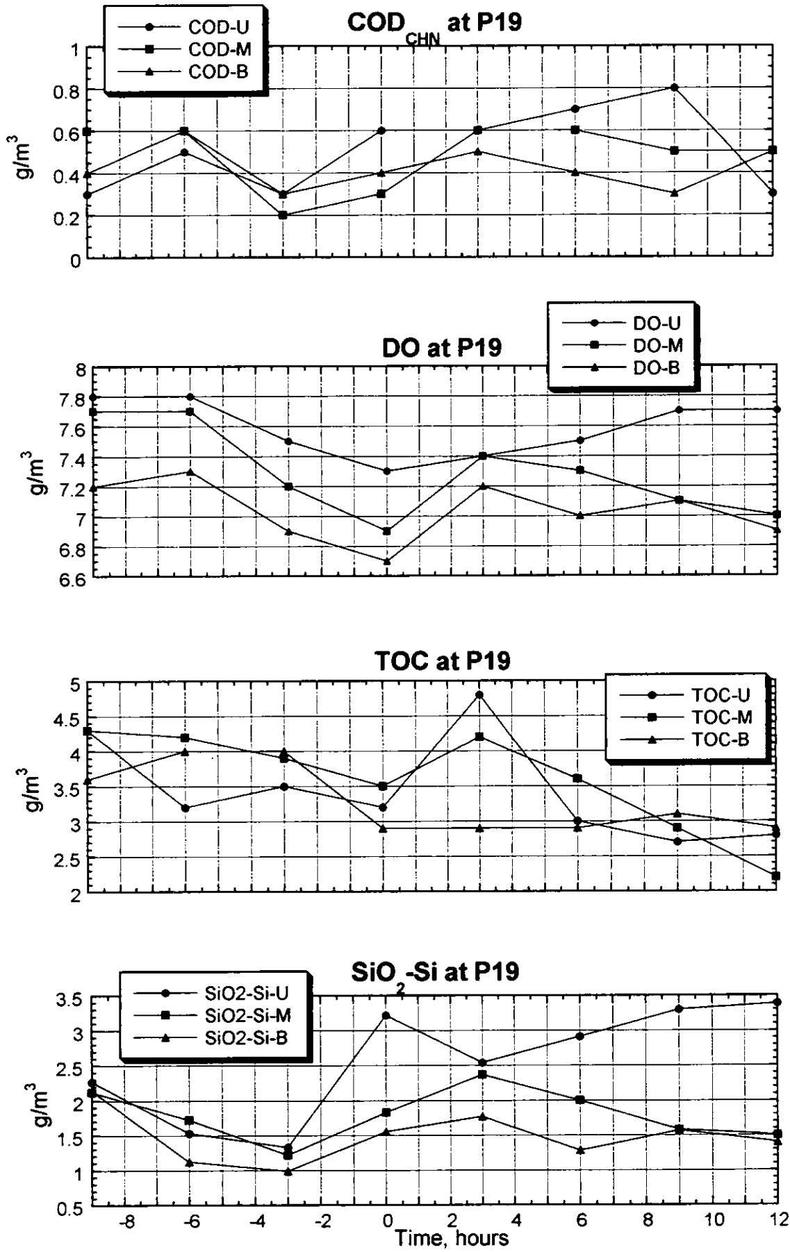
Figure 3.2.142(1) Result of the Survey on Water Quality (P19, Neap Tide, Dry Season)
