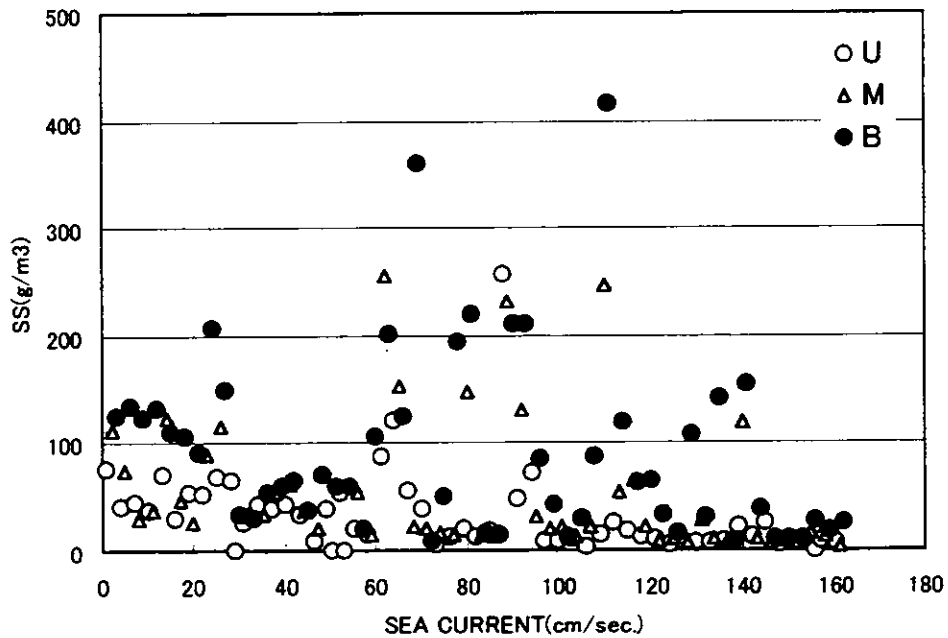
Figure 3.2.124 Scatter Chart of Sea Current - SS (Continuous Survey, Spring Tide, Rainy Season)
