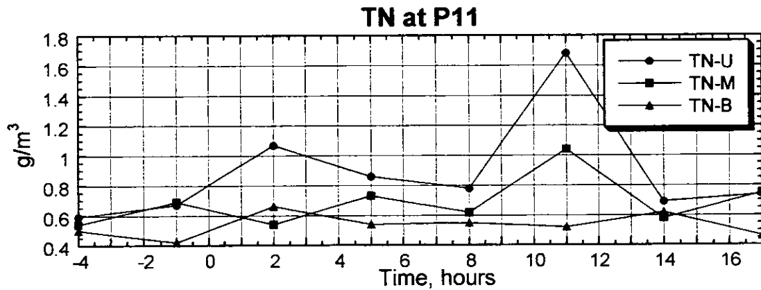
Figure 3.2.140(3) Result of the Survey on Water Quality (P11, Neap Tide, Dry Season)
