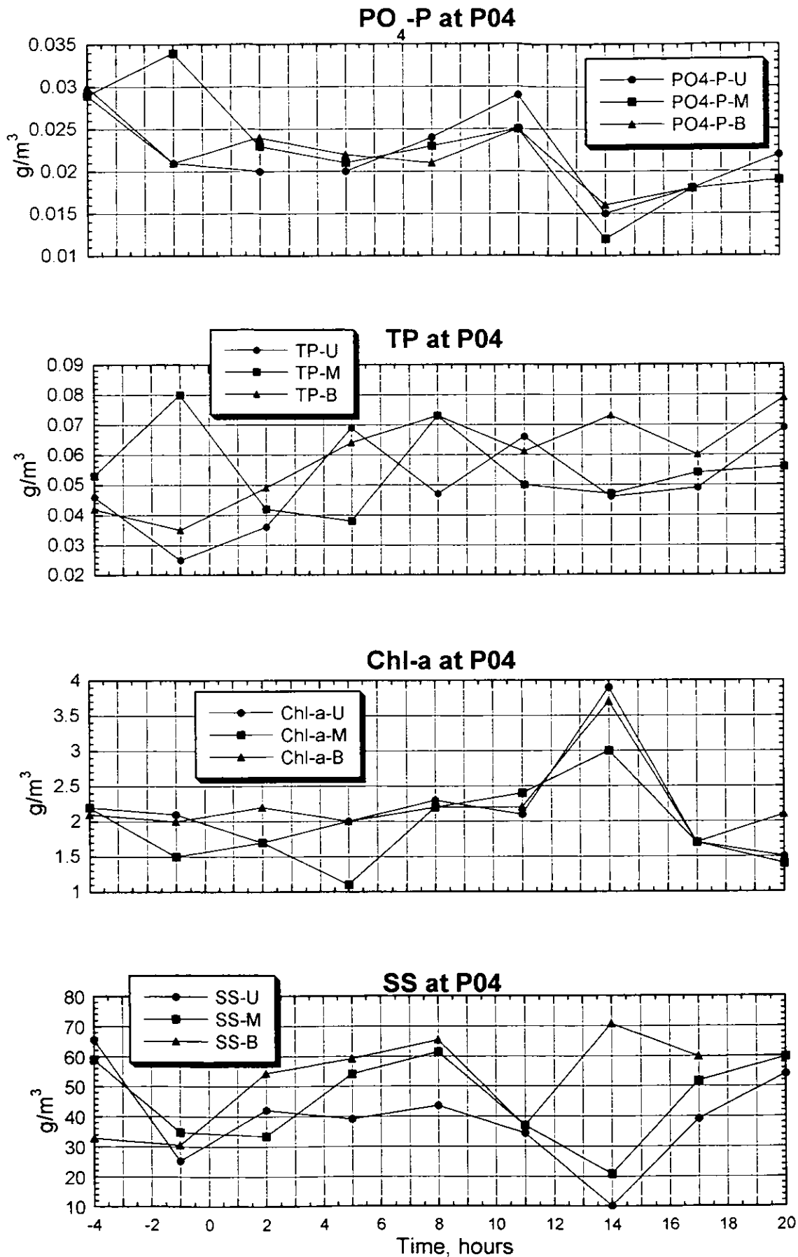
Figure 3.2.107(2) Result of the Survey on Water Quality (P04, Spring Tide, Rainy Season)
