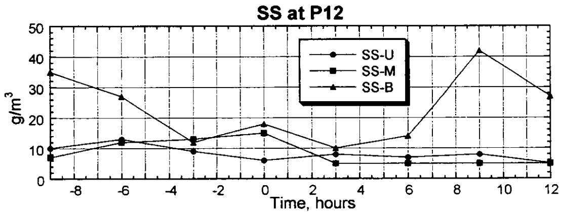
Figure 3.2.141(2) Result of the Survey on Water Quality (P12, Neap Tide, Dry Season)
