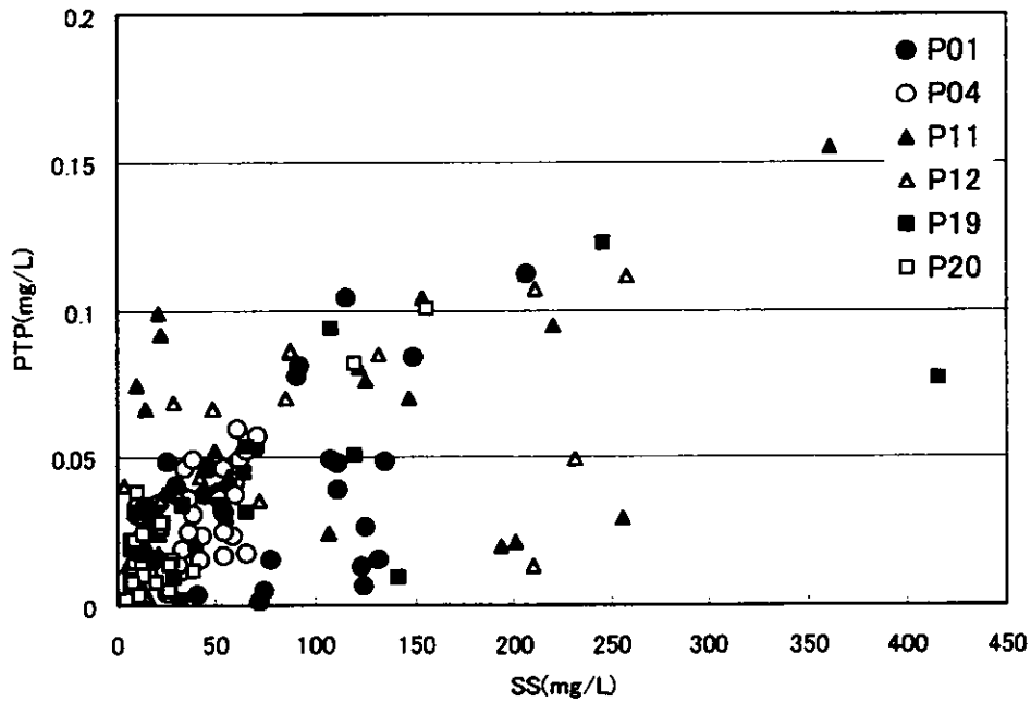
Figure 3.2.131 Scatter Chart of SS - PTP (Continuous Survey, Spring Tide, Rainy Season)
