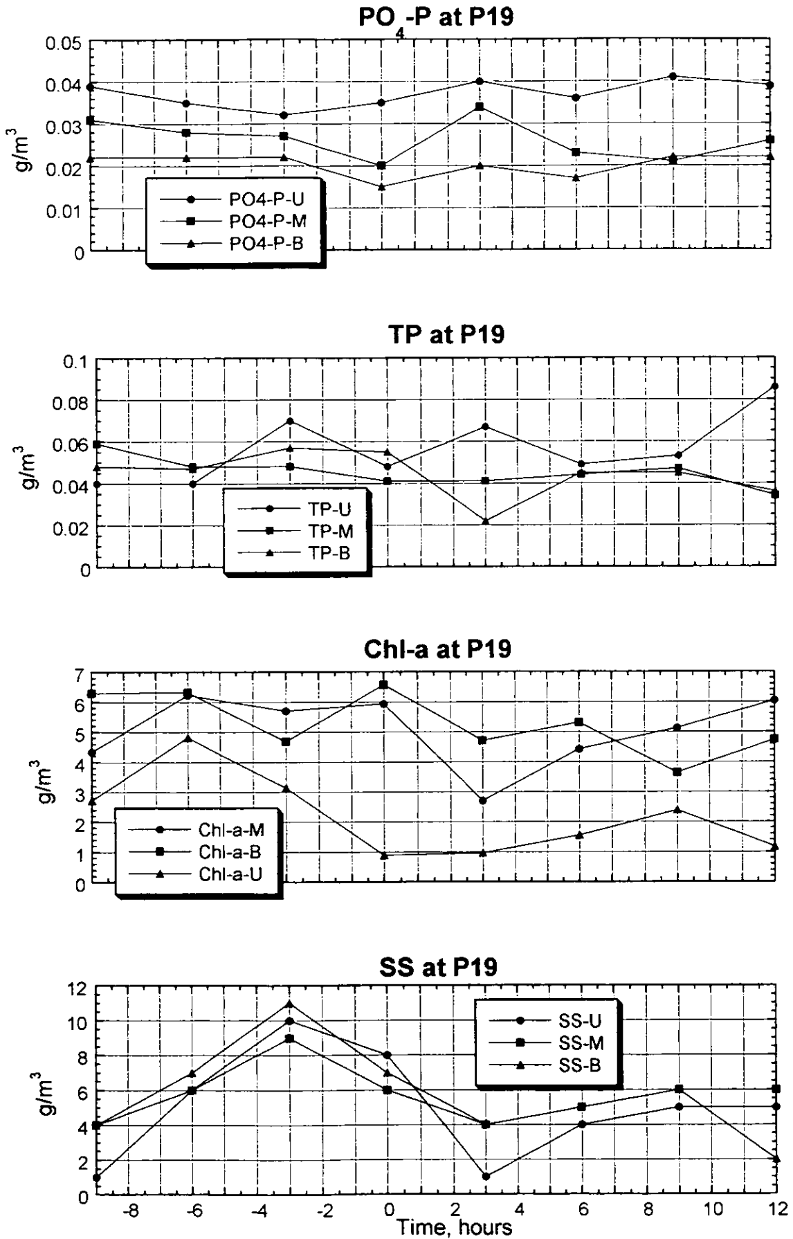
Figure 3.2.142(2) Result of the Survey on Water Quality (P19, Neap Tide, Dry Season)
