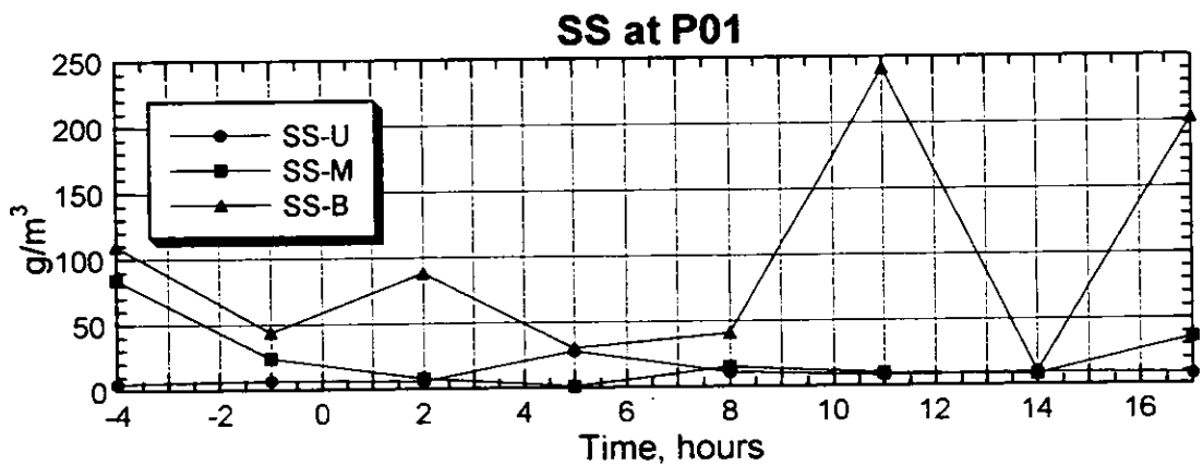
Figure 3.2.139(2) Result of the Survey on Water Quality (P01, Neap Tide, Dry Season)
