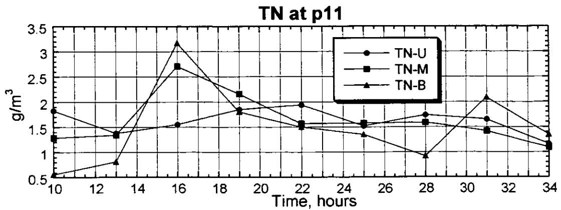
Figure 3.2.108(3) Result of the Survey on Water Quality (P11, Spring Tide, Rainy Season)
