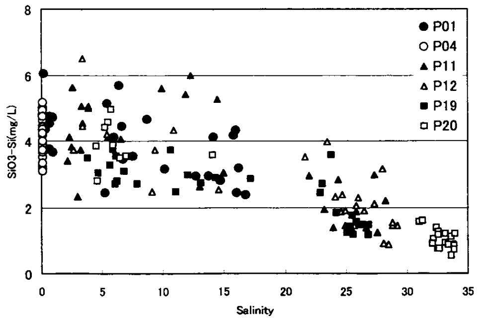
Figure 3.2.123 Scatter Chart of Salinity - \text{SiO}_3\text{-Si} (Continuous Survey, Neap Tide, Rainy Season)
