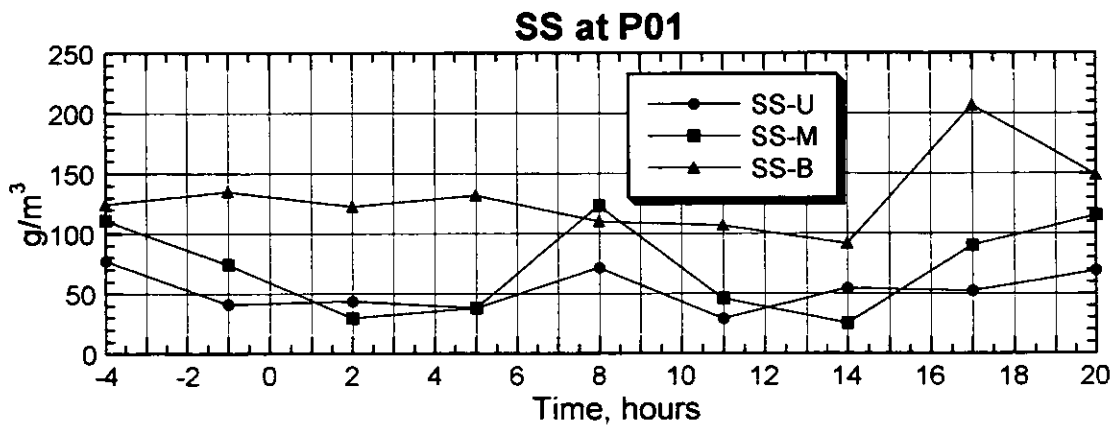
Figure 3.2.106(2) Result of the Survey on Water Quality (P01, Spring Tide, Rainy Season)
