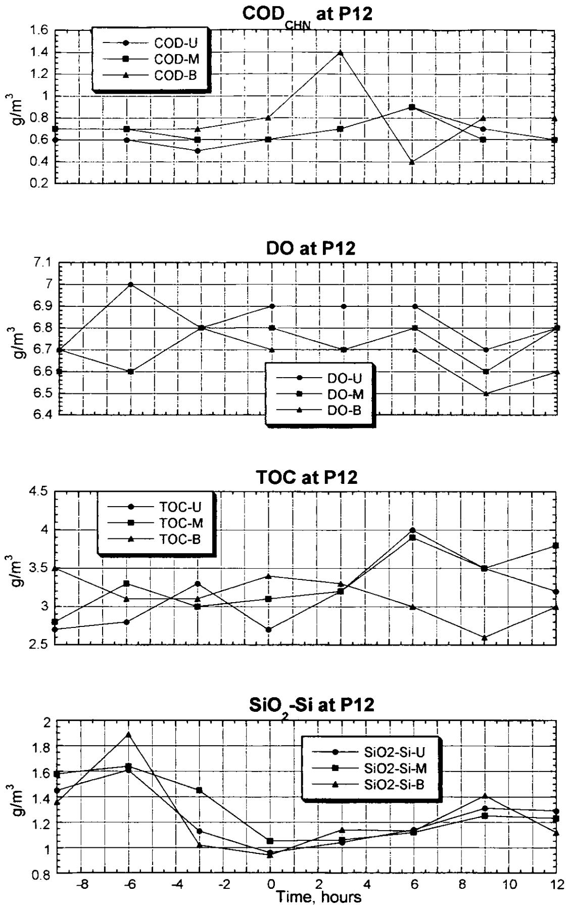
Figure 3.2.135(1) Result of the Survey on Water Quality (P12, Spring Tide, Dry Season)
