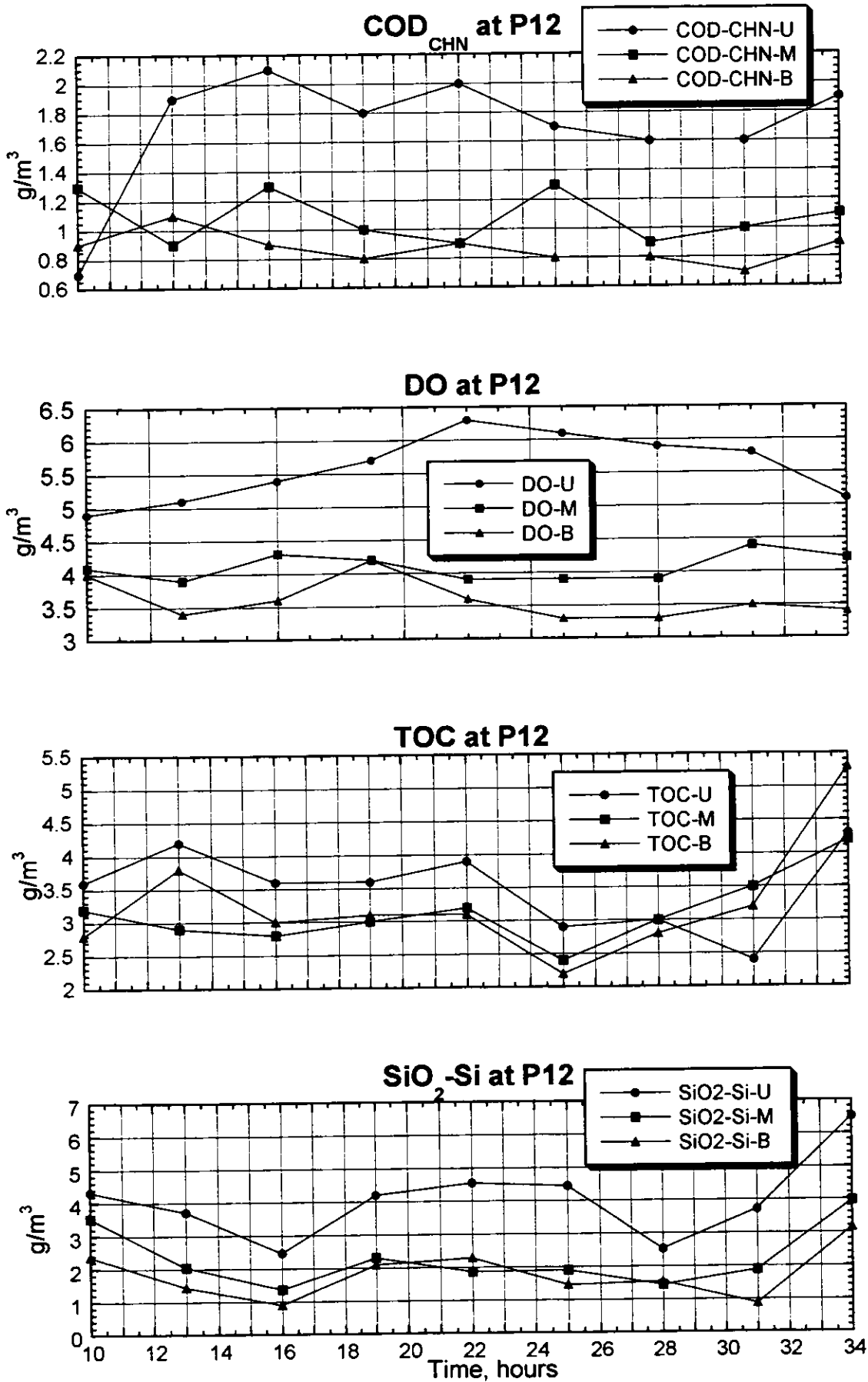
Figure 3.2.115(1) Result of the Survey on Water Quality (P12, Neap Tide, Rainy Season)
