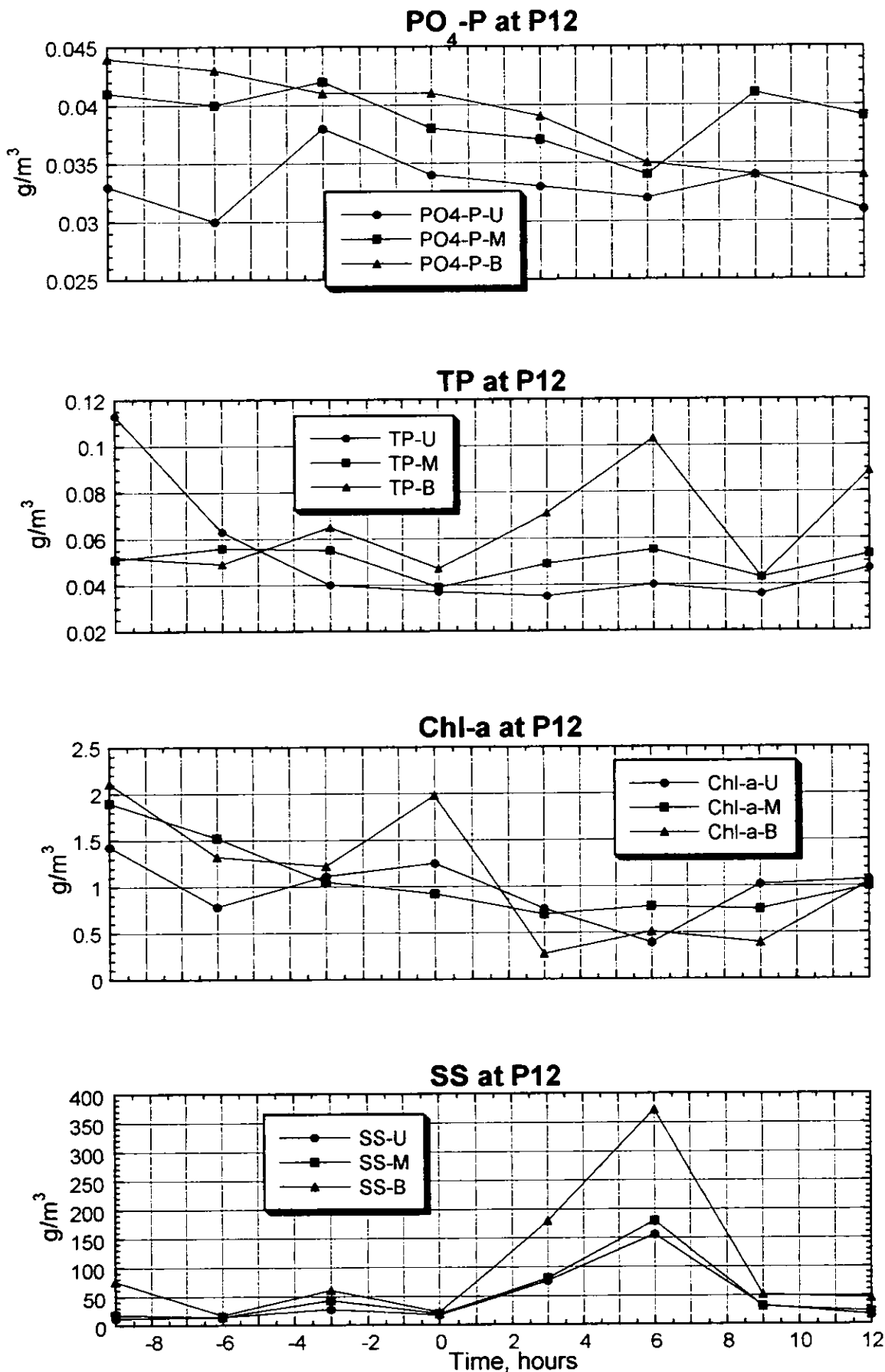
Figure 3.2.135(2) Result of the Survey on Water Quality (P12, Spring Tide, Dry Season)
