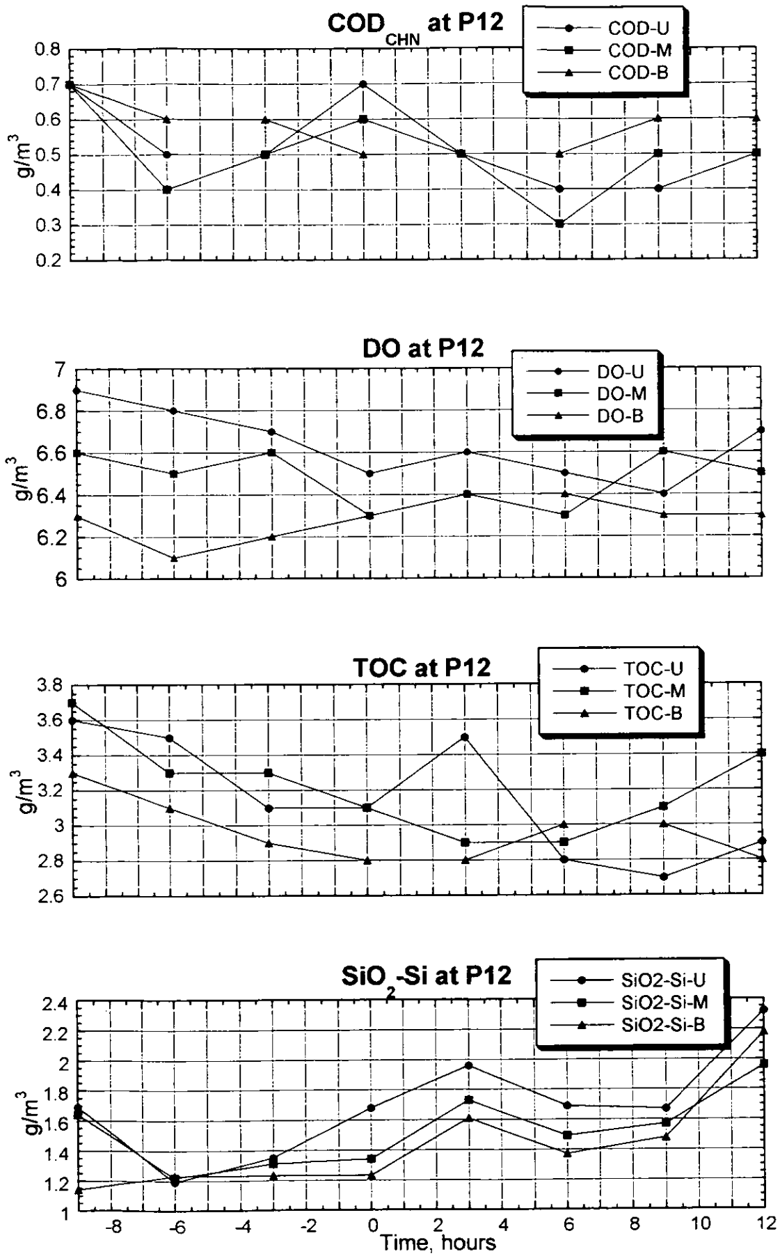
Figure 3.2.141(1) Result of the Survey on Water Quality (P12, Neap Tide, Dry Season)
