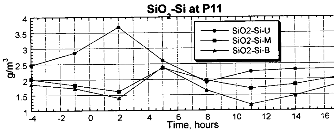
Figure 3.2.140(1) Result of the Survey on Water Quality (P11, Neap Tide, Dry Season)
