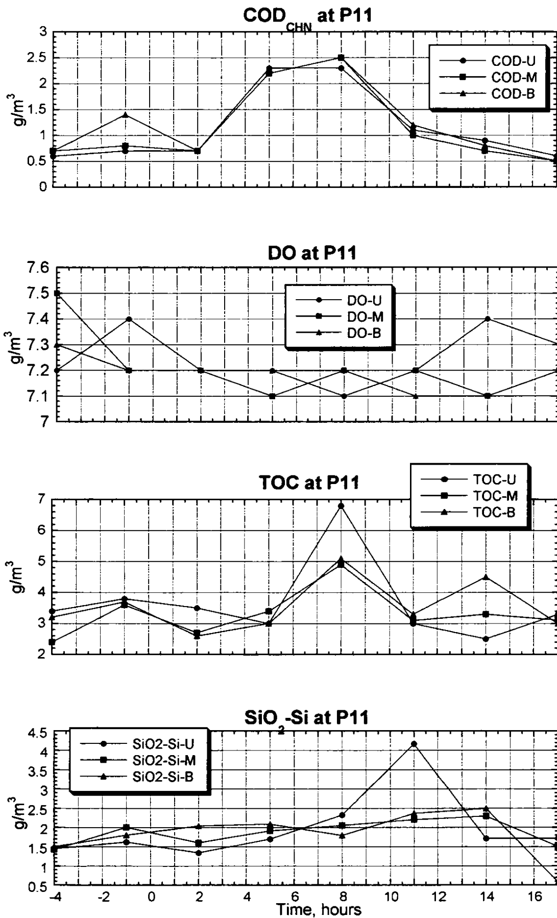
Figure 3.2.134(1) Result of the Survey on Water Quality (P11, Spring Tide, Dry Season)
