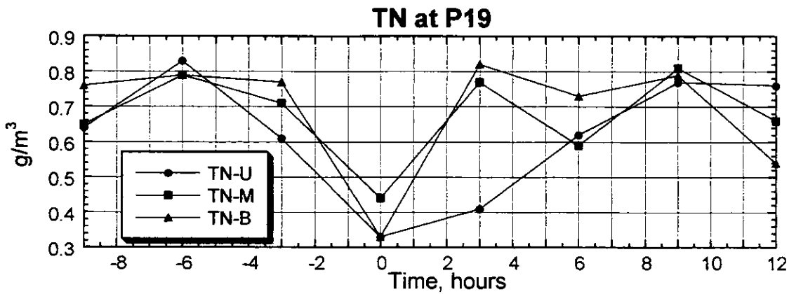
Figure 3.2.136(3) Result of the Survey on Water Quality (P19, Spring Tide, Dry Season)
