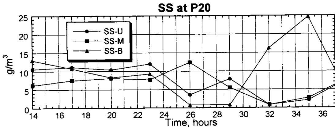
Figure 3.2.117(2) Result of the Survey on Water Quality (P20, Spring Tide, Rainy Season)
