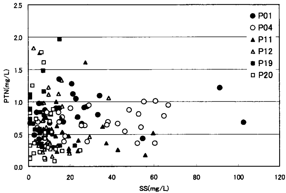
Figure 3.2.130 Scatter Chart of SS - PTN (Continuous Survey, Neap Tide, Rainy Season)
