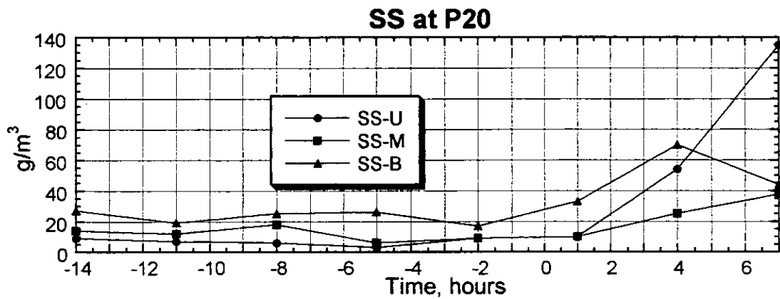
Figure 3.2.137(2) Result of the Survey on Water Quality (P20, Spring Tide, Dry Season)
