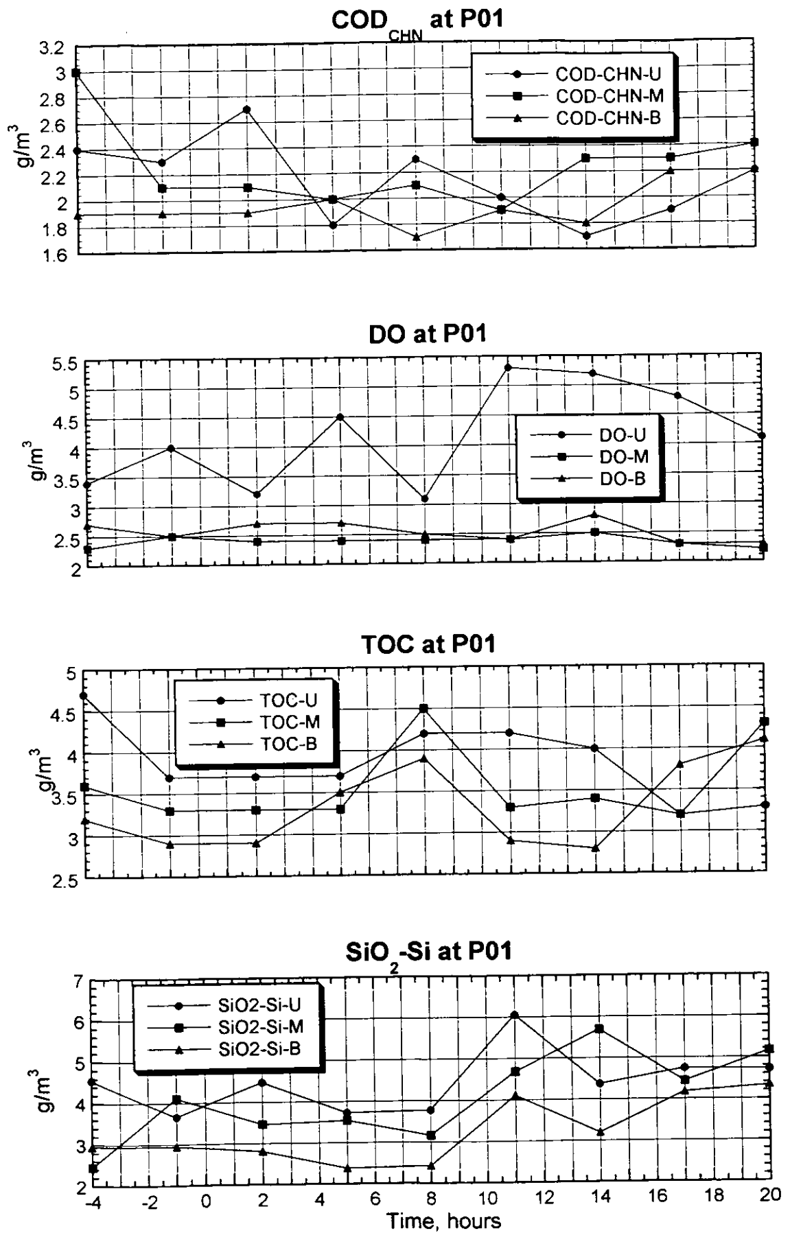
Figure 3.2.112(1) Result of the Survey on Water Quality (P01, Neap Tide, Rainy Season)
