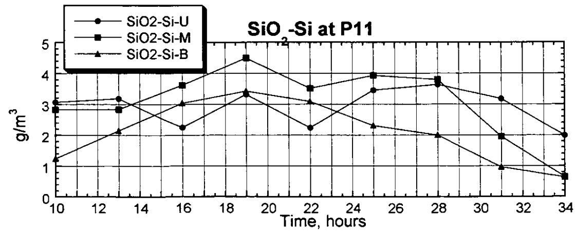
Figure 3.2.108(1) Result of the Survey on Water Quality (P11, Spring Tide, Rainy Season)
