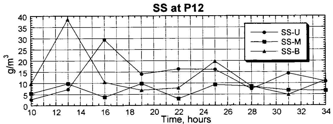
Figure 3.2.115(2) Result of the Survey on Water Quality (P12, Neap Tide, Rainy Season)
