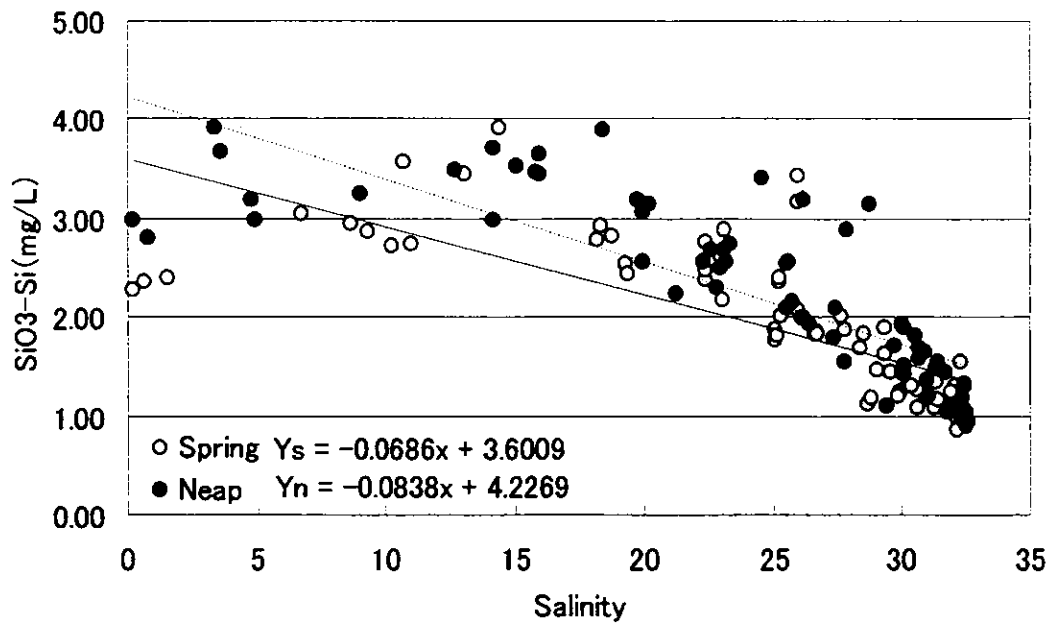
Figure 3.2.103 Scatter Chart of Salinity - SiO 3 -Si (Intensive Survey, Dry Season)
