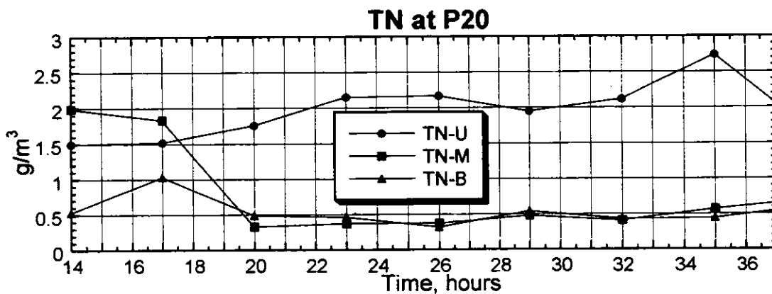
Figure 3.2.117(3) Result of the Survey on Water Quality (P20, Spring Tide, Rainy Season)
