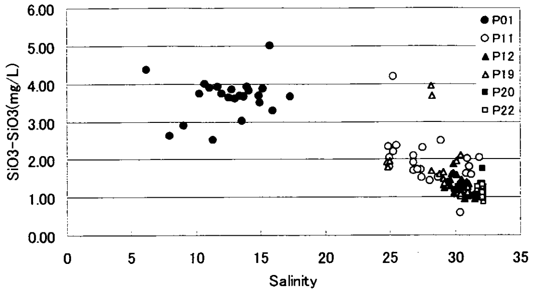
Figure 3.2.149 Scatter Chart of Salinity : SiO 3 -Si (Continuous Survey, Spring Tide, Dry Season)
