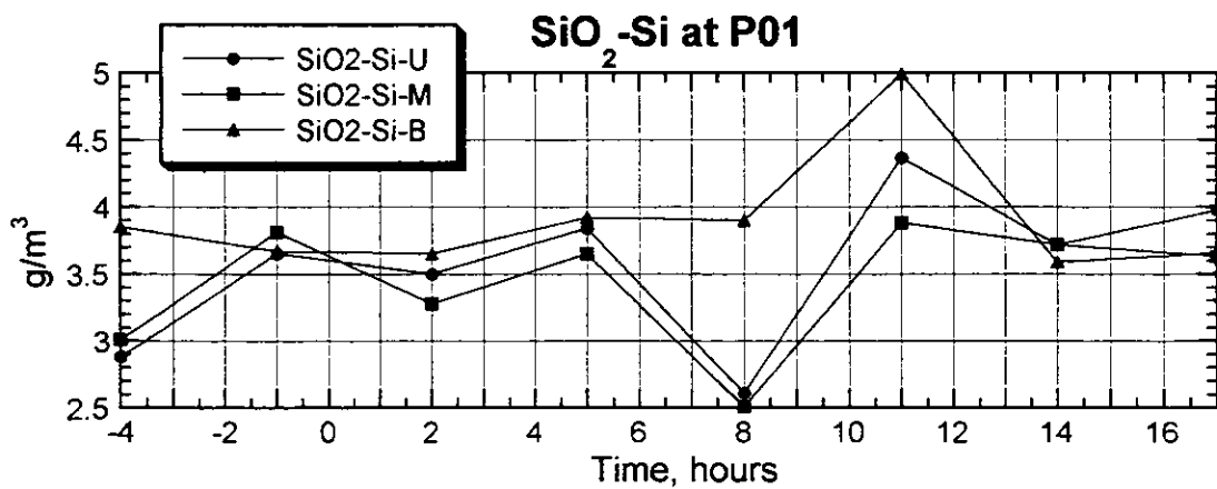
Figure 3.2.133(1) Result of the Survey on Water Quality (P01, Spring Tide, Dry Season)
