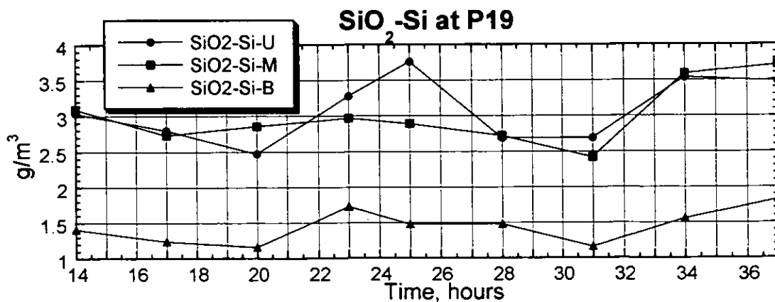
Figure 3.2.116(1) Result of the Survey on Water Quality (P19, Neap Tide, Rainy Season)
