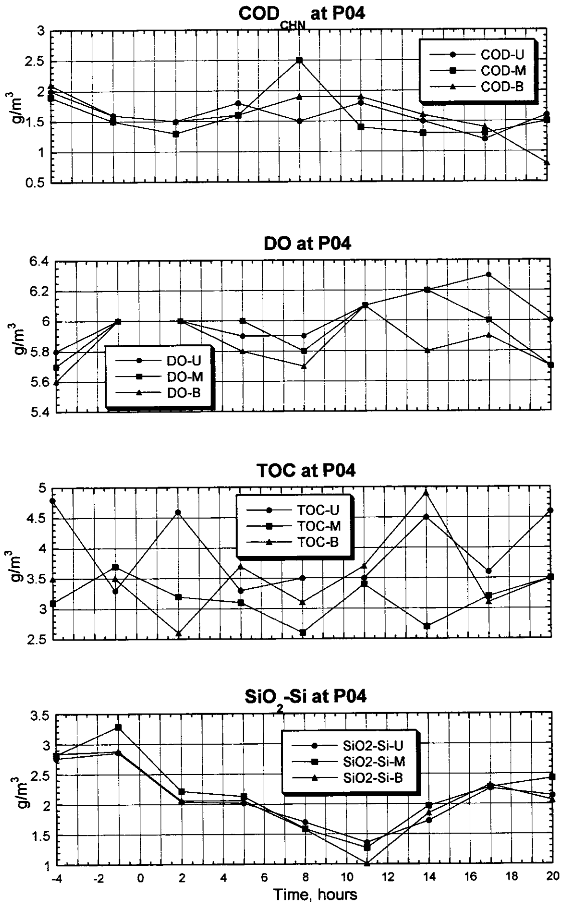
Figure 3.2.107(1) Result of the Survey on Water Quality (P04, Spring Tide, Rainy Season)
