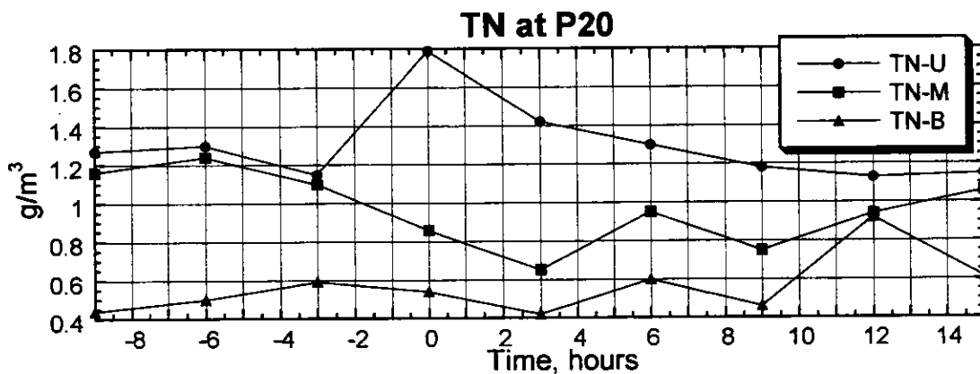
Figure 3.2.111(3) Result of the Survey on Water Quality (P20, Spring Tide, Rainy Season)
