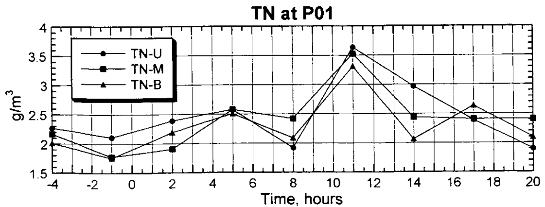
Figure 3.2.106(3) Result of the Survey on Water Quality (P01, Spring Tide, Rainy Season)
