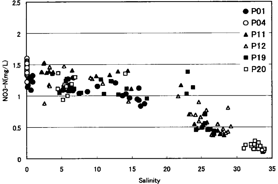
Figure 3.2.121 Scatter Chart of Salinity - NO 3 -N (Continuous Survey, Neap Tide, Rainy Season)
