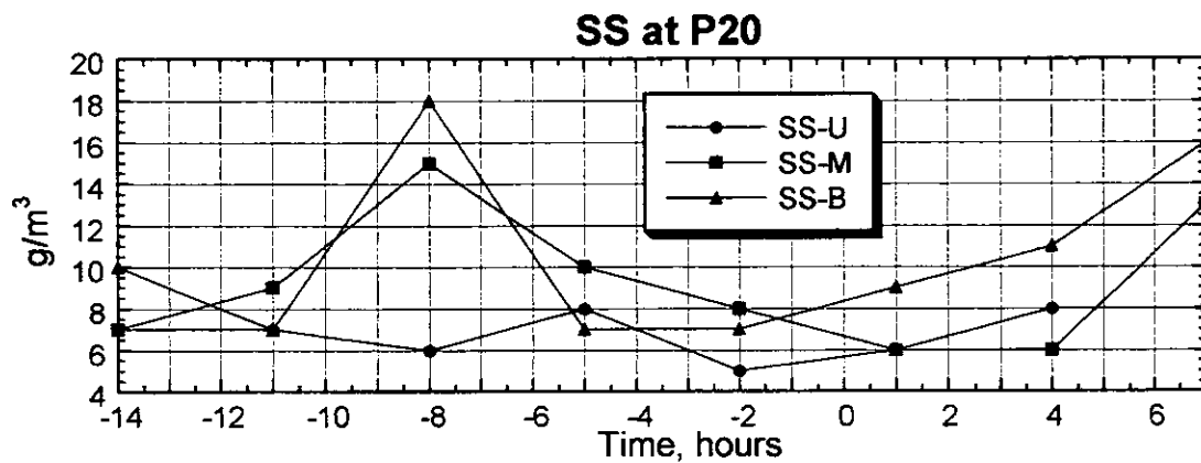
Figure 3.2.143(2) Result of the Survey on Water Quality (P20, Neap Tide, Dry Season)
