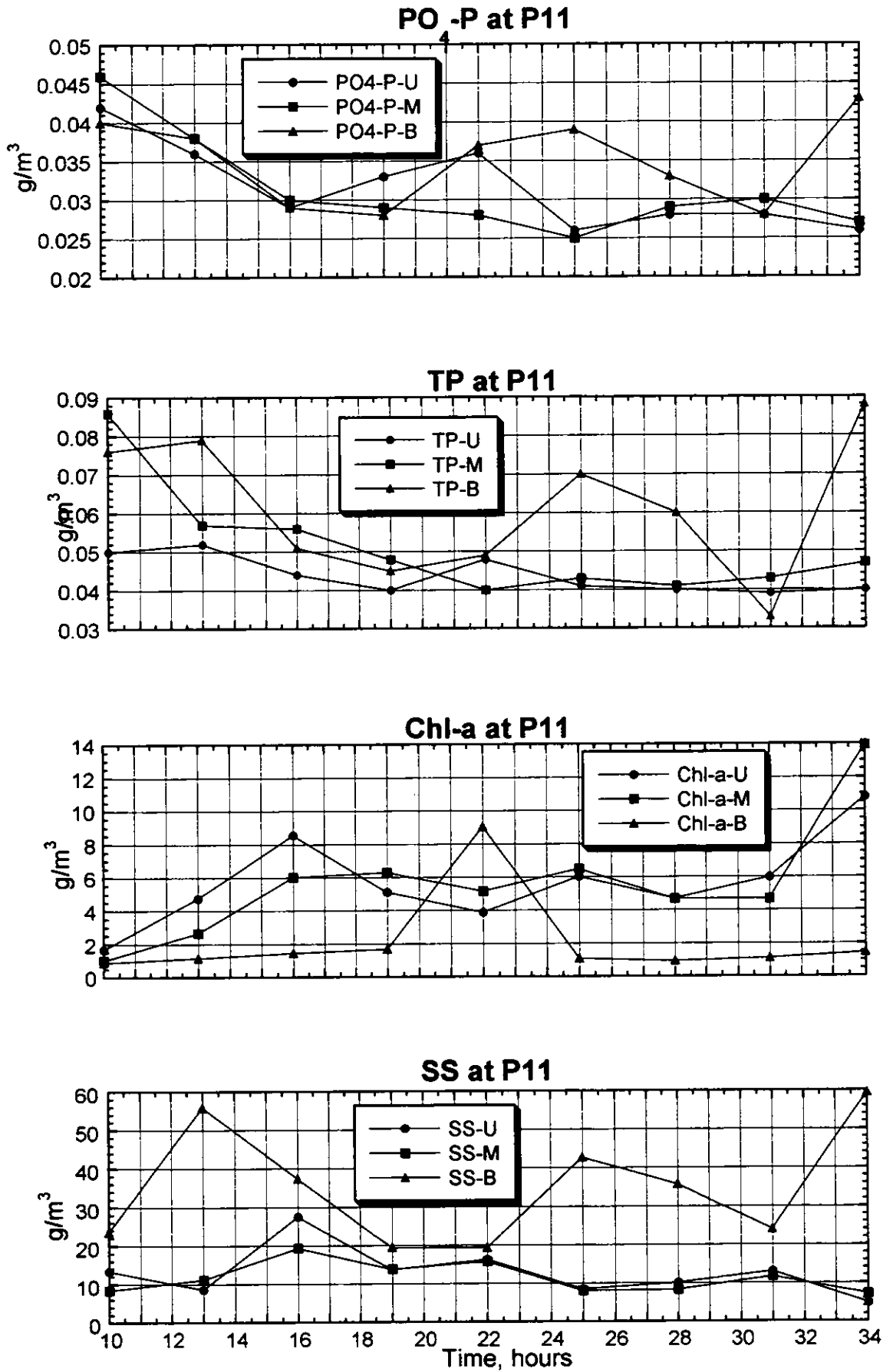
Figure 3.2.114(2) Result of the Survey on Water Quality (P11, Neap Tide, Rainy Season)
