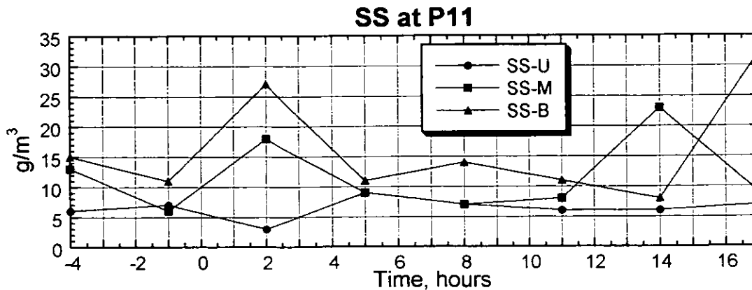
Figure 3.2.140(2) Result of the Survey on Water Quality (P11, Neap Tide, Dry Season)
