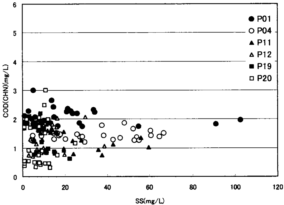
Figure 3.2.128 Scatter Chart of SS - COD (Continuous Survey, Neap Tide, Rainy Season)
