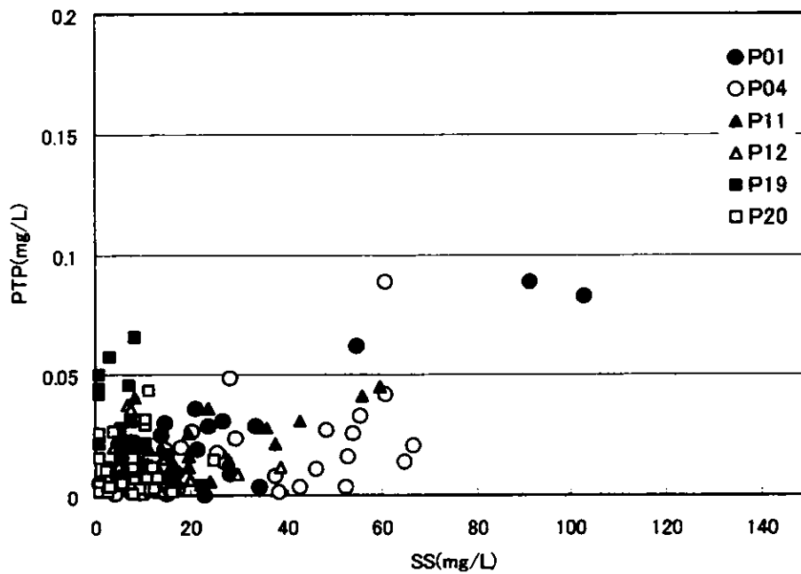
Figure 3.2.132 Scatter Chart of SS - PTP (Continuous Survey, Neap Tide, Rainy Season)
