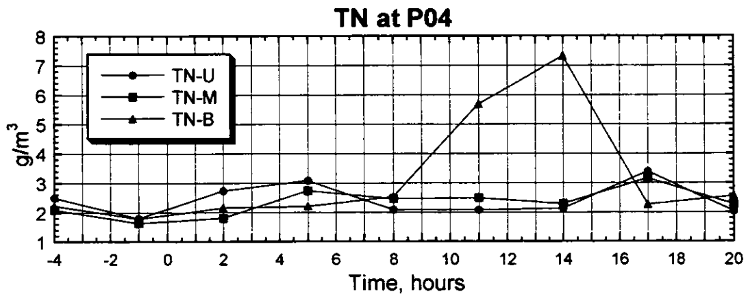
Figure 3.2.107(3) Result of the Survey on Water Quality (P04, Spring Tide, Rainy Season)
