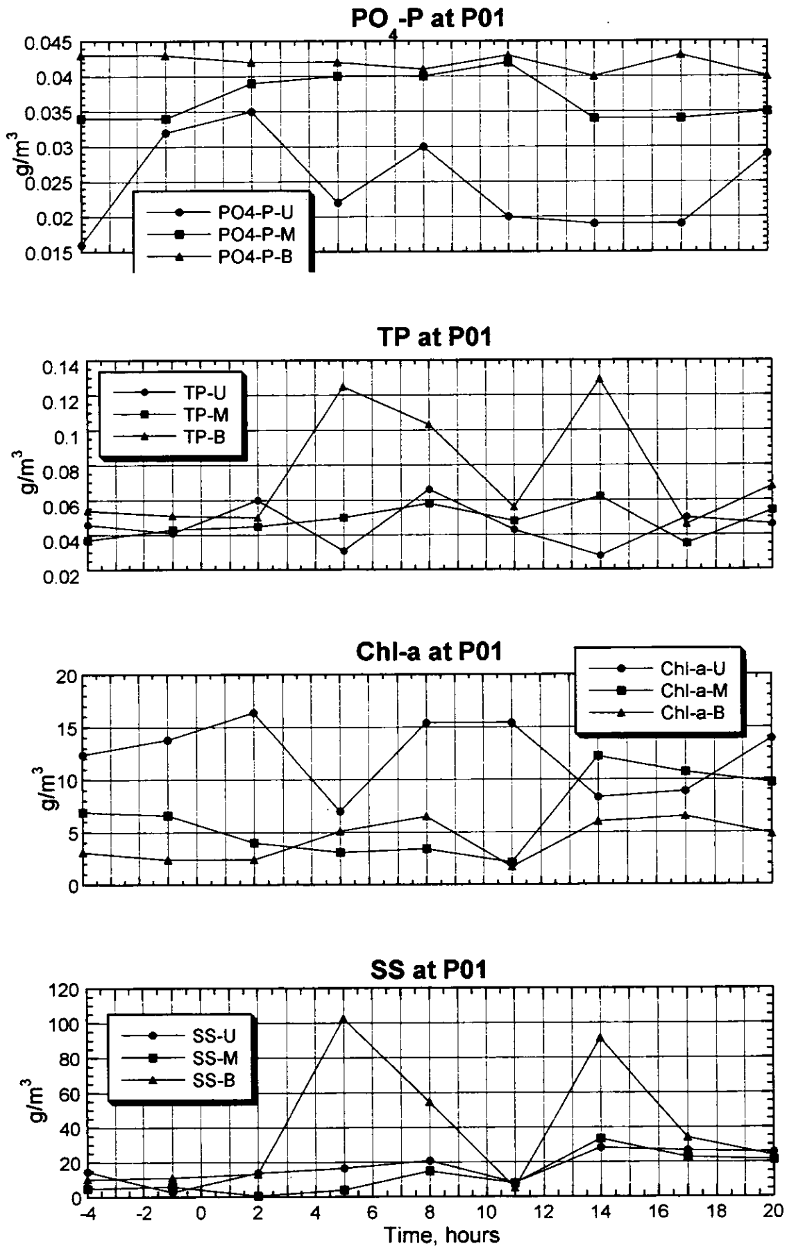
Figure 3.2.112(2) Result of the Survey on Water Quality (P01, Neap Tide, Rainy Season)
