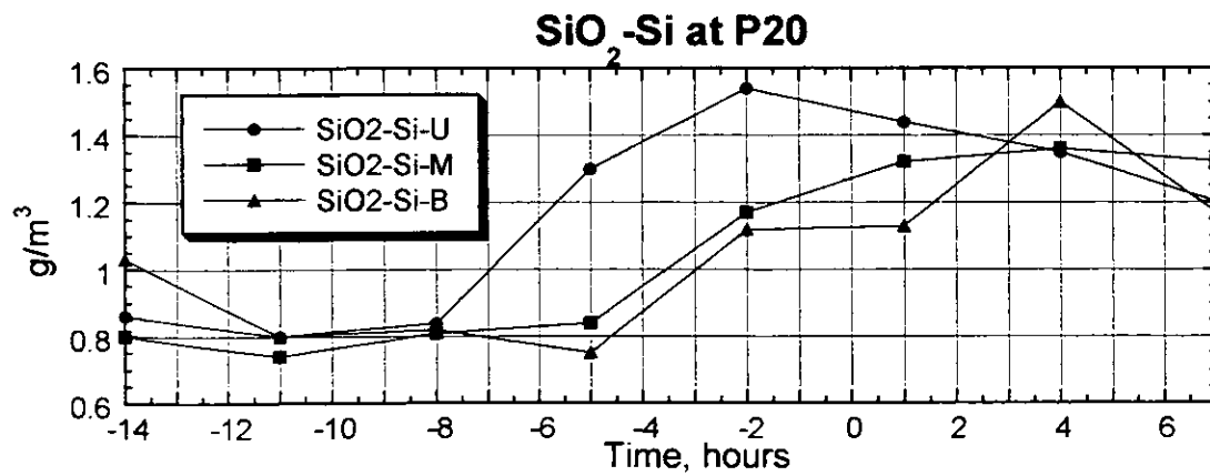
Figure 3.2.143(1) Result of the Survey on Water Quality (P20, Neap Tide, Dry Season)
