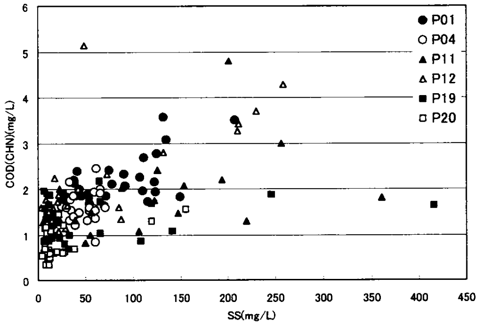
Figure 3.2.127 Scatter Chart of SS - COD (Continuous Survey, Spring Tide, Rainy Season)
