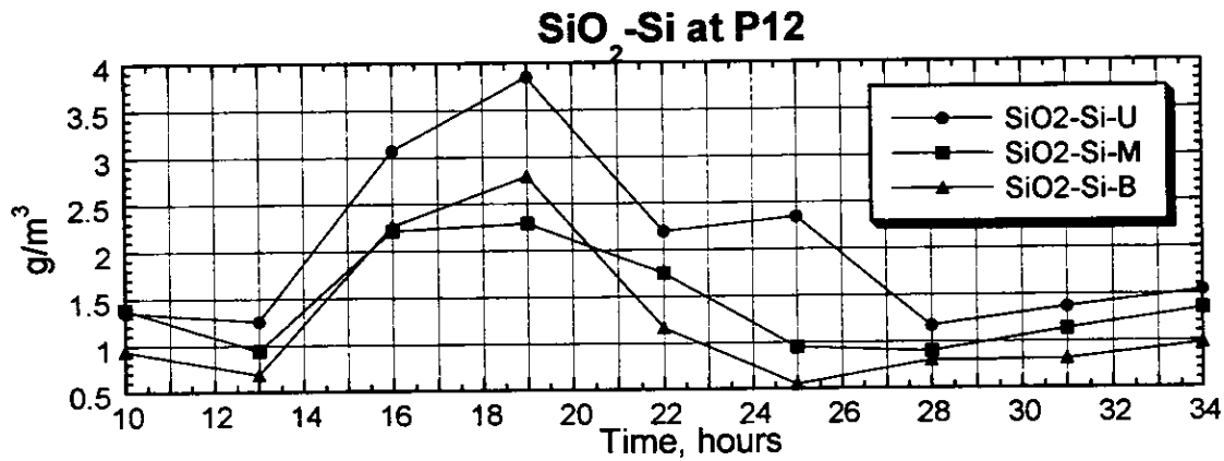
Figure 3.2.109(1) Result of the Survey on Water Quality (P12, Spring Tide, Rainy Season)
