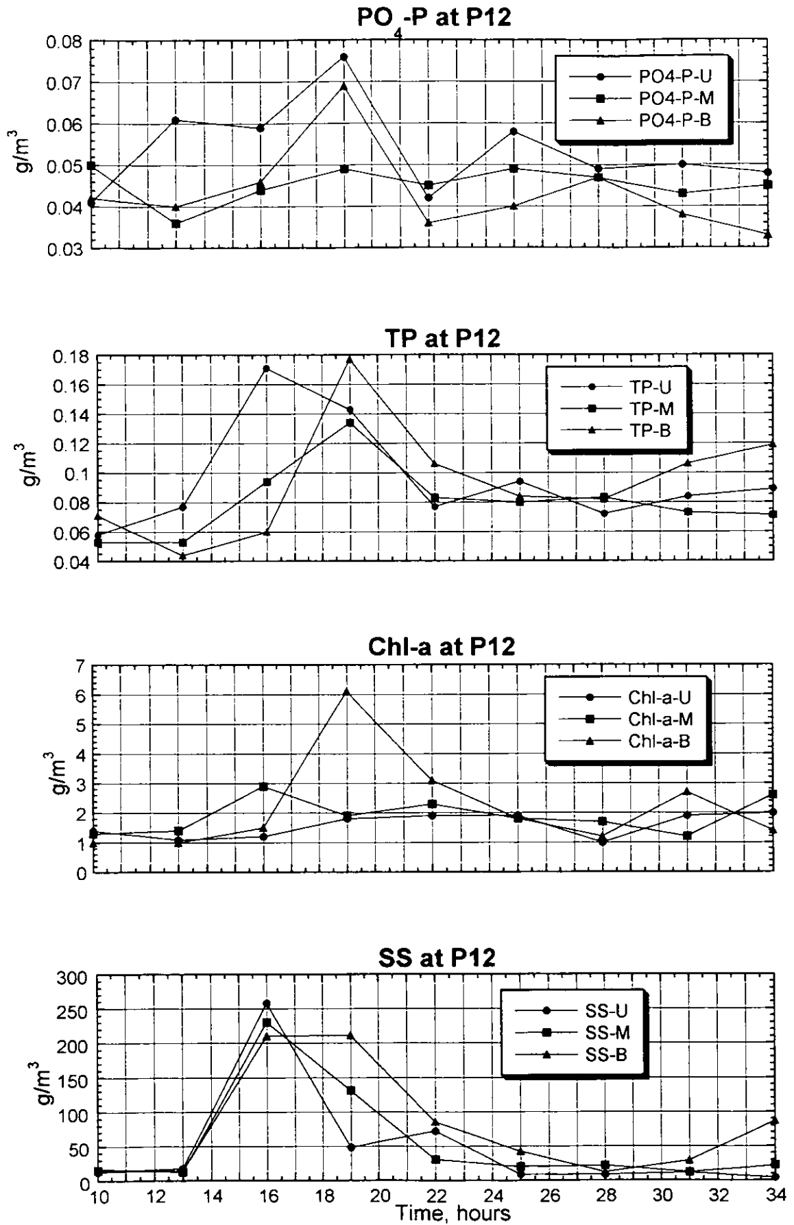
Figure 3.2.109(2) Result of the Survey on Water Quality (P12, Spring Tide, Rainy Season)
