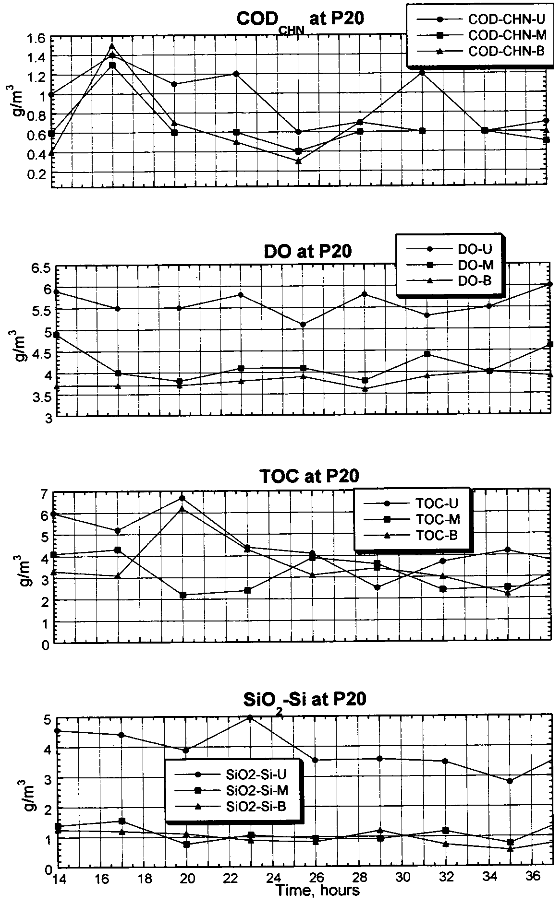
Figure 3.2.111(1) Result of the Survey on Water Quality (P20, Spring Tide, Rainy Season)
