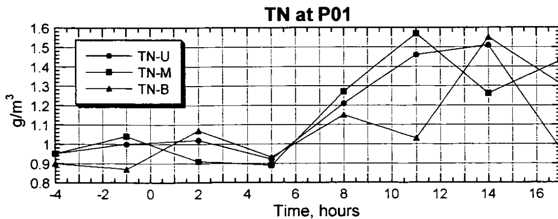
Figure 3.2.133(3) Result of the Survey on Water Quality (P01, Spring Tide, Dry Season)
