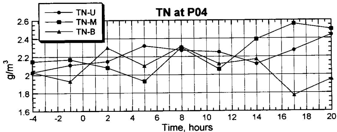
Figure 3.2.113(3) Result of the Survey on Water Quality (P04, Neap Tide, Rainy Season)
