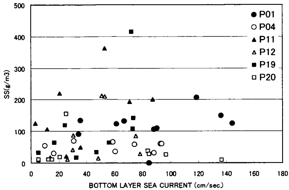
Figure 3.2.126 Scatter Chart of Bottom Layer Sea Current - SS (Continuous Survey, Neap Tide, Rainy Season)
