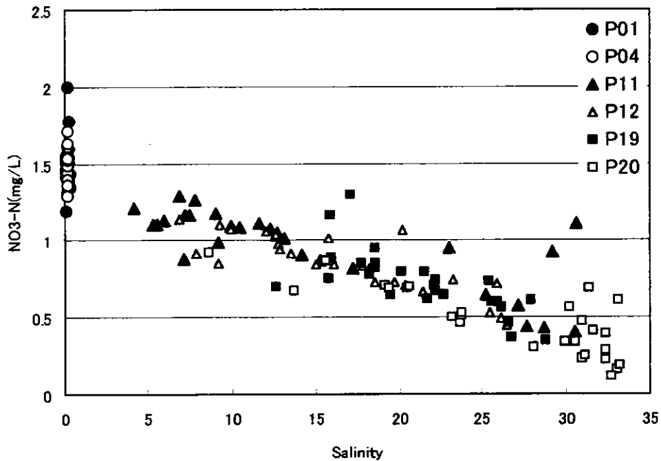
Figure 3.2.120 Scatter Chart of Salinity - NO 3 -N (Continuous Survey, Spring Tide, Rainy Season)
