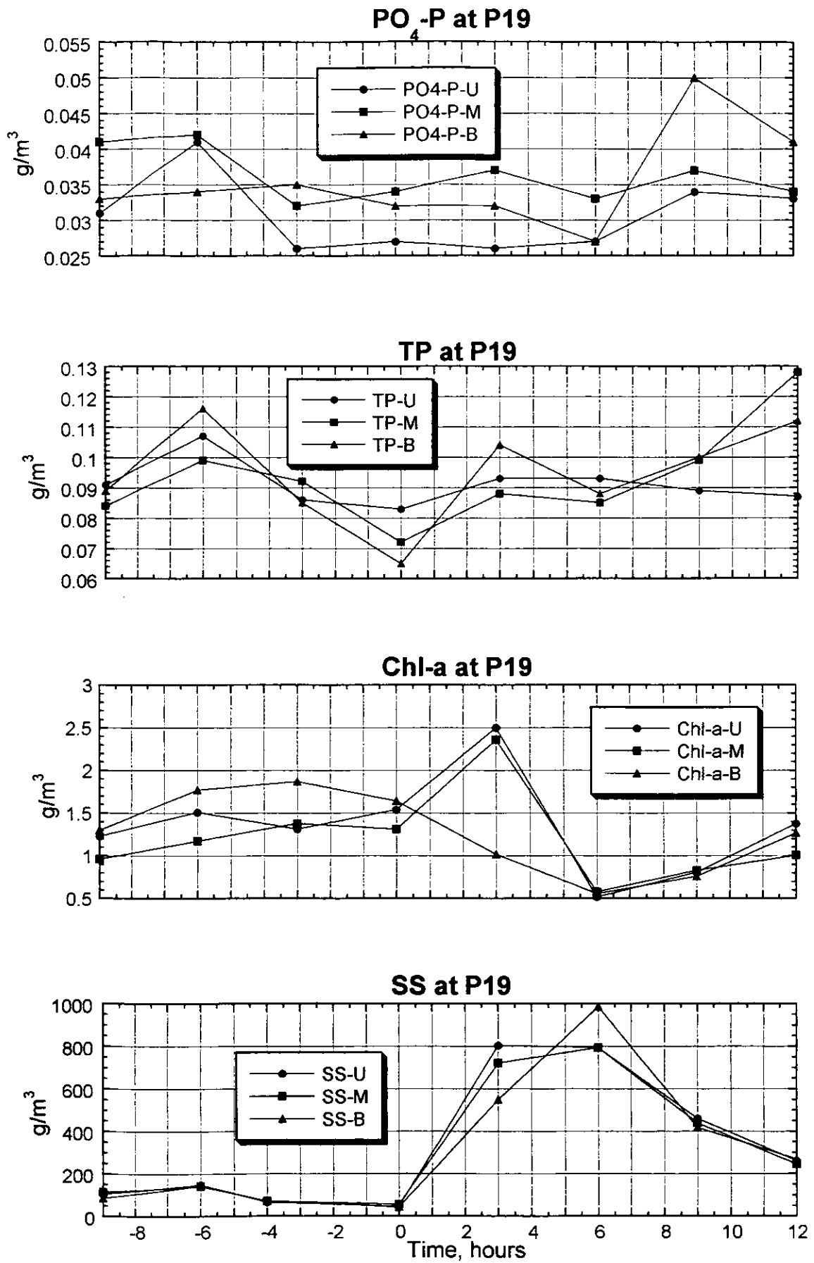
Figure 3.2.136(2) Result of the Survey on Water Quality (P19, Spring Tide, Dry Season)
