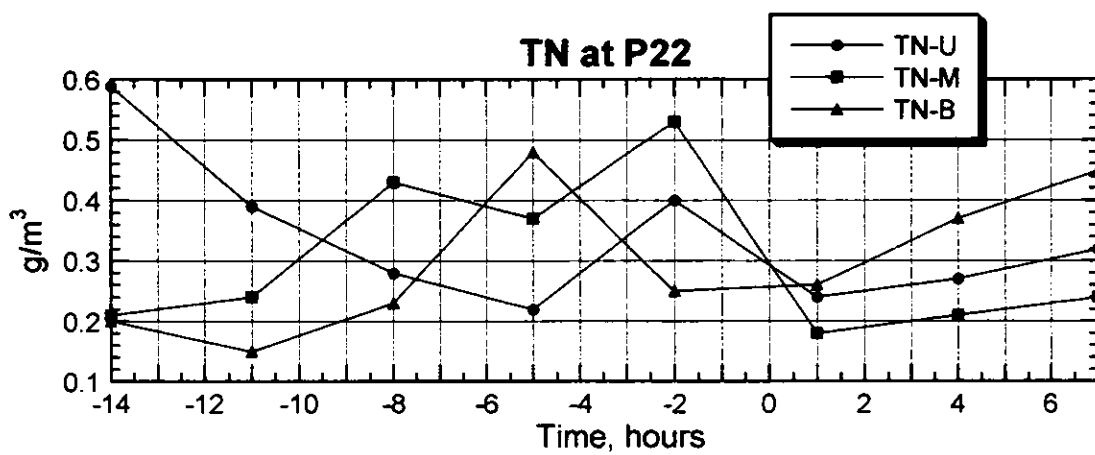
Figure 3.2.144(3) Result of the Survey on Water Quality (P22, Neap Tide, Dry Season)
