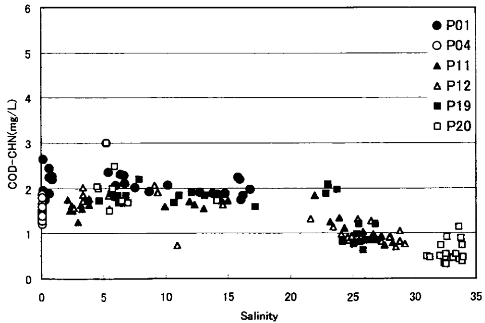
Figure 3.2.119 Scatter Chart of Salinity - COD_{CHN} (Continuous Survey, Neap Tide, Rainy Season)
