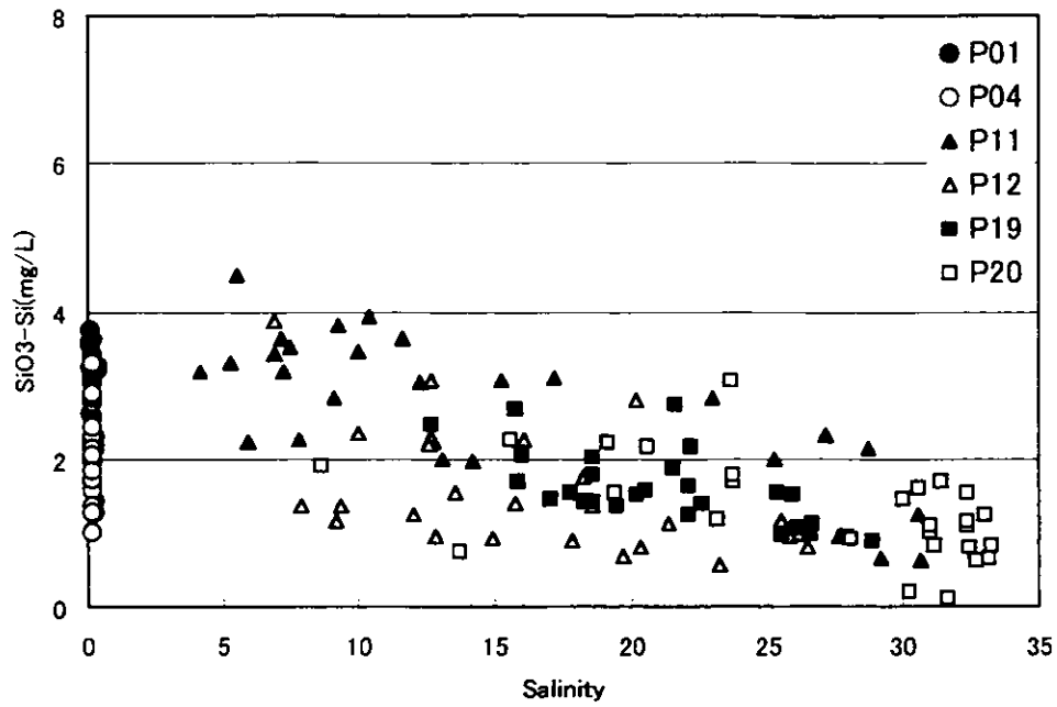
Figure 3.2.122 Scatter Chart of Salinity - \text{SiO}_3\text{-Si} (Continuous Survey, Spring Tide, Rainy Season)
