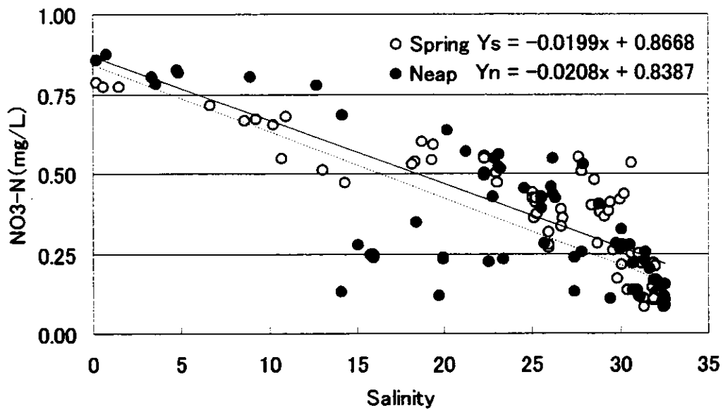
Figure 3.2.101 Scatter Chart of Salinity - NO 3 -N (Intensive Survey, Dry Season)
