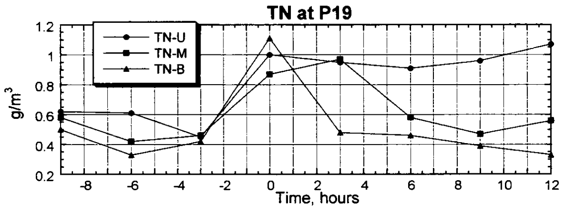
Figure 3.2.142(3) Result of the Survey on Water Quality (P19, Neap Tide, Dry Season)
