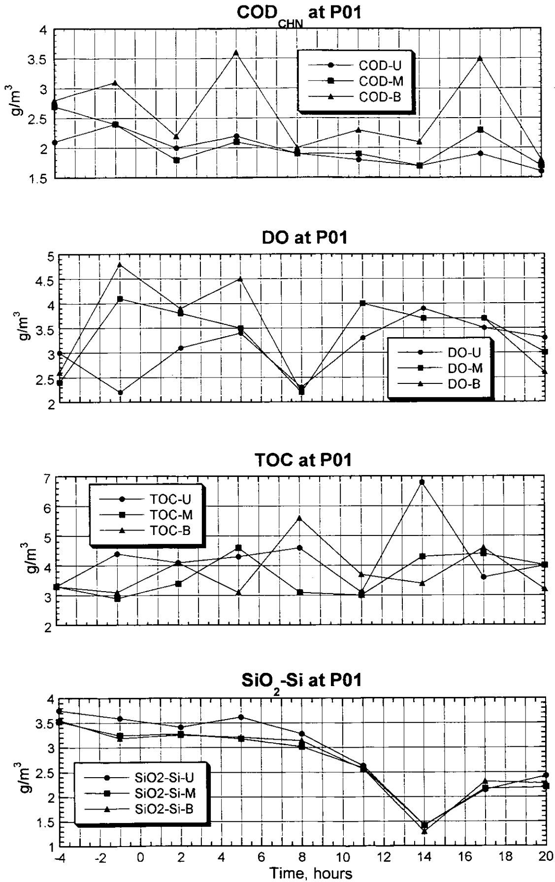
Figure 3.2.106(1) Result of the Survey on Water Quality (P01, Spring Tide, Rainy Season)
