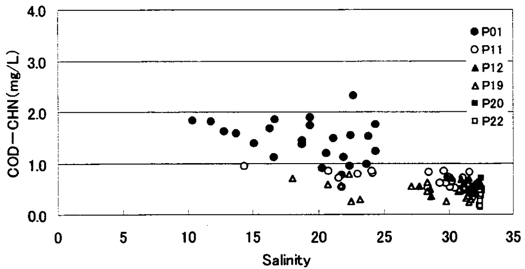
Figure 3.2.146 Scatter Chart of Salinity - COD CHN (Continuous Survey, Neap Tide, Dry Season)
