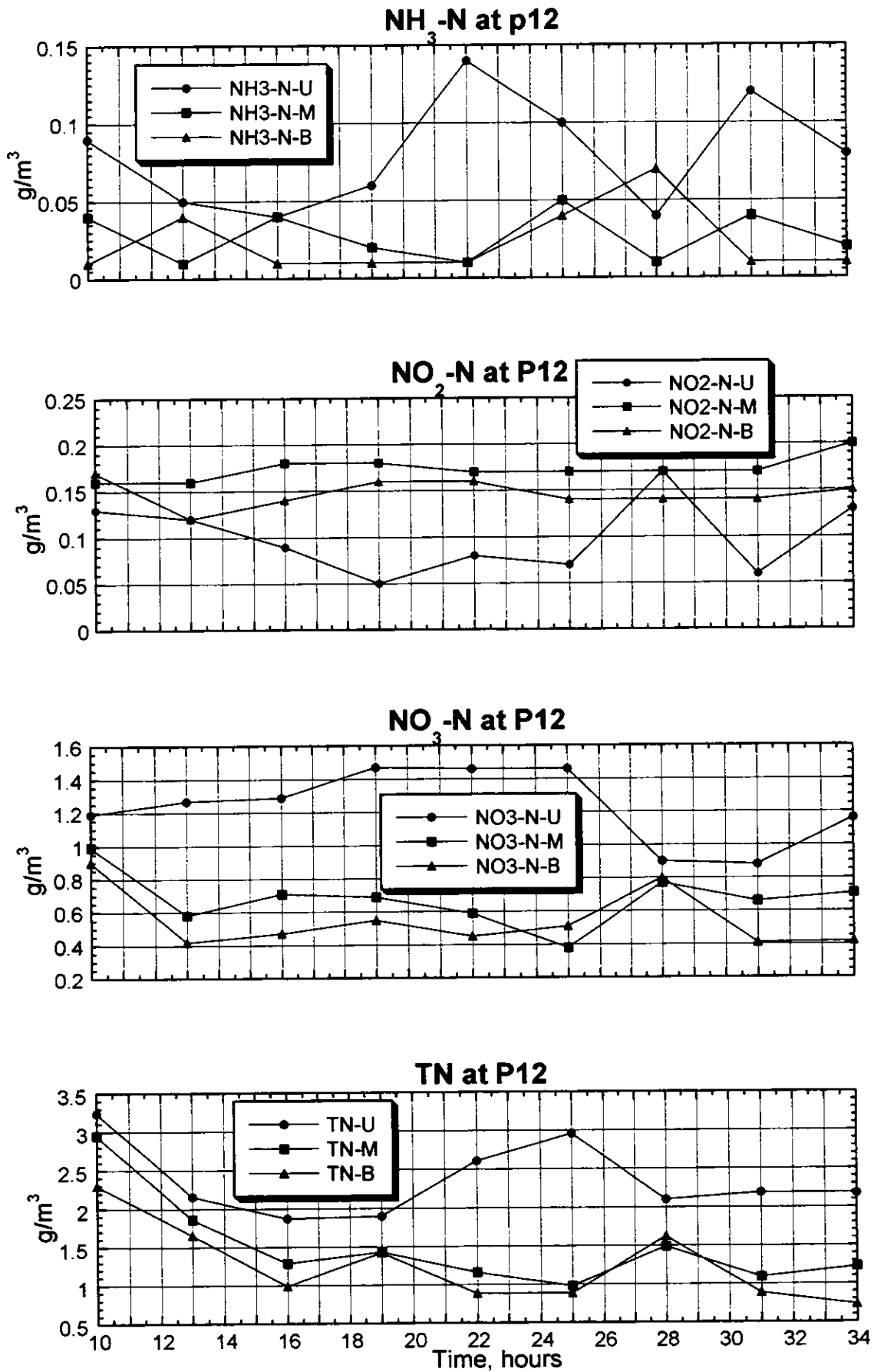
Figure 3.2.115(3) Result of the Survey on Water Quality (P12, Neap Tide, Rainy Season)
