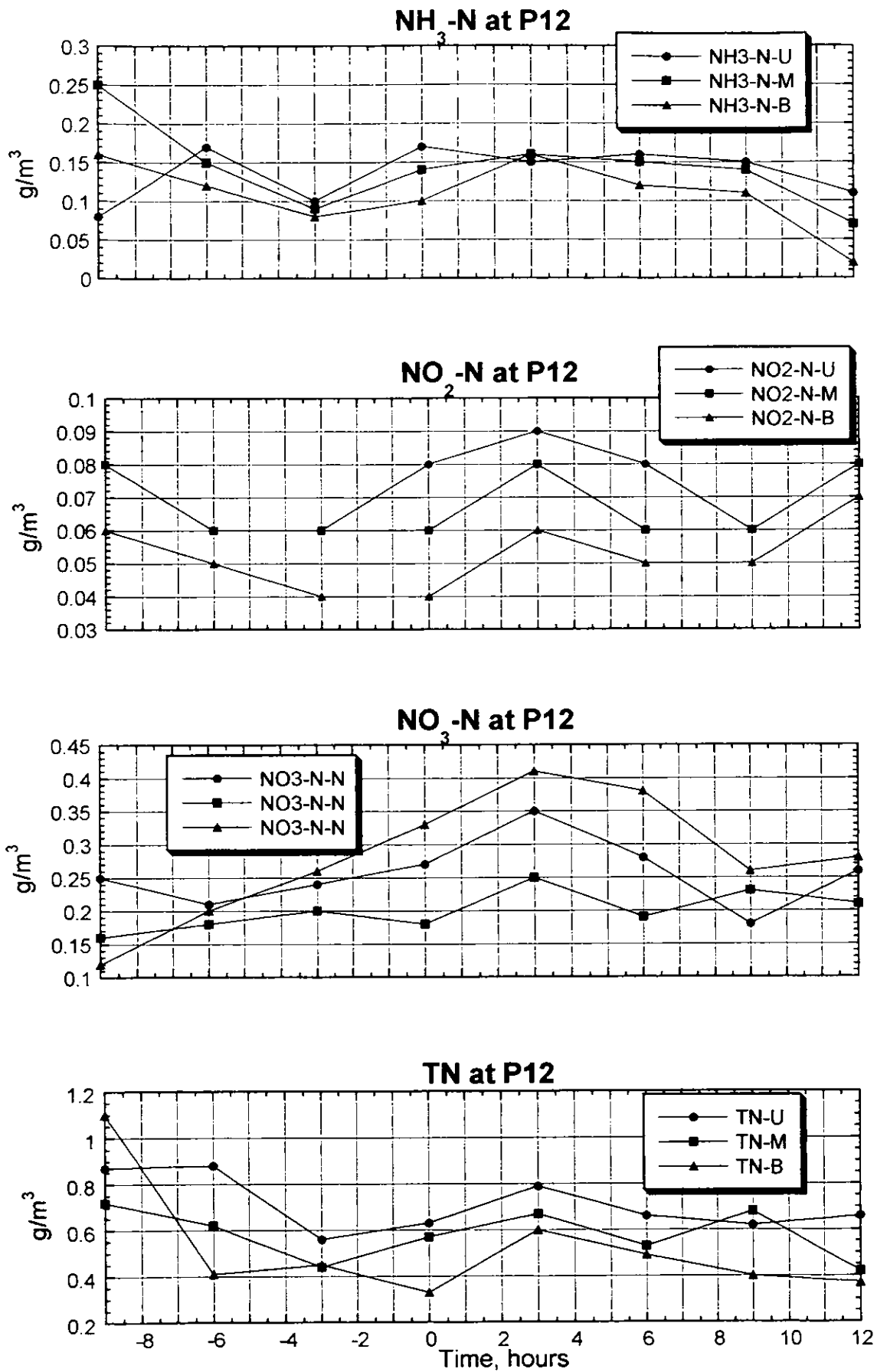
Figure 3.2.141(3) Result of the Survey on Water Quality (P12, Neap Tide, Dry Season)
