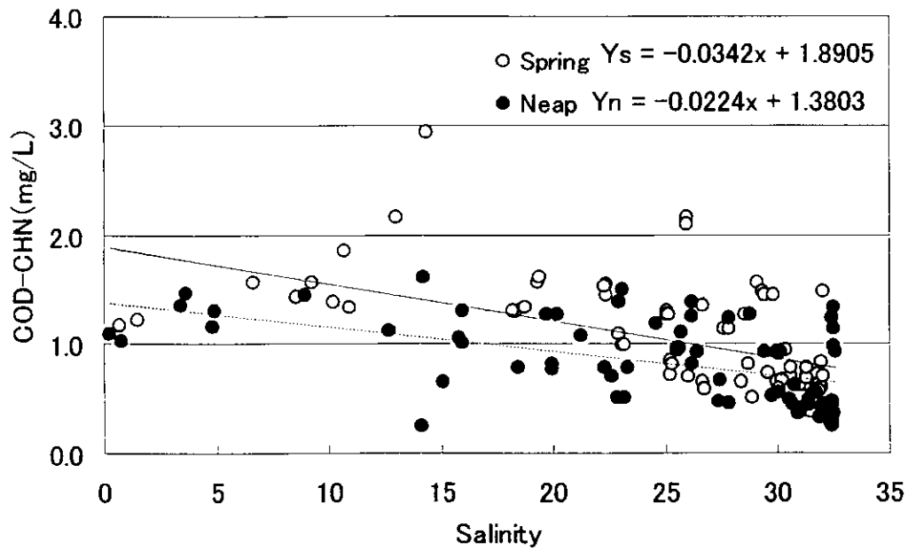
Figure 3.2.97 Scatter Chart of Salinity - COD CHN (Intensive Survey, Dry Season)
