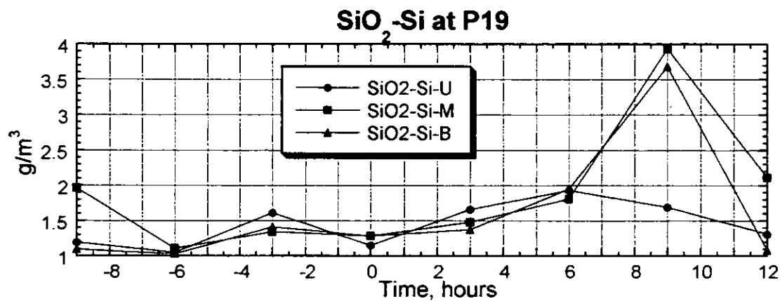
Figure 3.2.136(1) Result of the Survey on Water Quality (P19, Spring Tide, Dry Season)
