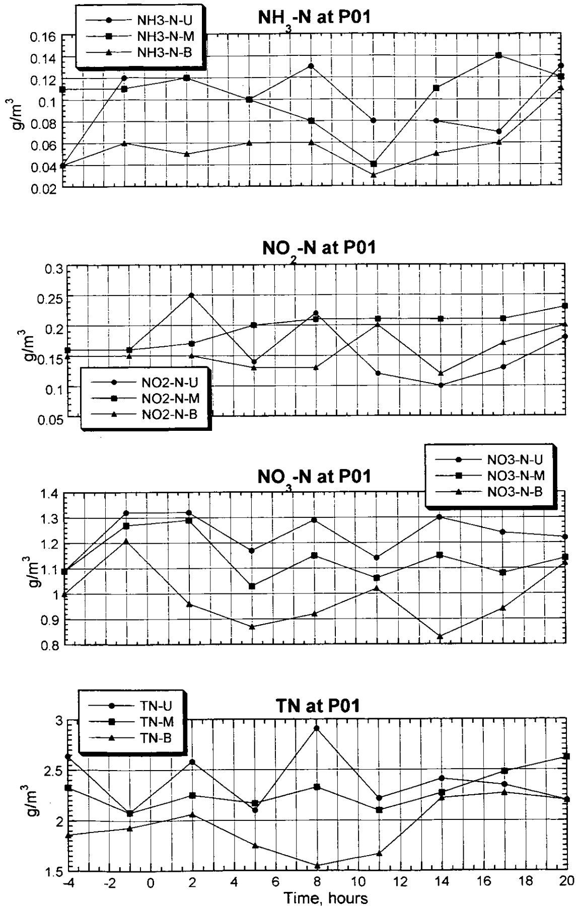
Figure 3.2.112(3) Result of the Survey on Water Quality (P01, Neap Tide, Rainy Season)
