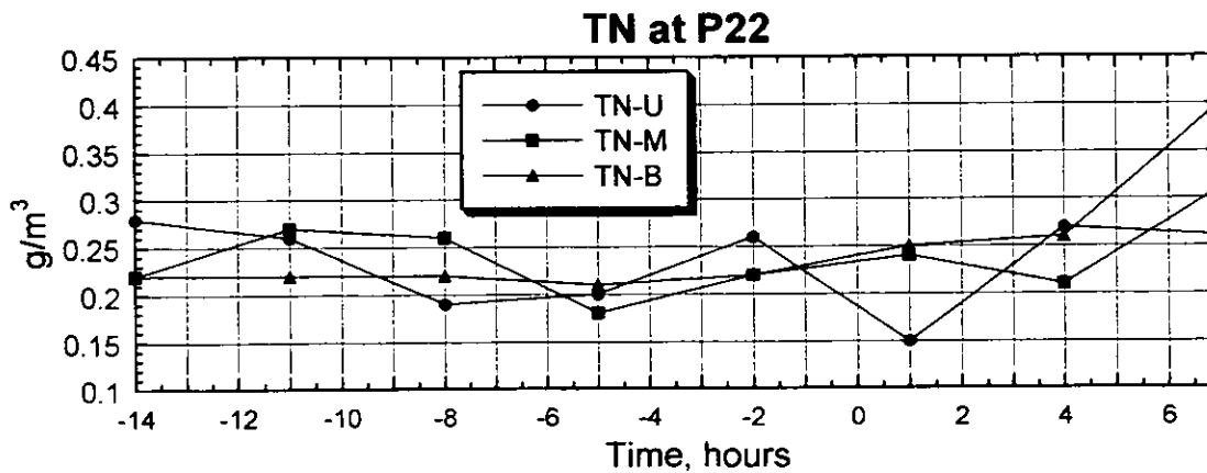
Figure 3.2.138(2) Result of the Survey on Water Quality (P22, Spring Tide, Dry Season)
