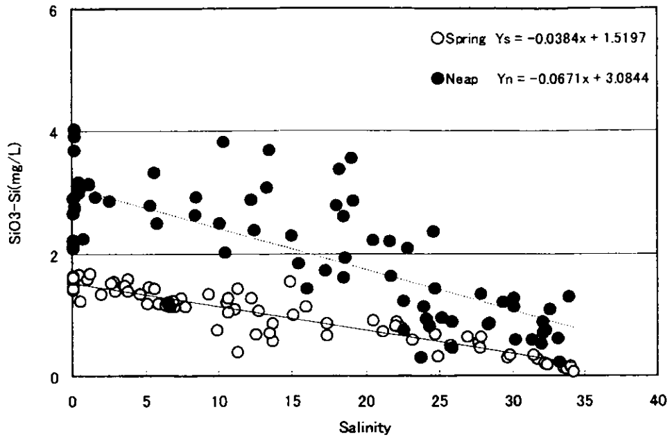
Figure 3.2.102 Scatter Chart of Salinity - SiO 3 -Si (Intensive Survey, Rainy Season)
