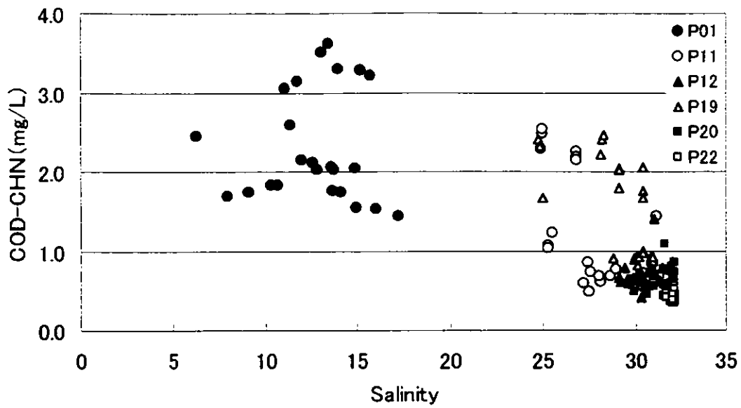
Figure 3.2.145 Scatter Chart of Salinity - COD CHN (Continuous Survey, Spring Tide, Dry Season)
