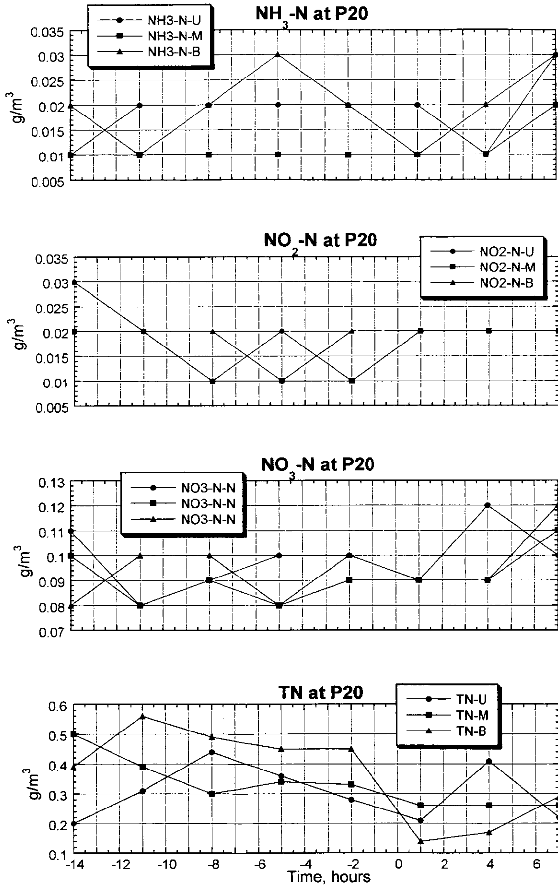
Figure 3.2.143(3) Result of the Survey on Water Quality (P20, Neap Tide, Dry Season)
