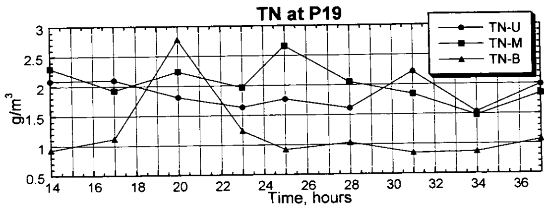
Figure 3.2.116(3) Result of the Survey on Water Quality (P19, Neap Tide, Rainy Season)
