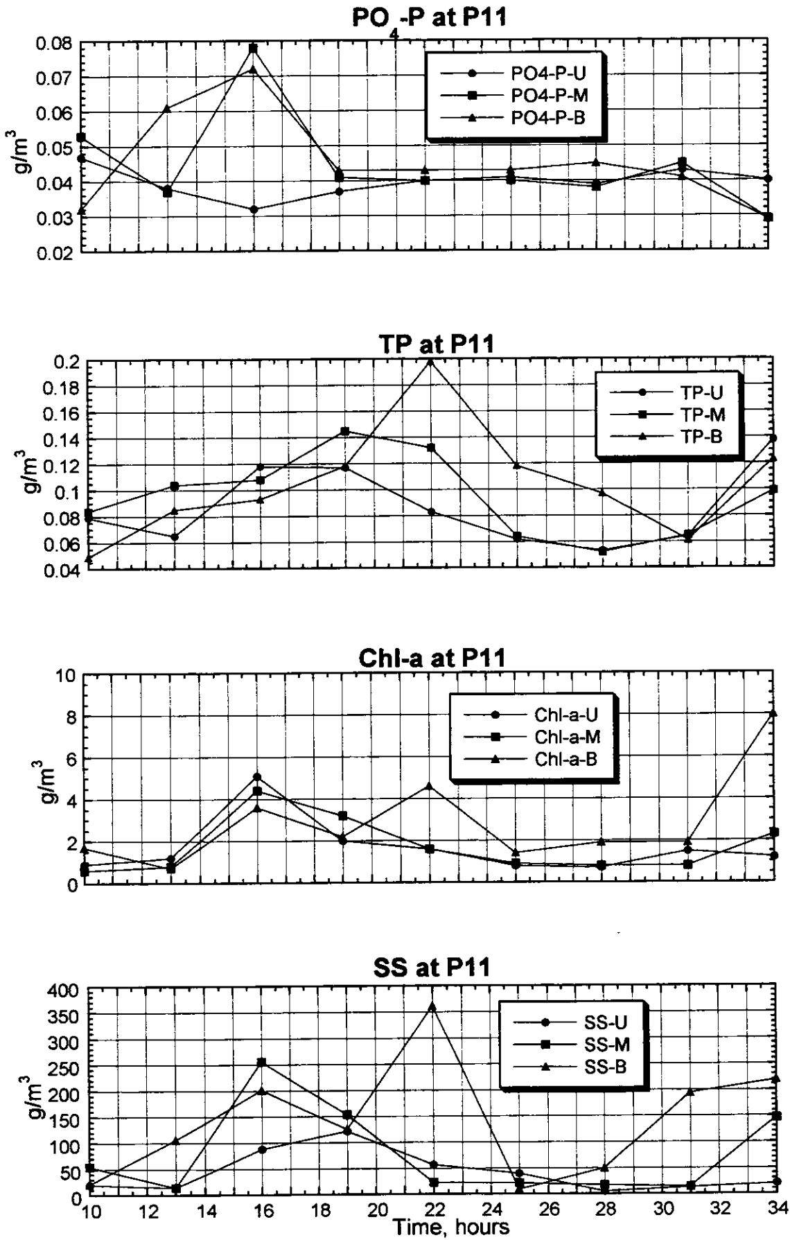
Figure 3.2.108(2) Result of the Survey on Water Quality (P11, Spring Tide, Rainy Season)
