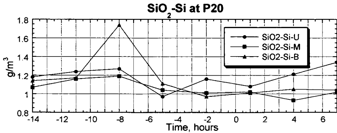
Figure 3.2.137(1) Result of the Survey on Water Quality (P20, Spring Tide, Dry Season)
