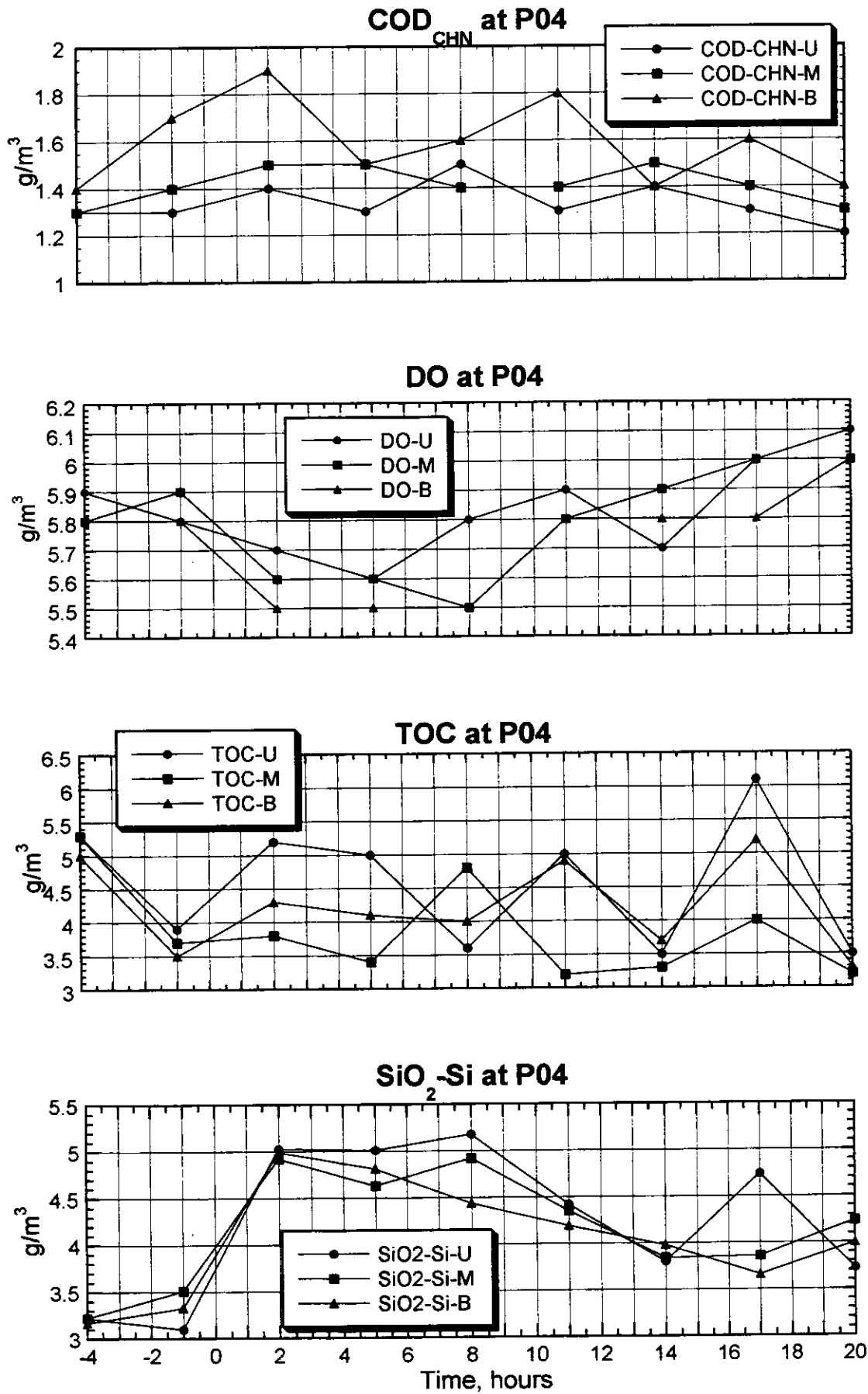
Figure 3.2.113(1) Result of the Survey on Water Quality (P04, Neap Tide, Rainy Season)
