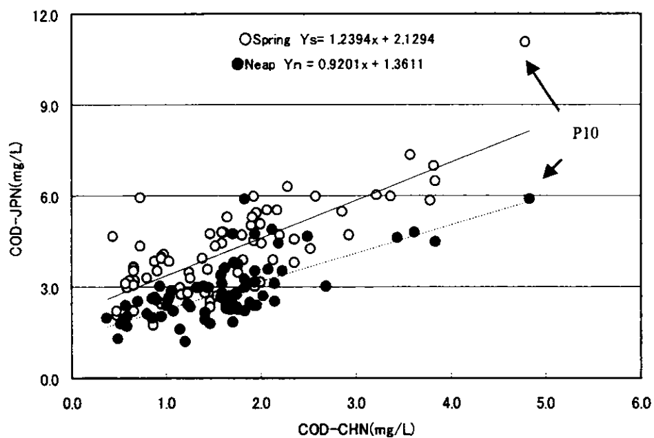
Figure 3.2.105 Scatter Chart of COD_{CHN} - COD_{JPN} (Intensive Survey, Rainy Season)
