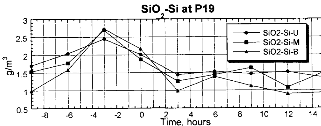
Figure 3.2.110(1) Result of the Survey on Water Quality (P19, Spring Tide, Rainy Season)
