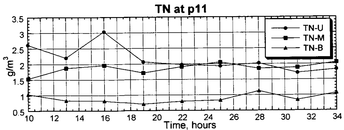
Figure 3.2.114(3) Result of the Survey on Water Quality (P11, Neap Tide, Rainy Season)
