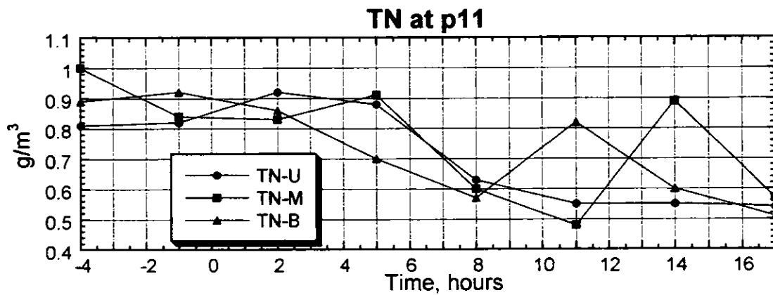
Figure 3.2.134(3) Result of the Survey on Water Quality (P11, Spring Tide, Dry Season)
