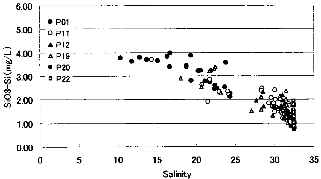
Figure 3.2.150 Scatter Chart of Salinity : SiO 3 -Si (Continuous Survey, Neap Tide, Dry Season)
