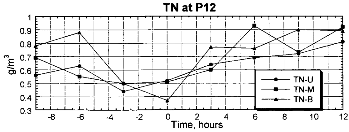
Figure 3.2.135(3) Result of the Survey on Water Quality (P12, Spring Tide, Dry Season)
