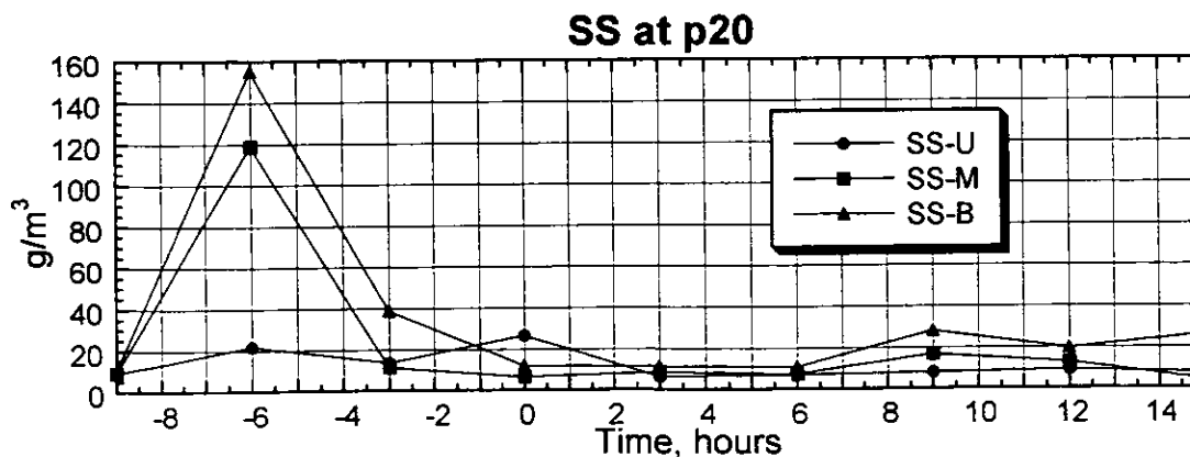
Figure 3.2.111(2) Result of the Survey on Water Quality (P20, Spring Tide, Rainy Season)
