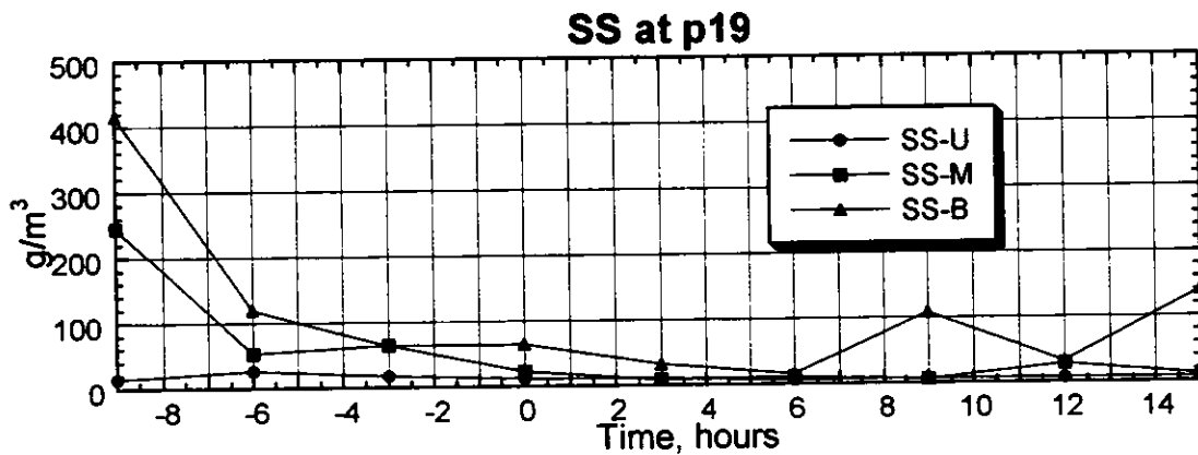
Figure 3.2.110(2) Result of the Survey on Water Quality (P19, Spring Tide, Rainy Season)
