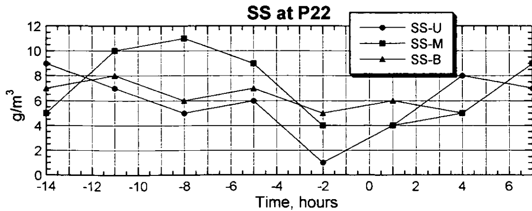
Figure 3.2.144(2) Result of the Survey on Water Quality (P22, Neap Tide, Dry Season)
