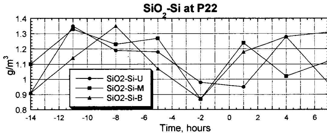
Figure 3.2.138(1) Result of the Survey on Water Quality (P22, Spring Tide, Dry Season)
