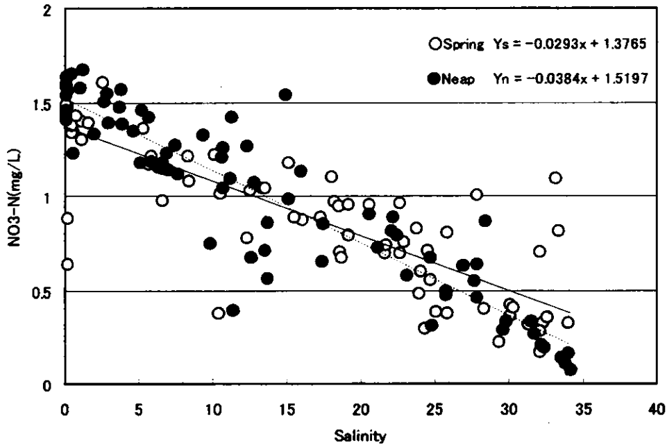
Figure 3.2.100 Scatter Chart of Salinity - NO 3 -N (Intensive Survey, Rainy Season)
