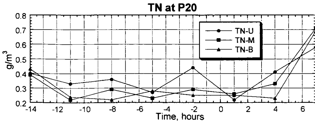
Figure 3.2.137(3) Result of the Survey on Water Quality (P20, Spring Tide, Dry Season)
