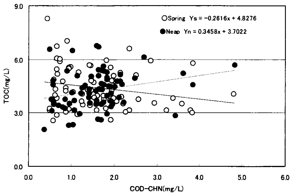
Figure 3.2.104 Scatter Chart of COD_{CHN} - TOC (Intensive Survey, Rainy Season)
