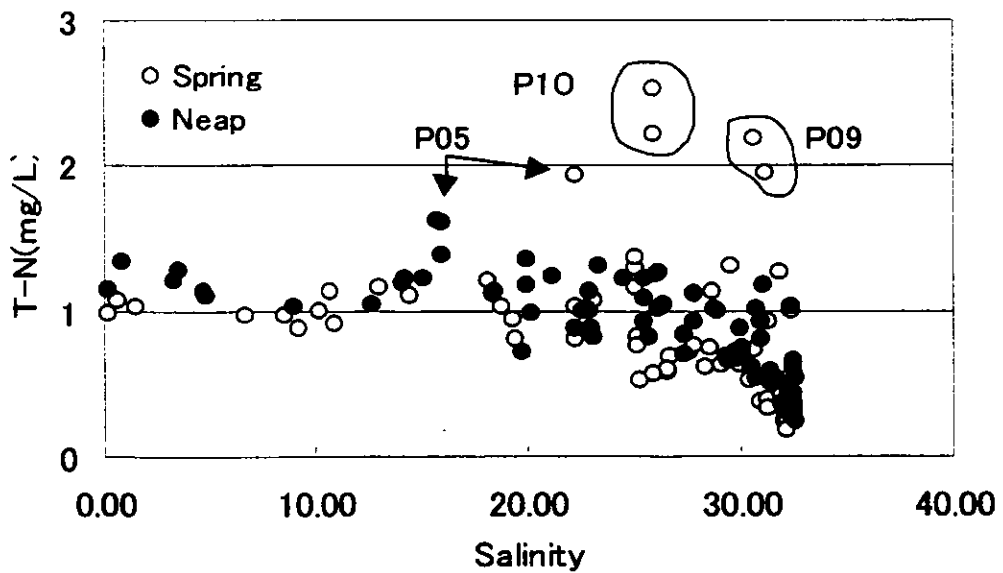
Figure 3.2.99 Scatter Chart of Salinity - TN (Intensive Survey, Dry Season)
