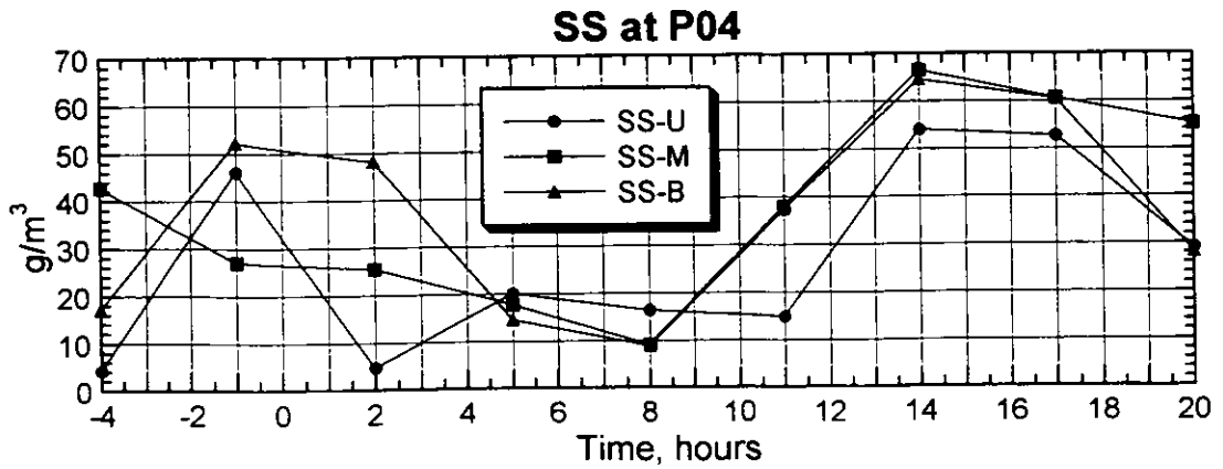
Figure 3.2.113(2) Result of the Survey on Water Quality (P04, Neap Tide, Rainy Season)
