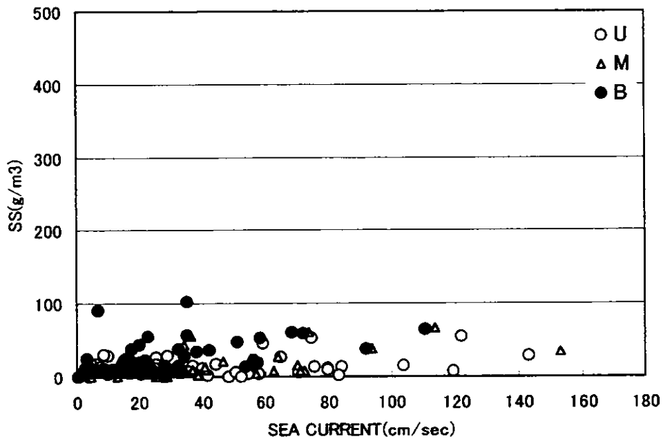
Figure 3.2.125 Scatter Chart of Sea Current - SS (Continuous Survey, Neap Tide, Rainy Season)
