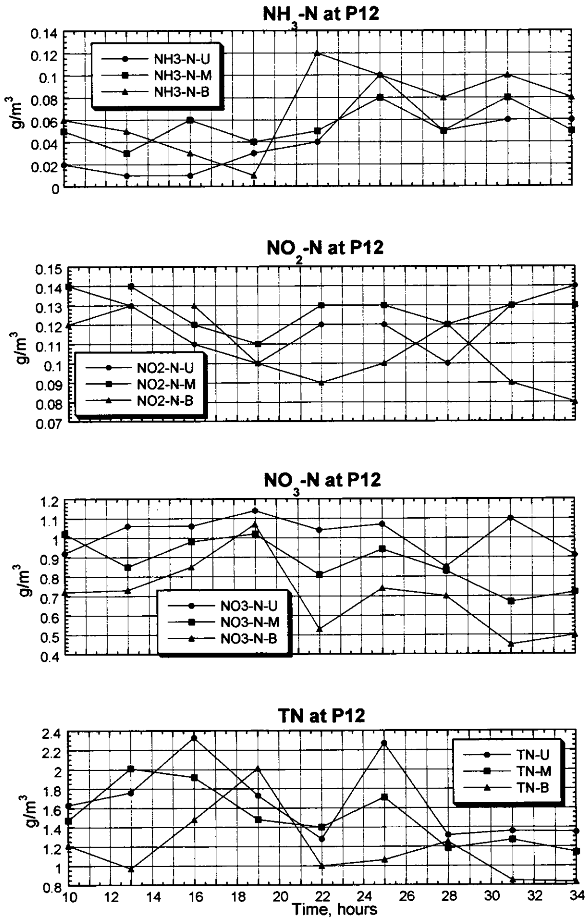
Figure 3.2.109(3) Result of the Survey on Water Quality (P12, Spring Tide, Rainy Season)
