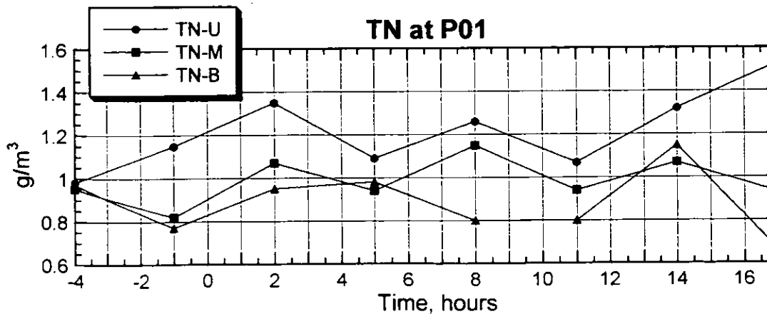
Figure 3.2.139(3) Result of the Survey on Water Quality (P01, Neap Tide, Dry Season)
