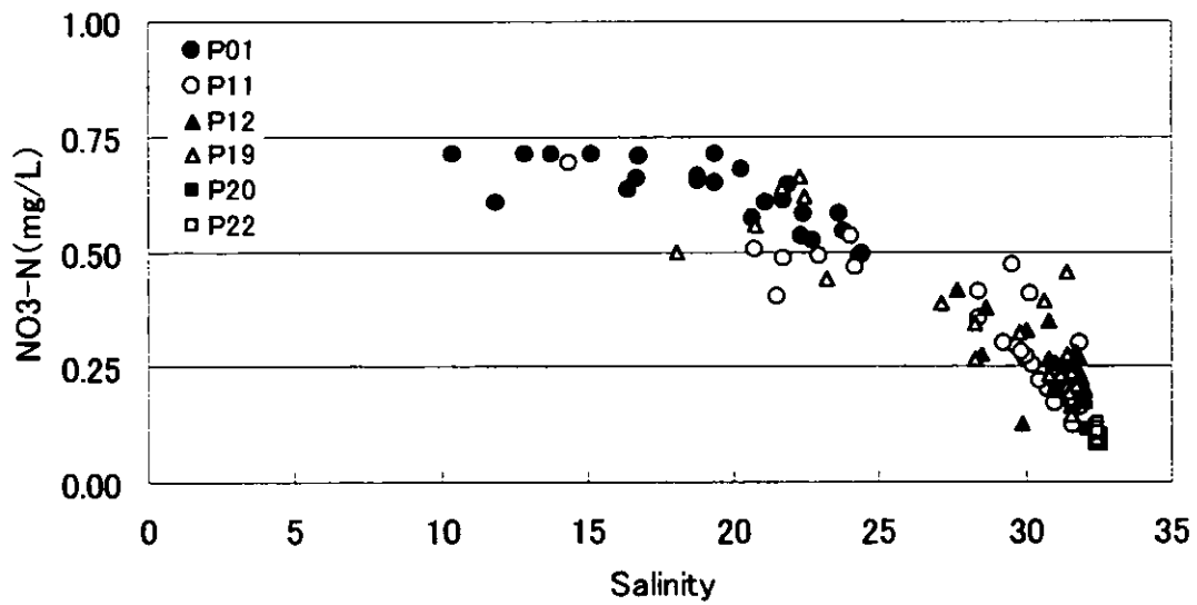
Figure 3.2.148 Scatter Chart of Salinity - NO 3 -N (Continuous Survey, Neap Tide, Dry Season)
