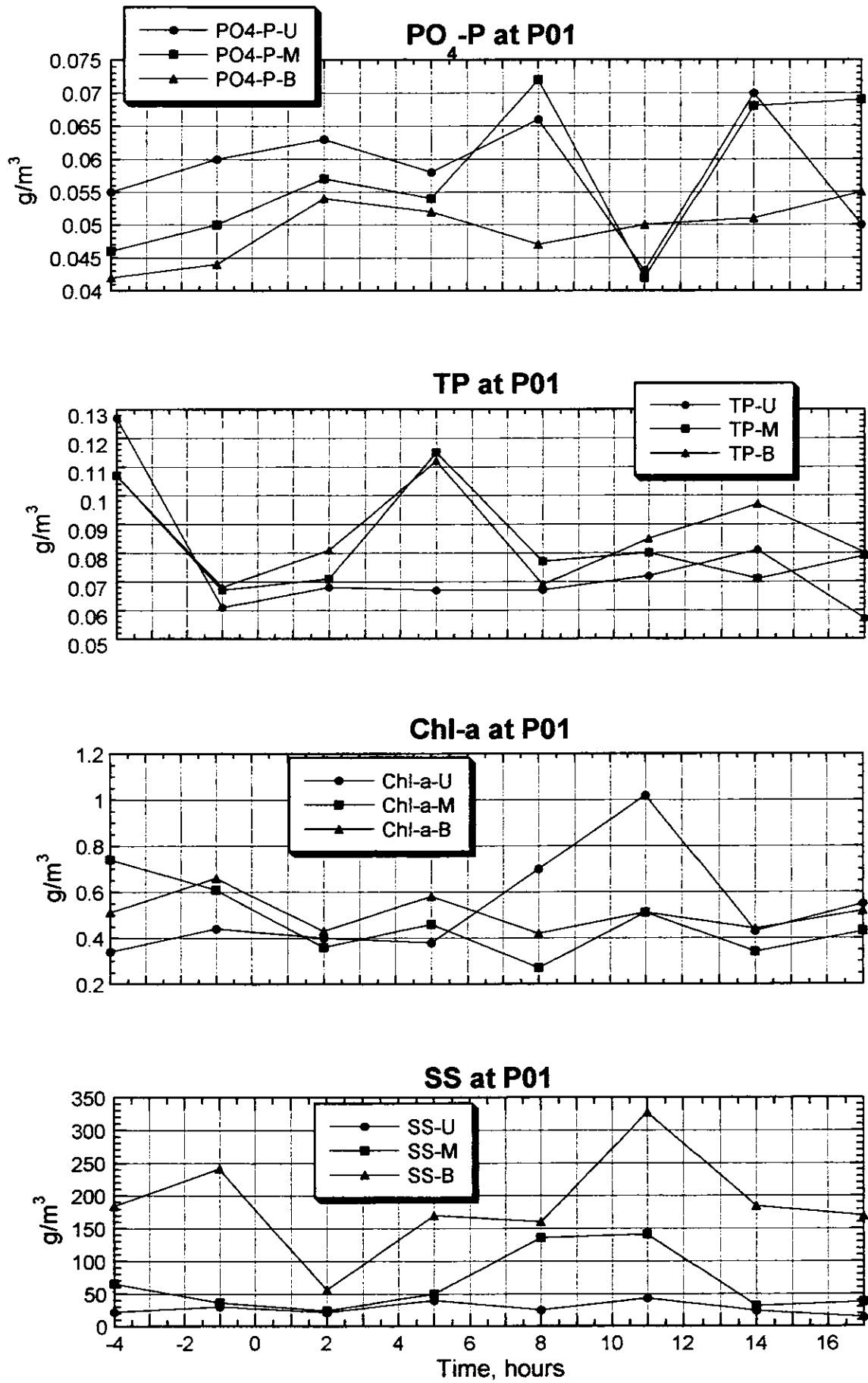
Figure 3.2.133(2) Result of the Survey on Water Quality (P01, Spring Tide, Dry Season)
