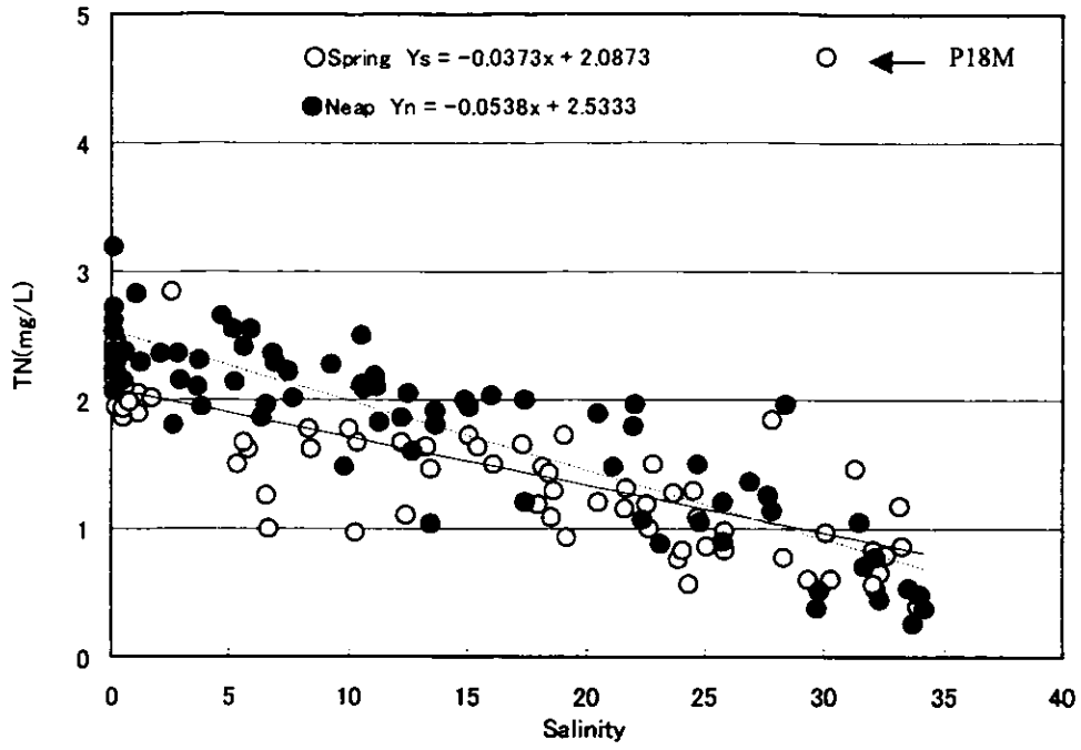
Figure 3.2.98 Scatter Chart of Salinity - TN (Intensive Survey, Rainy Season)
