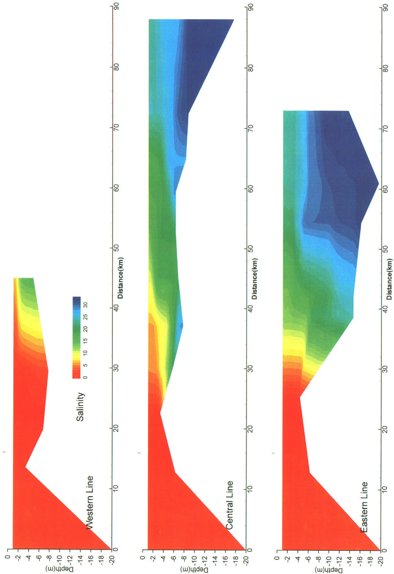
Figure 3.1.31 Vertical Distribution of Salinity (Spring Tide, Rainy Season, from 31 July to 4 Aug. 2000)
