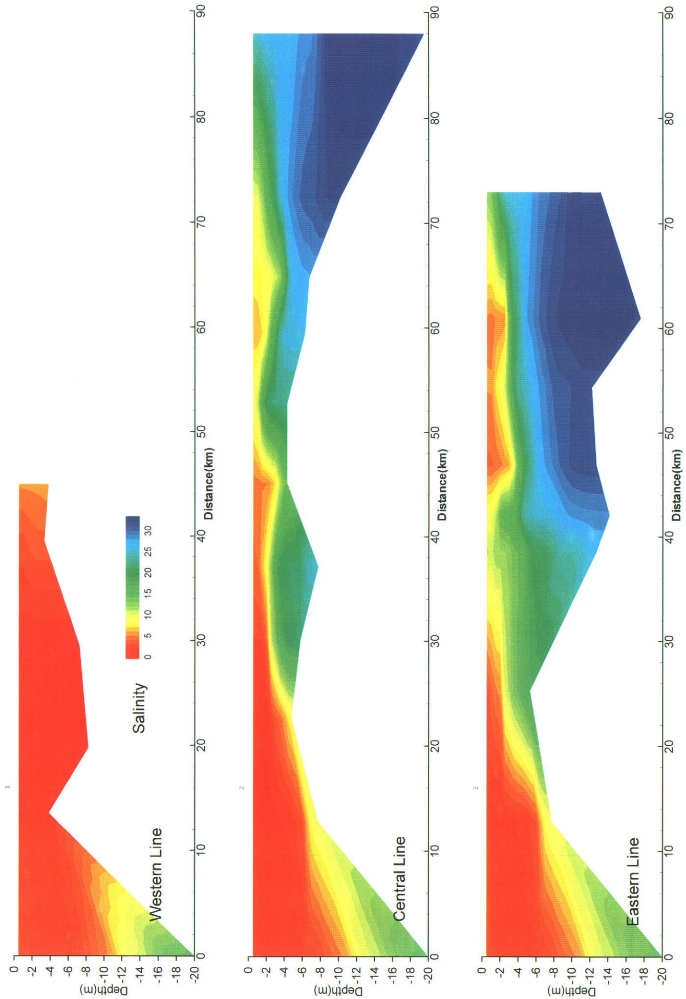
Figure 3.1.33 Vertical Distribution of Salinity (Neap Tide, Rainy Season, from 6 to 9 Aug. 2000)
