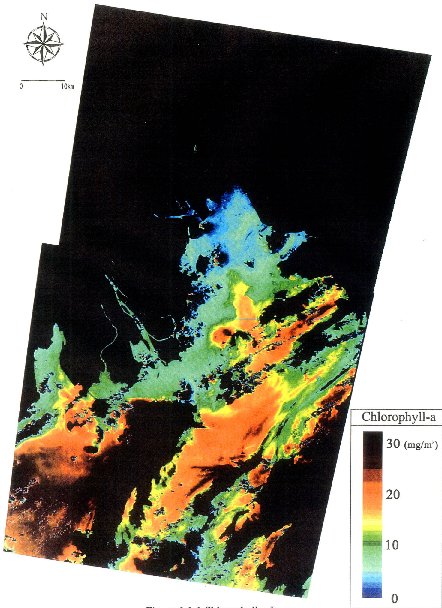
Figure 2.2.6 Chlorophyll-a Image (Date 2000/08/13)
