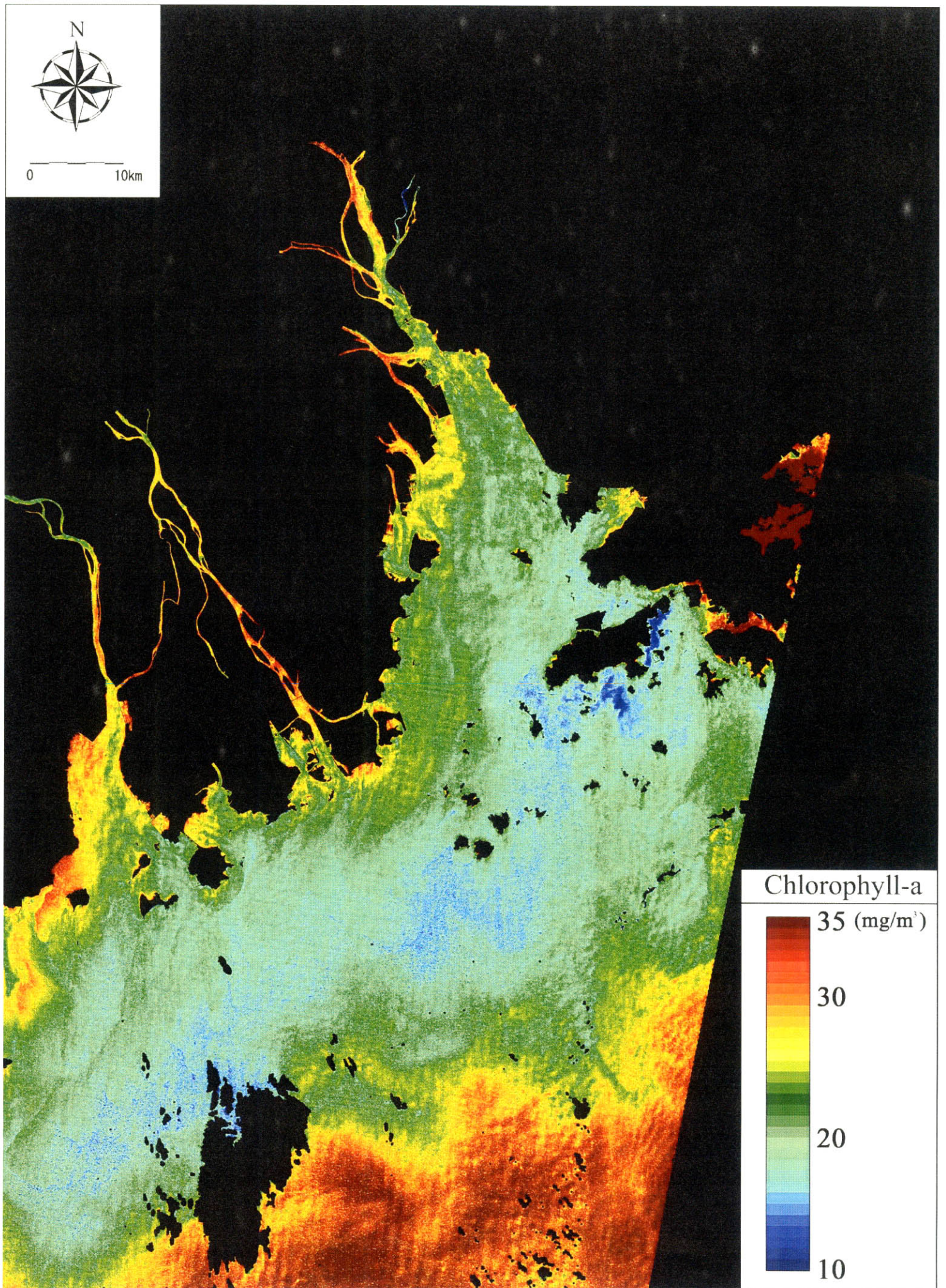
Figure 2.2.7 Chlorophyll-a Image (Date 2000/11/01)
