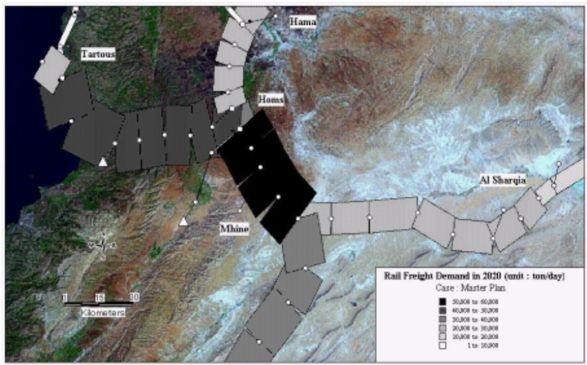
Figure 4.3 (2) Traffic Demand en Route in 2020 (Freight)
