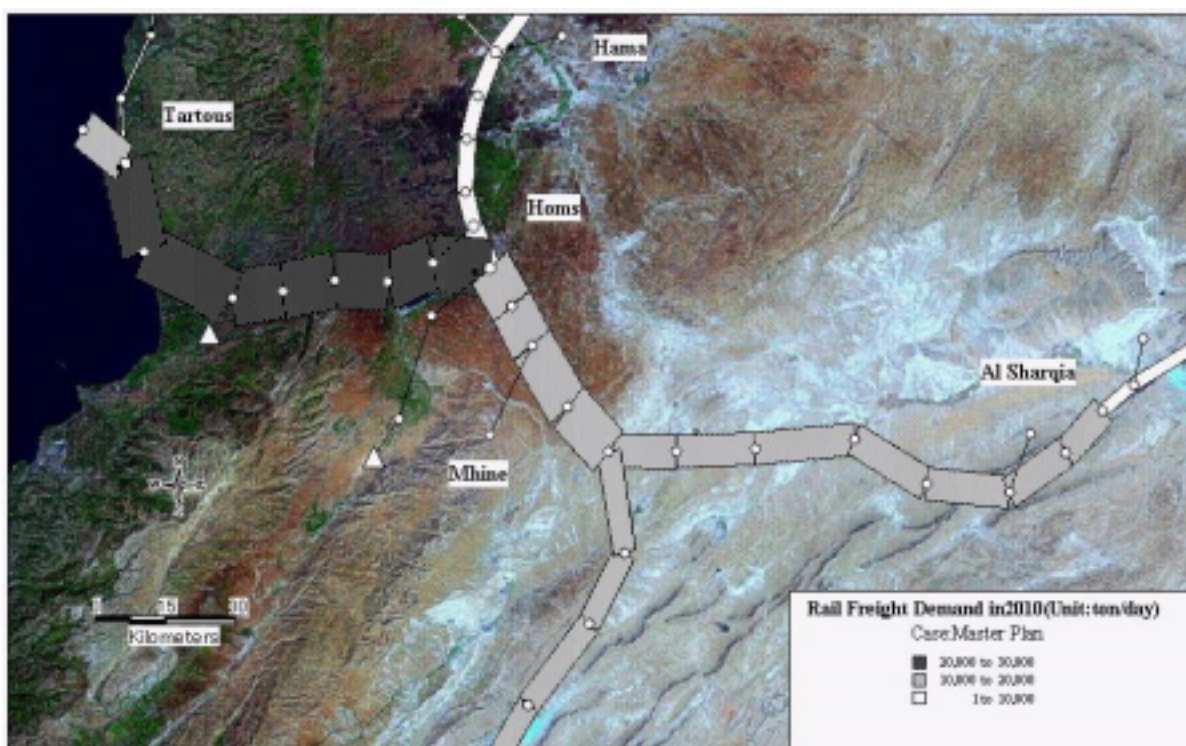
Figure 4.2(2) Traffic Demand en Route in 2010 (Freight)
