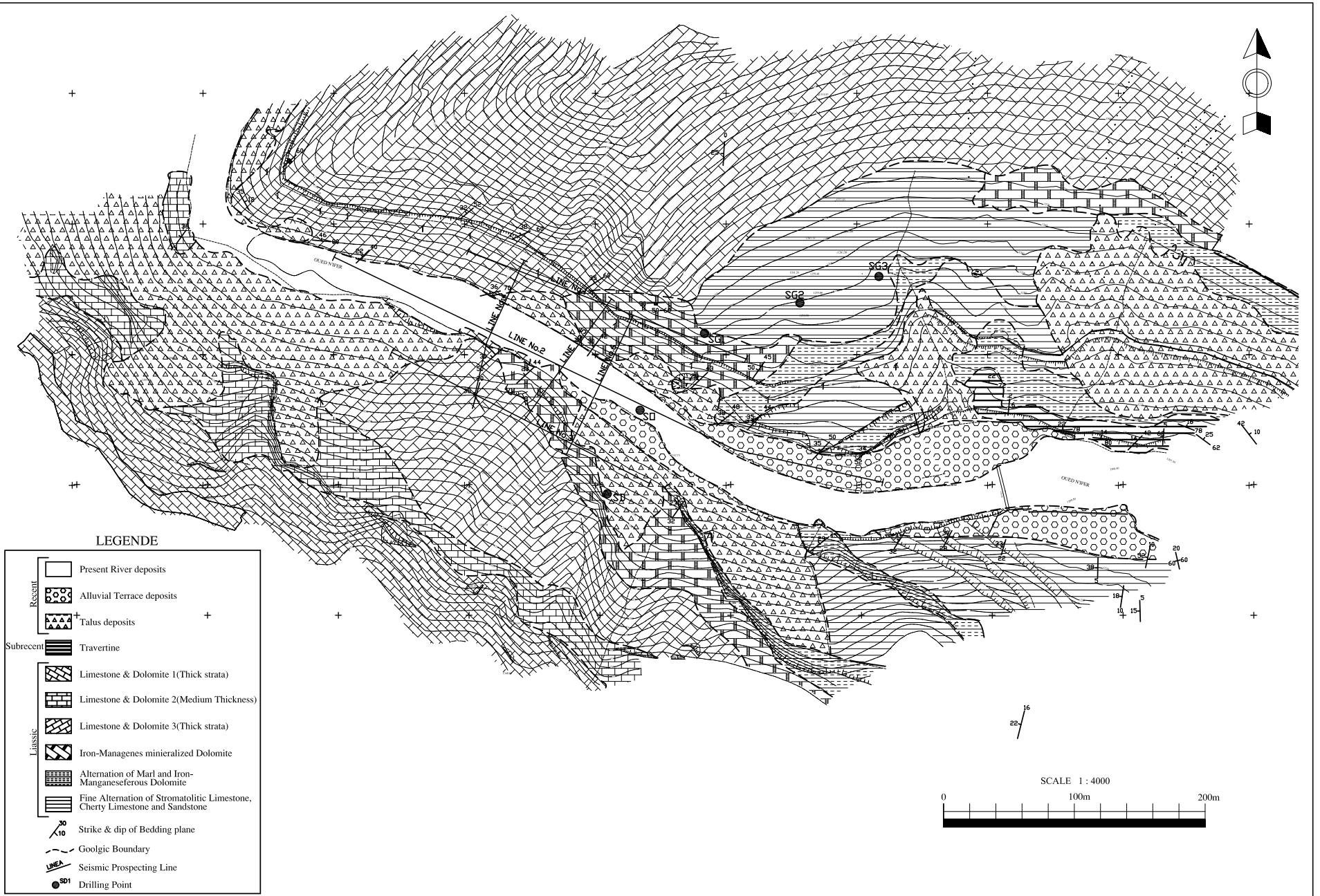
Figure GC1.3 Geological Map around Tinkit Dam Site & Location Map of Drilling and Seismic Prospecting
