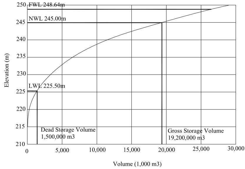
N'Fifikh Dam H-V Curve
