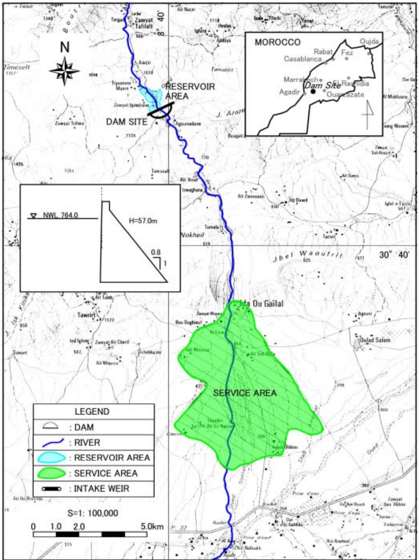
Figure VIII.1.23 General Plan of IGUI N'OUAQA (No.23)
