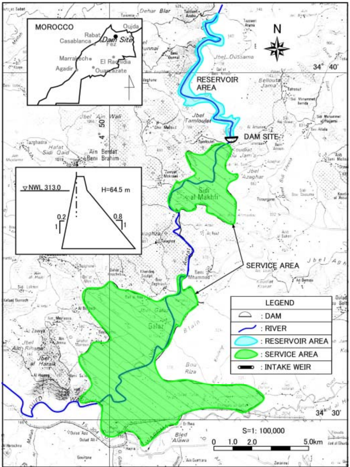
Figure VIII.1.21 General Plan of SIDI EL MOKHFI (No.21)
