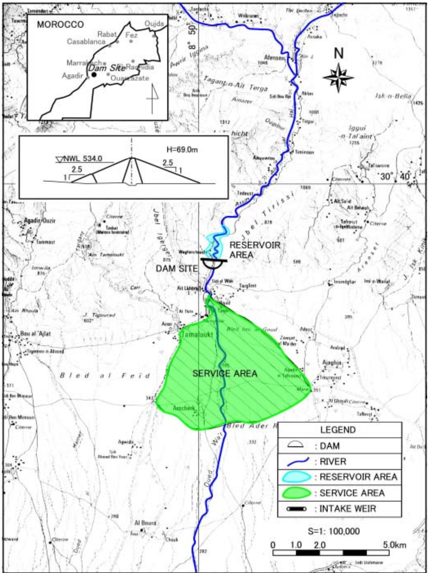
Figure VIII.1.25 General Plan of SIDI ABDELLAH (No.25)
