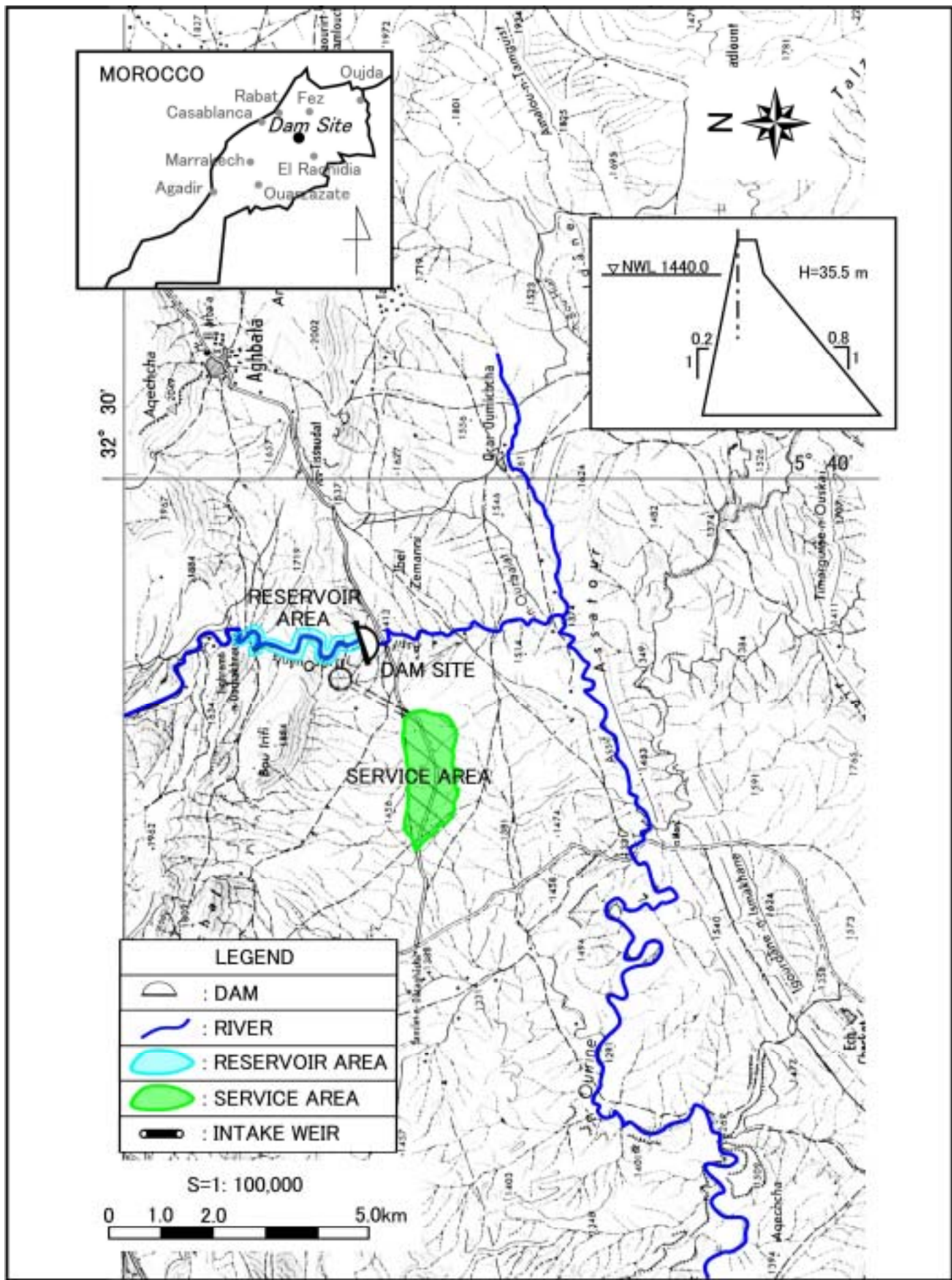
Figure VIII.1.22 General Plan of N'OUANTZ (No.22)
