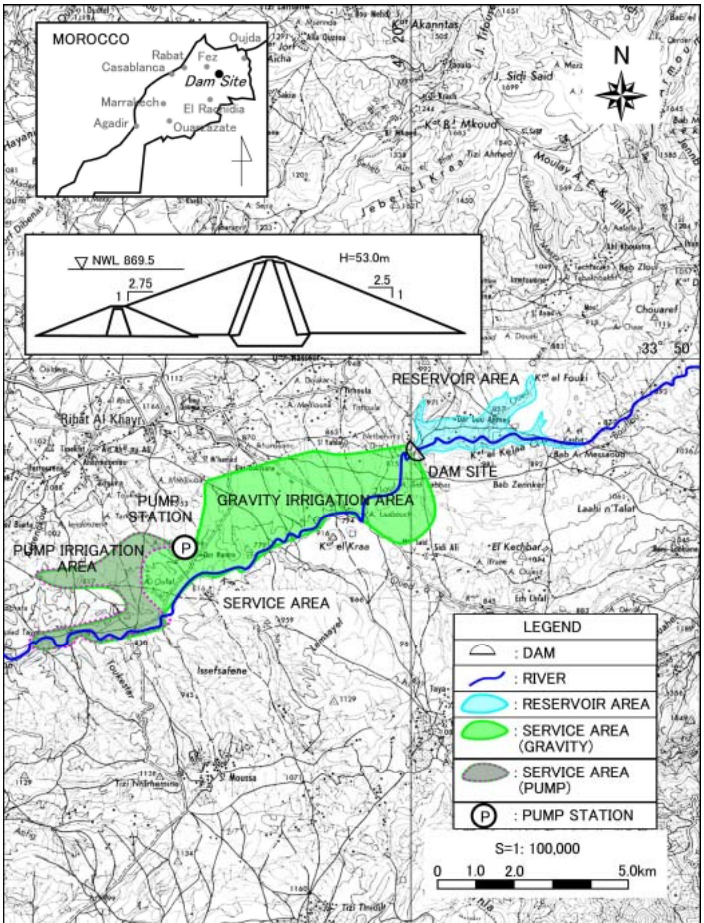
Figure VIII.1.17 General Plan of AZGHAR (No.17)
