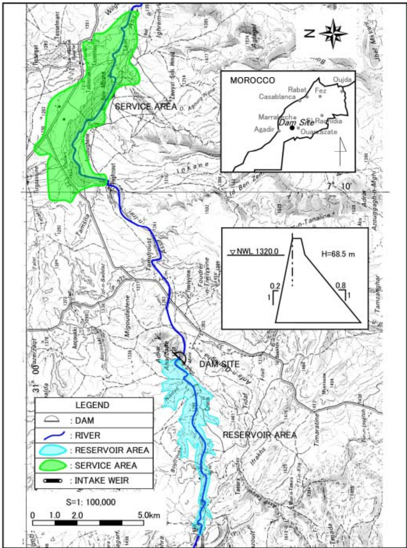
Figure VIII.1.16 General Plan of TIOUINE (No16)
