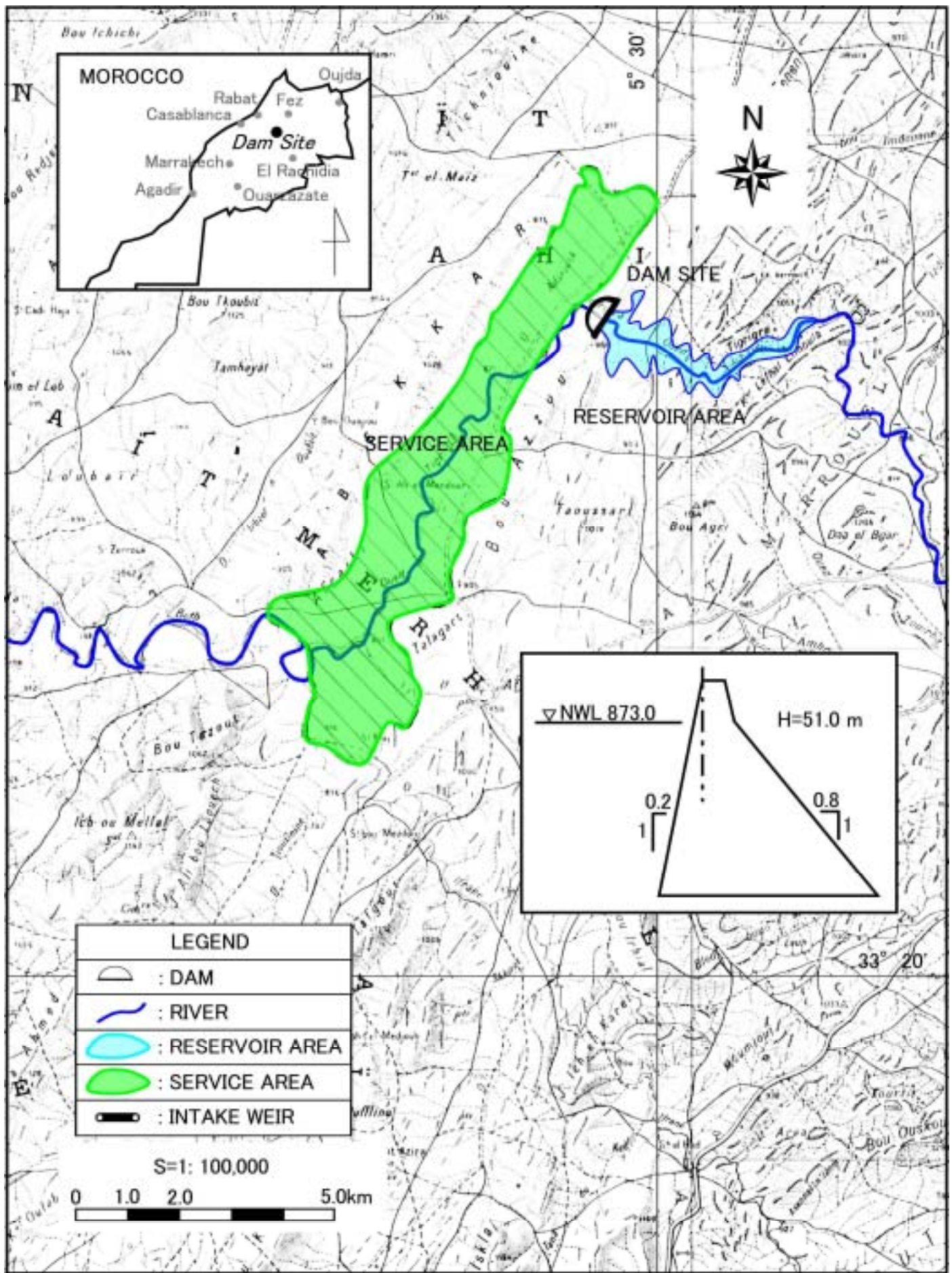
Figure VIII.1.14 General Plan of ADAROUCH (No.14)
