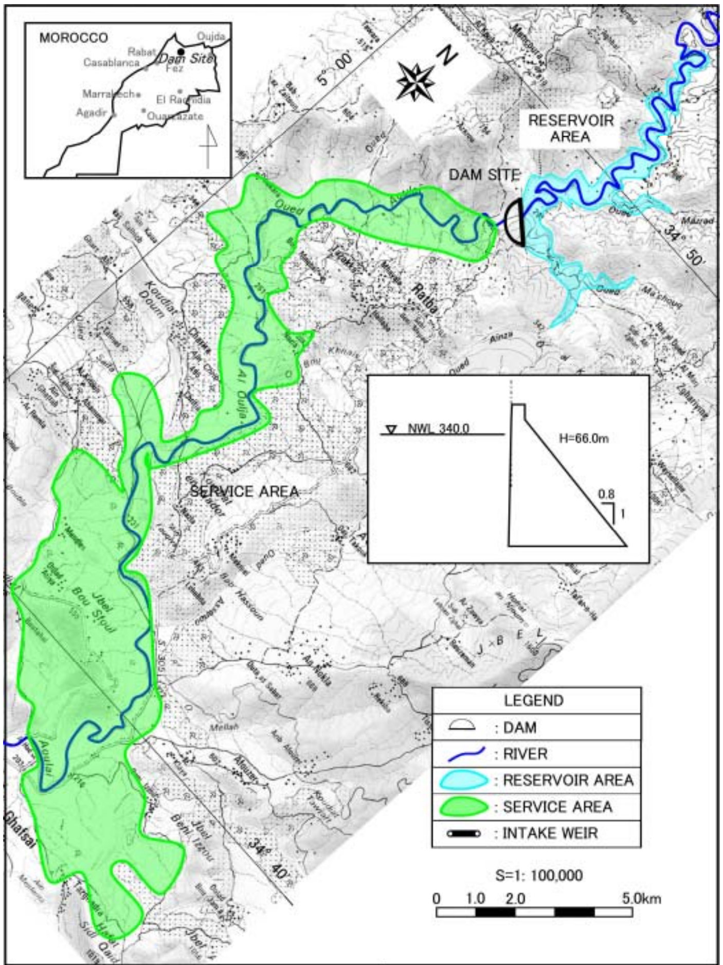
Figure VIII.1.19 General Plan of AOULAI (No.19)
