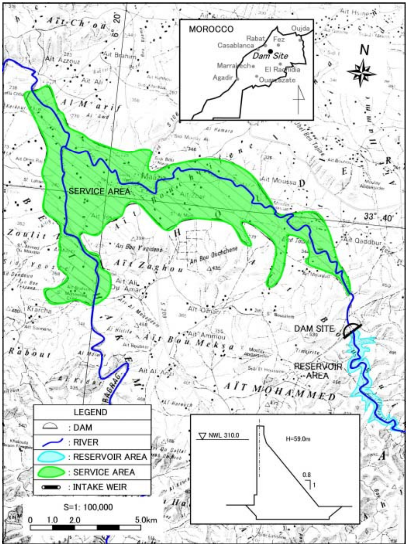
Figure VIII.1.15 General Plan of SIDI OMAR (No.15)
