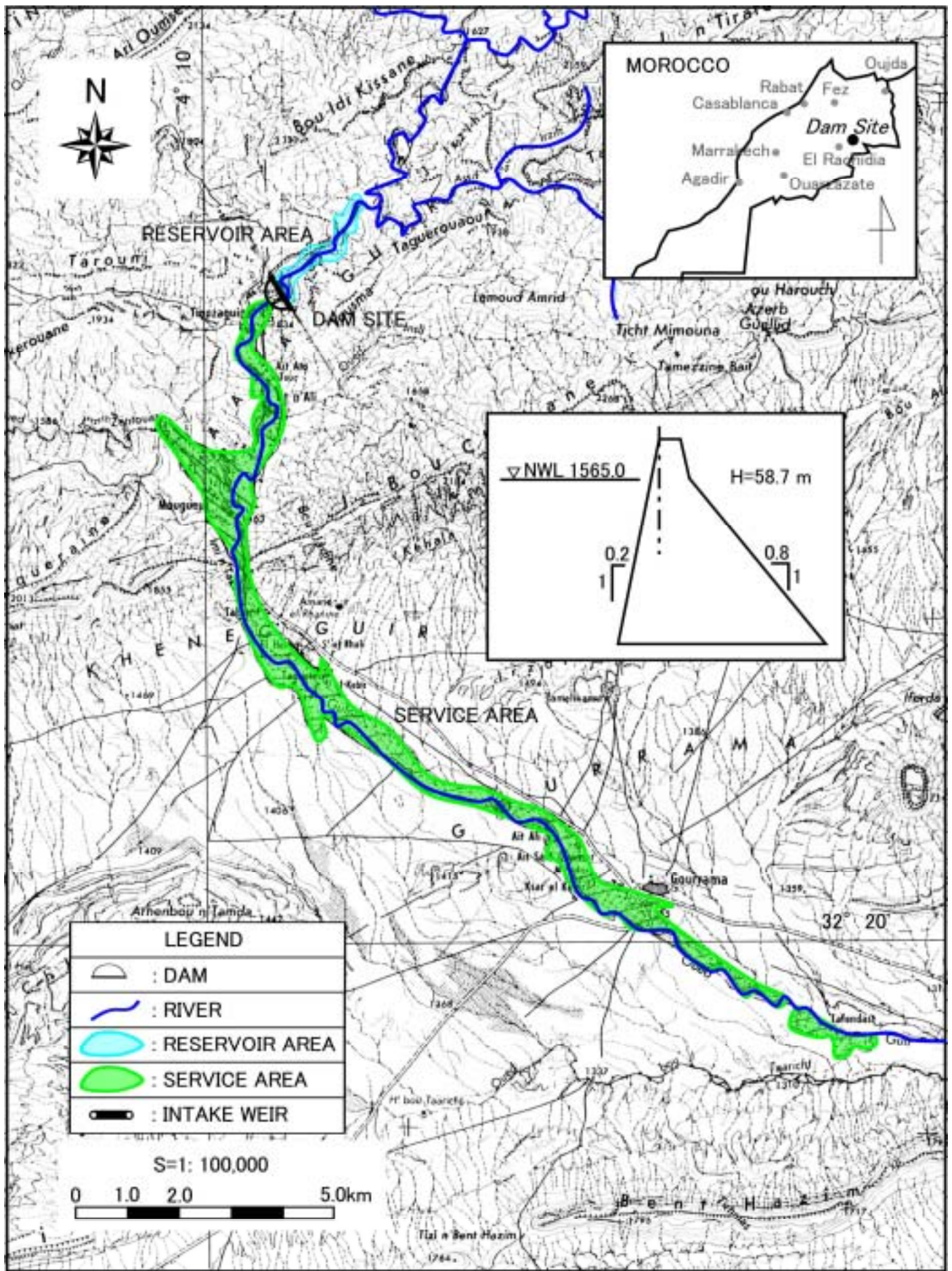
Figure VIII.1.12 General Plan of TIOUZAGUINE (No.12)
