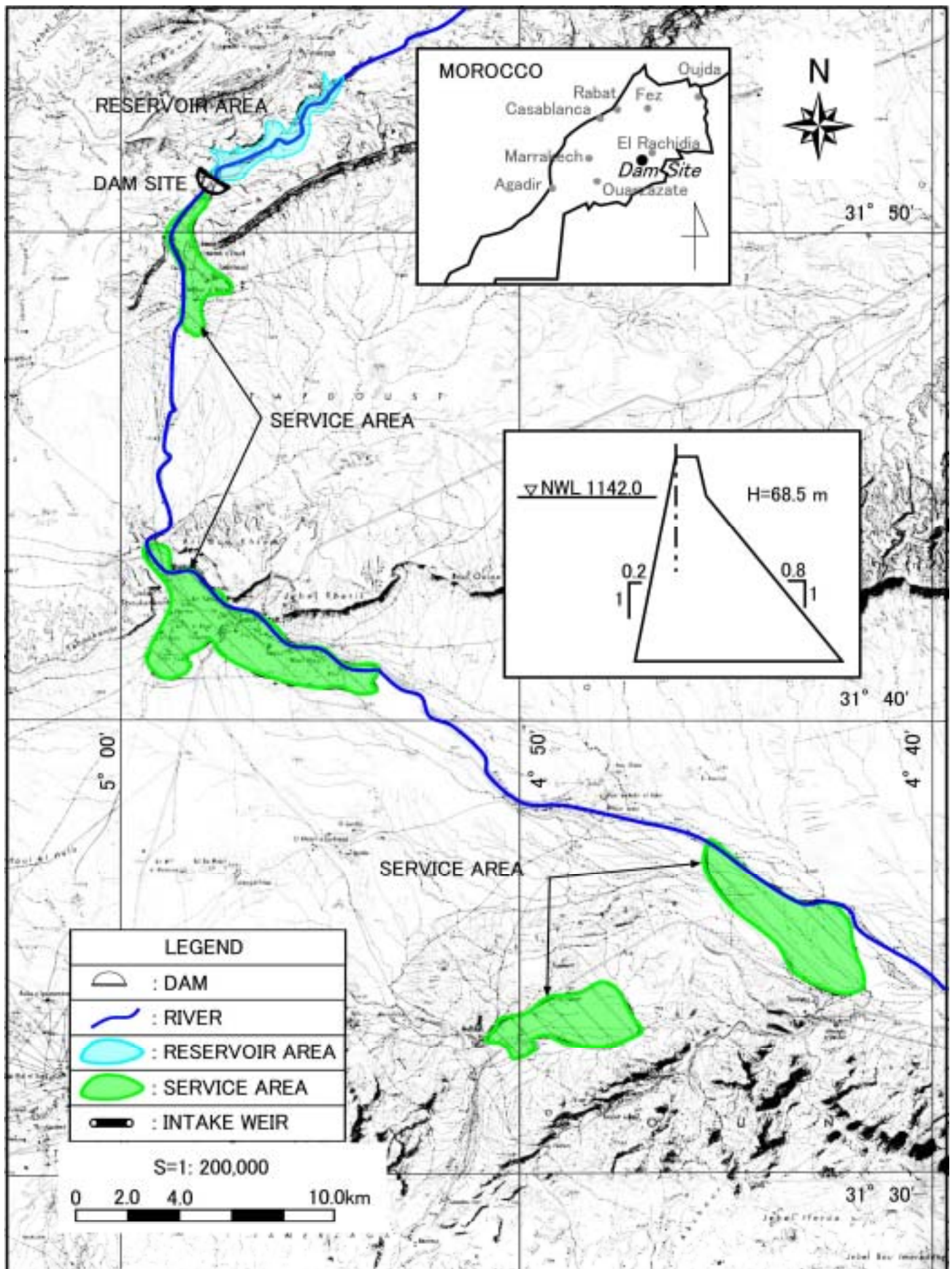
Figure VIII.1.11 General Plan of TADIGHOUST (No.11)
