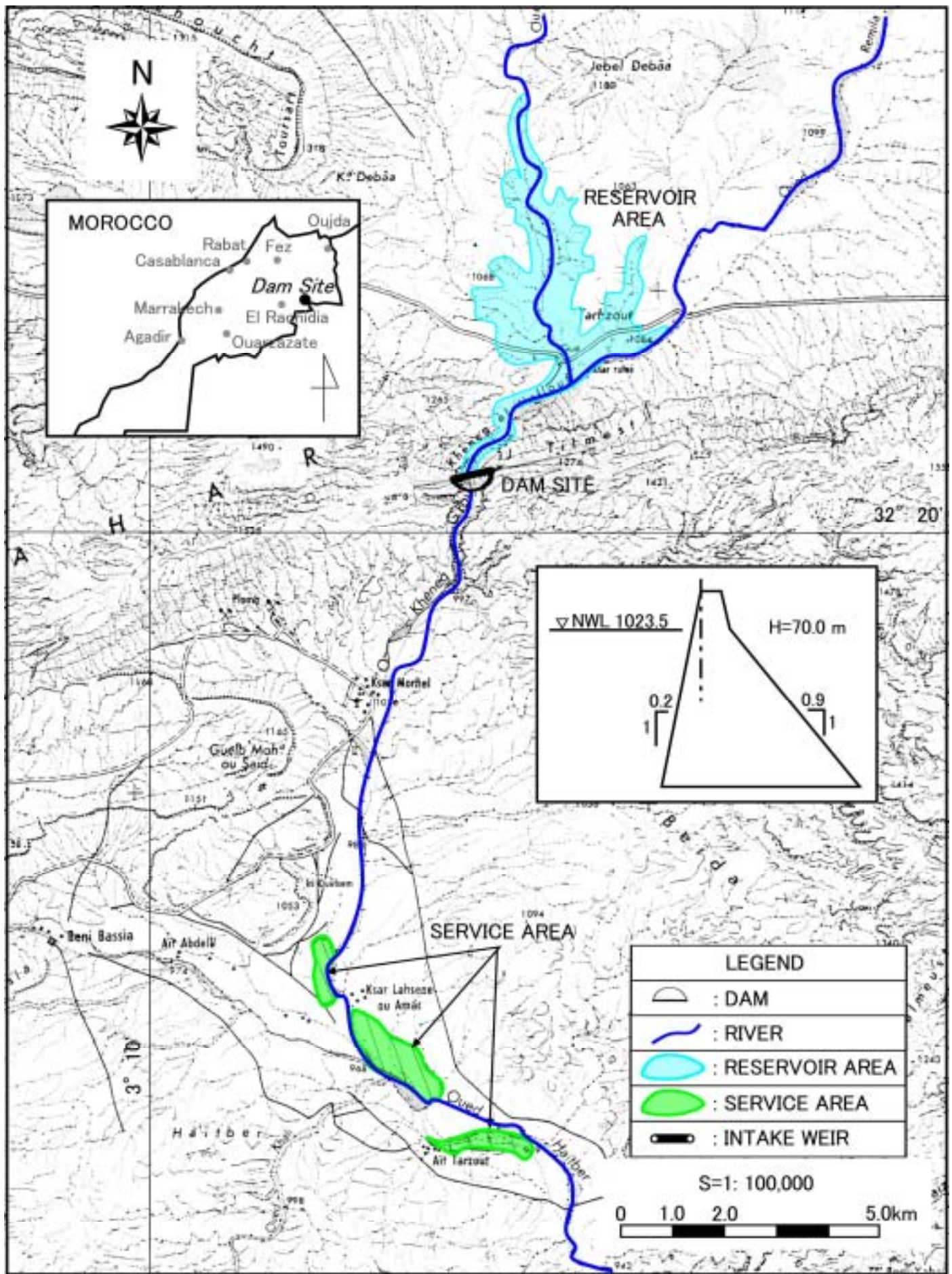
Figure VIII.1.13 General Plan of KHENG GROU (No.13)
