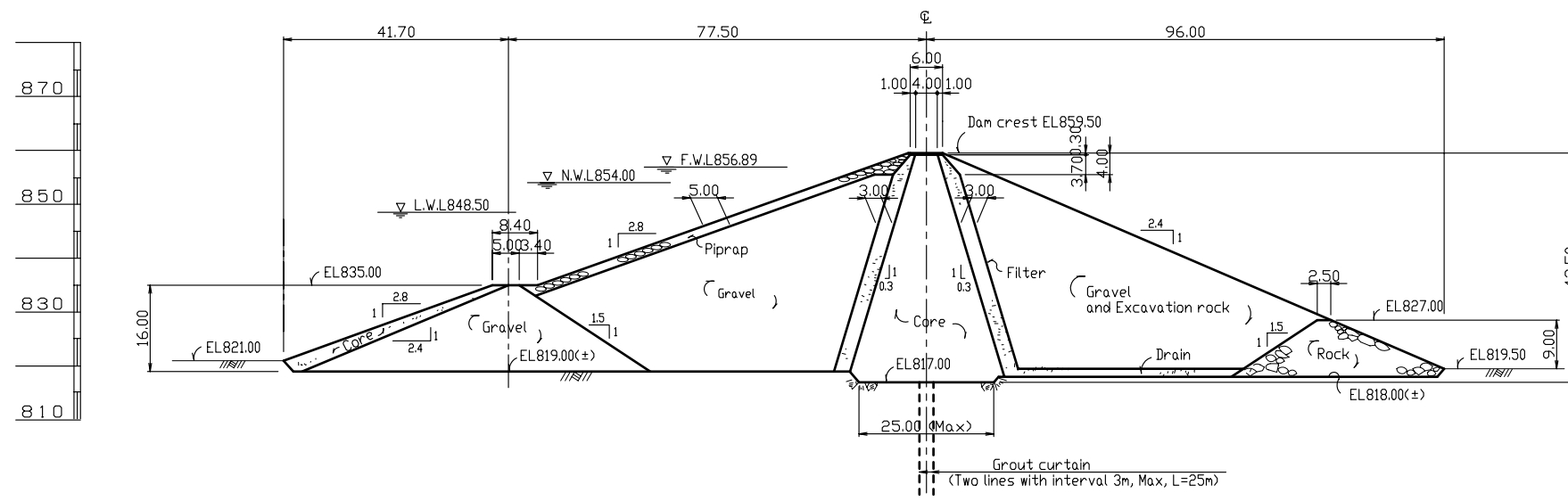
STANDARD CROSS SECTION SCALE A
