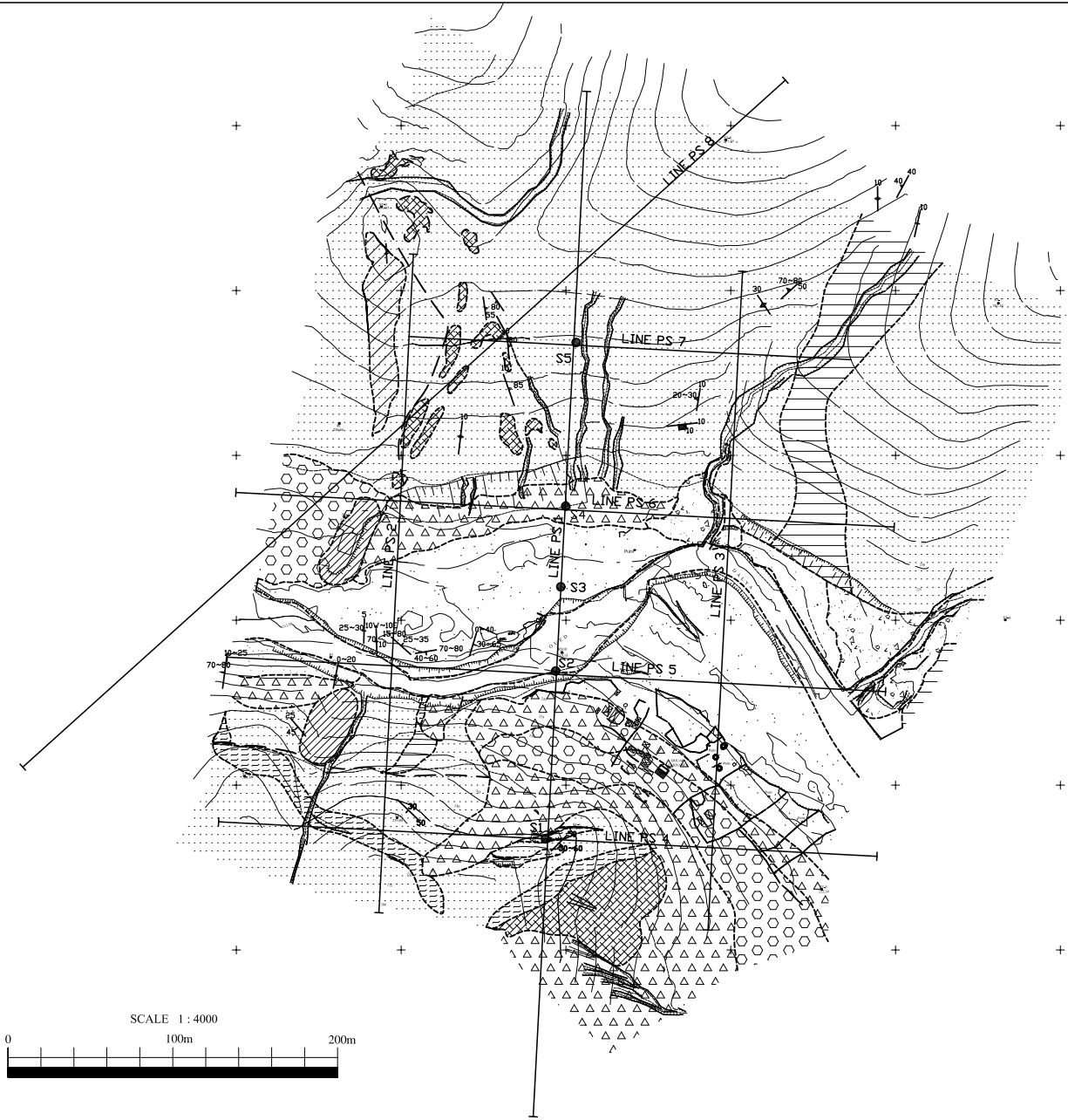
Figure GC1.1 Geological Map around N'frikh Dam Site & Location Map of Drilling and Seismic Prospecting
