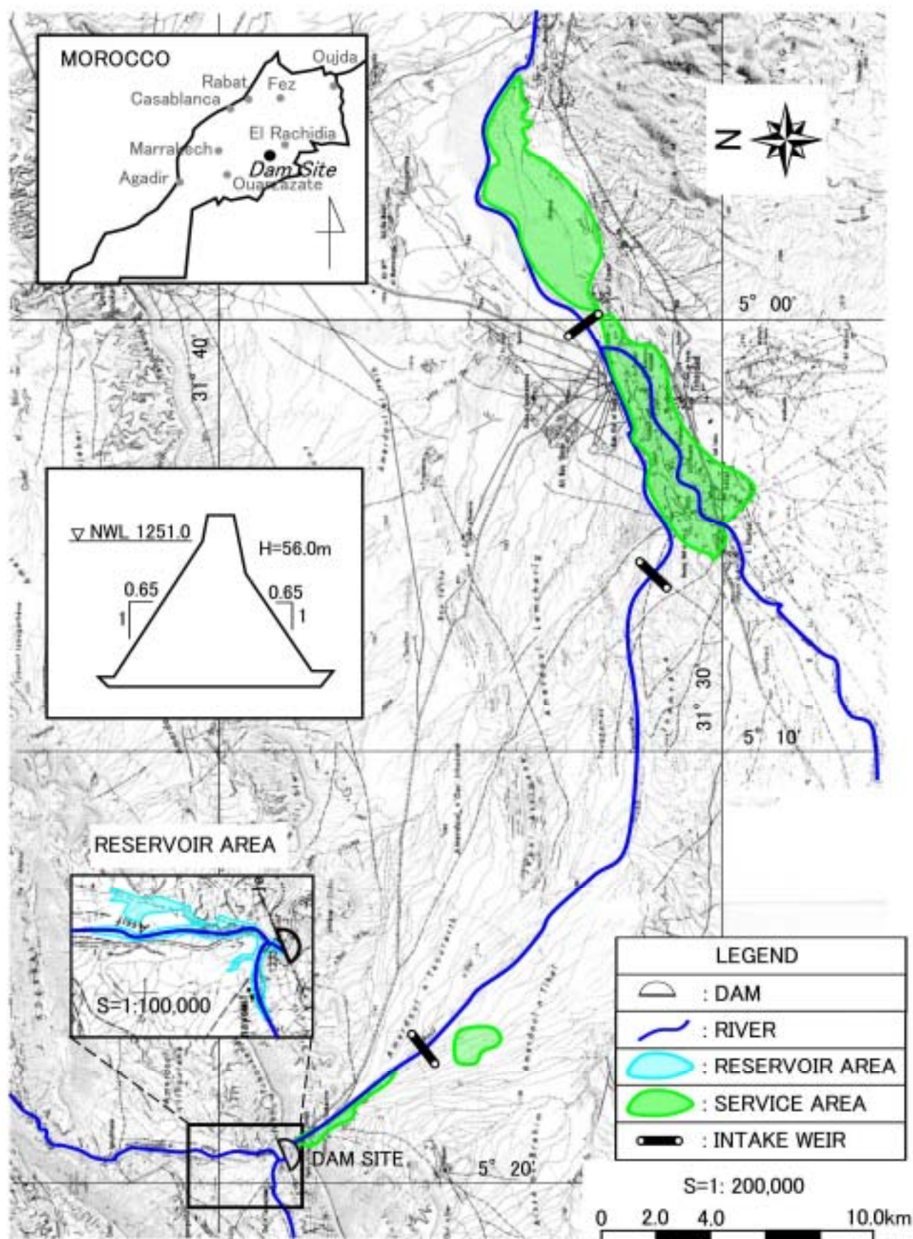
FigureVII.1.1.10 General Plan of TIMKIT (No.10)
