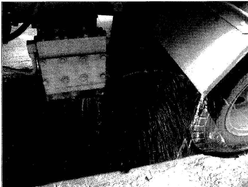
Photo : 15 Leakage of Pressurized Water from Plunger Pump of High Pressure Cleaner
