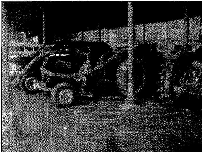
Photo : 3 MODS Zone VI Tractor & Trailer-mounted Desludging Pump
