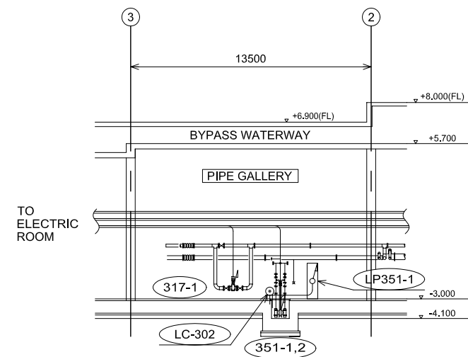
SECTION H-H
