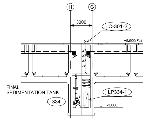
SECTION G-G
