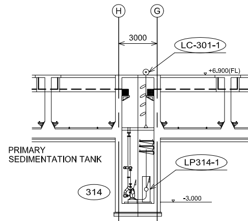
SECTION F-F
