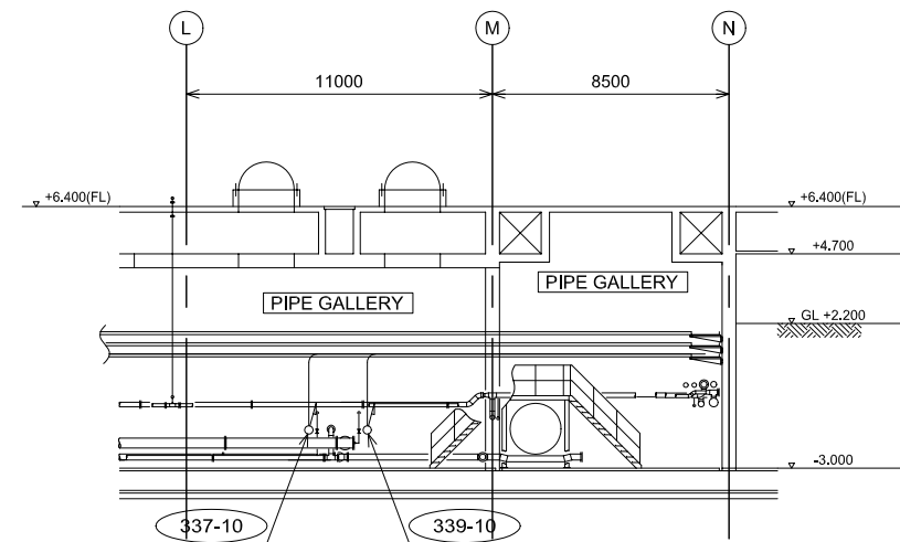
SECTION E-E
