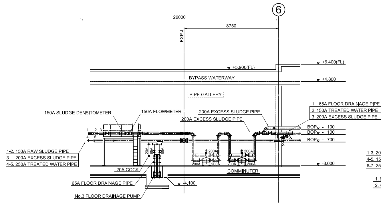
SECTION J-J
