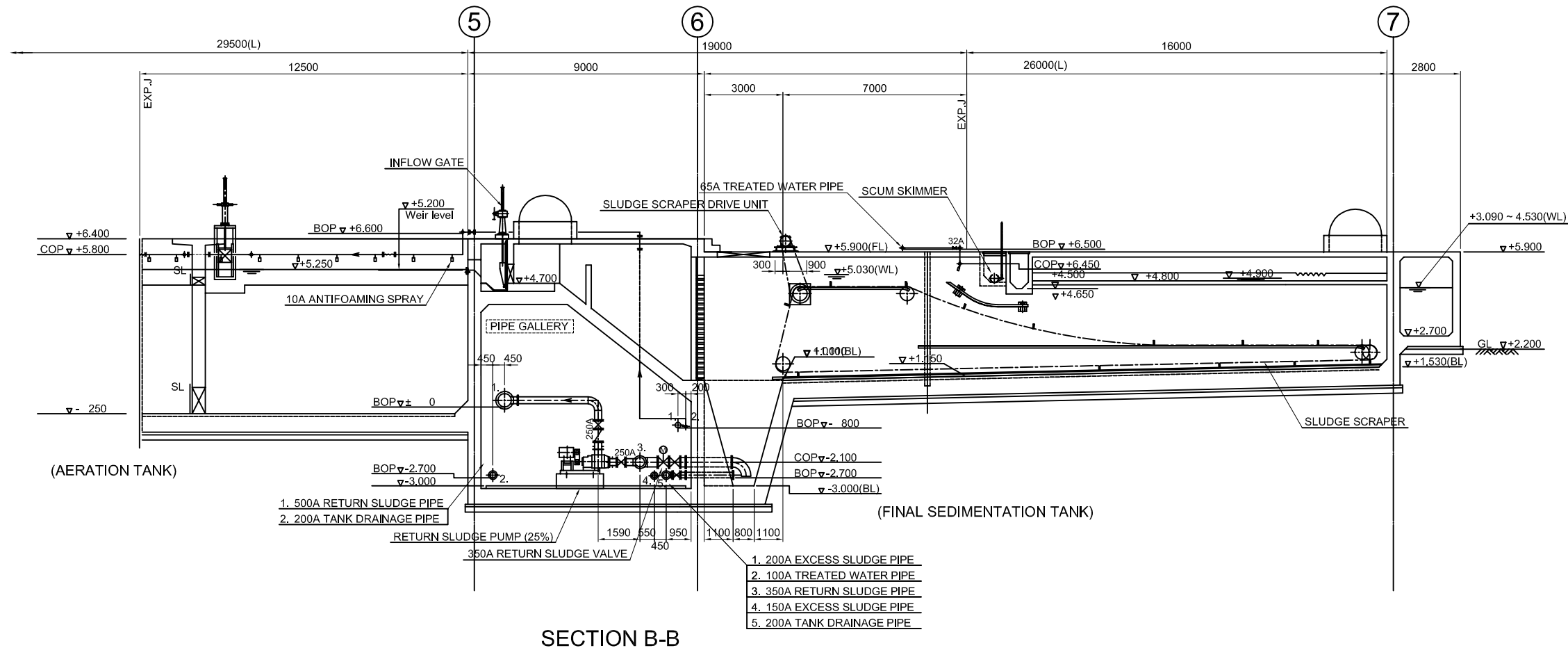
SECTION B-B
