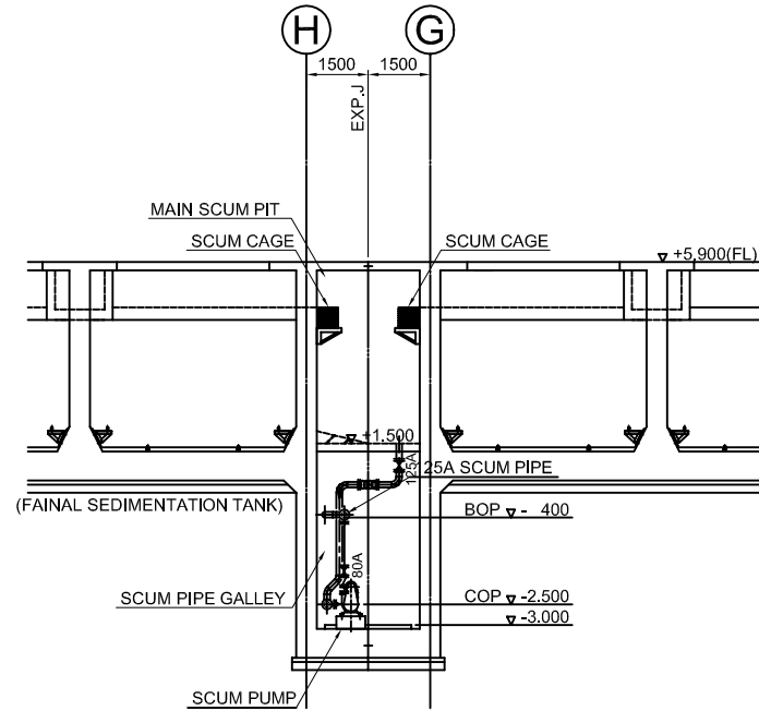
SECTION H-H
