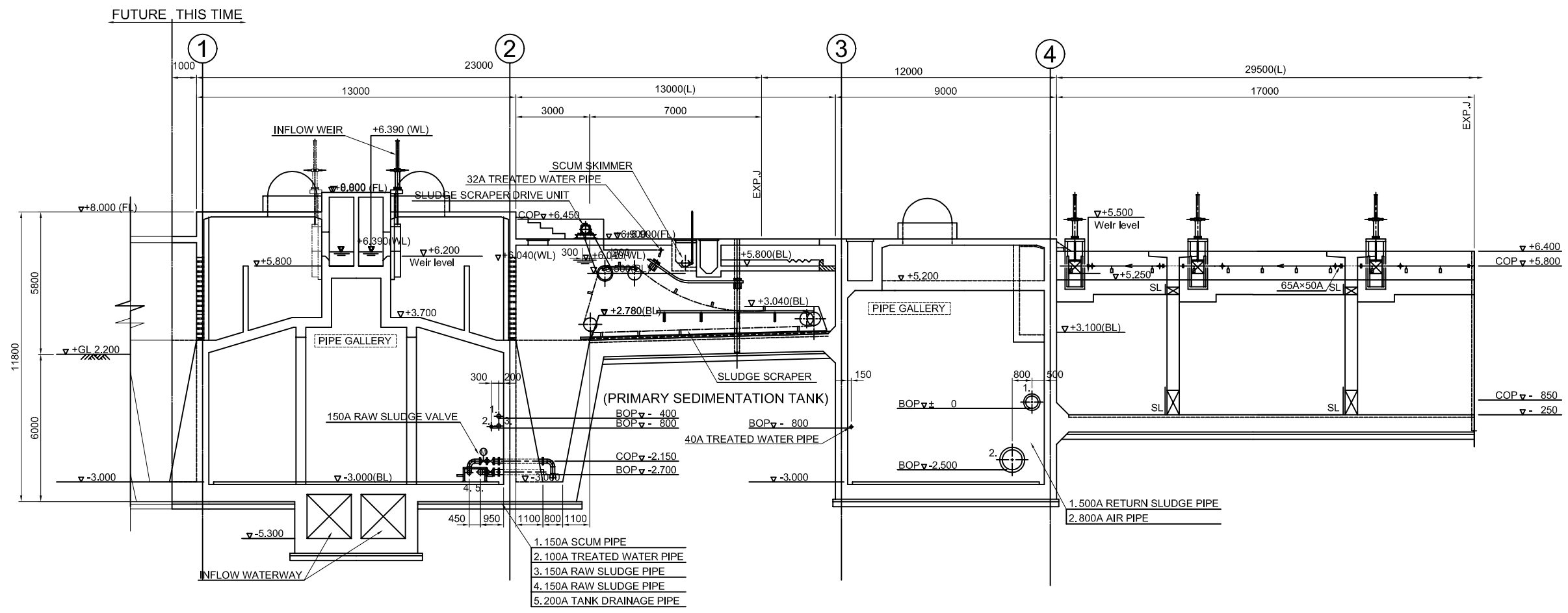
SECTION B-B
