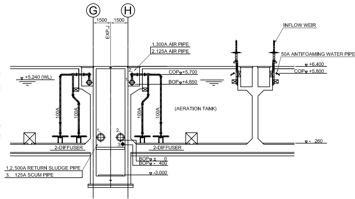
SECTION I-I
