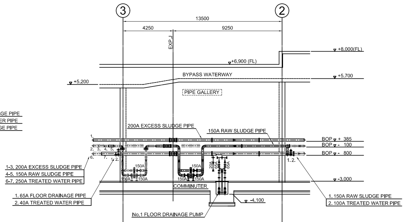
SECTION J-J
