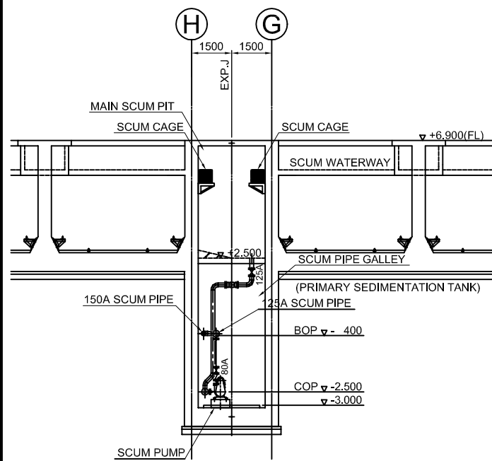
SECTION G-G
