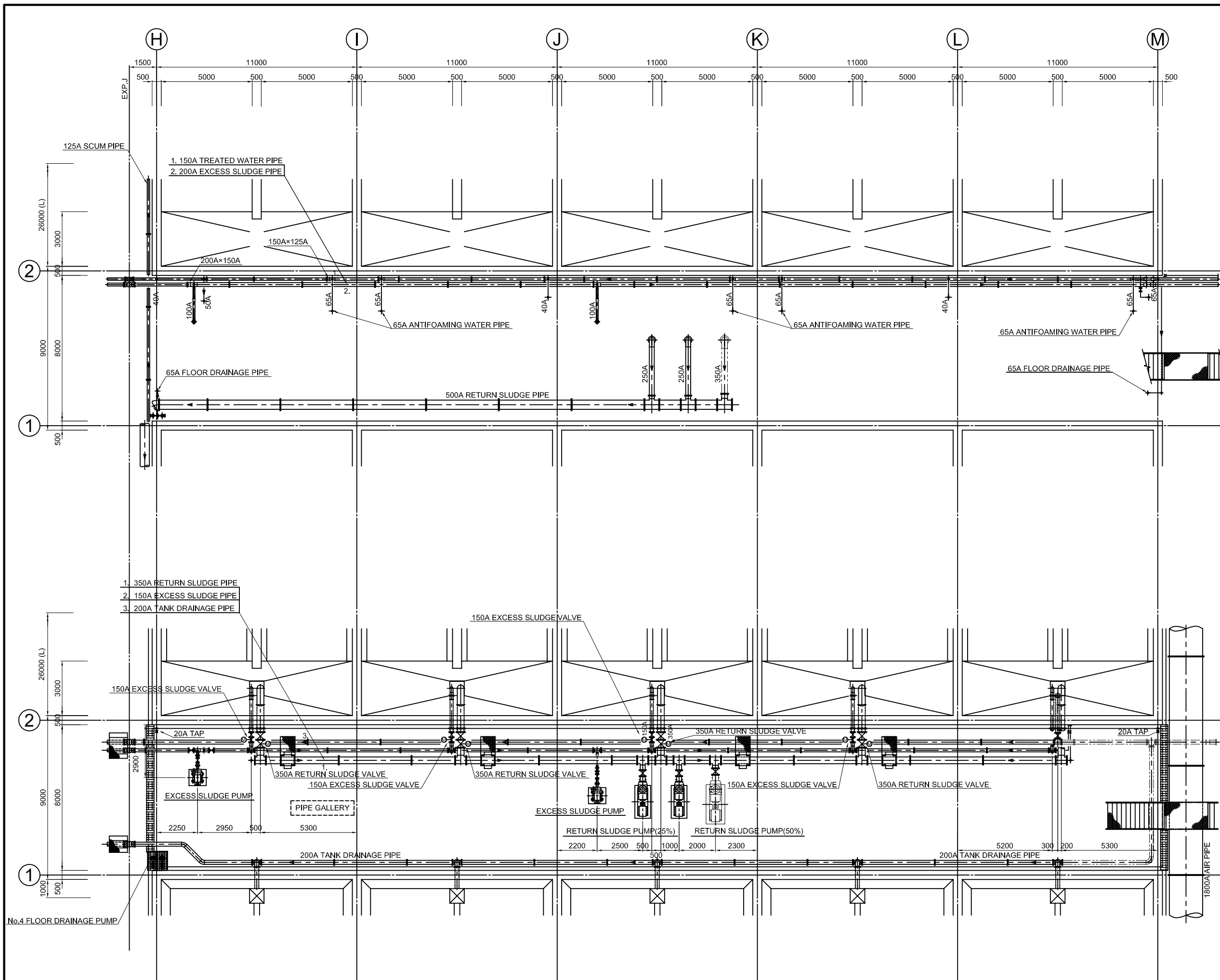
FINAL SEDIMENTATION TANK PIPE GALLERY LOWER&MIDDLE PLAN (2)
