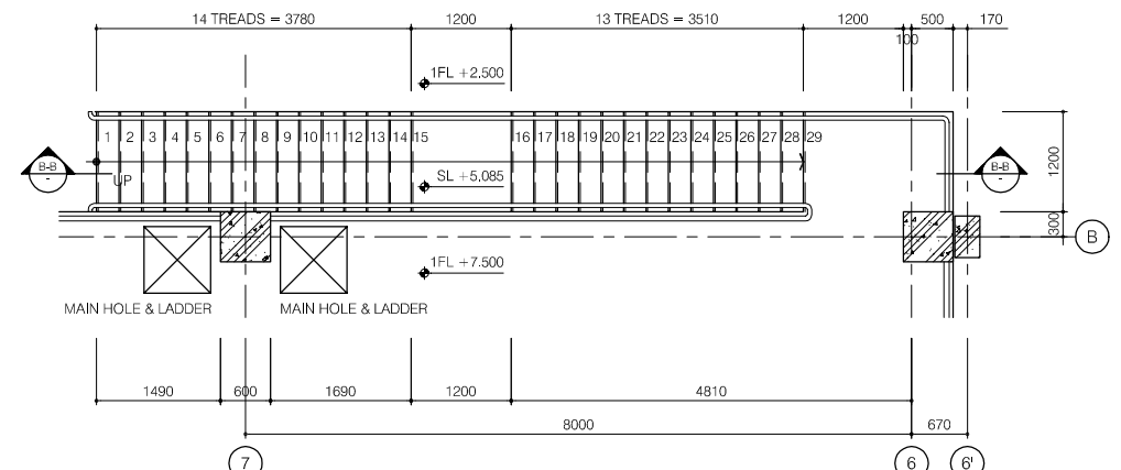
FLOOR PLAN (S03)
