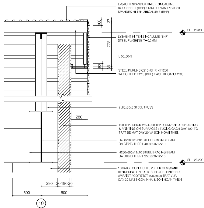
SECTION DETAIL - R03
