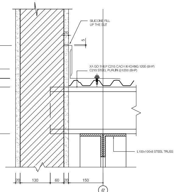
SECTION DETAIL - R04
