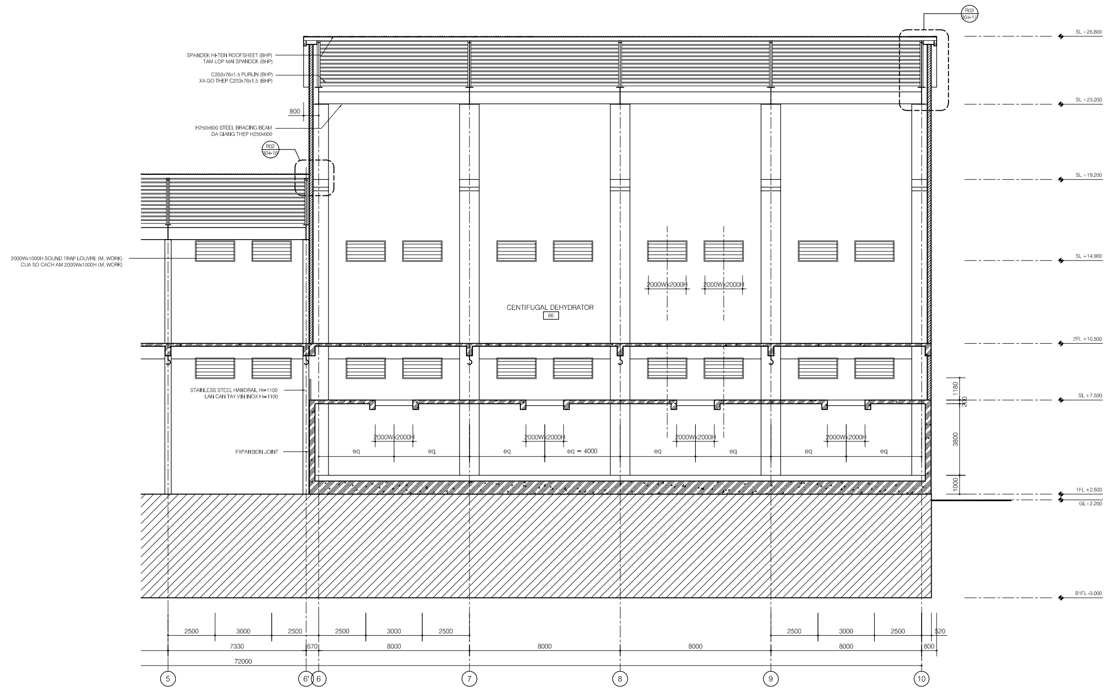
LONGITUDINAL SECTION C-C (2/2)
