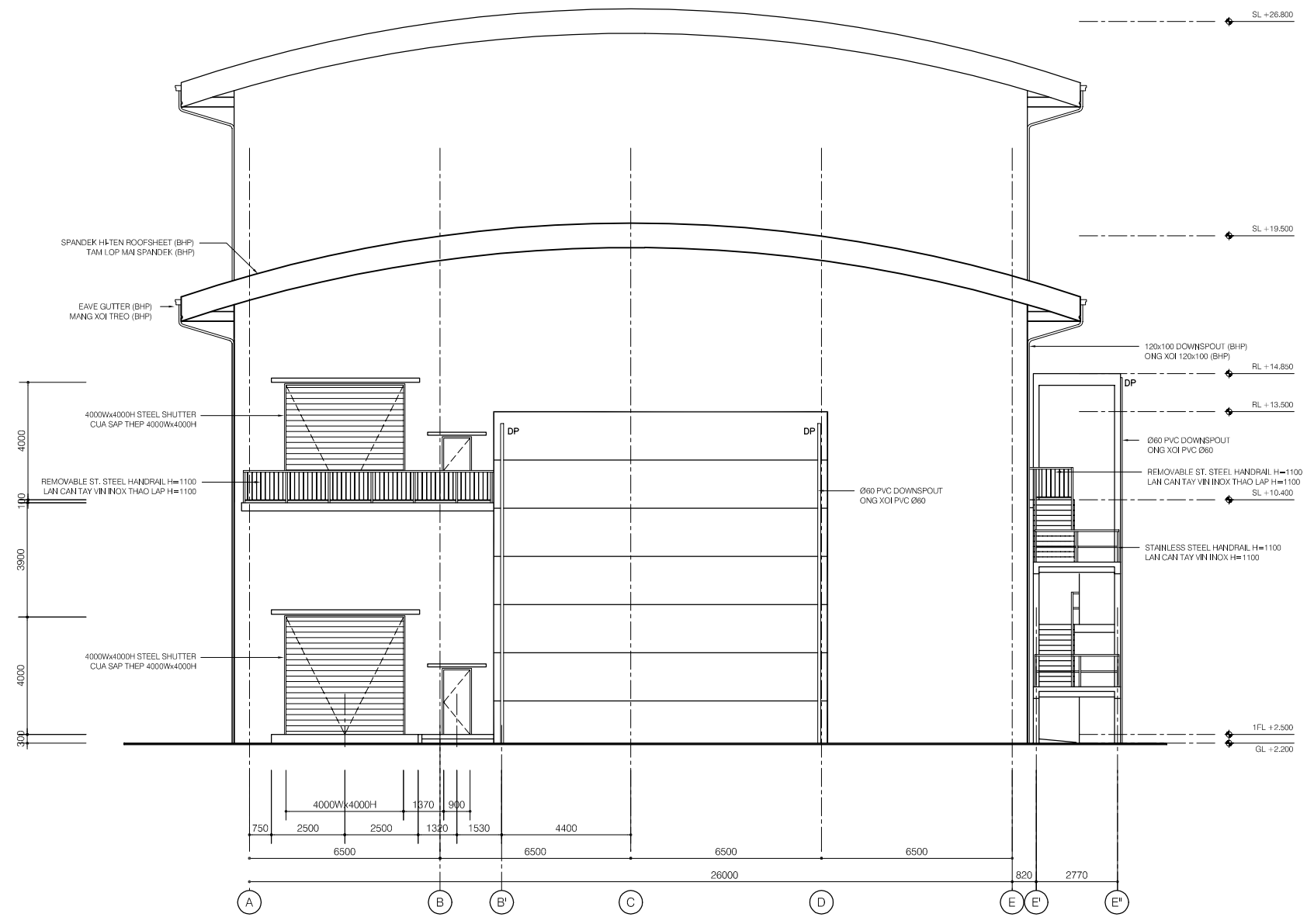
ELEVATION LINE 1
