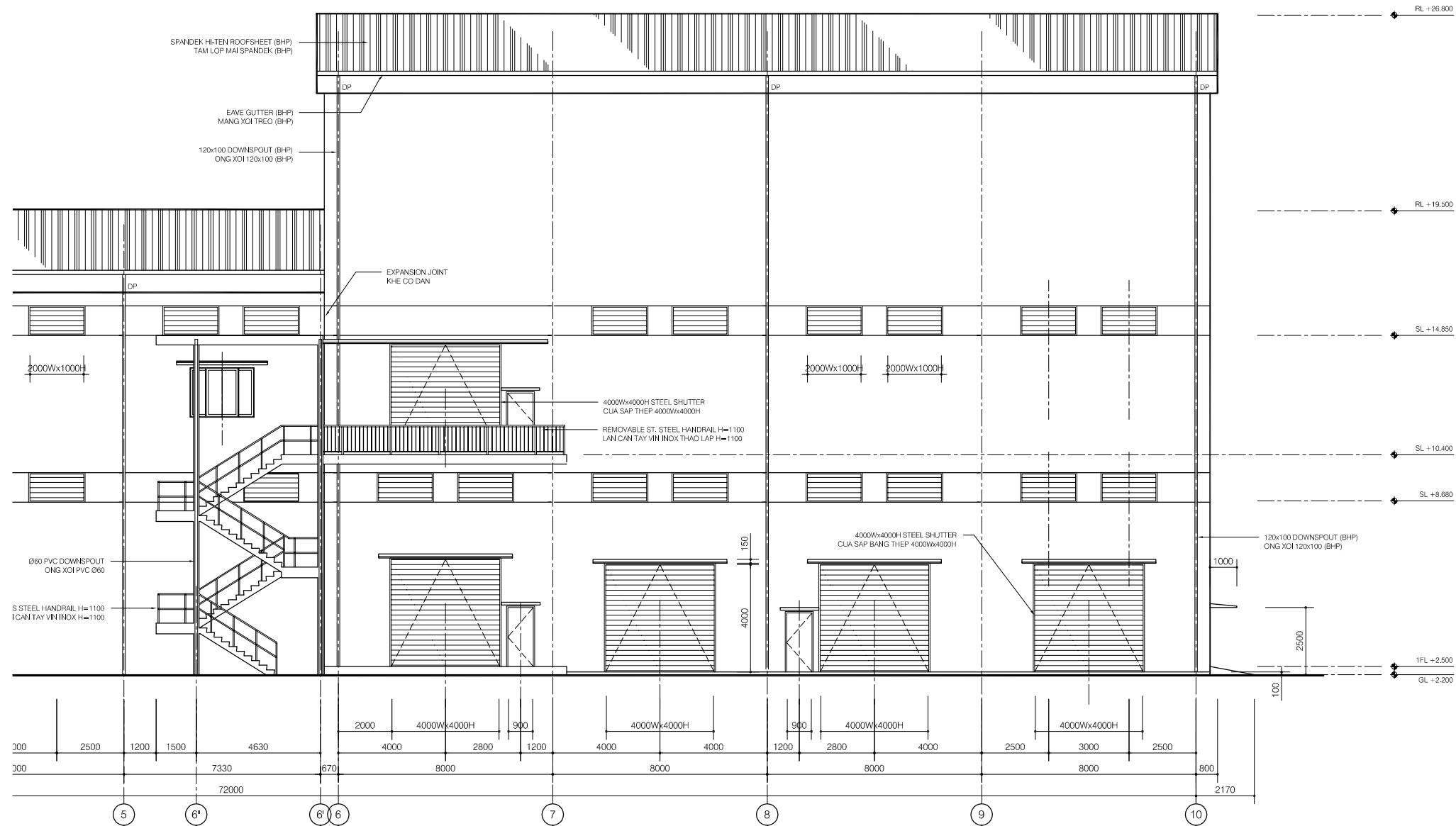
ELEVATION LINE E (2/2)
