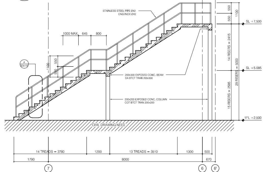
SECTION B-B
