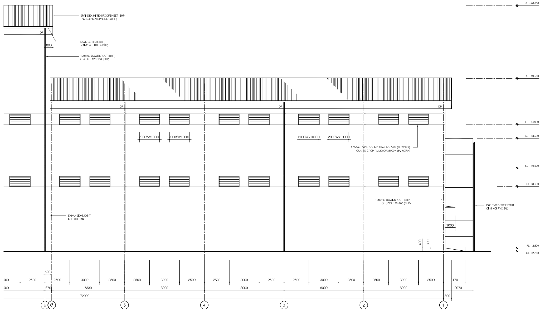
ELEVATION LINE A (2/2)
