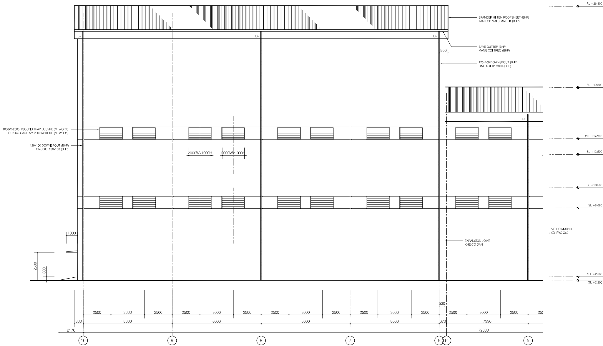
ELEVATION LINE A (1/2)
