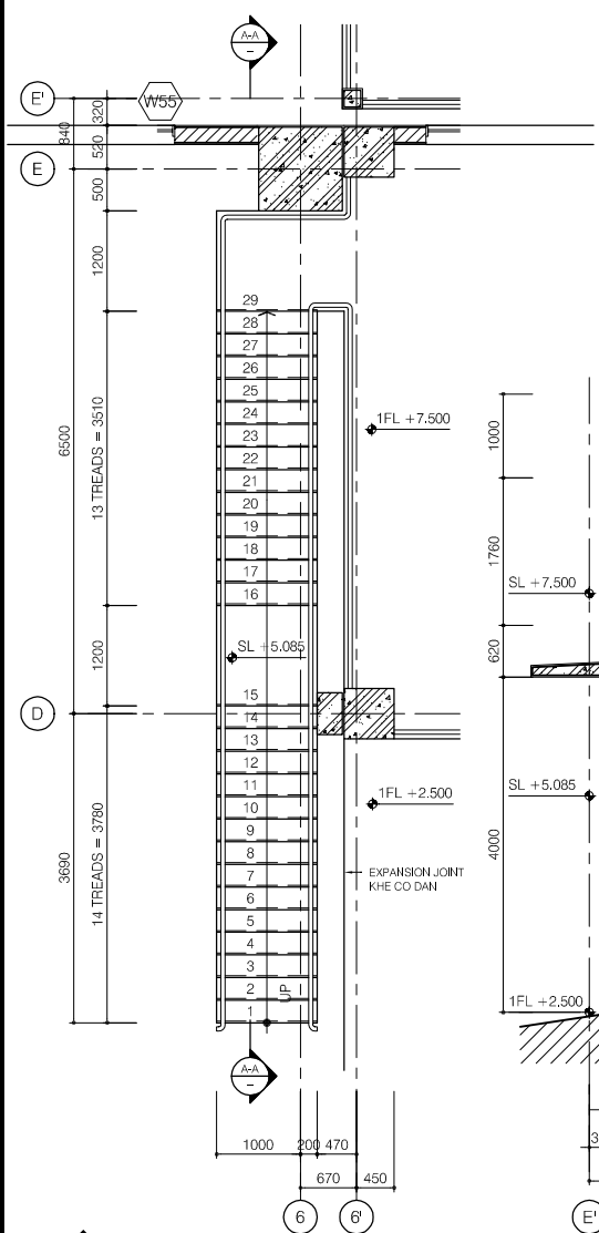
FLOOR PLAN (S02)
