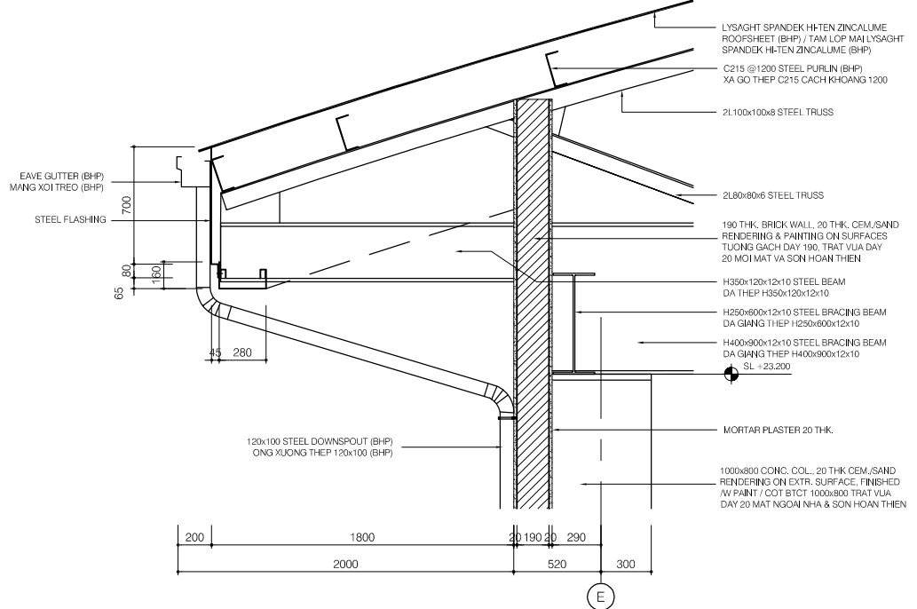
SECTION DETAIL - R01
