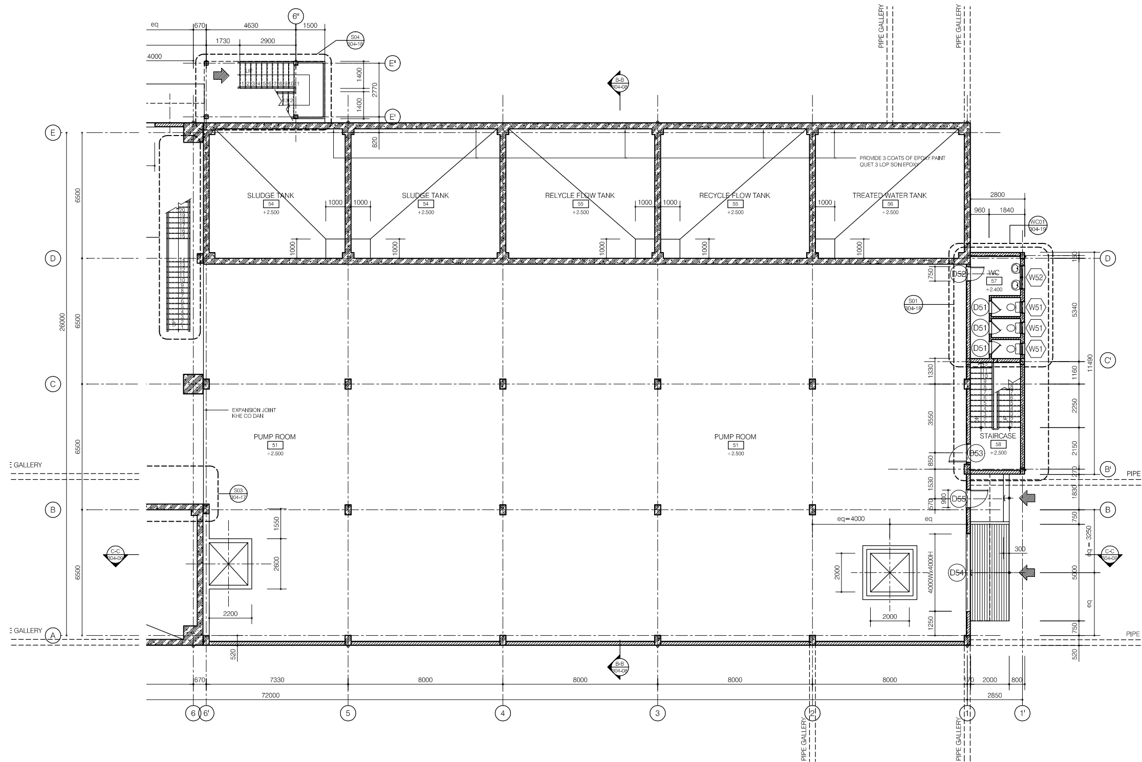
FIRST FLOOR PLAN (2/2)
