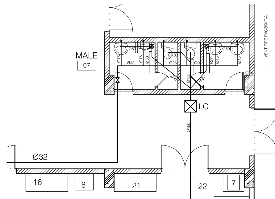
WC ENLARGED TOILET PLAN SCALE : 1/50
