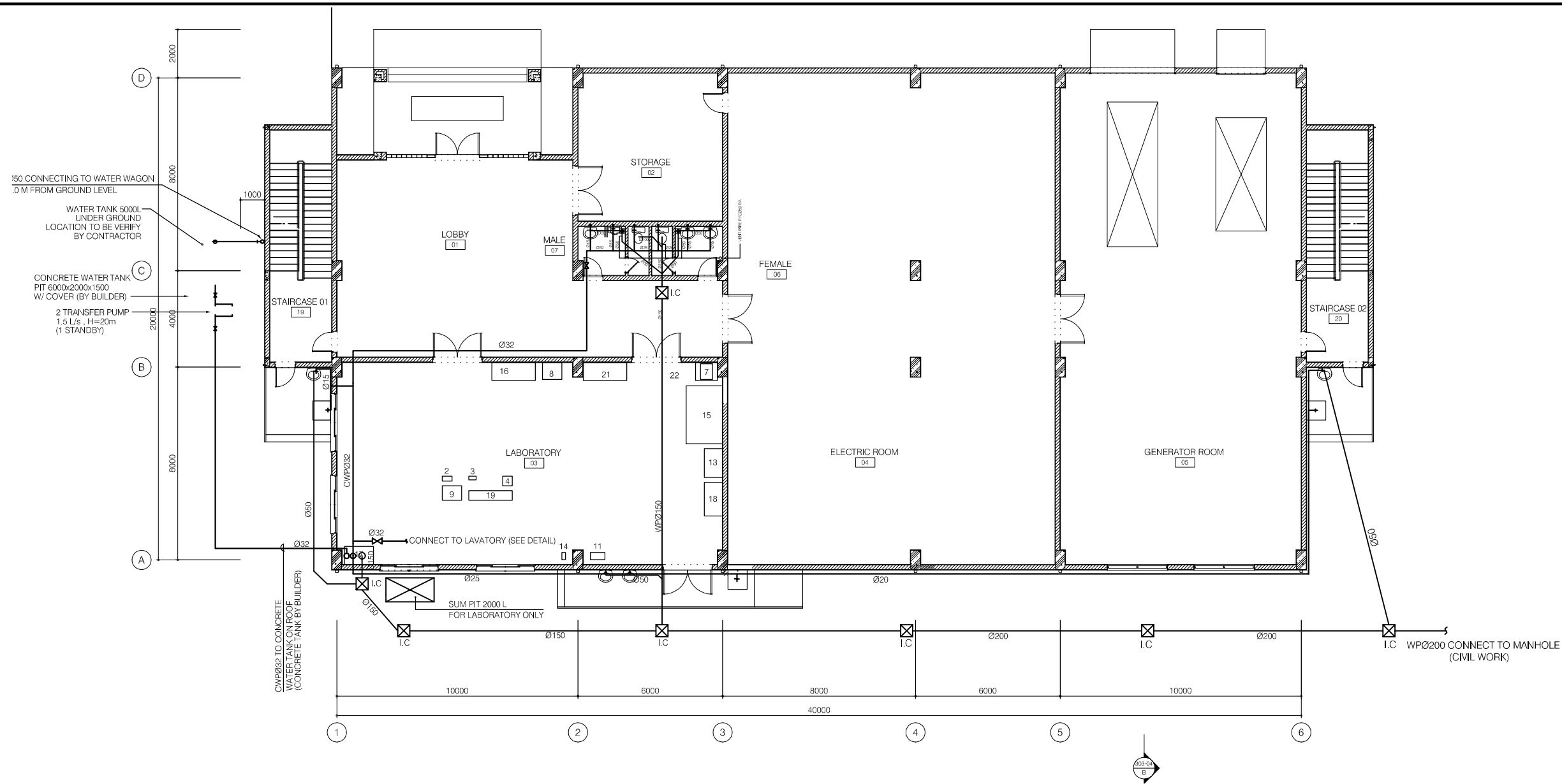
FIRST FLOOR - PLUMBING AND DRAINAGE PLAN SCALE : 1/100
