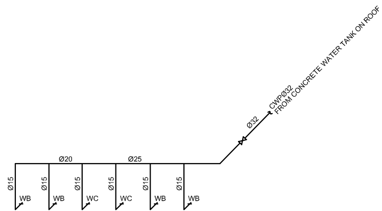
ISOMETRIC OF COLD WATER SUPPLY SYSTEM
