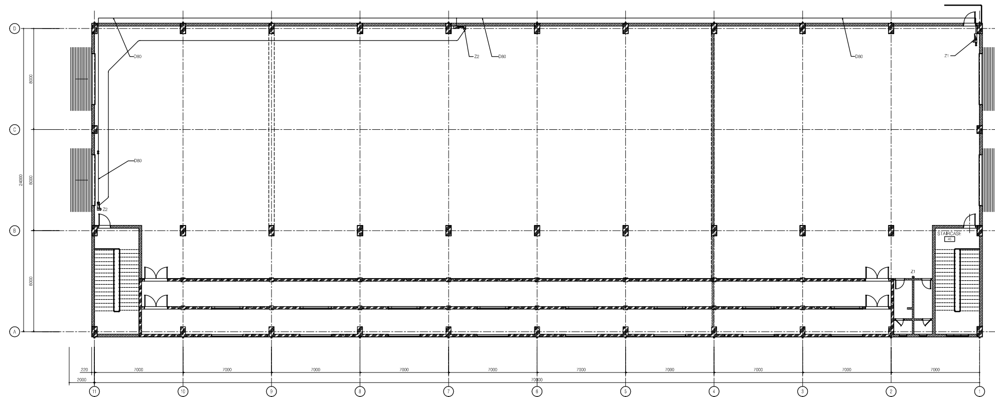
FIRST FLOOR - FIRE ALARM PLAN SCALE: 1/150
