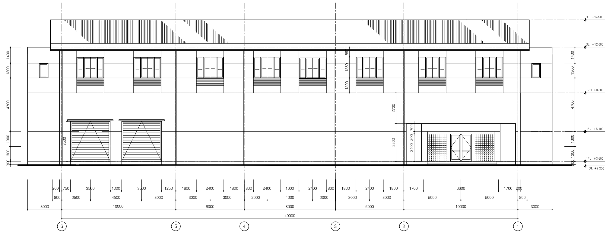
ELEVATION LINE D
