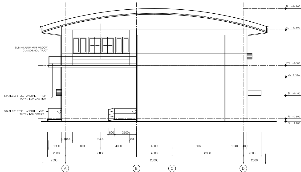
ELEVATION LINE 6
