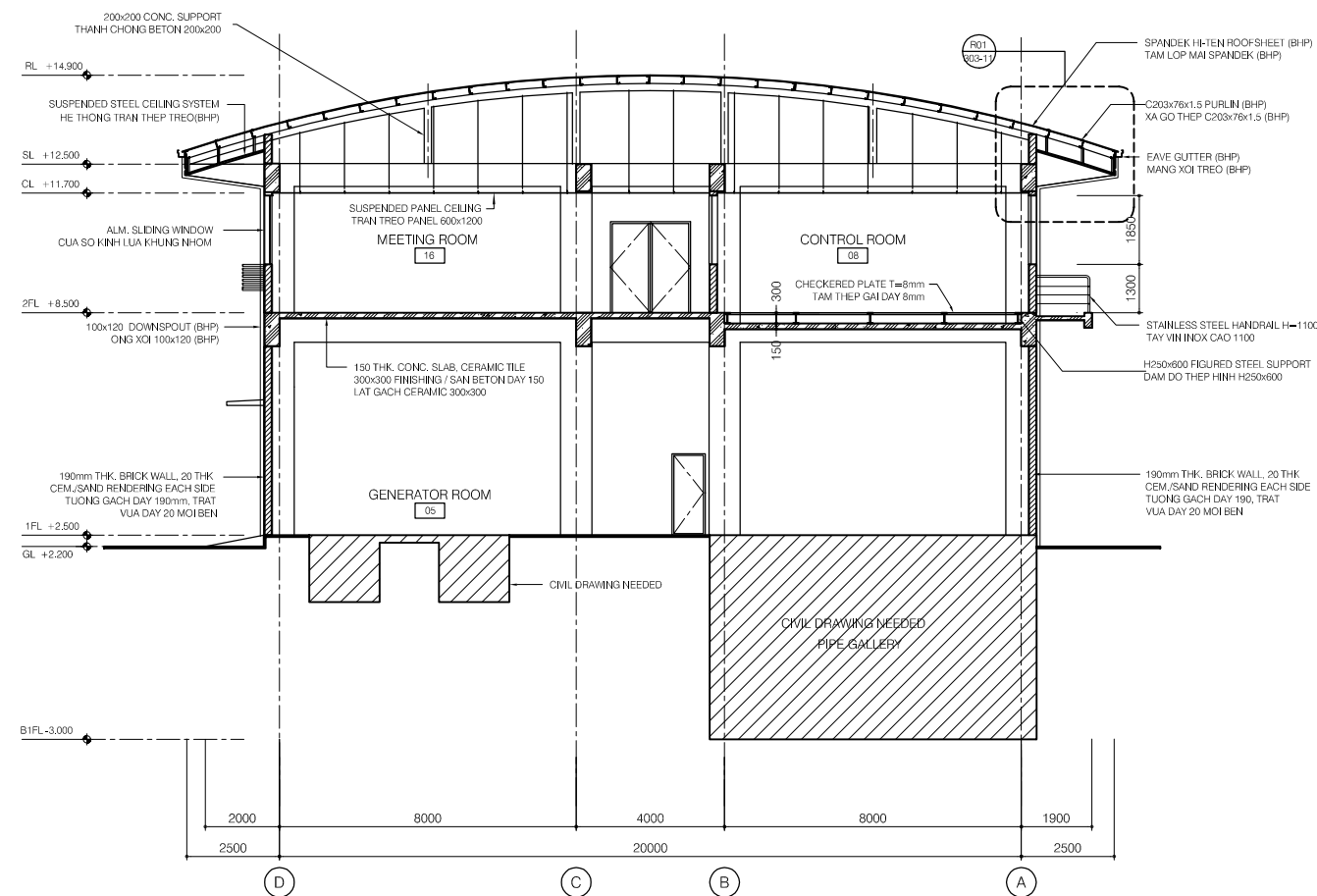
SECTION B-B
