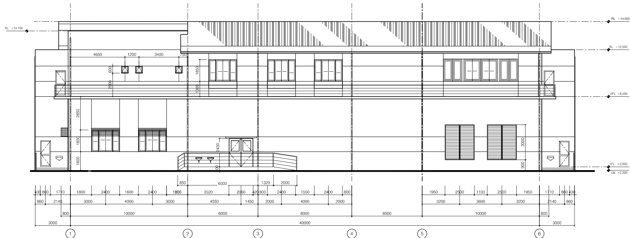
ELEVATION LINE A
