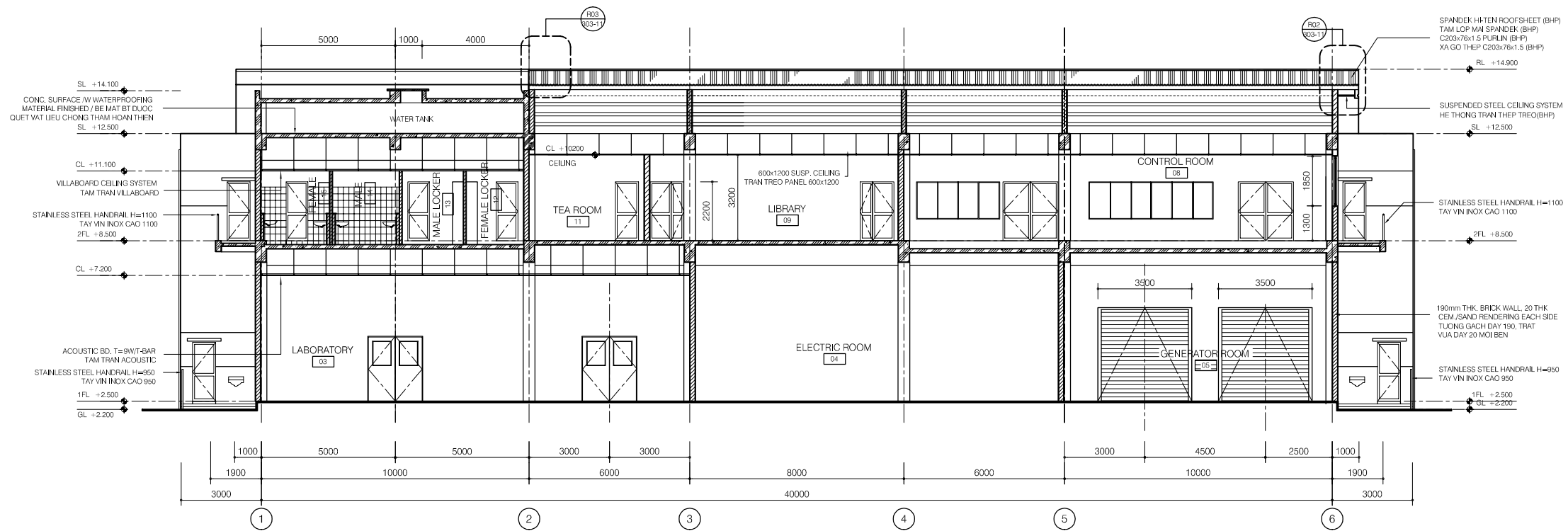
SECTION C-C
