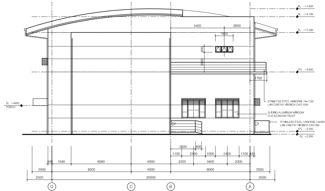
ELEVATION LINE 1
