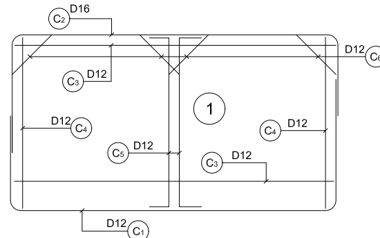
BAR SKELETON @250
