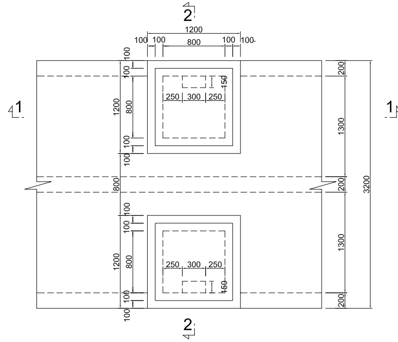
PLAN 1
