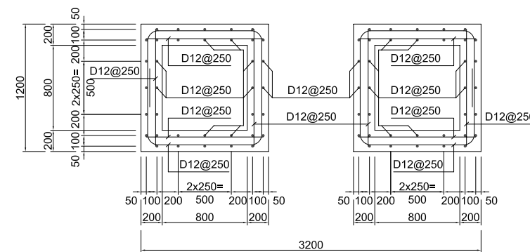
SECTION 1-1
