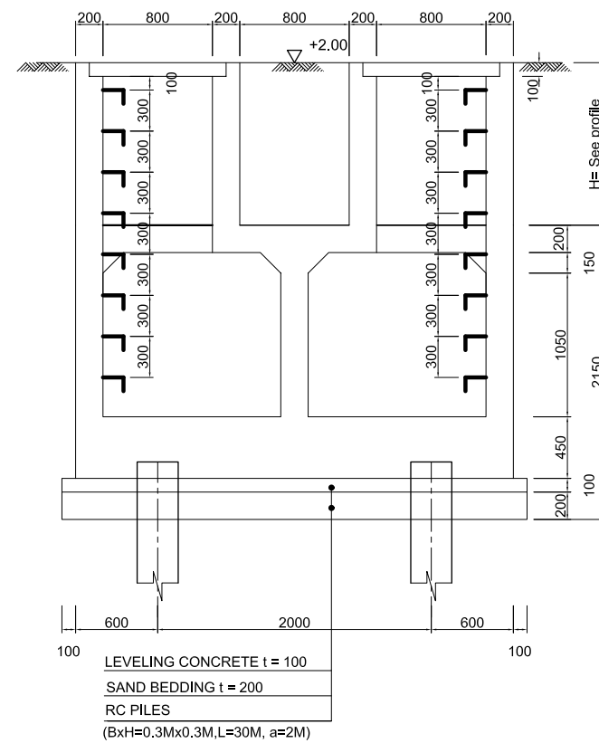
SECTION 4-4
