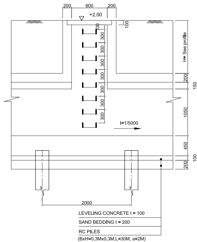
SECTION 3-3
