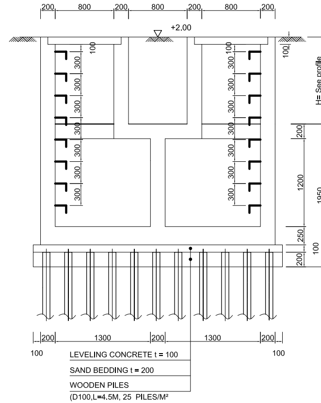
SECTION 2-2
