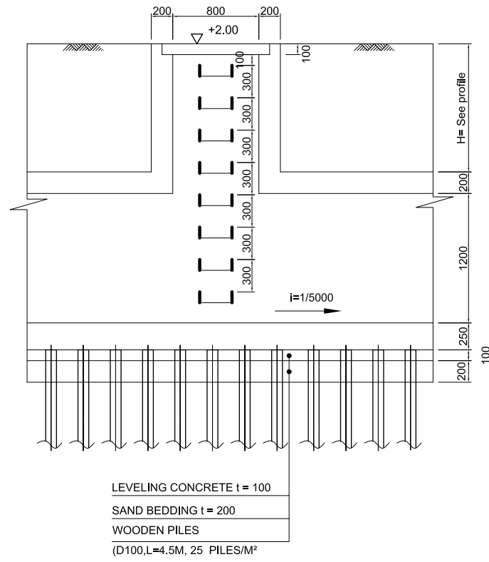
SECTION 1-1
