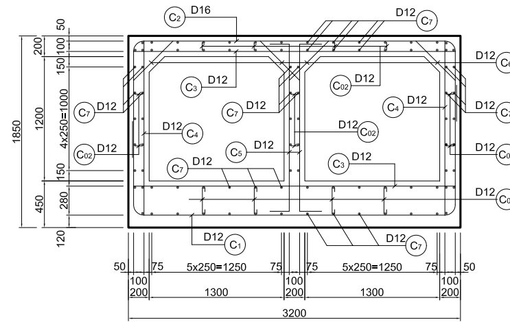
BAR SKELETON @250
