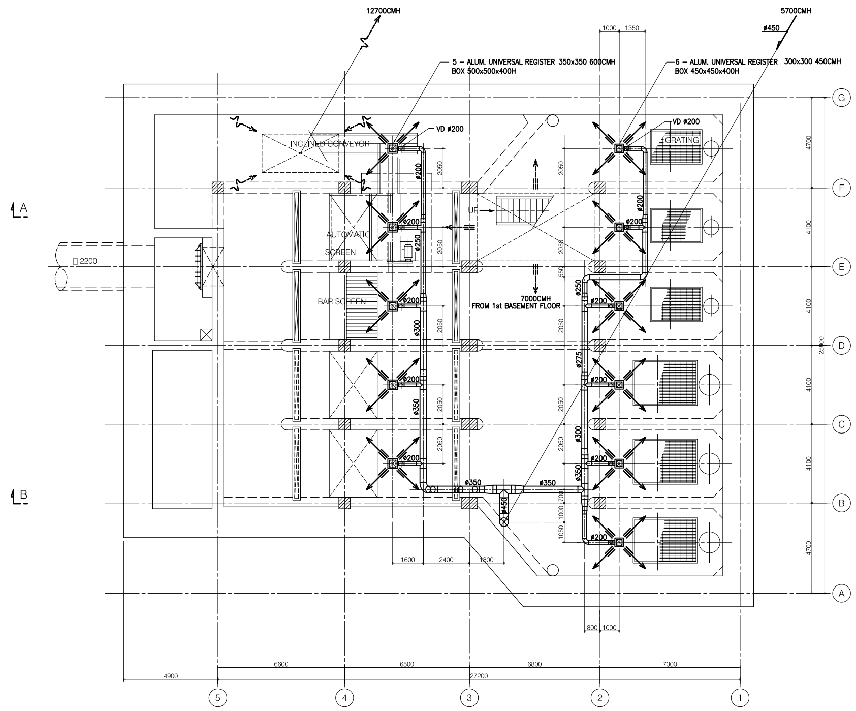
2nd BASEMENT FLOOR PLAN
