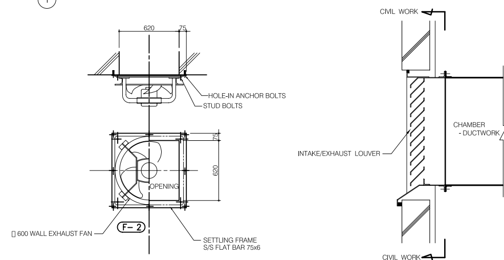
DETAILS OF WALL EXHAUST FAN & INTAKE/EXHAUST LOUVER
