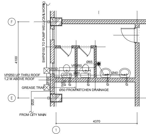
WC LAYOUT PLAN
