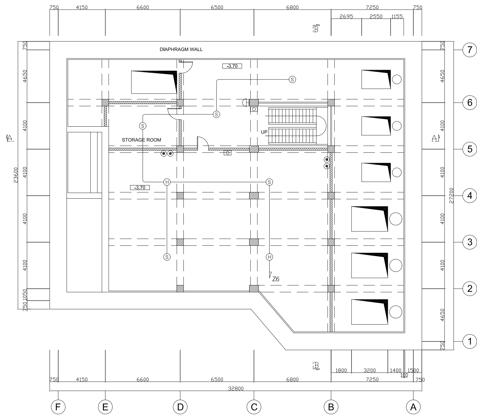
FIRE FIGHTING PLAN OF BASEMENT 1
