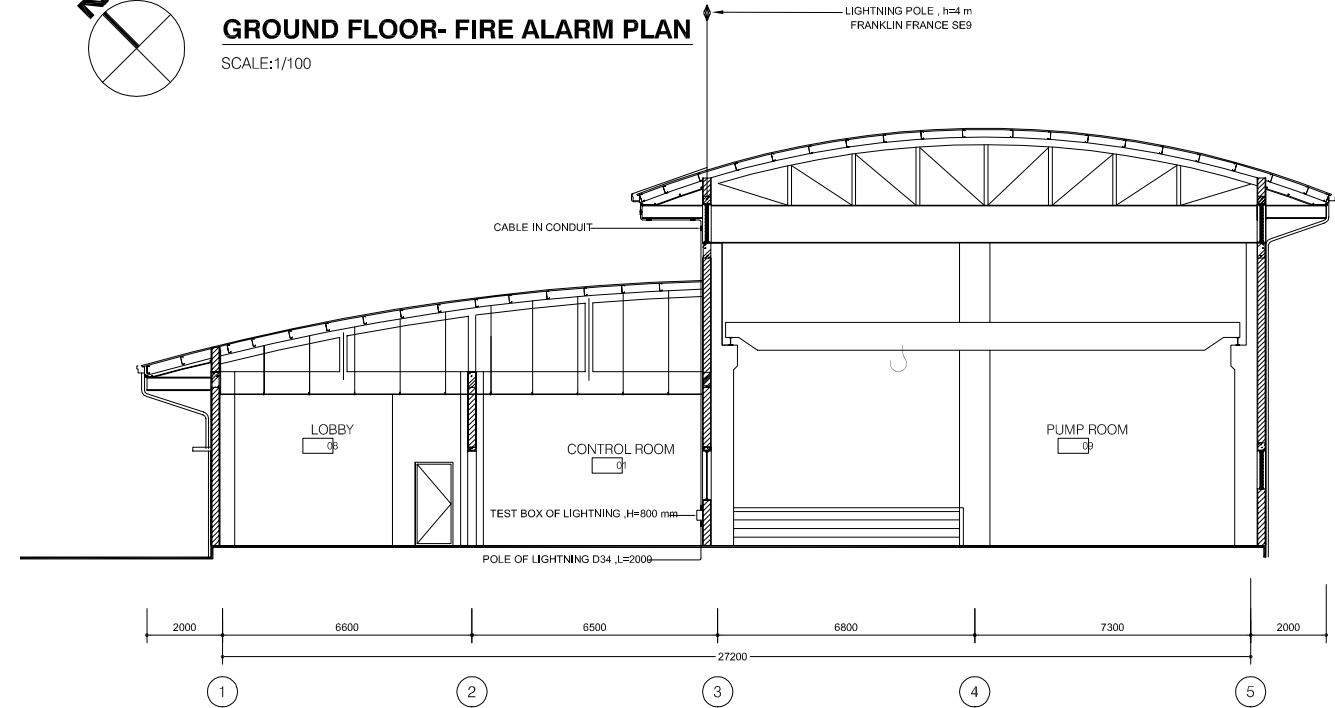
LIGHTNING SYSTEM SCALE: 1/100
