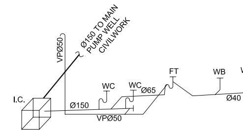
ISOMETRIC OF WASTEWATER SYSTEM
