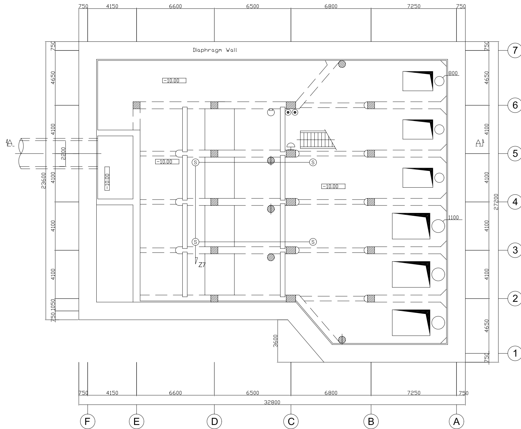
FIRE FIGHTING PLAN OF BASEMENT 2
