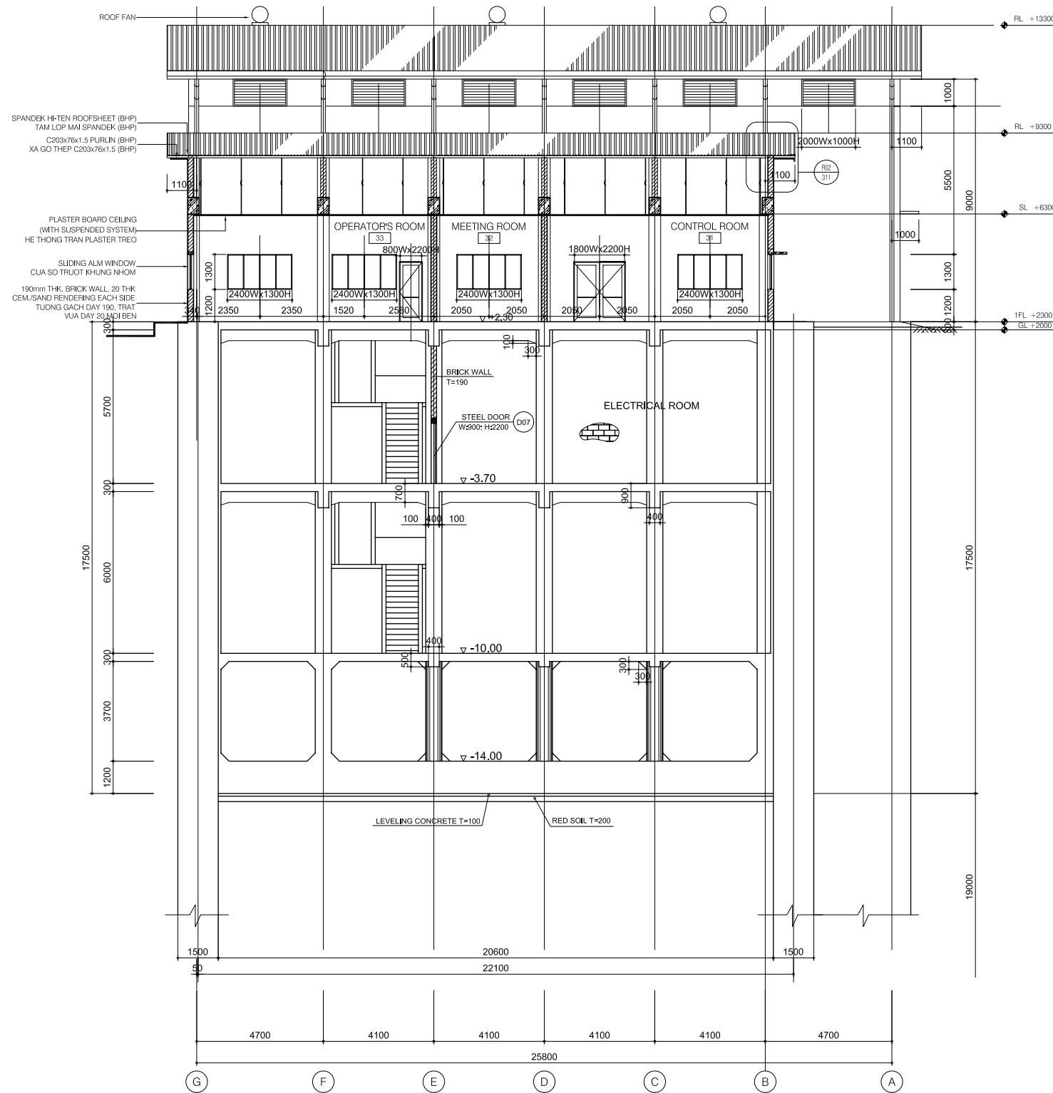
SECTION B-B
