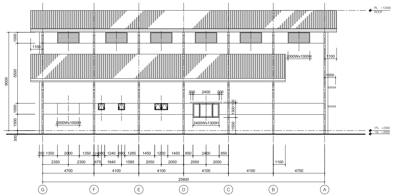
ELEVATION LINE 1
