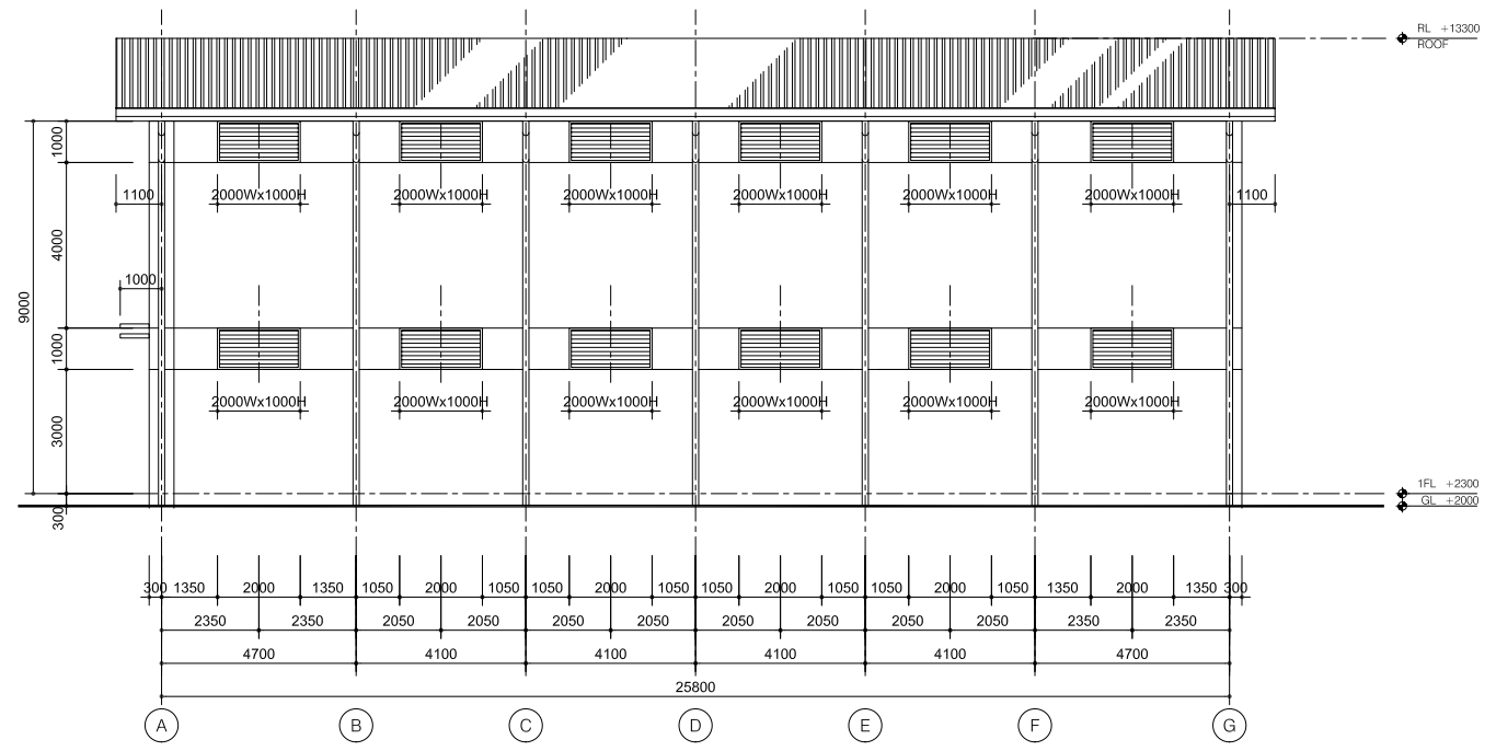
ELEVATION LINE 5
