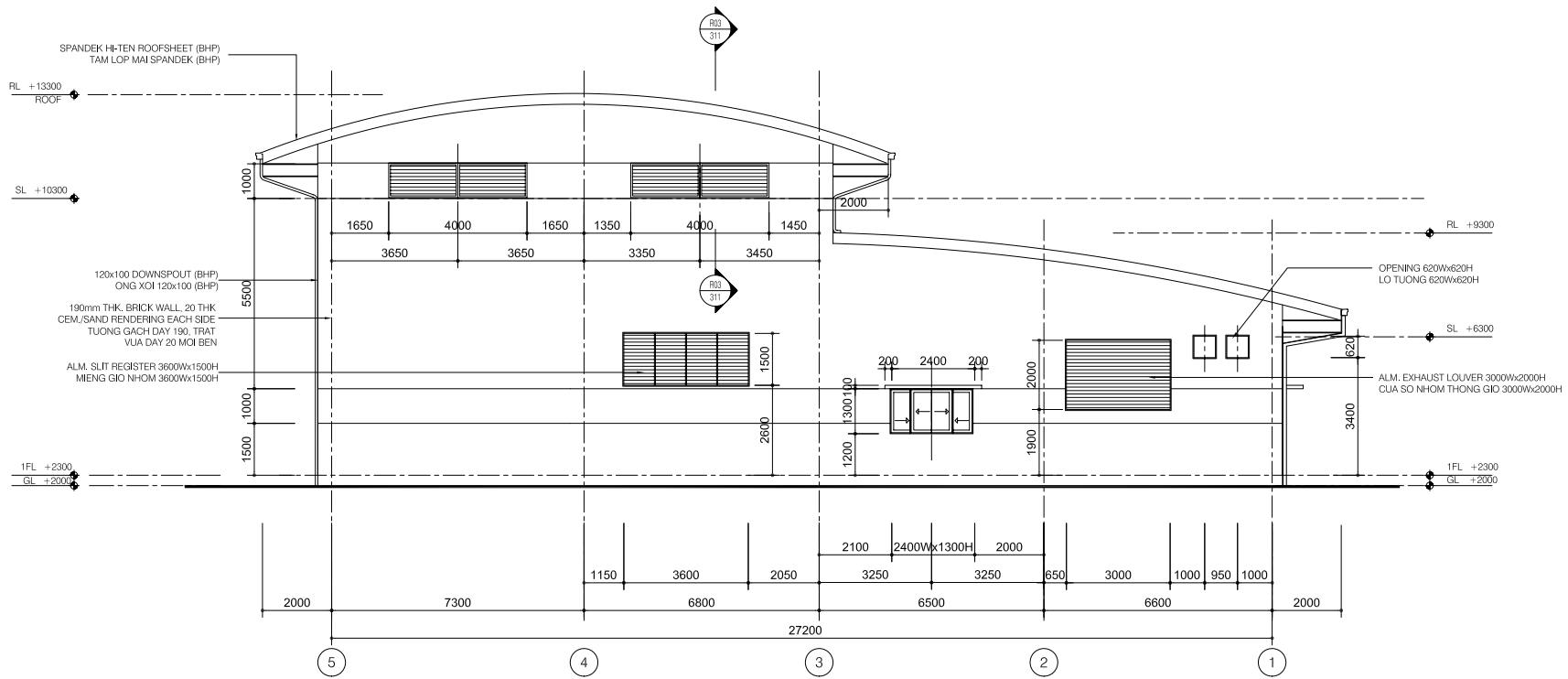
ELEVATION LINE A
