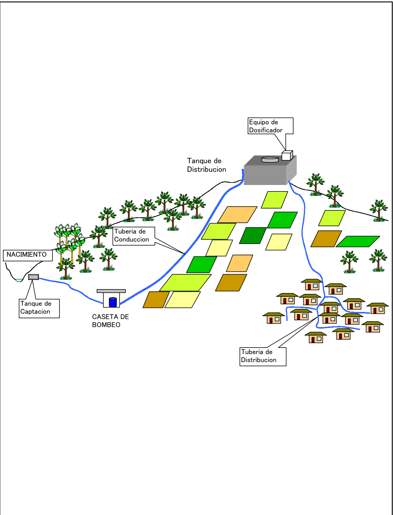
Figure 8.3.3 (1) Drinking Water Quality Improvement Plan Outline of Drinking Water Supply System Xeatzan Bajo, Patzun, Chimaltenango
