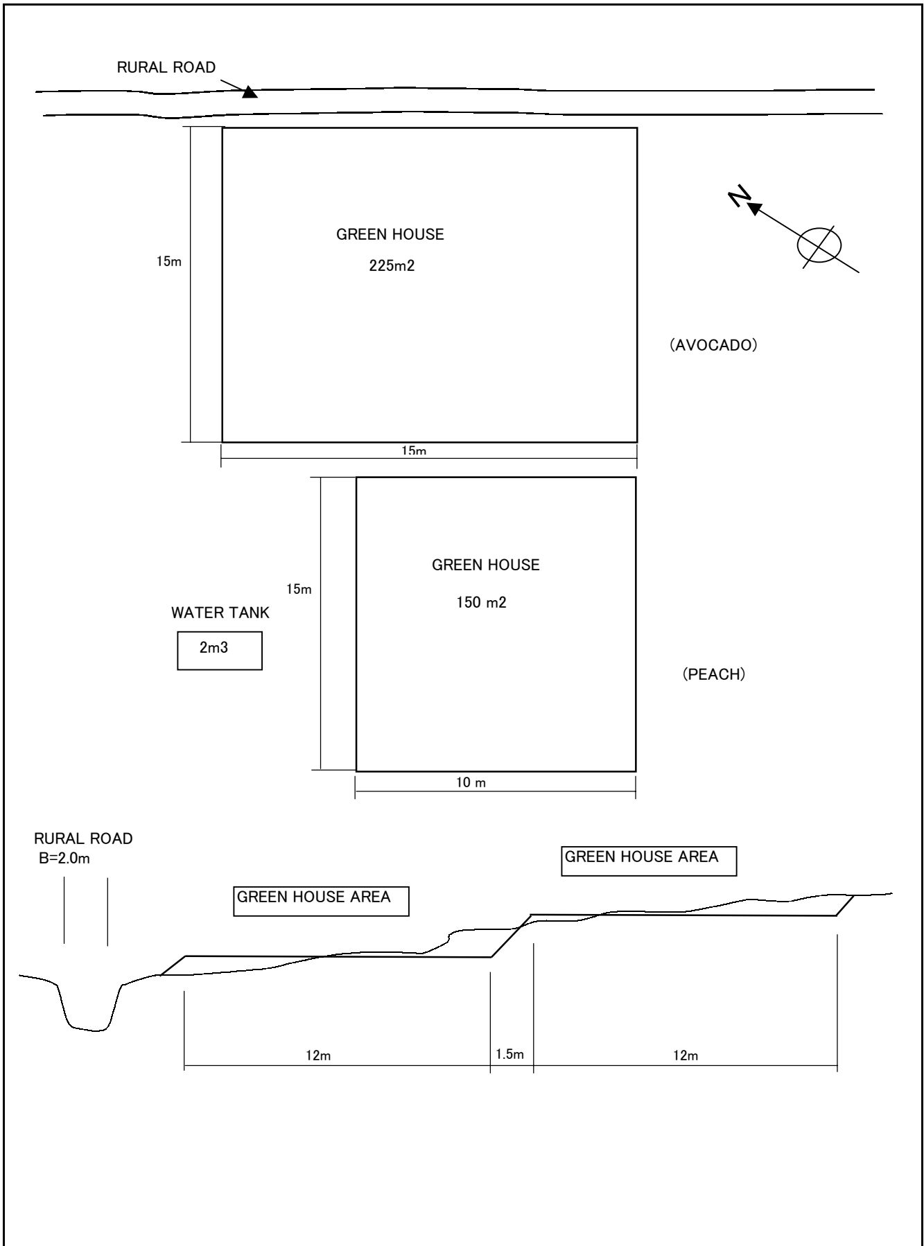
Figure 8.4.1(5) Proposed Land for Vinylhouse B
