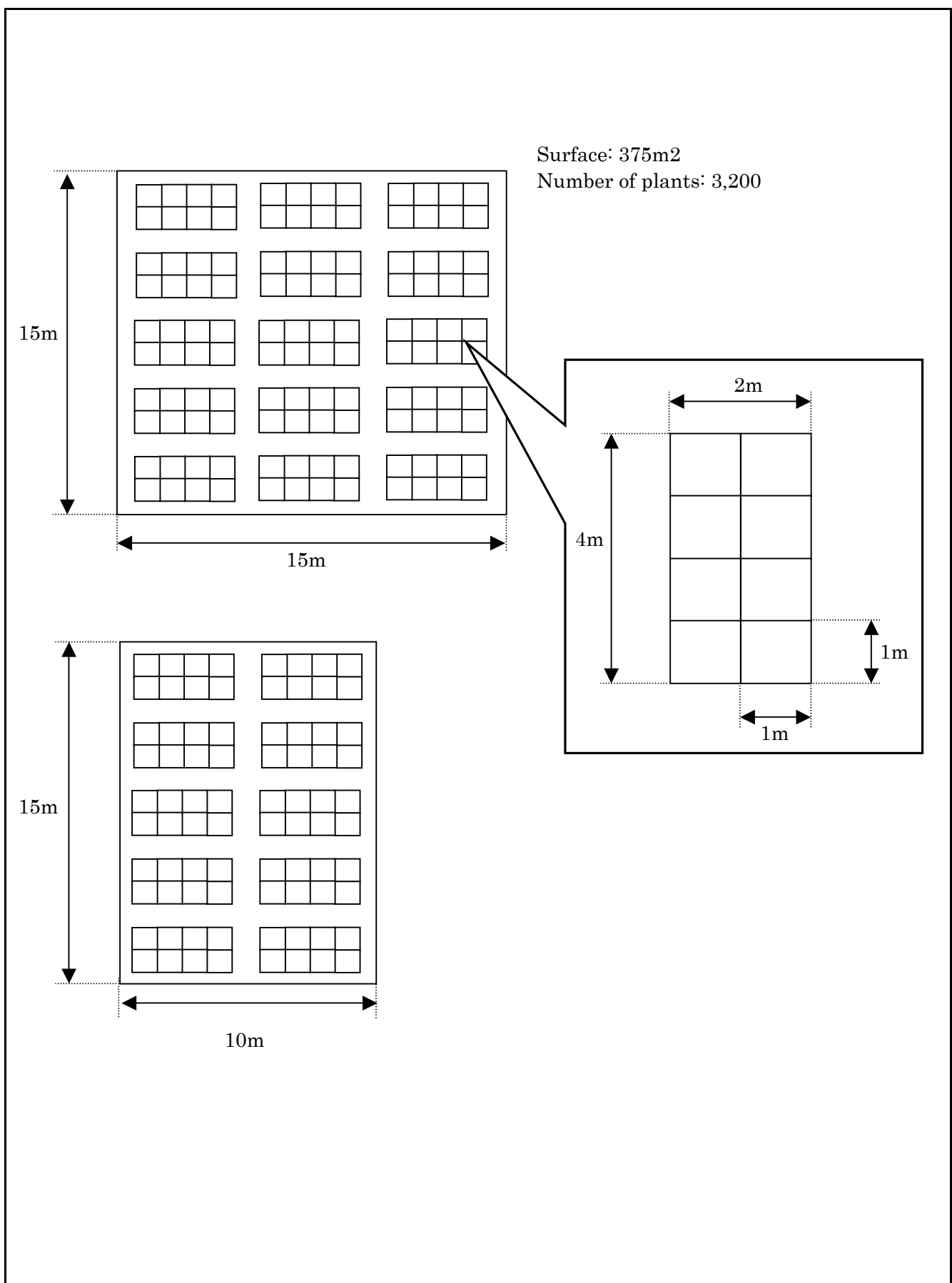
Figure 8.4.1(3) Nursery Arrangement of Vinyl House B
