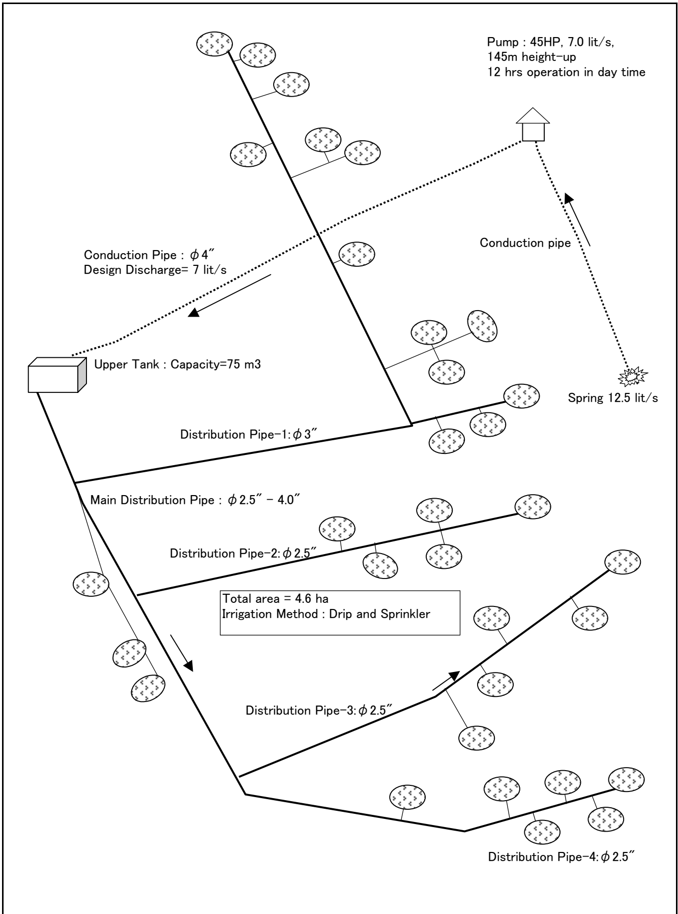
Figure 8.3.1 (5) General Feature of Irrigation System in Yeatzan Rain
