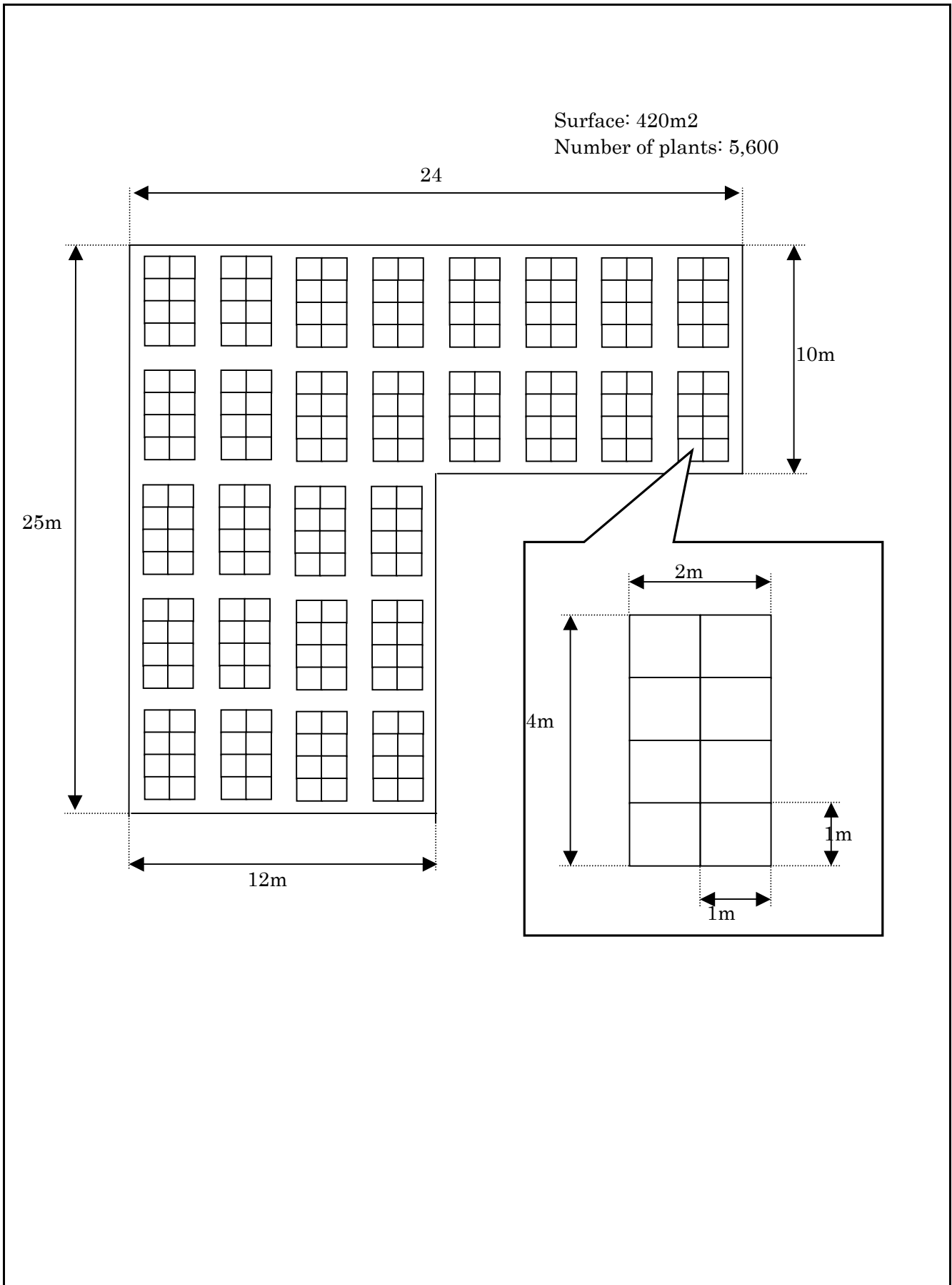
Figure 8.4.1(2) Nursery Arrangement of Vinylhouse A
