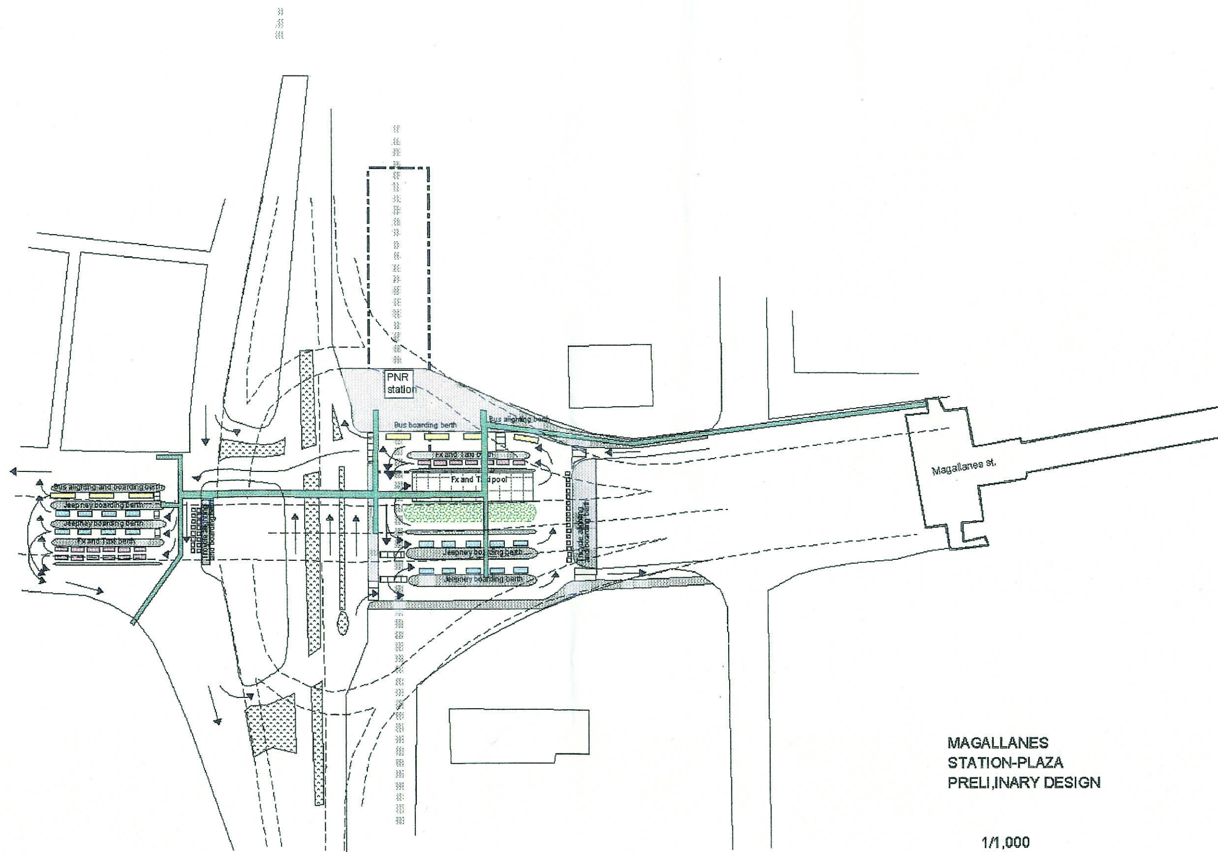
Fig. 8.3.7 Station Plaza Development Plan, Magallanes
