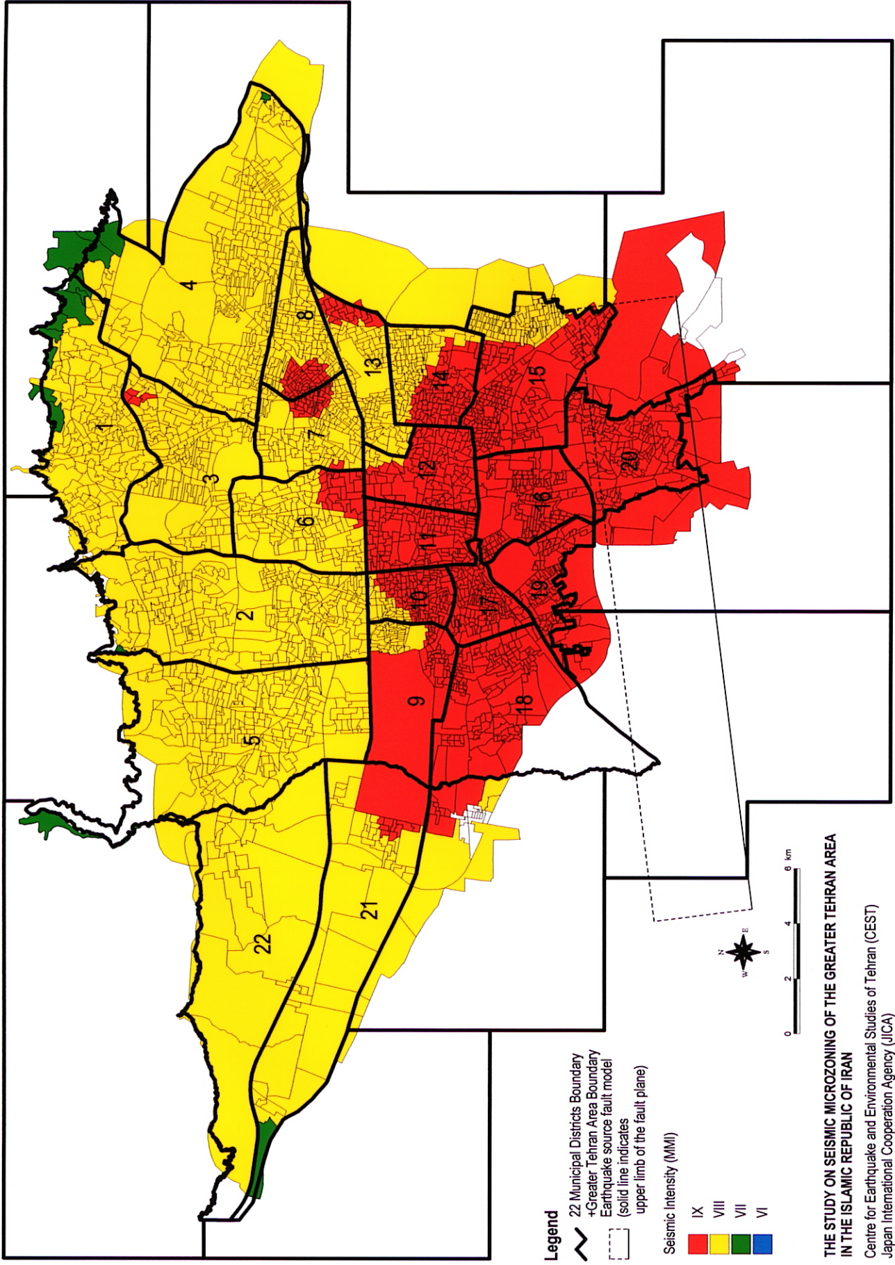
Seismic Intensity Distribution Map (Ray Fault model)
