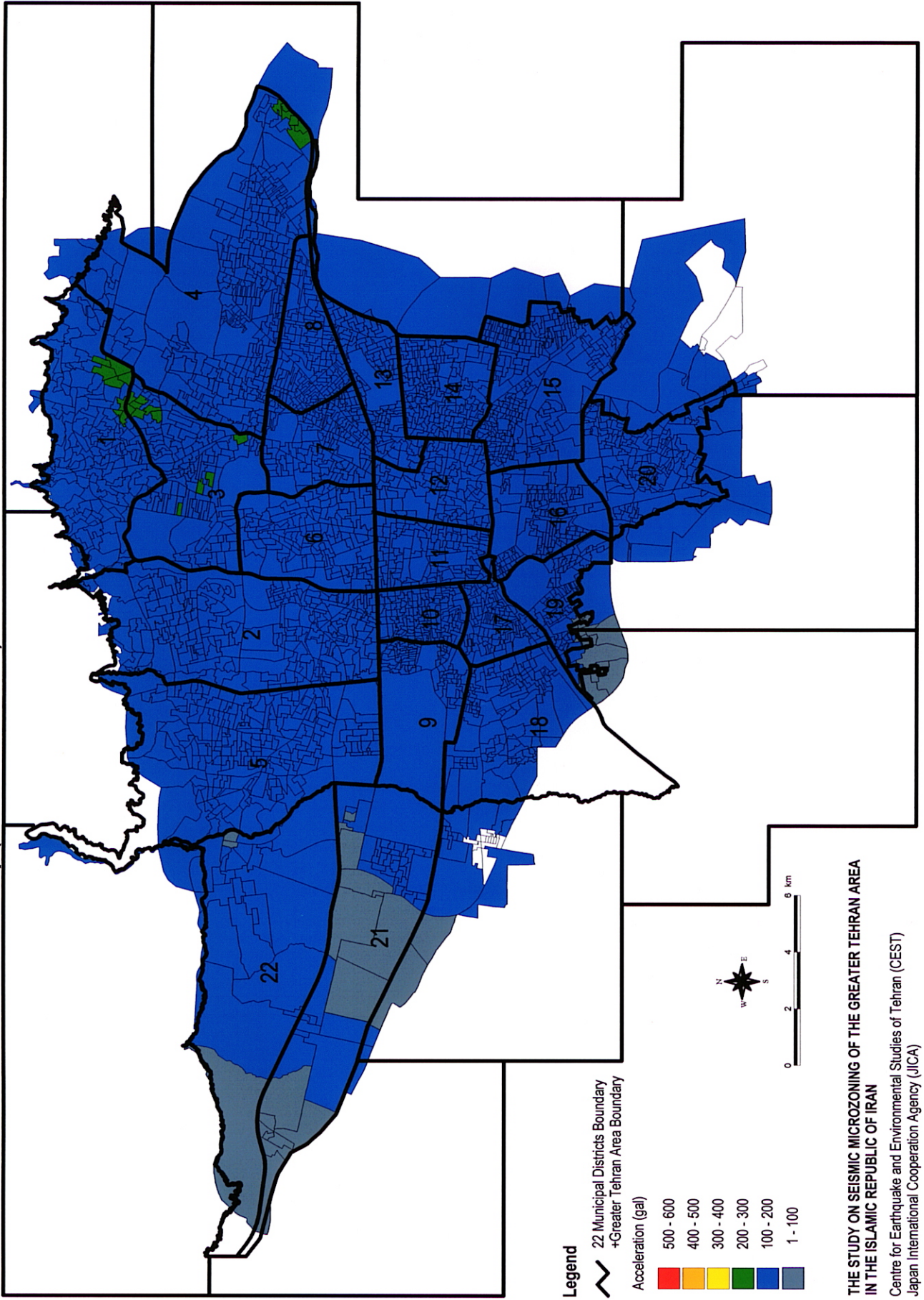
Peak Ground Acceleration Distribution Map (Moshfa Fault model)
