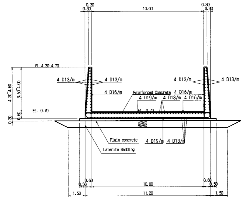
SECTION B-B SCALE 1:200
