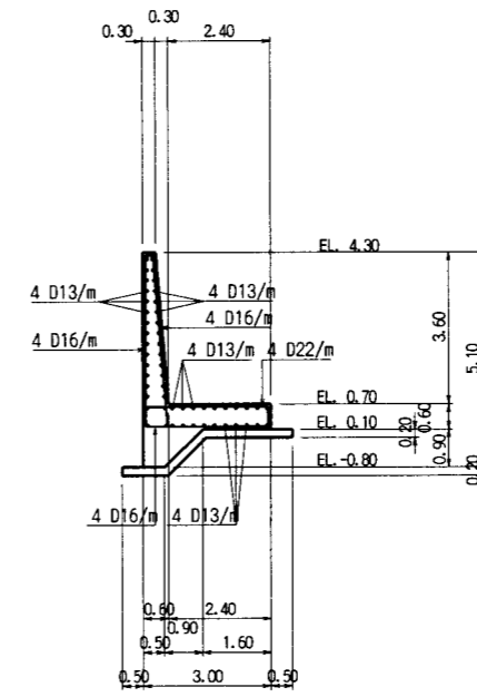
SECTION D-D SCALE 1:200
