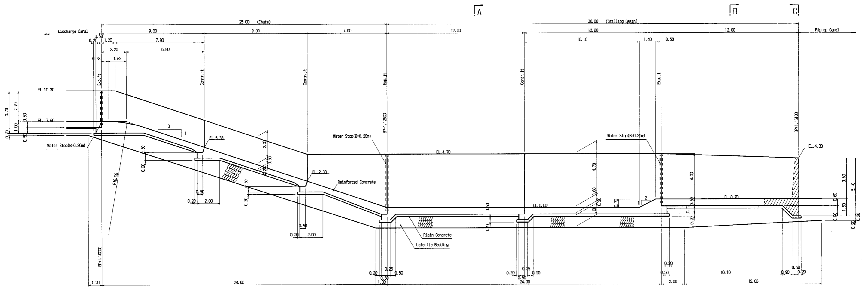
PROFILE SCALE 1:200
