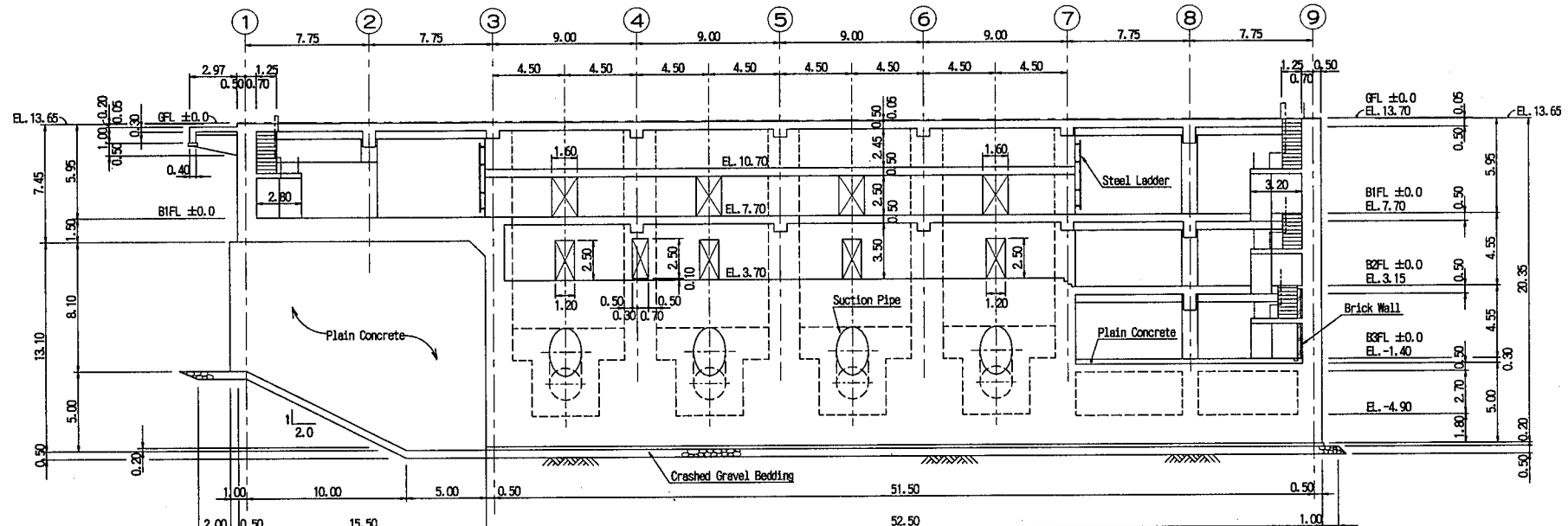
SECTION D-D SCALE 1:400
