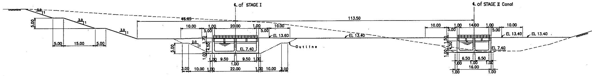
SECTION D - D S=1/1000
