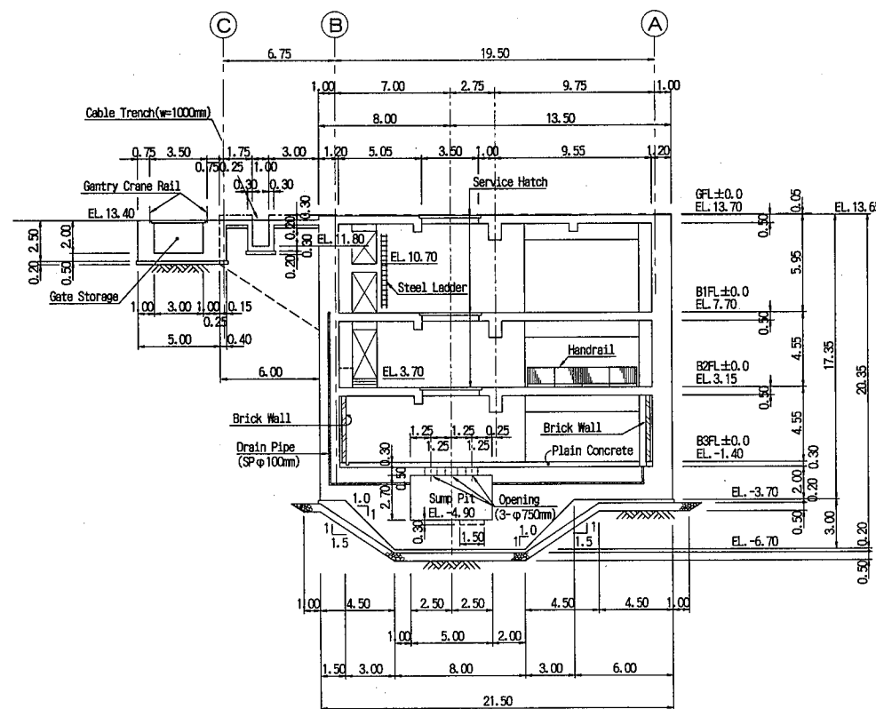
SECTION B-B SCALE 1:400
