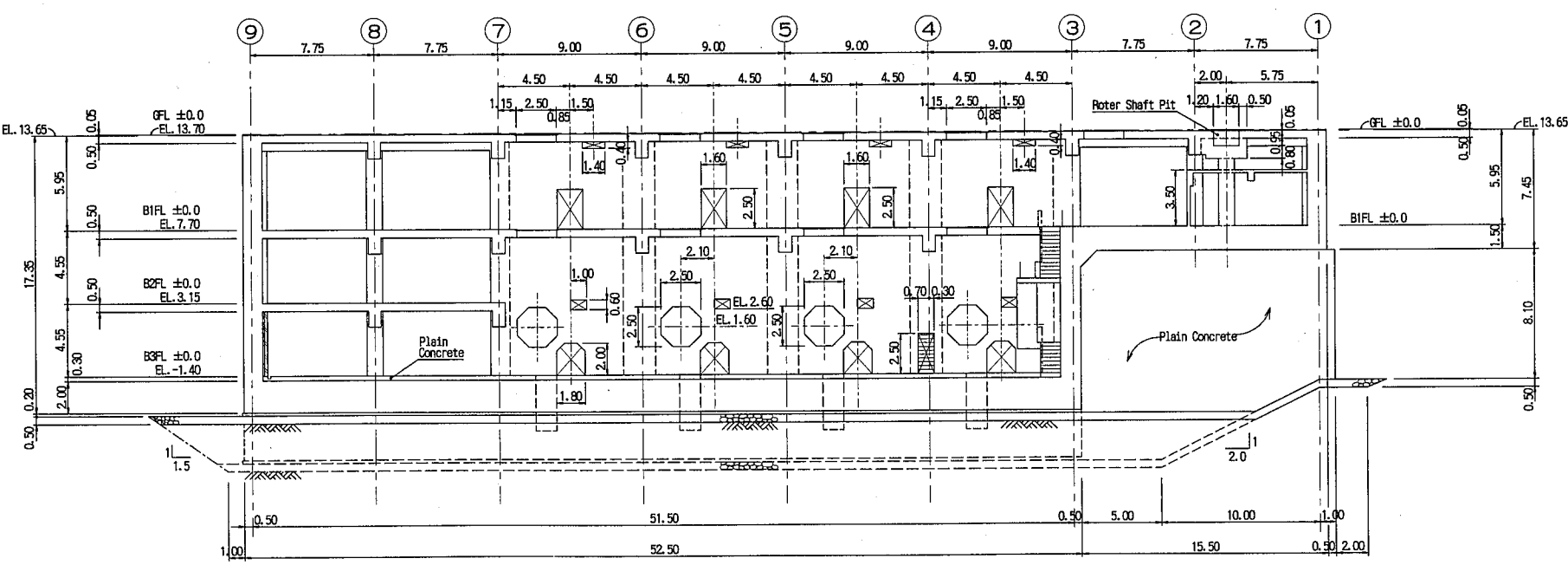
SECTION F-F SCALE 1:400
