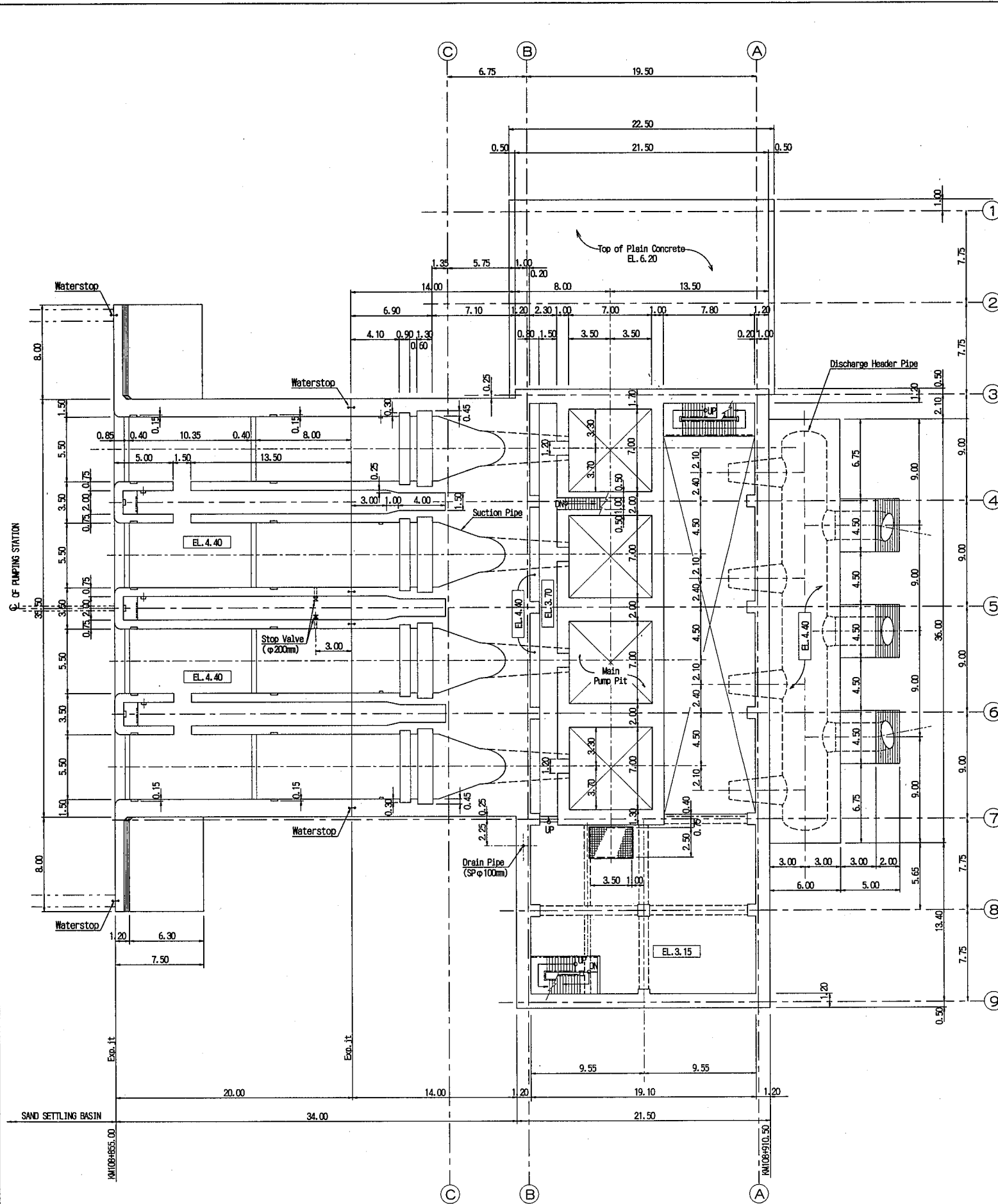
PLAN OF B2 FLOOR SCALE 1:400
