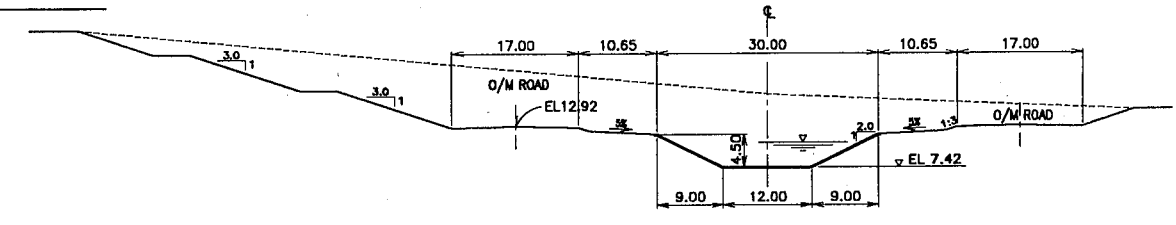
SECTION B-B S=1/1000
