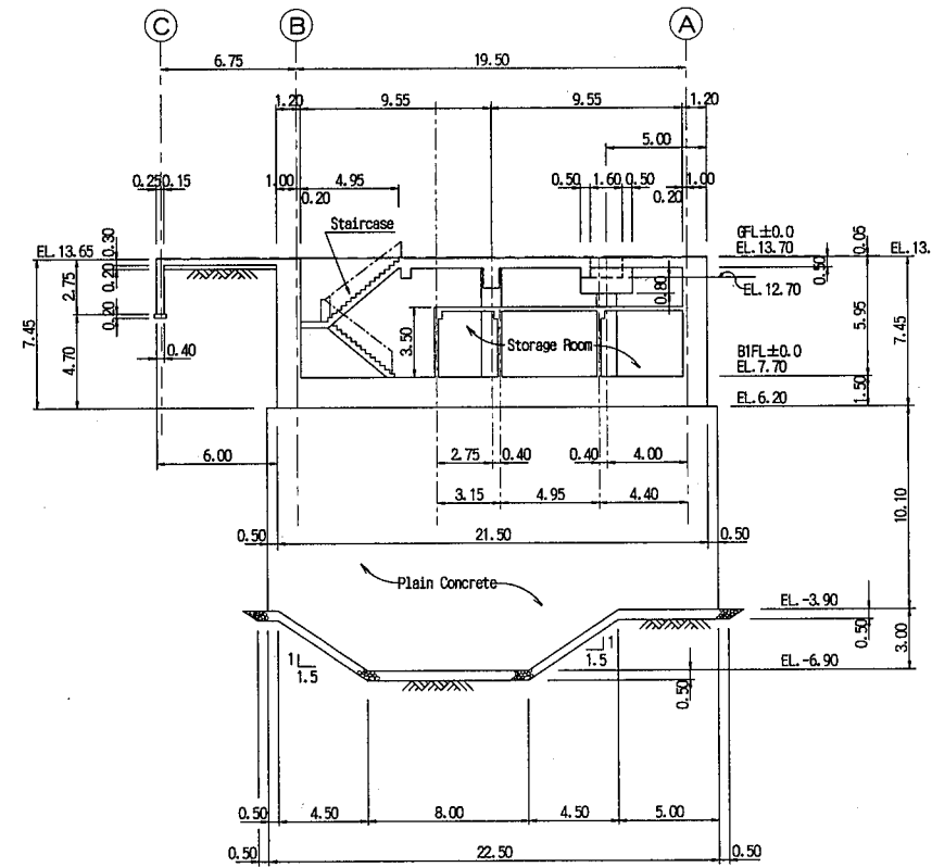
SECTION C-C SCALE 1:400
