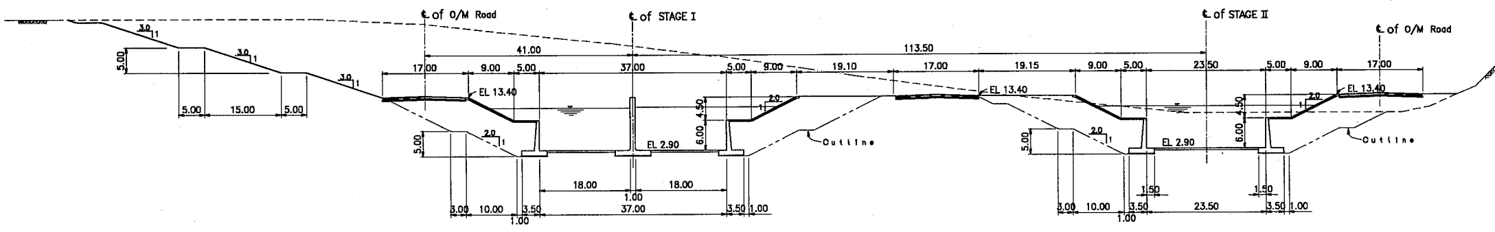
SECTION F - F S=1/1000
