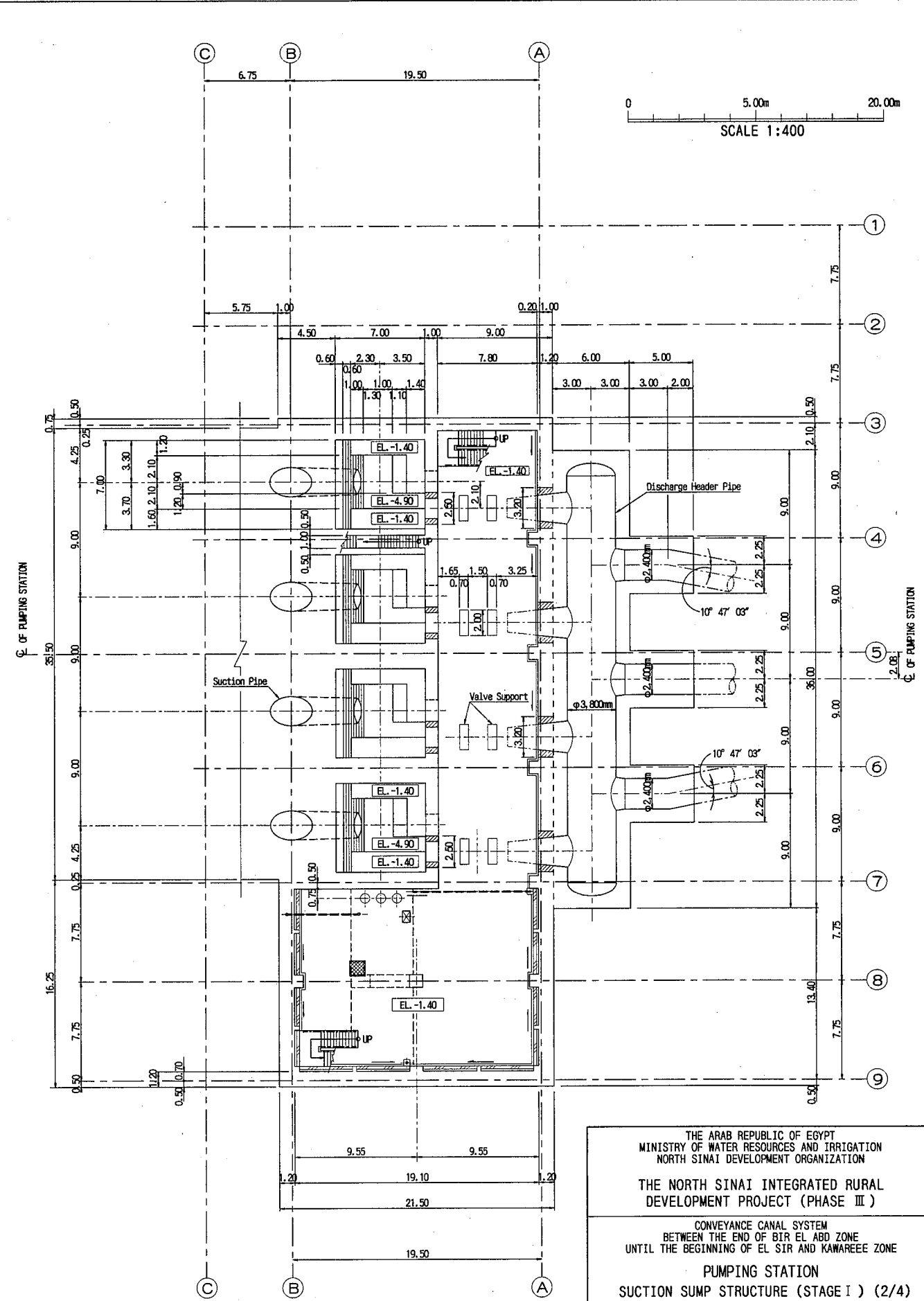
PLAN OF B3 FLOOR SCALE 1:400
