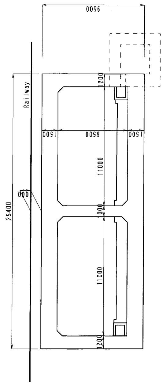
Box Culvert Section
