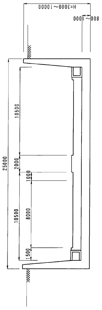
U-Shape Retaining Wall Section
