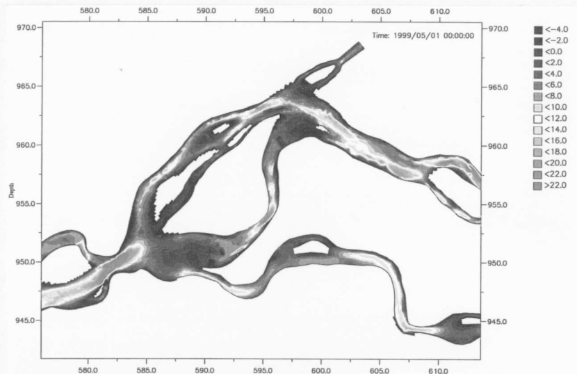
Depth below MSL in m (Alt.B2-1, Initial Condition)
