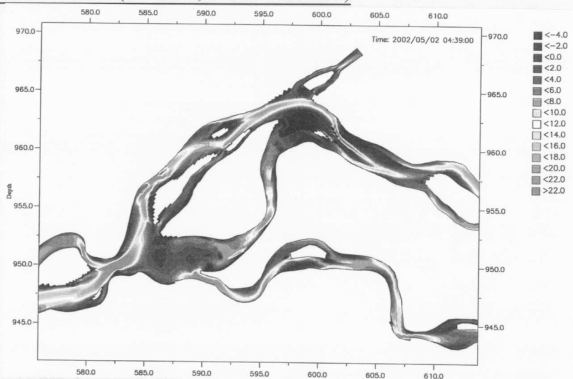
Depth below MSL in m (Alt.B2-1, 3 years after)
