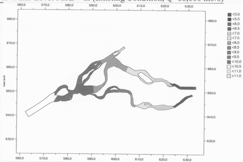
Contour of Water Level MSL + m (Alt.B2-1, Q=66,000 \text{ m}^3/\text{s} )
