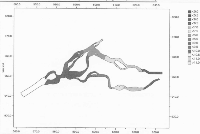
Contour of Water Level MSL + m (Alt.B2-2, Q=66,000 \text{ m}^3/\text{s} )
